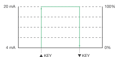
4-20 mA Span check example
