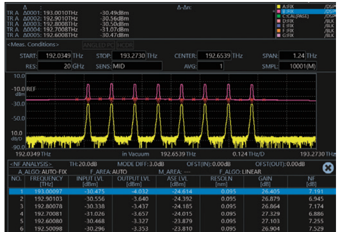
AQ6370E Measurement Screen
