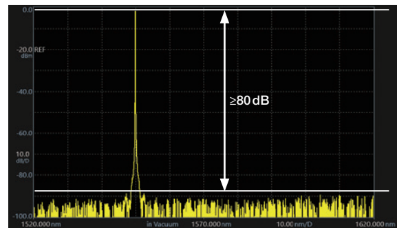
Stray light suppression performance
