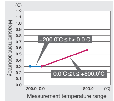
[Example] Measurement accuracy: Pt100 (3851)
