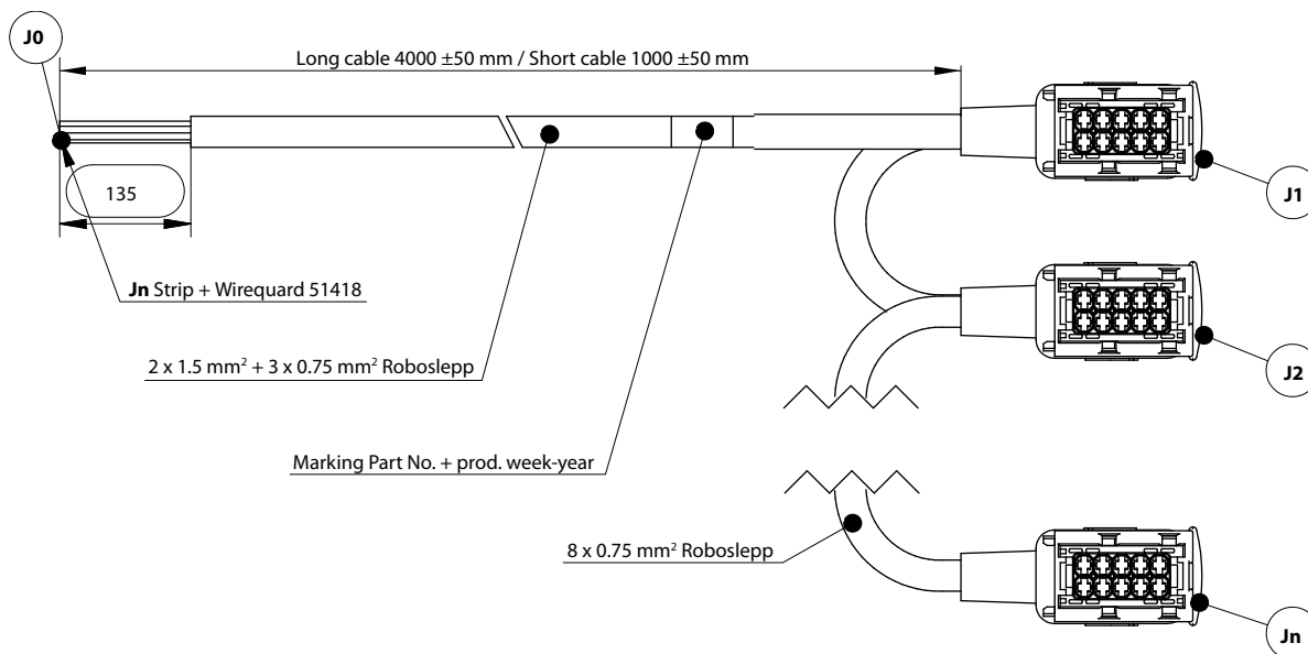
Cable dimensions
