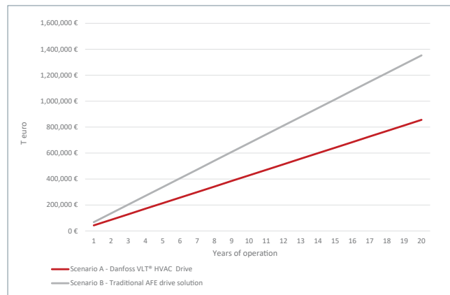
Figure 4. Total cost of electricity losses over time
