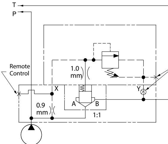
CPF15-10/12-* -20 with remote control
