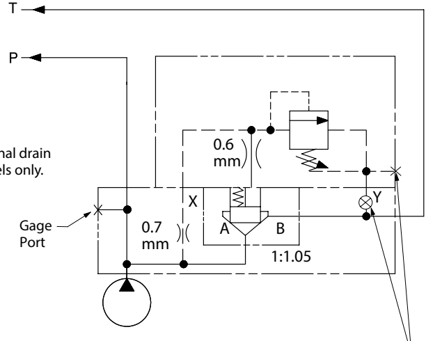
CPF15-06/08-P-* -20 without remote control
