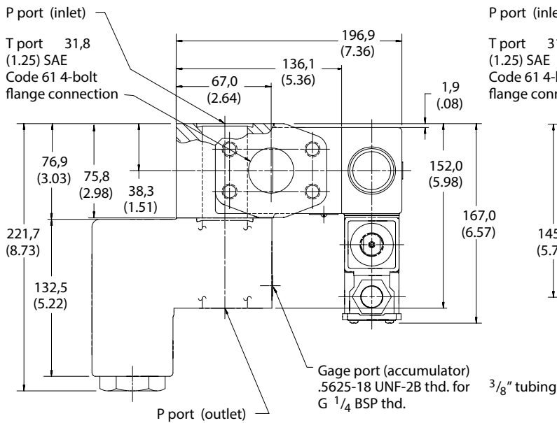
"C" Models Right Angle Check
