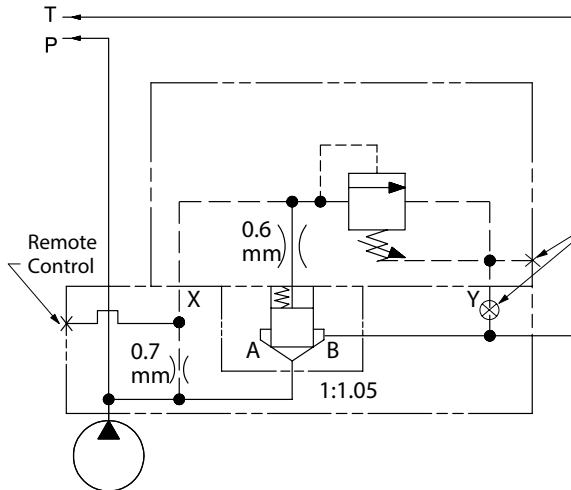
CPF15-06/08-* -20 with remote control
