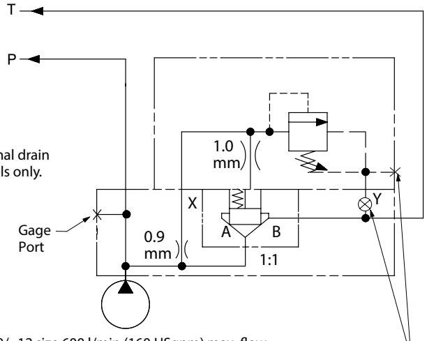
CPF15-10/12-P-* -20 without remote control
