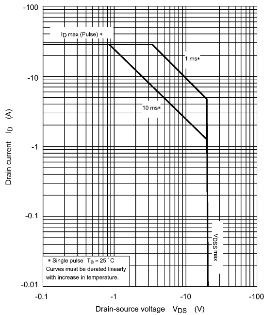
Fig. 8.13 Safe Operating Area (Guaranteed Maximum)
