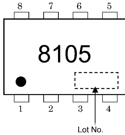
Fig. 7.1 Marking
