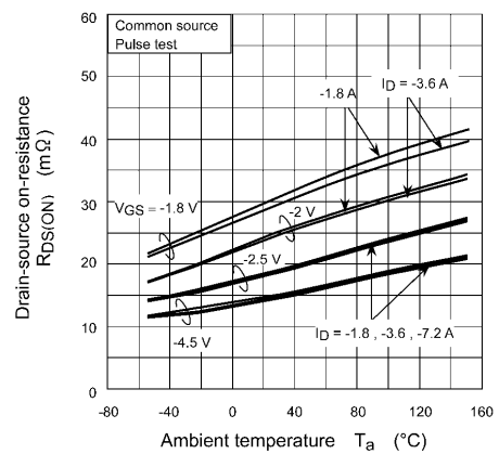
Fig. 8.6 R_{DS(ON)} - T_a
