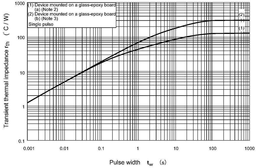
Fig. 8.12 r_{th} - t_w (Guaranteed Maximum)
