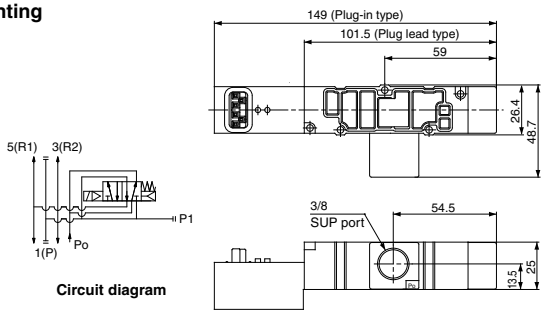
Circuit diagram
