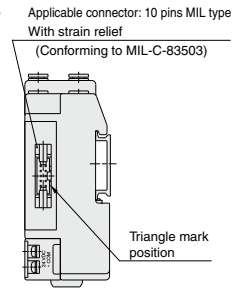
60PH (10 pins)
