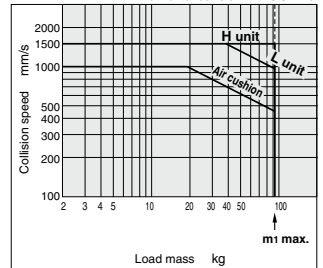
MY1C50
