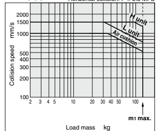
MY1C63
