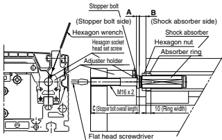
Figure (1) Stroke adjusting section detail
