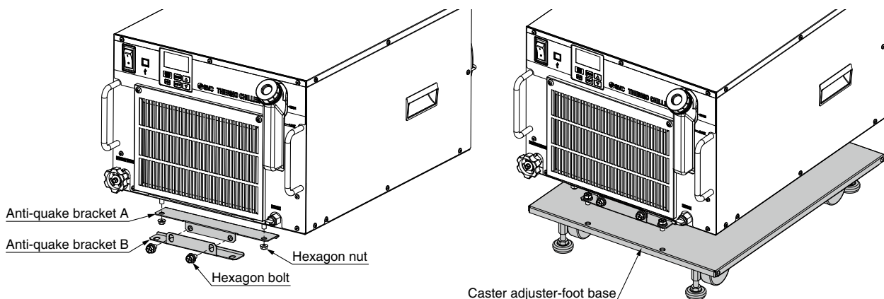
Mounting view
