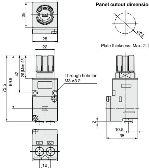
Panel cutout dimensions
