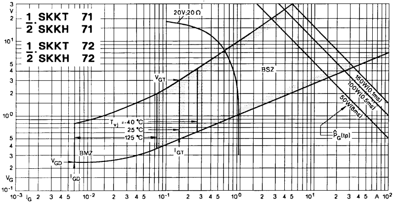
Fig. 10 Gate trigger characteristics
