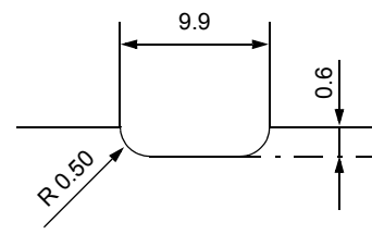
Detail C
