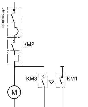
Solution with magnetic motor circuit breaker.
