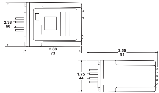
Dimensions of Type JCK60 and JCK70
