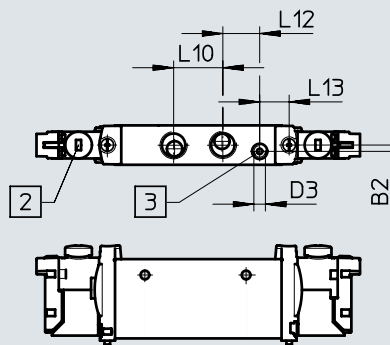
[3] Port for external pilot air supply
