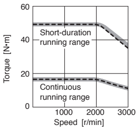
HG-SR3524(B) (Note 1, 2, 3)
