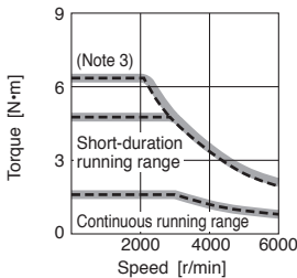
HG-JR2034(B) (Note 1, 2, 4)
