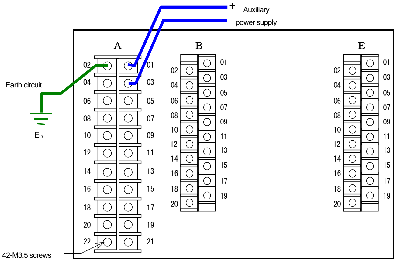
Figure 5.10 Rear view of type CMP1-A02D2 relay (terminal arrangement)
