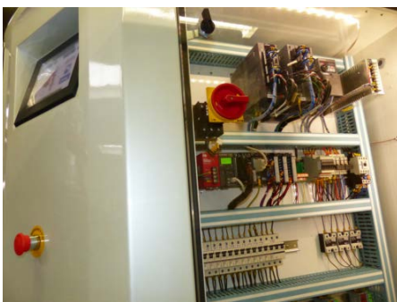
Figure 3: Tubular bag machine Detail: Besides the iQ Platform, the tubular bag machine includes a PLC, a motion controller, servomotors, and GOT2000 HMI from Mitsubishi Electric.
