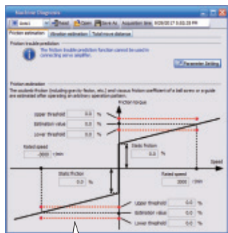
[Machine diagnosis function window on MR Configurator2]
