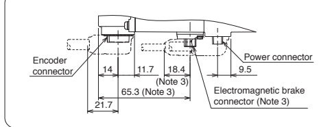
When the cables are led out in the opposite direction of the load side
