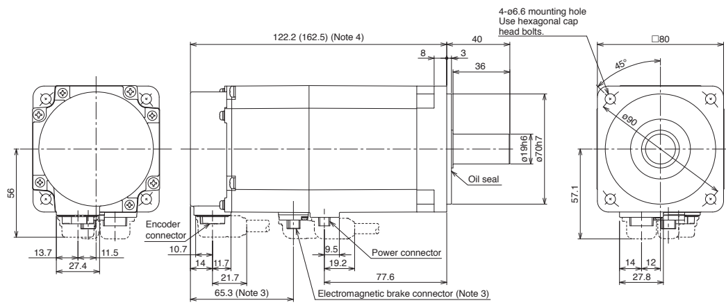
When the cables are led out in the opposite direction of the load side
