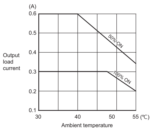
*1 Temperature derating chart
