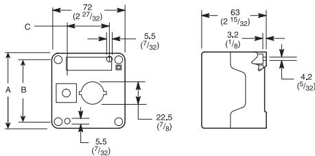
Plastic Enclosures [mm (in.)]
