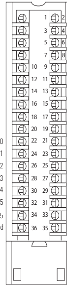
1756-0A16I
