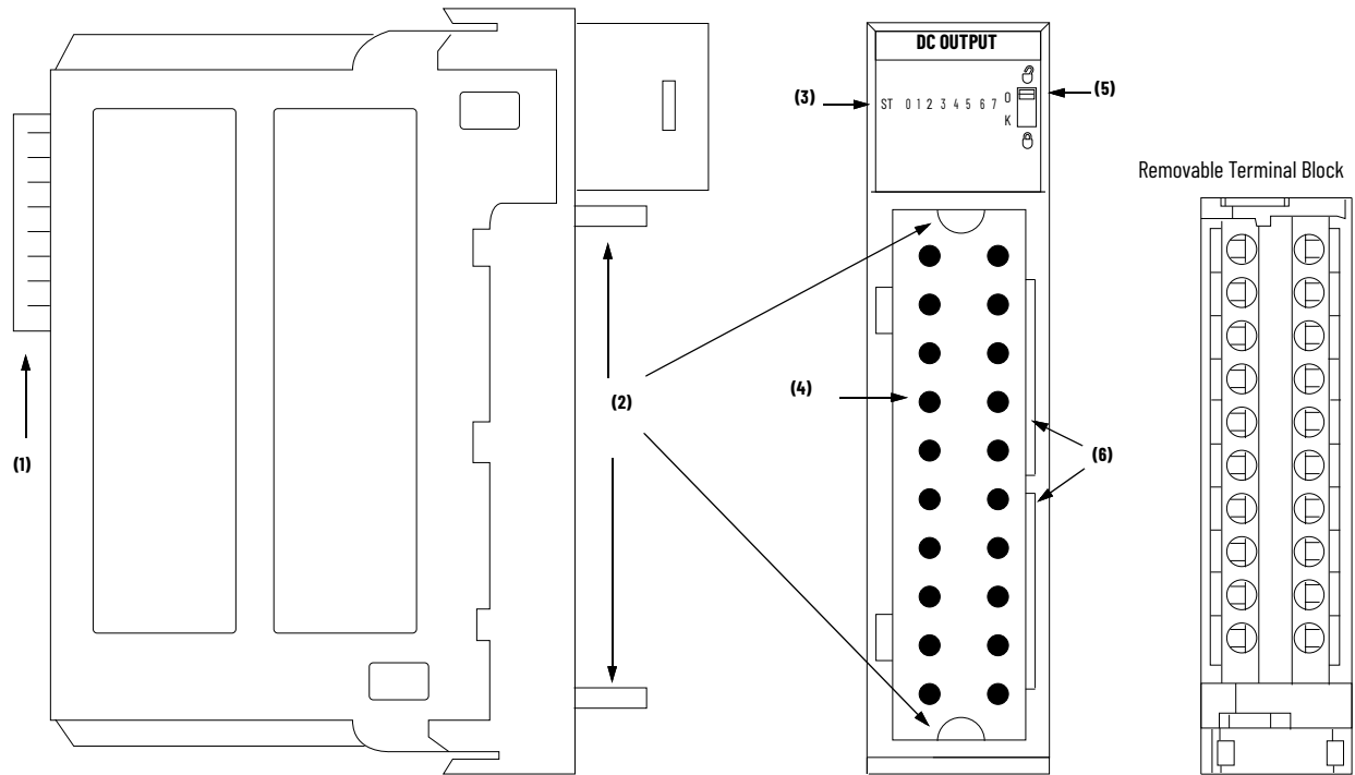
Figure 1 - Parts Illustration
