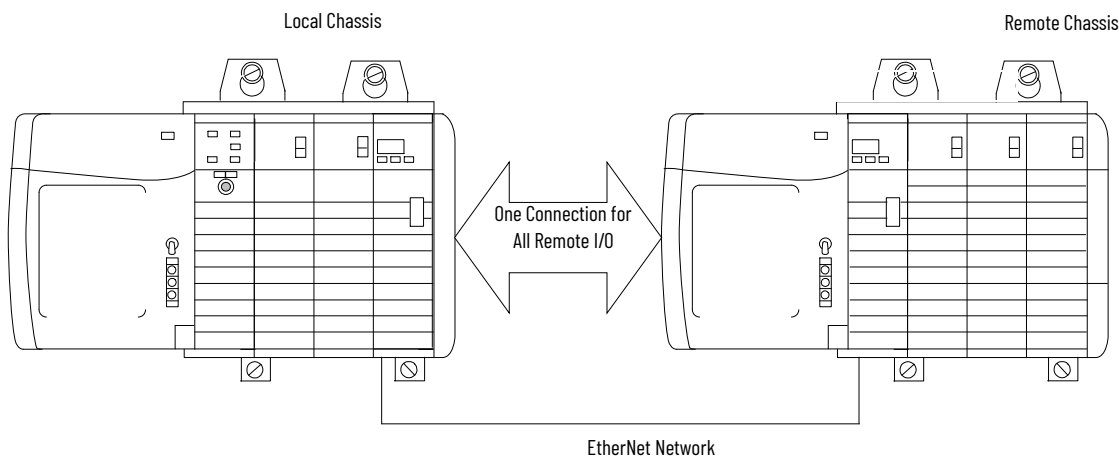
Figure 4 - Rack-optimized Connection
