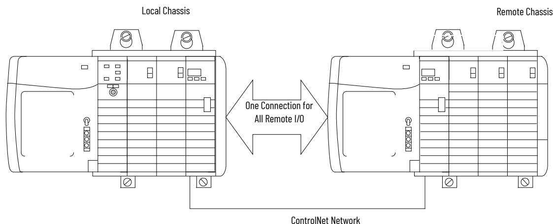
Figure 25 - Rack-optimized Connection
