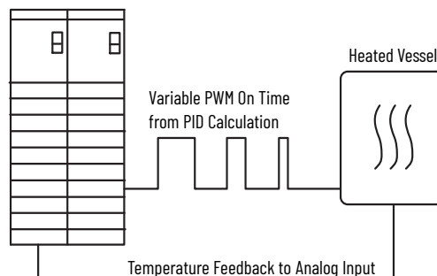
Figure 14 - PWM for Time Proportioned Control
