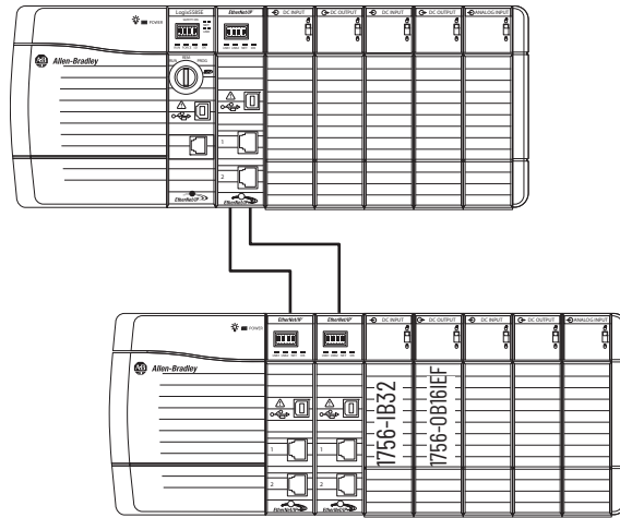
Figure 18 - Single Controller
