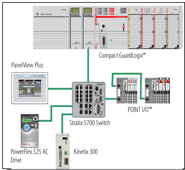
The Integrated Architecture System Scalable integrated safety, motion control and visualization capabilities for applications of all sizes and complexities.
