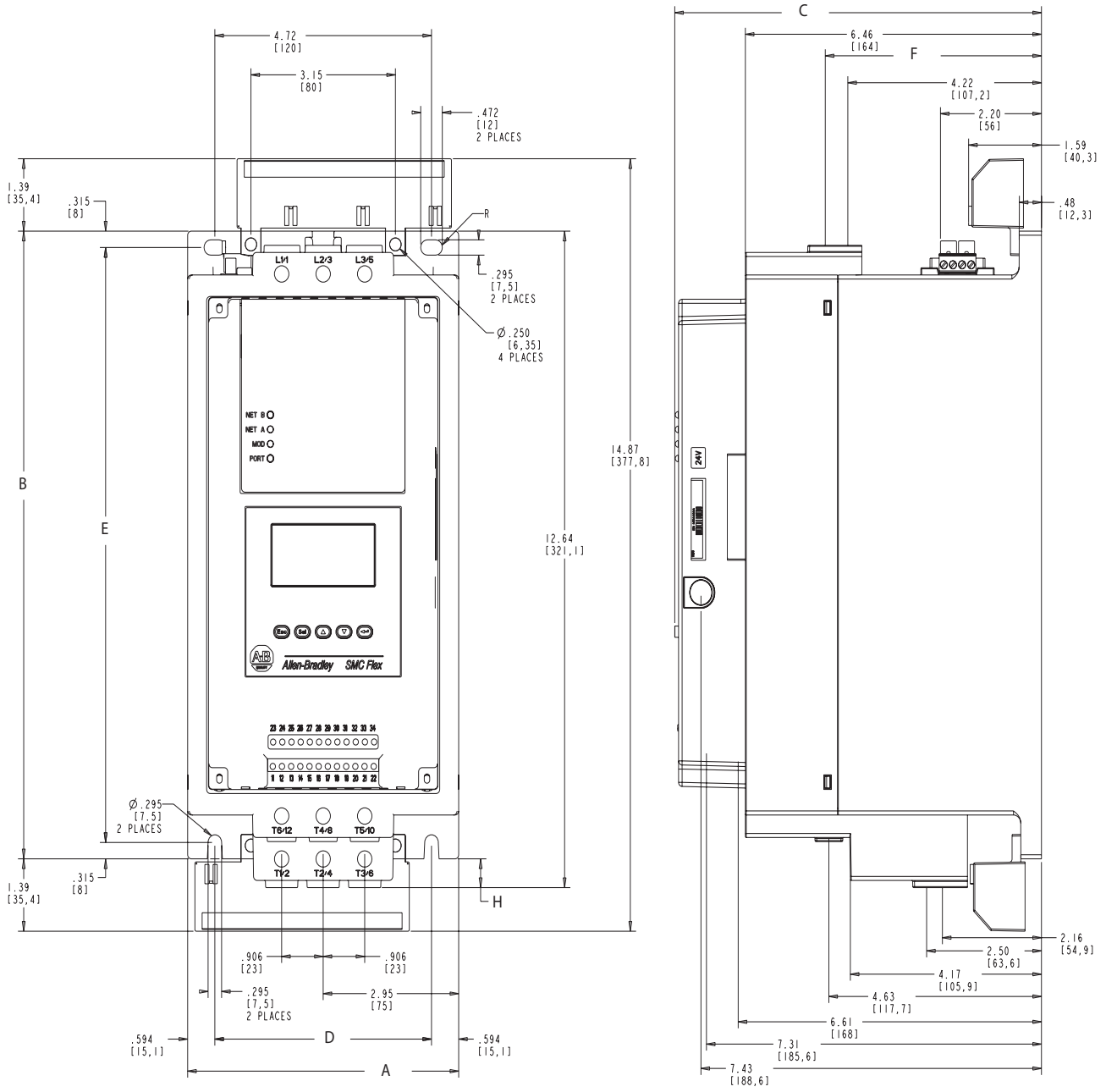
Figure 13 - 5...85 A Controllers
