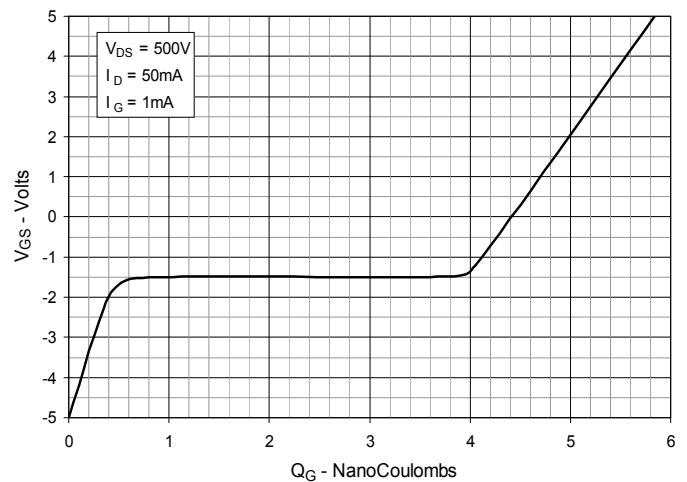
Fig. 12. Gate Charge
