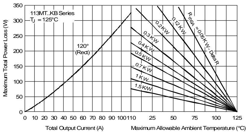
Fig. 13 - Total Power Loss Characteristics
