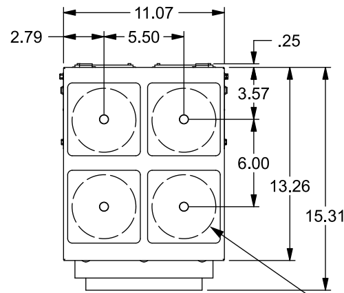
FRONT VIEW SHOWN WITH COVER AND SHIELDS REMOVED
