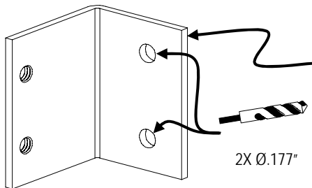
Dimensions for Welded or Screw mounting the cover catch
