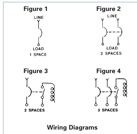
Switching Neutral
