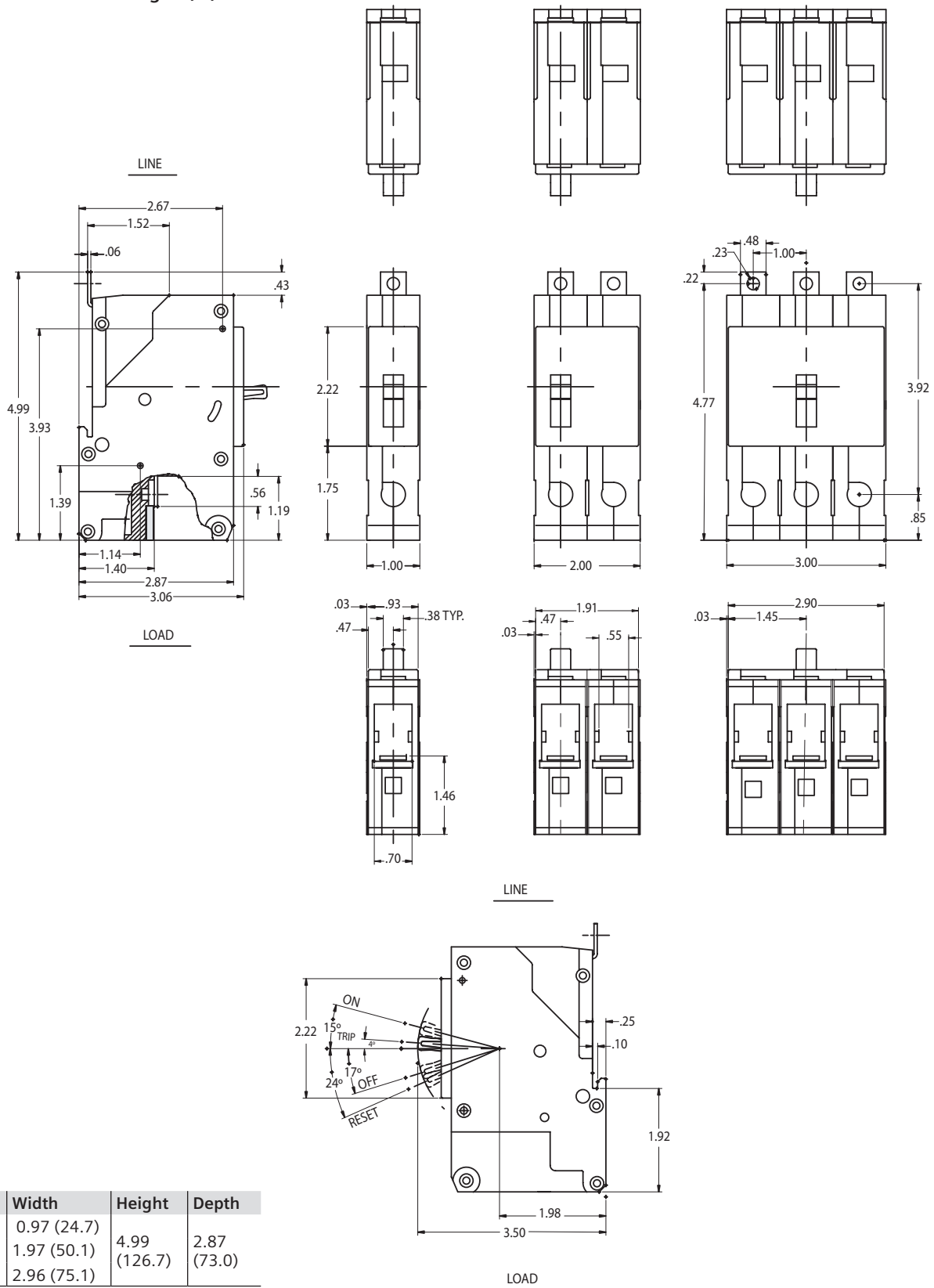
GB Frame Outline Drawing – 1, 2, 3 Pole
