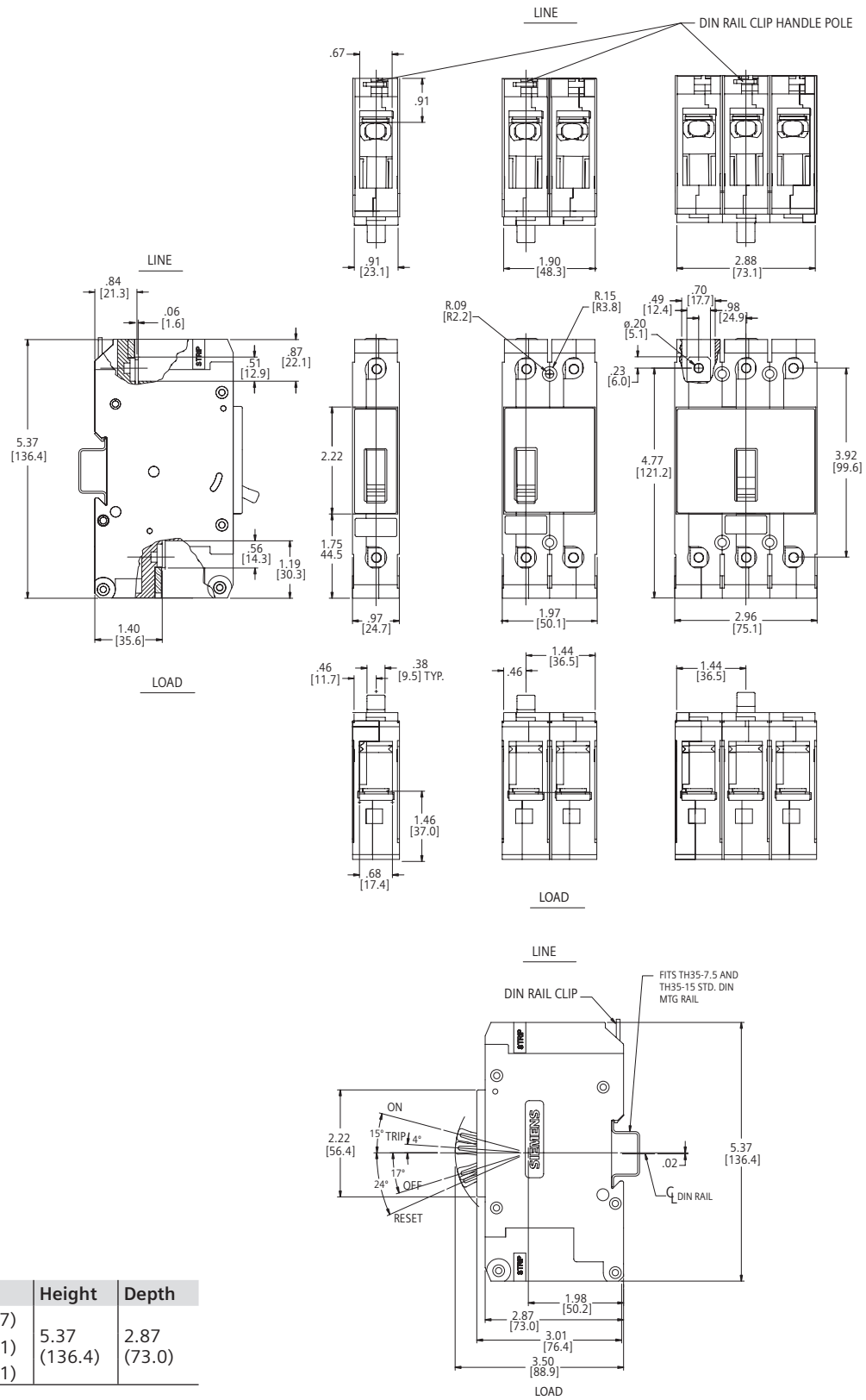
GG/GB2 Frame Outline Drawing – 1, 2, 3 Pole
