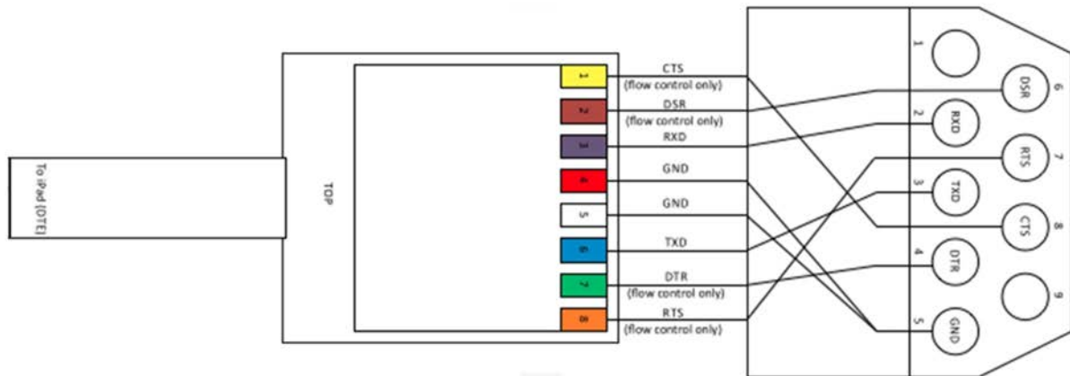
Figure 6-1 C2-RJ45V Cable Pinouts
