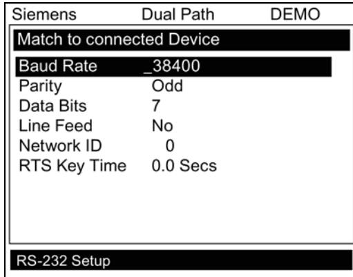
Figure 3-2 RS-232 Setup
