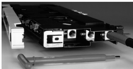
Fig. 5: Size 00, view of 3 terminals, 1 cable connected
