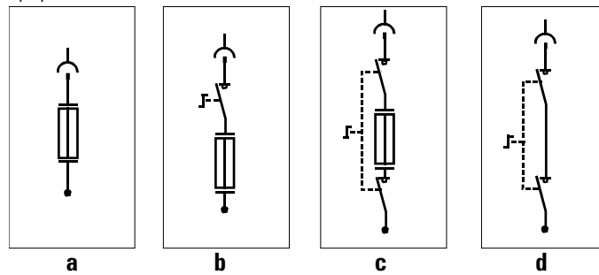
Fig 2: Electrical design
