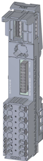
Figure 5-25 BU type D0, dark-colored version, without AUX terminals, supply over supply terminals
