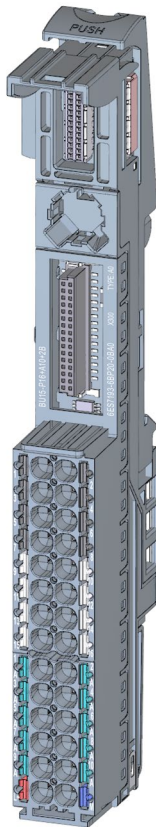
Figure 5-5 BU type A0, dark-colored version, with AUX terminals
