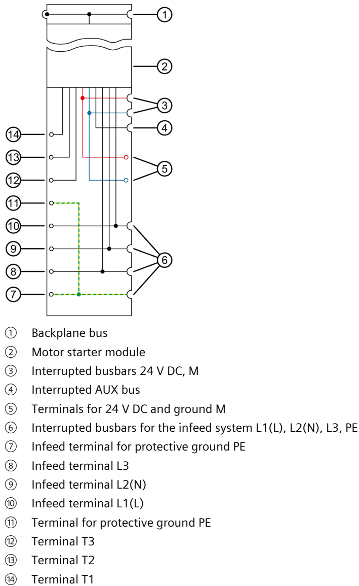
Figure 6-2 Block diagram BaseUnit with 24 V DC and 500 V AC infeed
