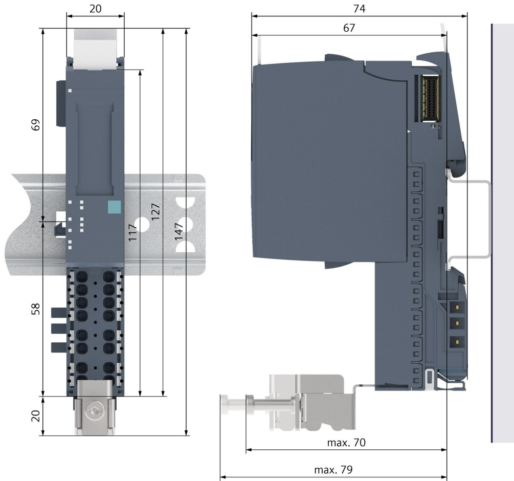
Figure B-3 Dimension drawing BU20-P12+A4+0B
