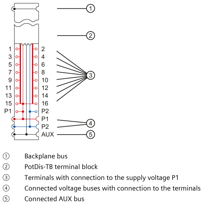
Figure 7-4 Block diagram of the PotDis-BU type P1, dark-colored version
