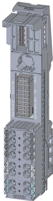
Figure 5-27 BU type F0, dark-colored version, with AUX terminals, supply over supply terminals
