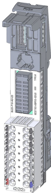
Figure 5-29 BU type U0, light-colored version without AUX terminals
