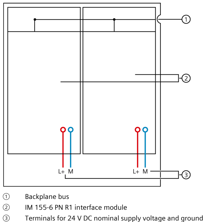
Figure 4-2 Circuit diagram of BU type M0
