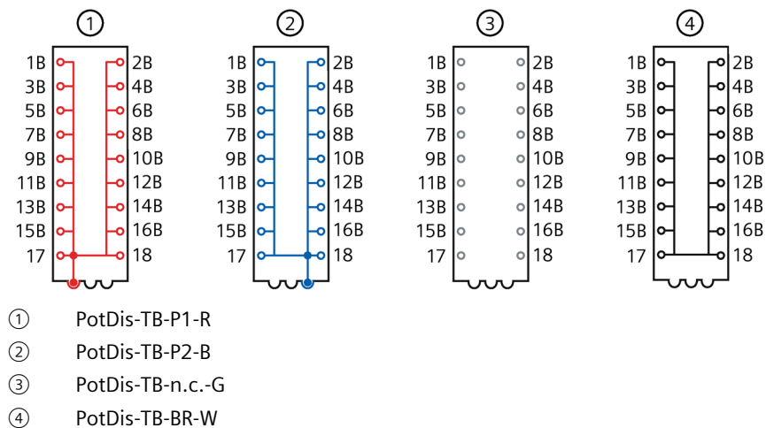
Figure 7-10 PotDis-TB block diagram
