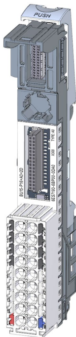
Figure 5-3 BU type A0, light-colored version, without AUX terminals
