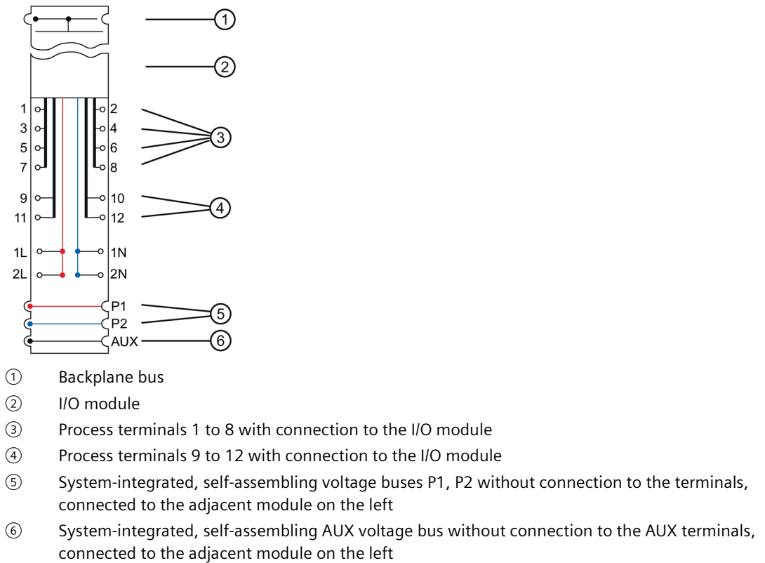
Figure 5-20 Circuit diagram of the BU type B1, dark-colored version, without AUX terminals, supply over supply terminals
