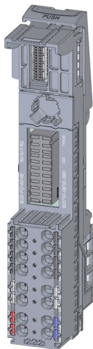
Figure 5-19 BU type B1, dark-colored version, without AUX terminals, supply over supply terminals
