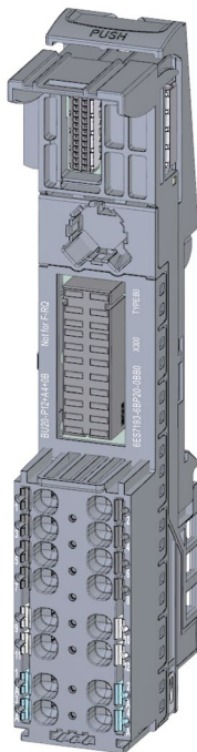
Figure 5-17 BU type B0, dark-colored version, with AUX terminals, supply over P1, P2 busbar
