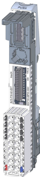
Figure 5-11 BU type A1, light-colored version, without additional terminals
