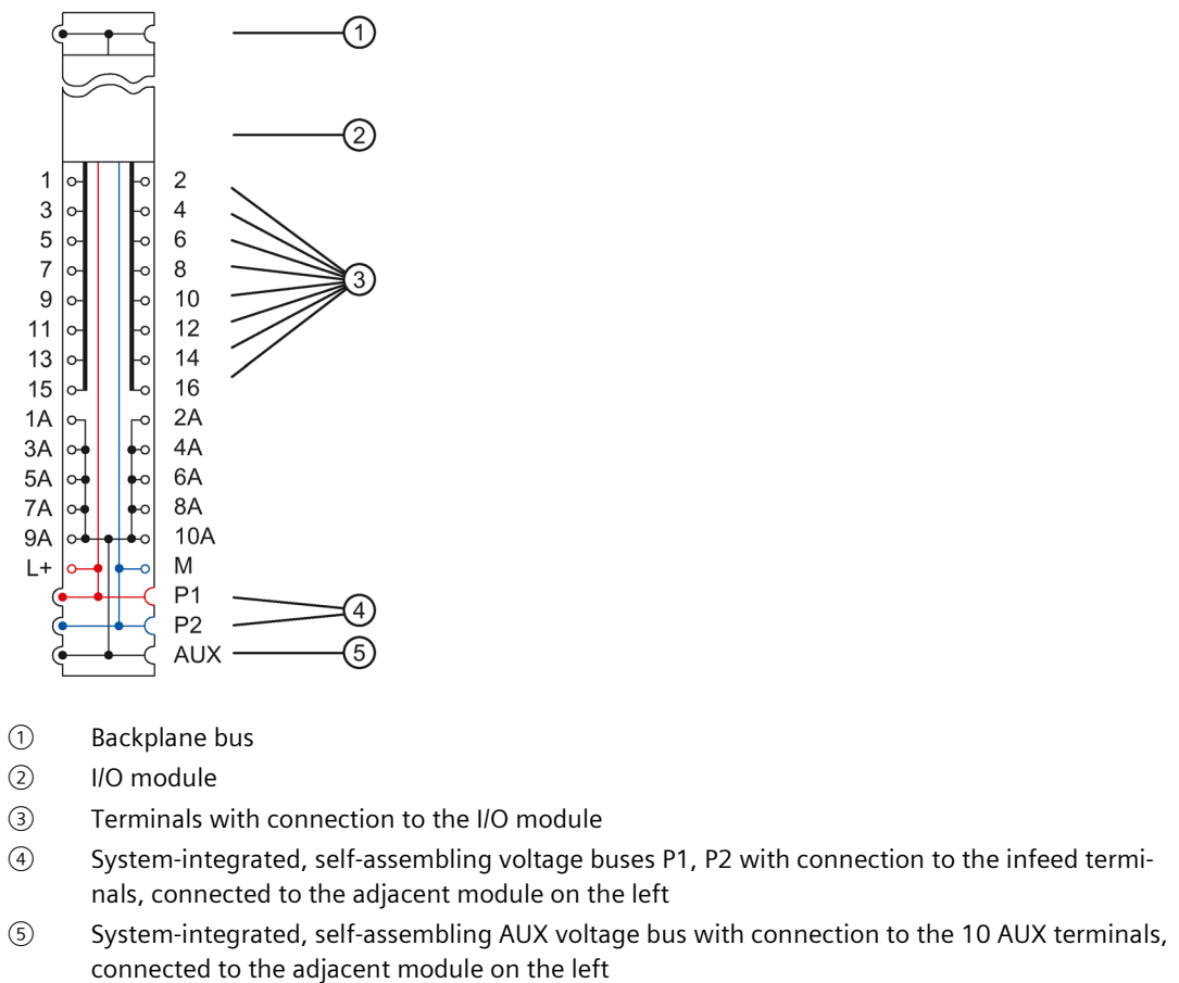
Figure 5-6 Block diagram of the BU type A0, dark-colored version, with AUX terminals
