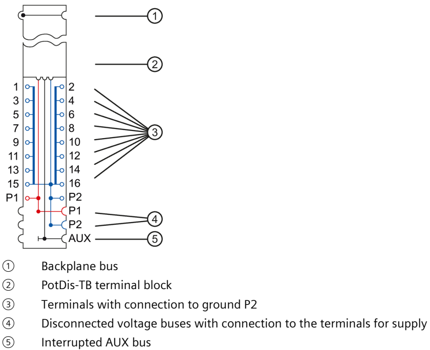
Figure 7-6 Block diagram of the PotDis-BU type P2, light-colored version
