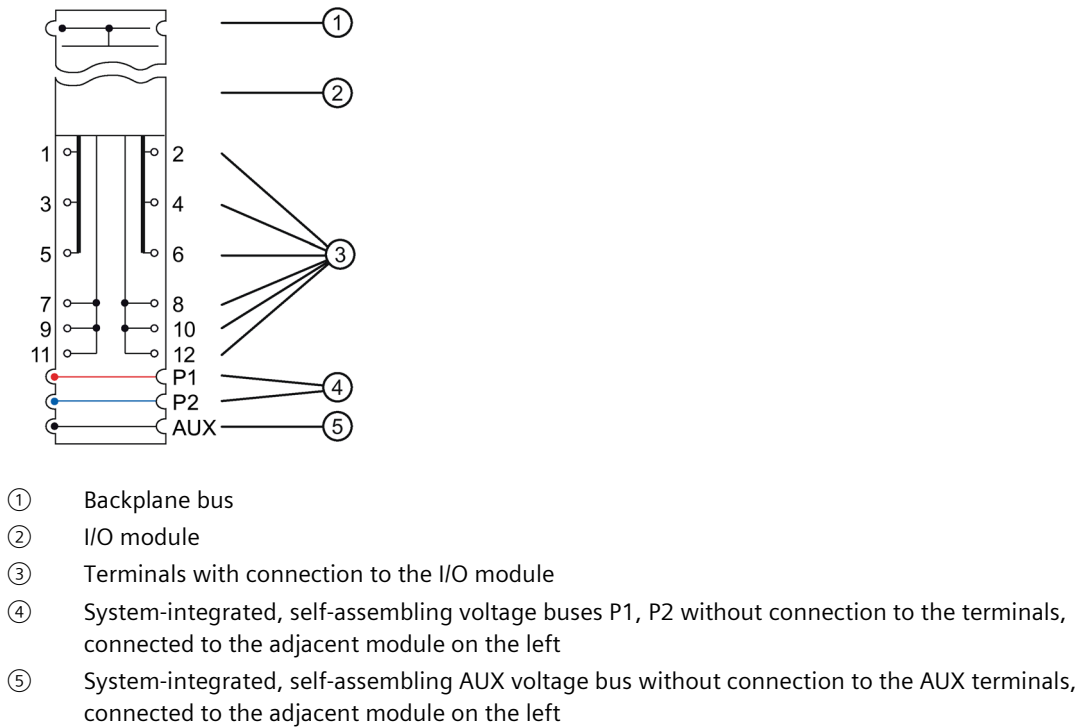
Figure 5-26 Block diagram of the BU type D0, dark-colored version, without AUX terminals, supply over supply terminals
