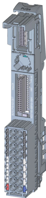
Figure 5-15 BU type A1, dark-colored version, without additional terminals
