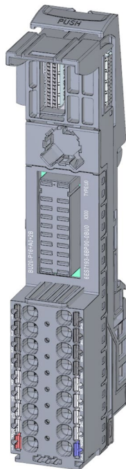
Figure 5-31 BU type U0, dark-colored version, without AUX terminals
