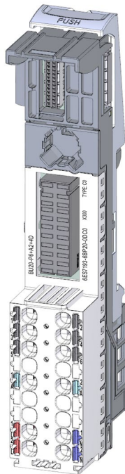
Figure 5-21 BU type C0, light-colored version, with AUX terminals, supply over supply terminals
