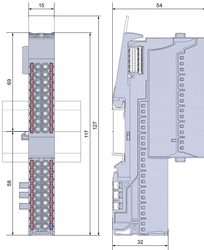
Figure D-1 Dimension drawing of PotDis BU-P1/B-R with plugged-in terminal block
