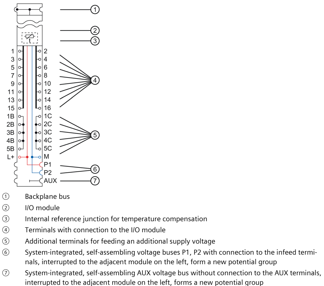
Figure 5-10 Block diagram of the BU type A1, light-colored version, with additional terminals
