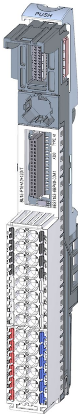
Figure 5-9 BU type A1, light-colored version, with additional terminals
