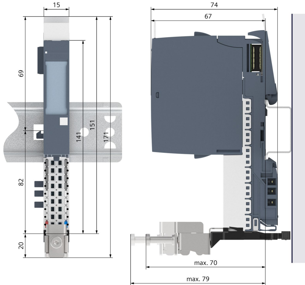
Figure B-2 Dimension drawing BU15-P16+A0+2D
