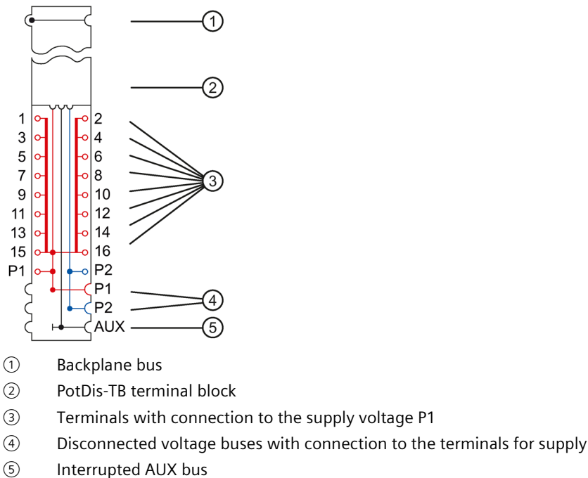
Figure 7-2 Block diagram of the PotDis-BU type P1, light-colored version
