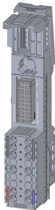
Figure 5-23 BU type C1, dark-colored version, with AUX terminals, supply over P1, P2 busbar
