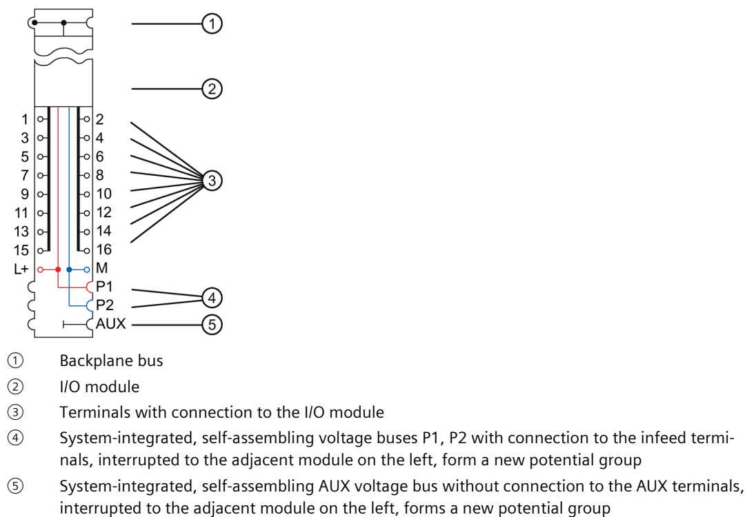
Figure 5-4 Block diagram of the BU type A0, light-colored version, without AUX terminals
