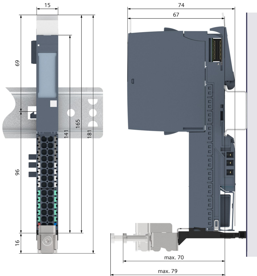
Figure B-1 Dimension drawing BU15-P16+A10+2D
