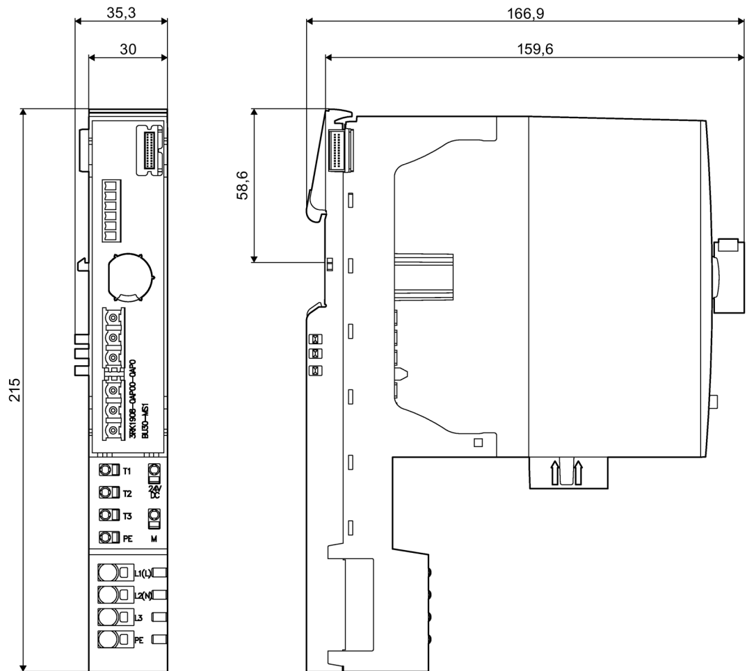
Figure C-1 Dimension drawing BU30-MS1
