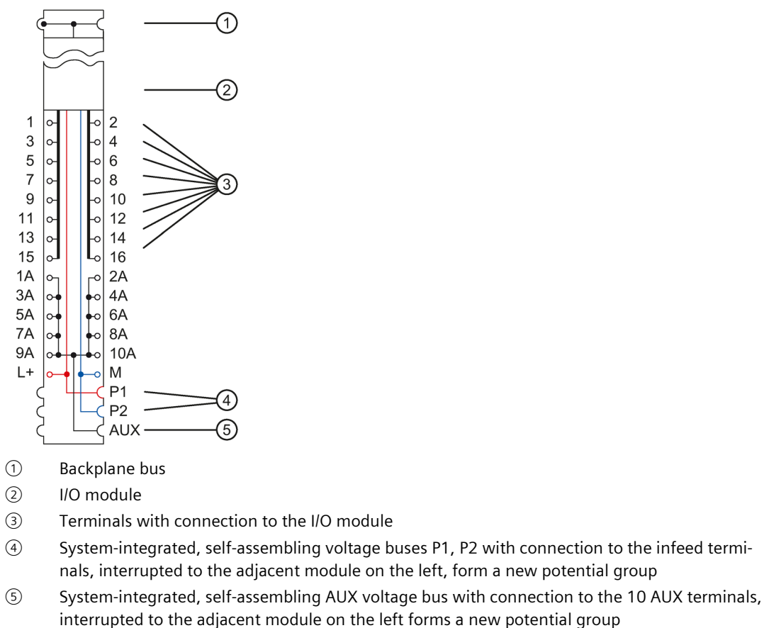
Figure 5-2 Block diagram of the BU type A0, light-colored version with AUX terminals
