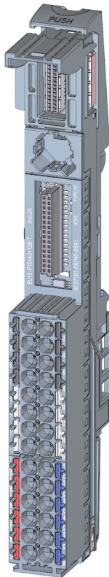
Figure 5-13 BU type A1, dark-colored version, with additional terminals
