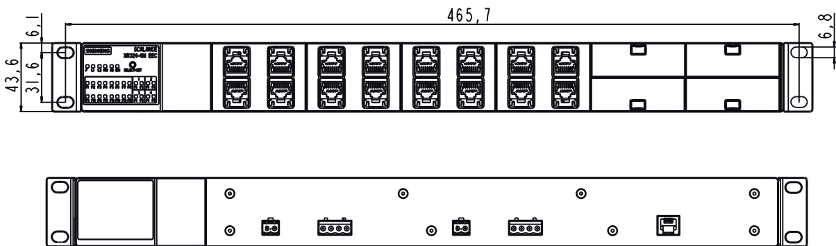
Figure 9-1 Housing front and rear
