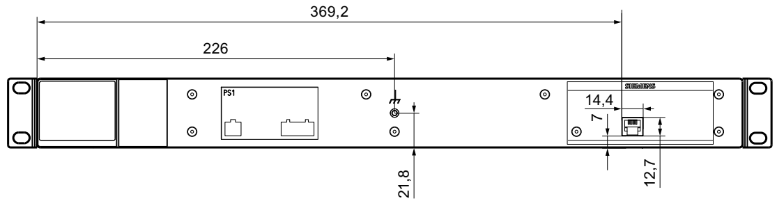
Figure 9-4 Example of a XR324-4M EEC (1 x 24 VDC, cable outlet front)
