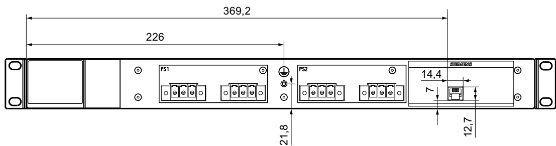
Figure 9-3 Example of a XR324-4M EEC (2 x 100 to 240 VAC, cable outlet front)
