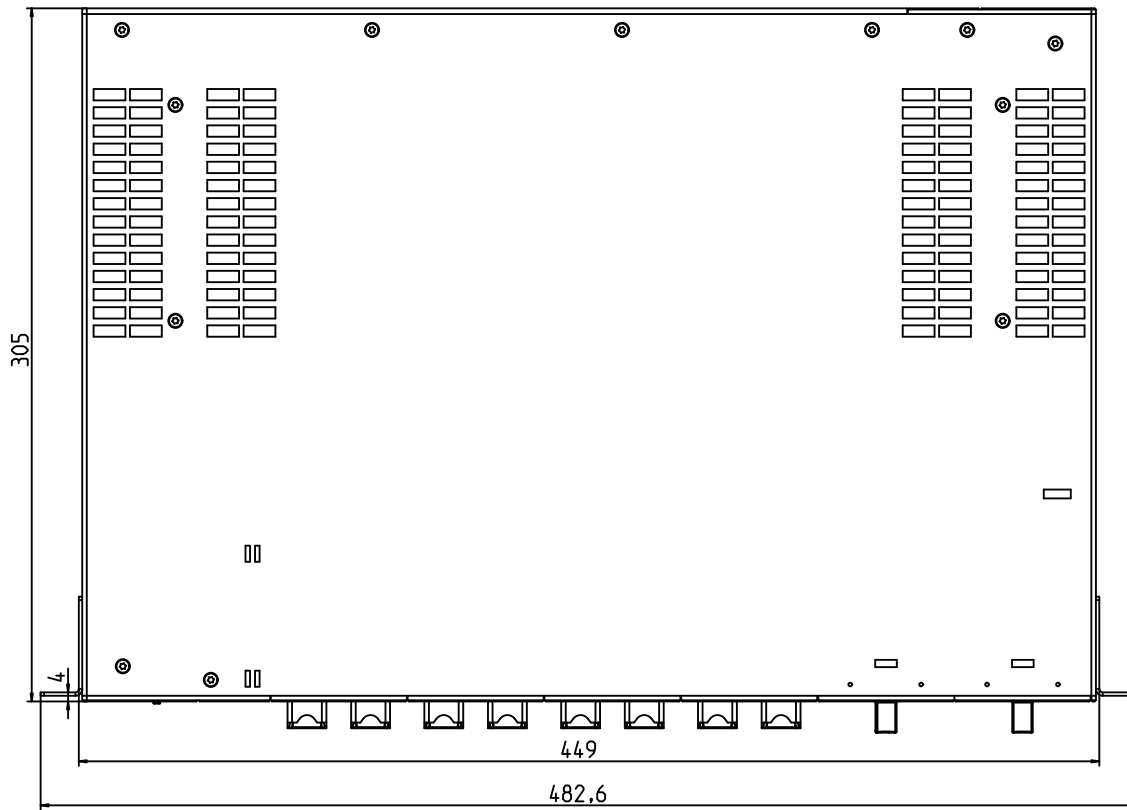
Figure 9-2 Top of the housing
