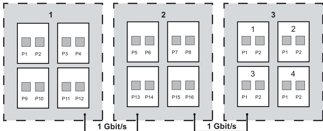
Figure 8-2 Block architecture of the XR324-4M
