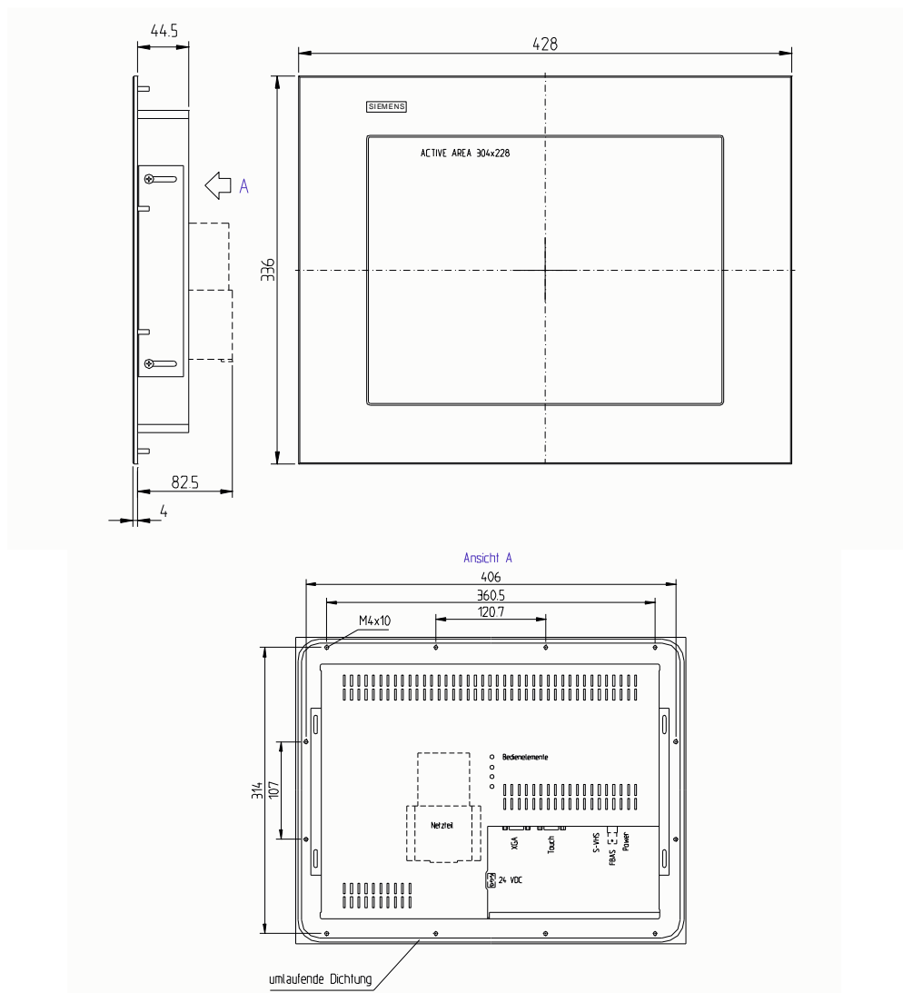
Figure1: Dimensions of the SCD 1597-Exx
