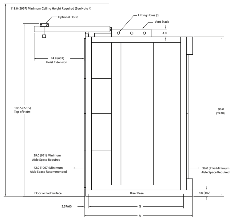
Side view
