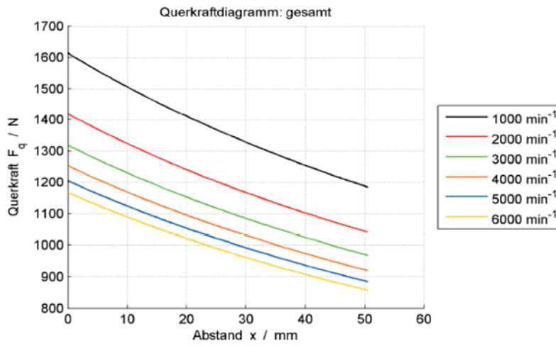
Figure 4-8 Radial force diagram 1FT7064
