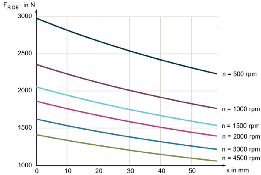
Figure 3-9 Radial force F_R at a distance x from the shaft shoulder for a statistical bearing lifetime of 25000 hours
