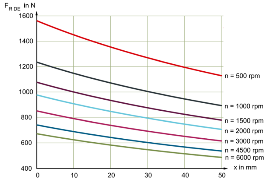
Figure 3-8 Radial force F_R at a distance x from the shaft shoulder for a statistical bearing lifetime of 25000 hours
