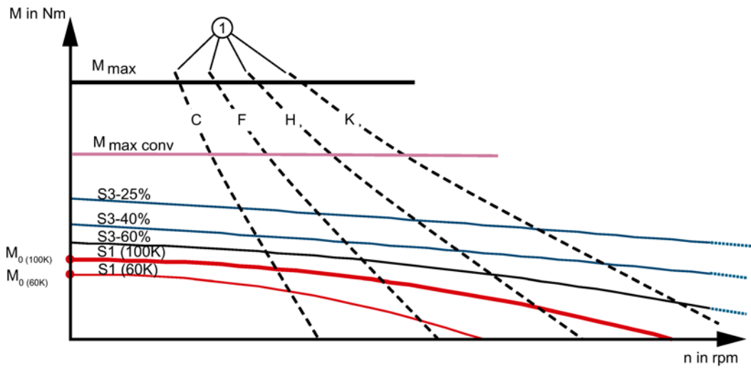
① Voltage limiting characteristic curve = torque limit without field weakening, e.g. with winding types C, F, H, K
