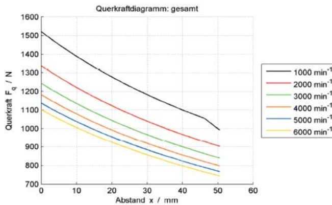
Figure 4-7 Radial force diagram 1FT7062
