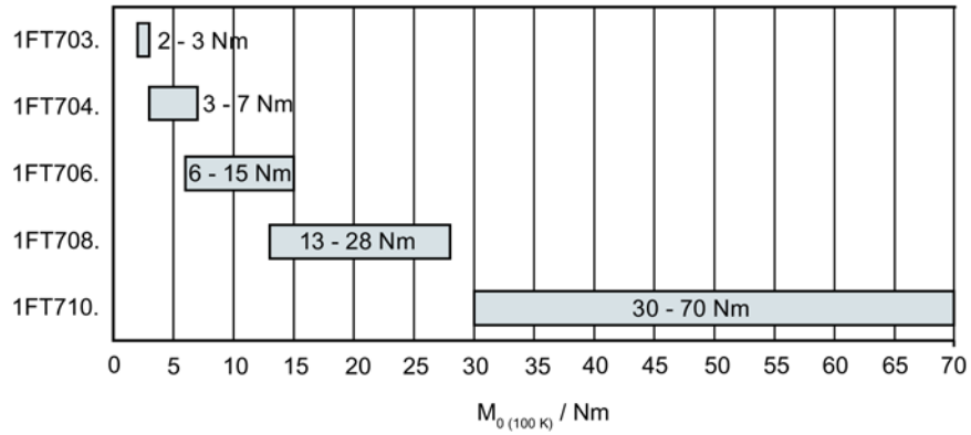
Static torques for the 1FT7 Compact, natural cooling
