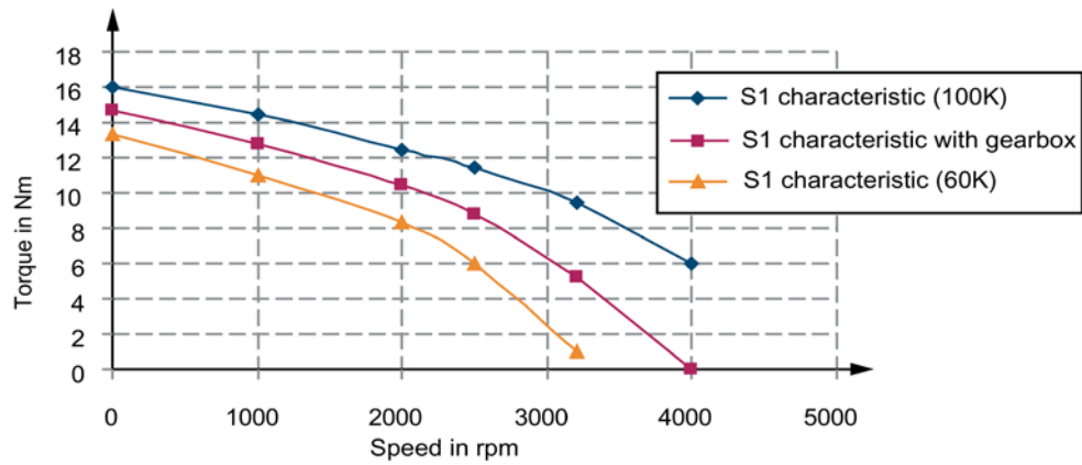
Figure 5-8 S1 characteristic (example)
