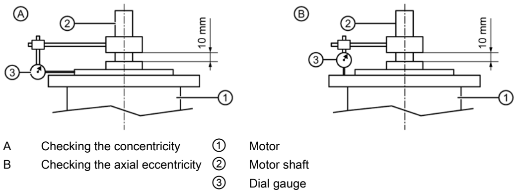
Figure 3-14 Checking the concentricity and axial eccentricity
