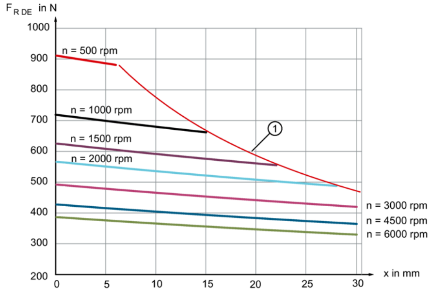
Radial force 1FT703□
