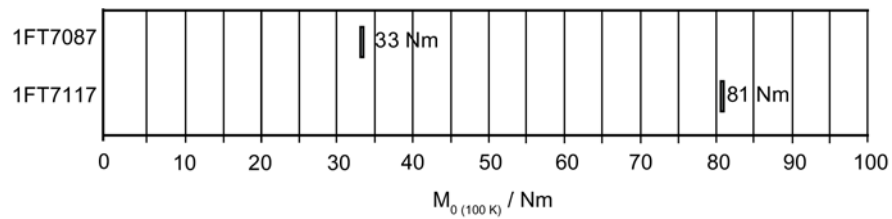
Figure 2-2 Static torque High Dyn natural cooling
