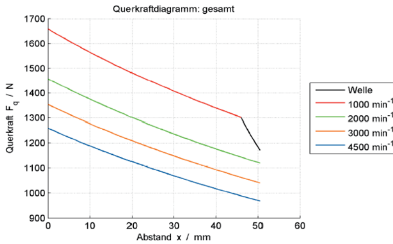
Figure 4-9 Radial force diagram 1FT7066
