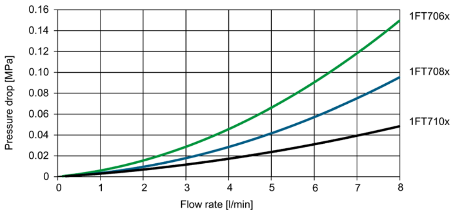
Figure 3-3 Pressure drop 1FT7
