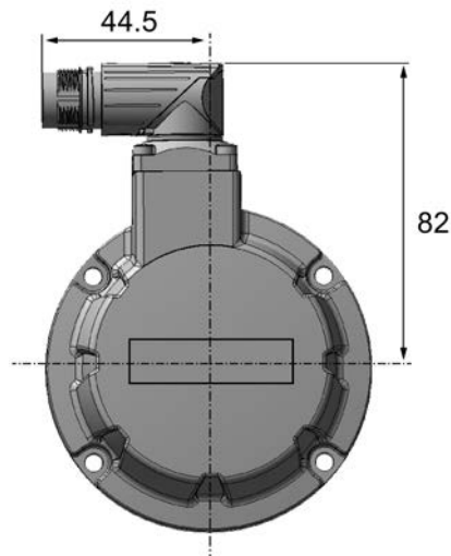
Figure 8-11 Installation dimensions encoder M17
