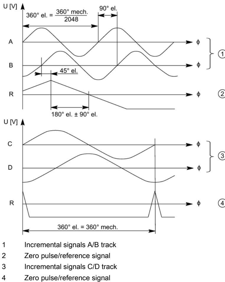
Figure 4-2 Signal sequence and assignment for encoder IC2048S/R without a DRIVE-CLiQ interface, for a positive direction of rotation
