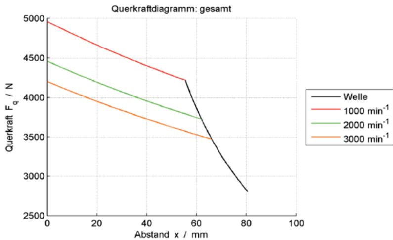
Figure 4-16 Radial force diagram 1FT7108
