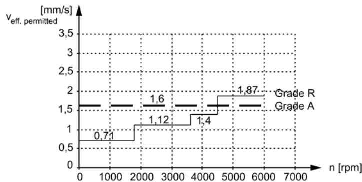
Figure 3-15 Vibration severity grades
