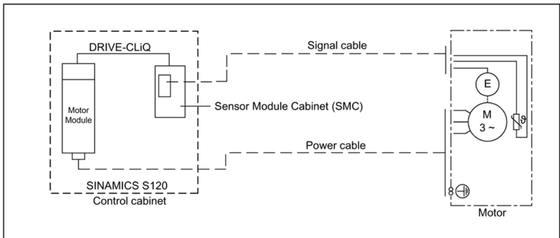
Figure 8-13 Encoder interface without DRIVE-CLiQ
