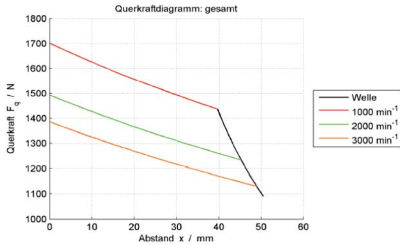
Figure 4-10 Radial force diagram 1FT7068
