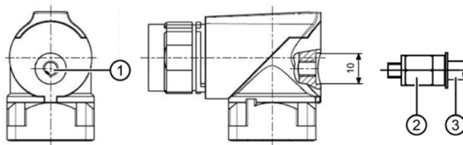
1 Sealing air connection M5
