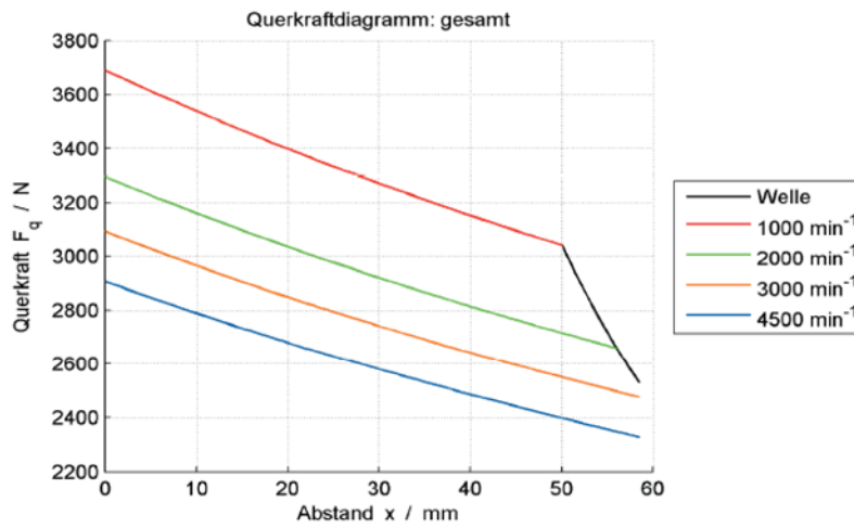
Figure 4-13 Radial force diagram 1FT7086
