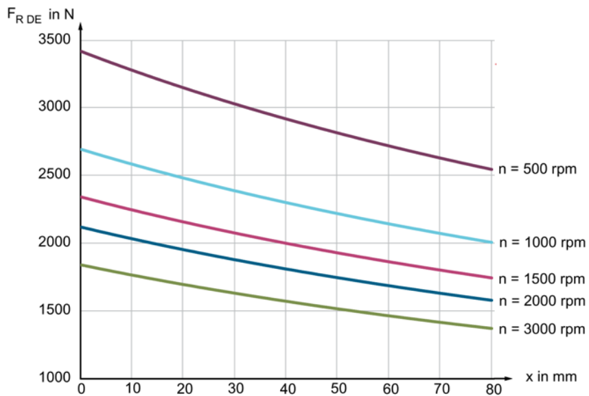
Figure 3-10 Radial force F_R at a distance x from the shaft shoulder for a statistical bearing lifetime of 25000 hours
