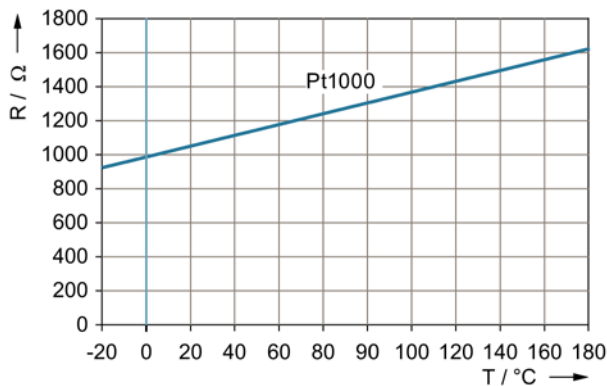
Figure 4-1 Characteristic Pt1000
