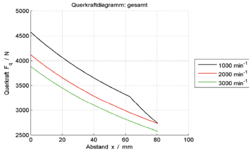
Figure 4-14 Radial force diagram 1FT7102
