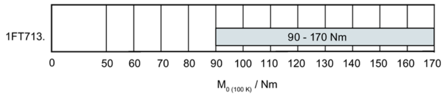
Static torques for the 1FT7 Compact, forced ventilation
