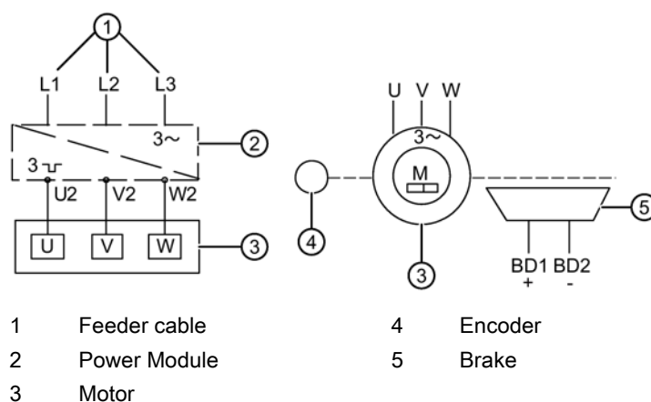
Figure 8-1 Circuit diagram
