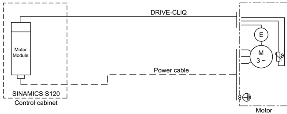
Figure 8-10 Encoder interface with DRIVE-CLiQ
