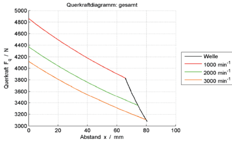
Figure 4-15 Radial force diagram 1FT7105
