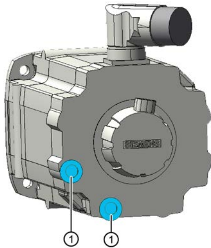
1 Ports (internal thread) for the water cooling
