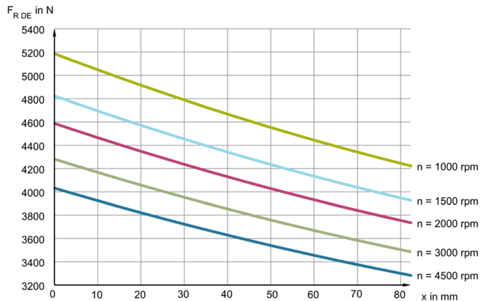
Figure 3-12 Radial force F_R at a distance x from the shaft shoulder for a statistical bearing lifetime of 25000 hours
