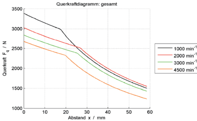
Figure 4-11 Radial force diagram 1FT7082
