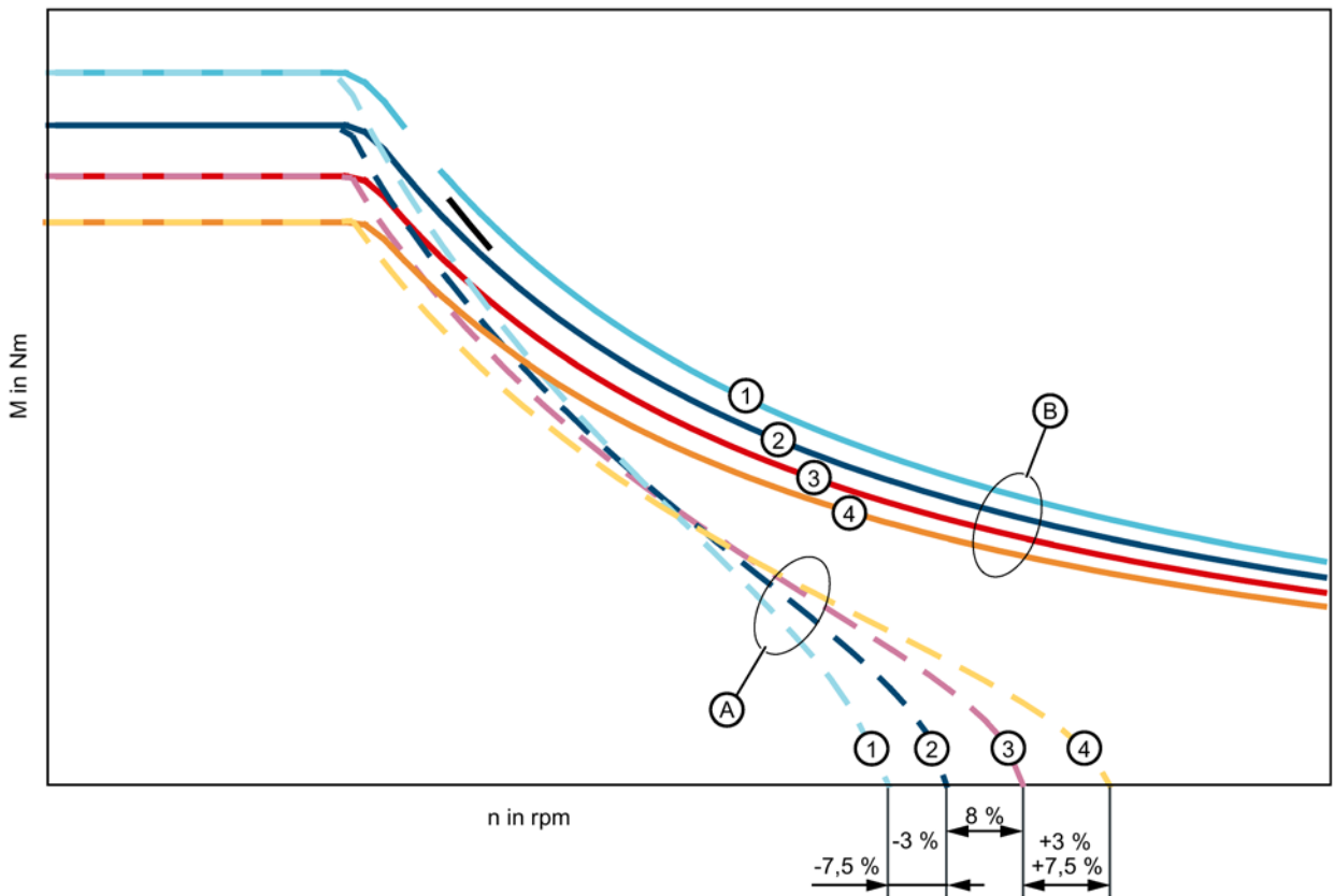
Figure 6-6 Effect of the parameter spread
