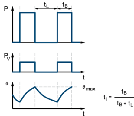
Figure 5-4 S3 duty (intermittent operation without influencing starting)
