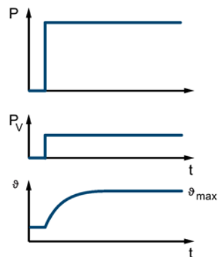
Figure 5-2 S1 duty (continuous operation)
