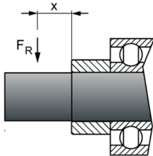
Figure 3-5 Force application point at DE
