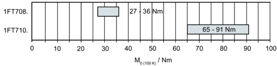
Static torques for the 1FT7 Compact, forced ventilation
