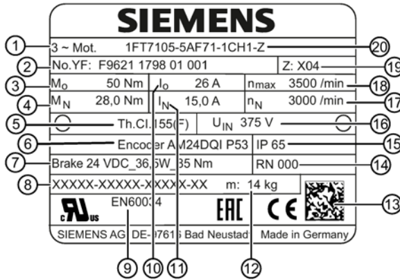
Figure 2-3 Rating plate 1FT7
