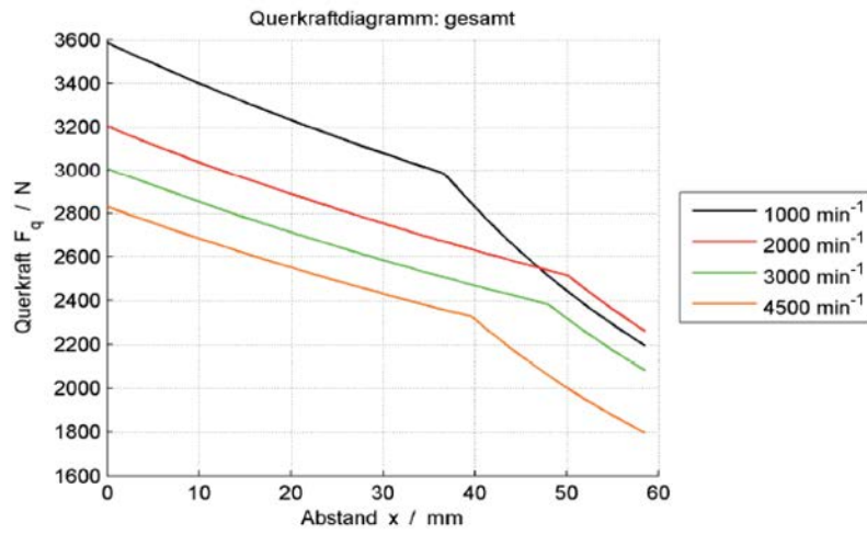
Figure 4-12 Radial force diagram 1FT7084
