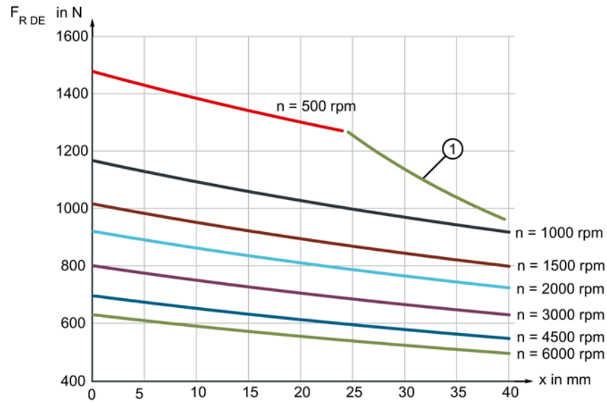
Figure 3-7 Radial force F_R at a distance x from the shaft shoulder for a statistical bearing lifetime of 25000 hours
