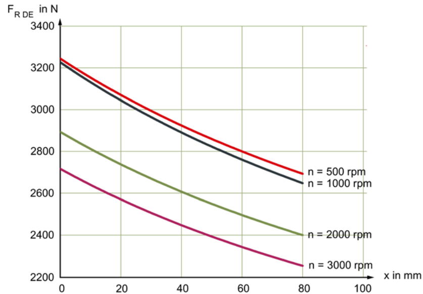
Figure 3-11 Radial force F_R at a distance x from the shaft shoulder for a statistical bearing lifetime of 25000 hours
