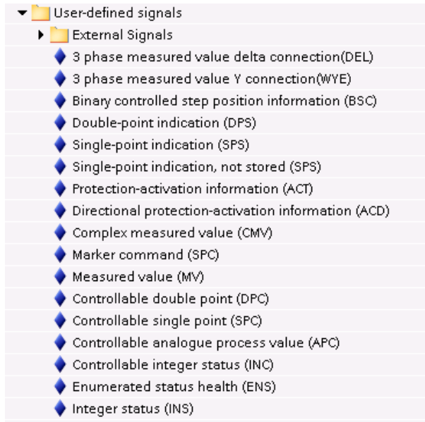
Figure 3-50 User-Defined Signals
