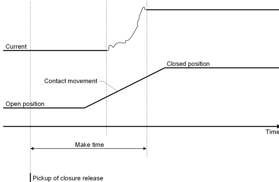
Figure 11-6 Definition of Make Time
