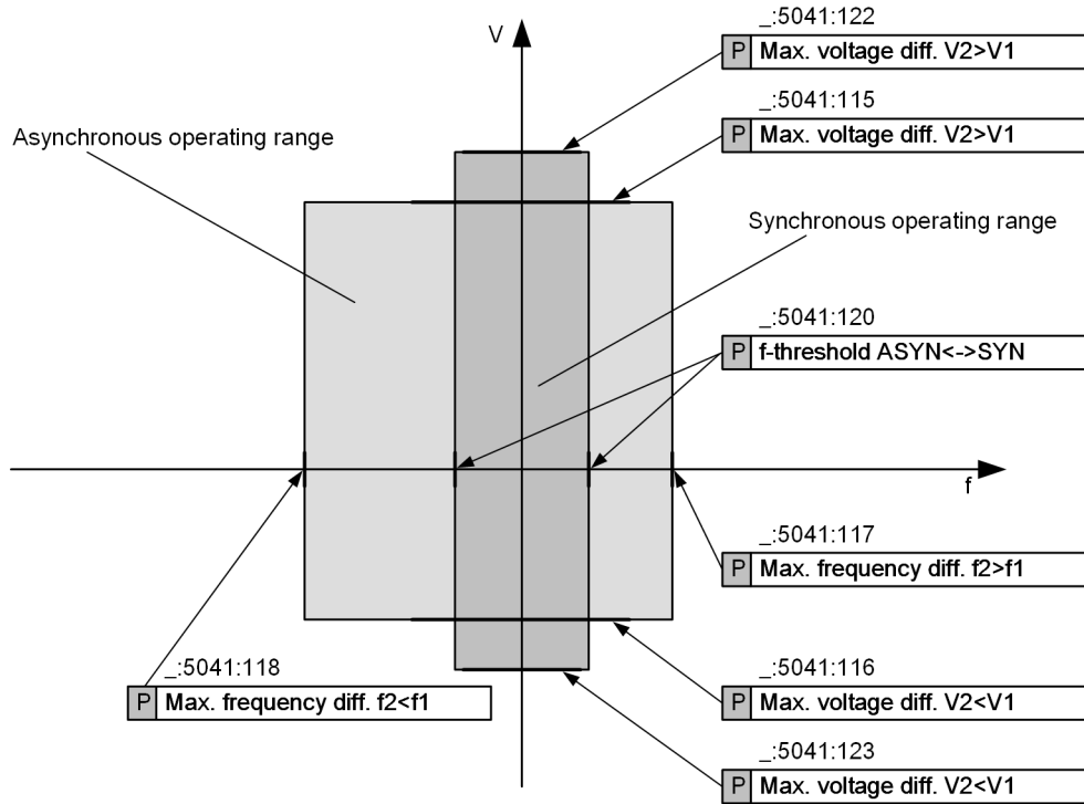
Figure 9-62 Operating Range under Synchronous and Asynchronous Conditions for Voltage (V) and Frequency (f)
