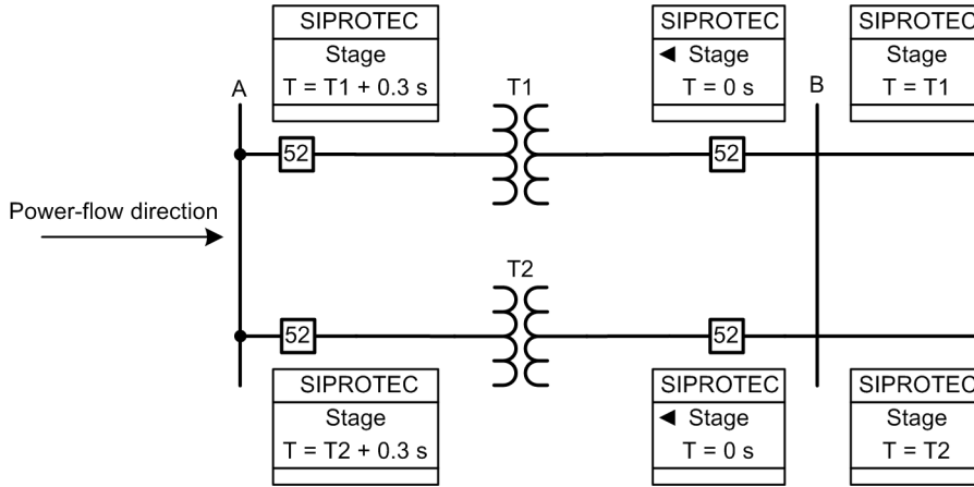
Figure 6-49 Parallel Line with Transformers
