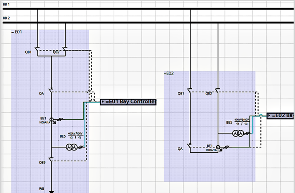
Figure 9-37 System with Feeder and Coupler Bays
