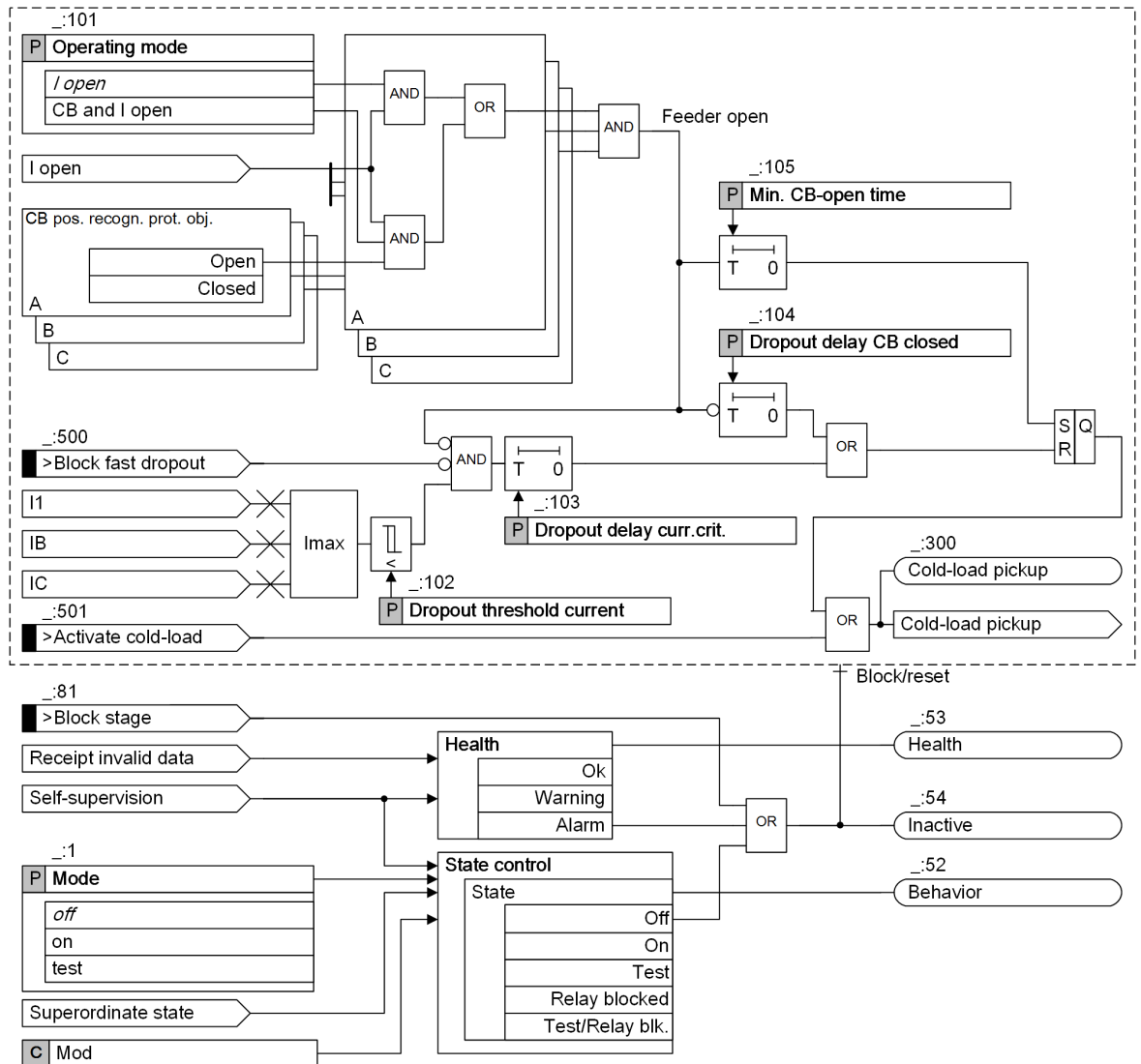
Figure 5-142 Logic Diagram of the Cold-Load Pickup Detection Function Block
