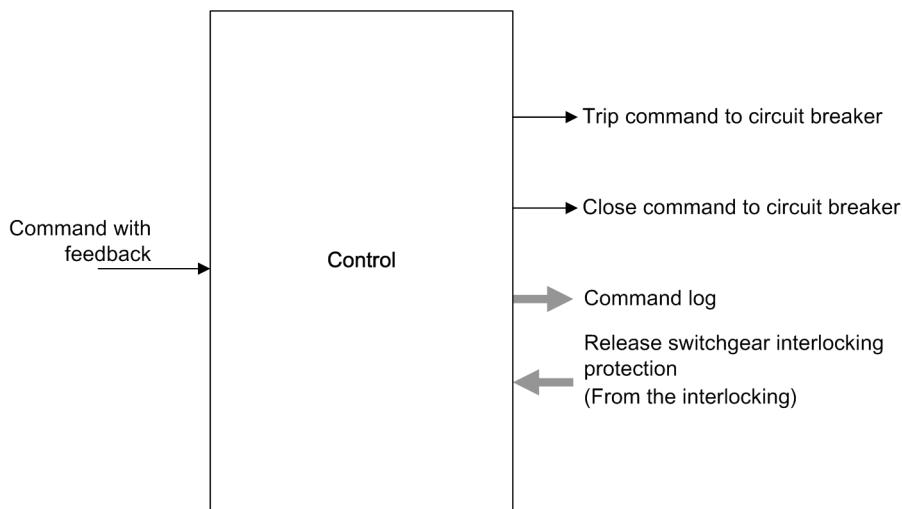
Figure 9-6 Logical Inputs and Outputs of the Control Function Block
