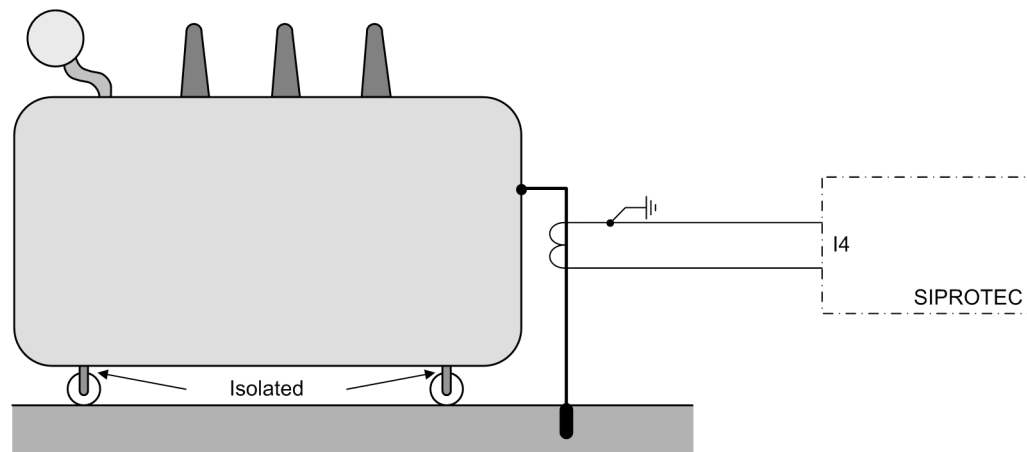
Figure 6-98 Tank-Control Principle
