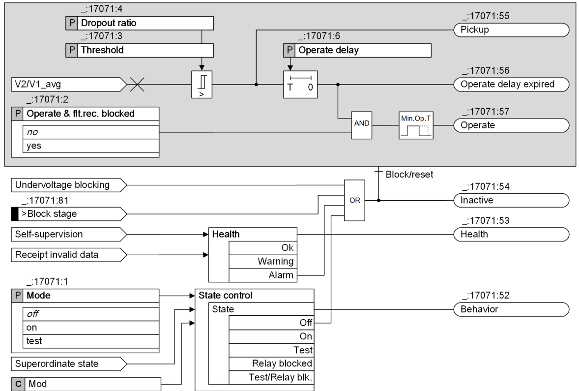
Figure 6-194 Logic Diagram of the Stage: Overvoltage Protection with Negative-Sequence Voltage/Positive-Sequence Voltage
