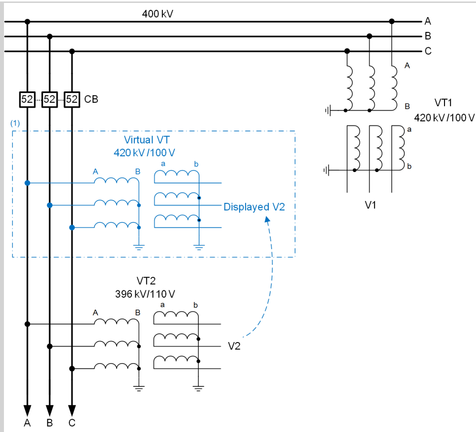
Figure 9-54 Example: the Electrical Power System without a Power Transformer
