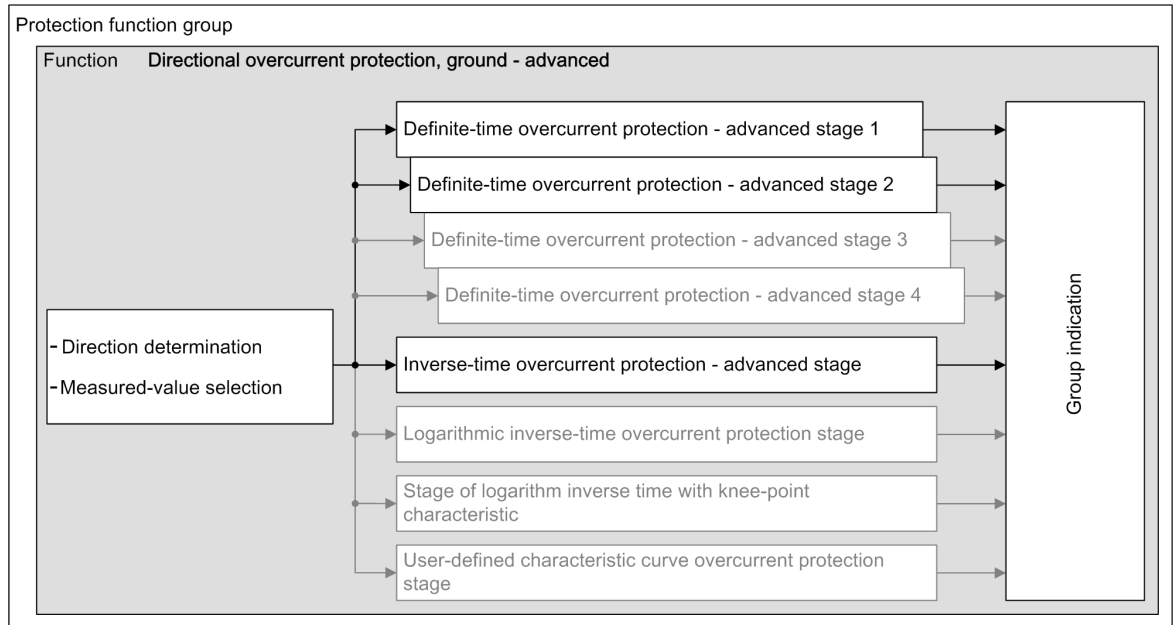
Figure 6-51 Structure/Embedding of the Function Directional Overcurrent Protection, Ground – Advanced
