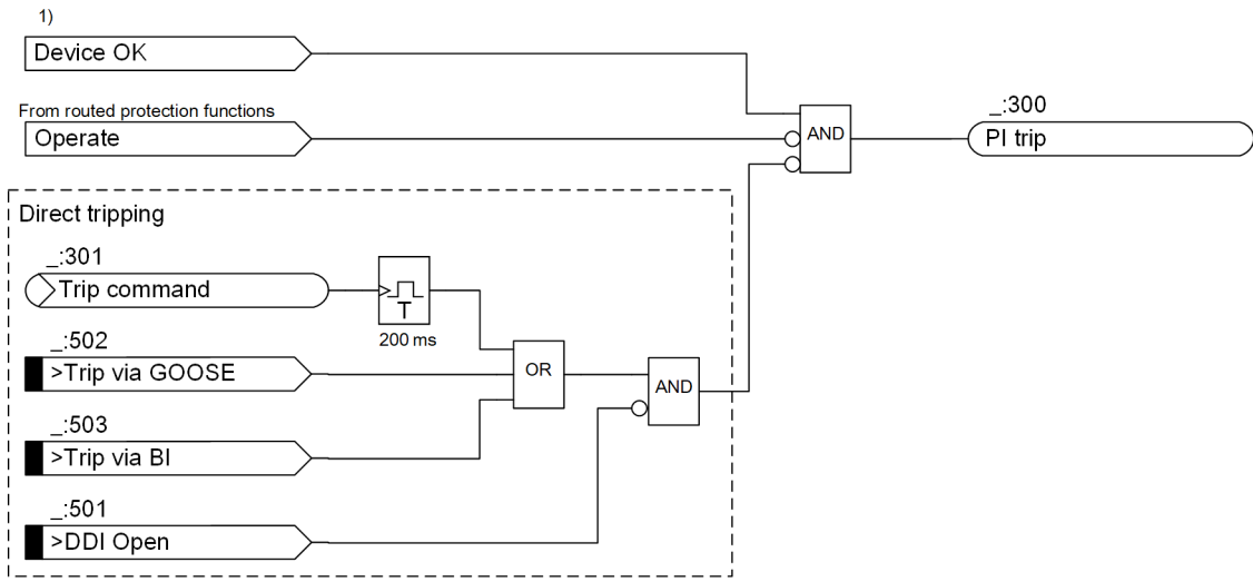
Figure 6-370 Logic Diagram of the PI Trip
