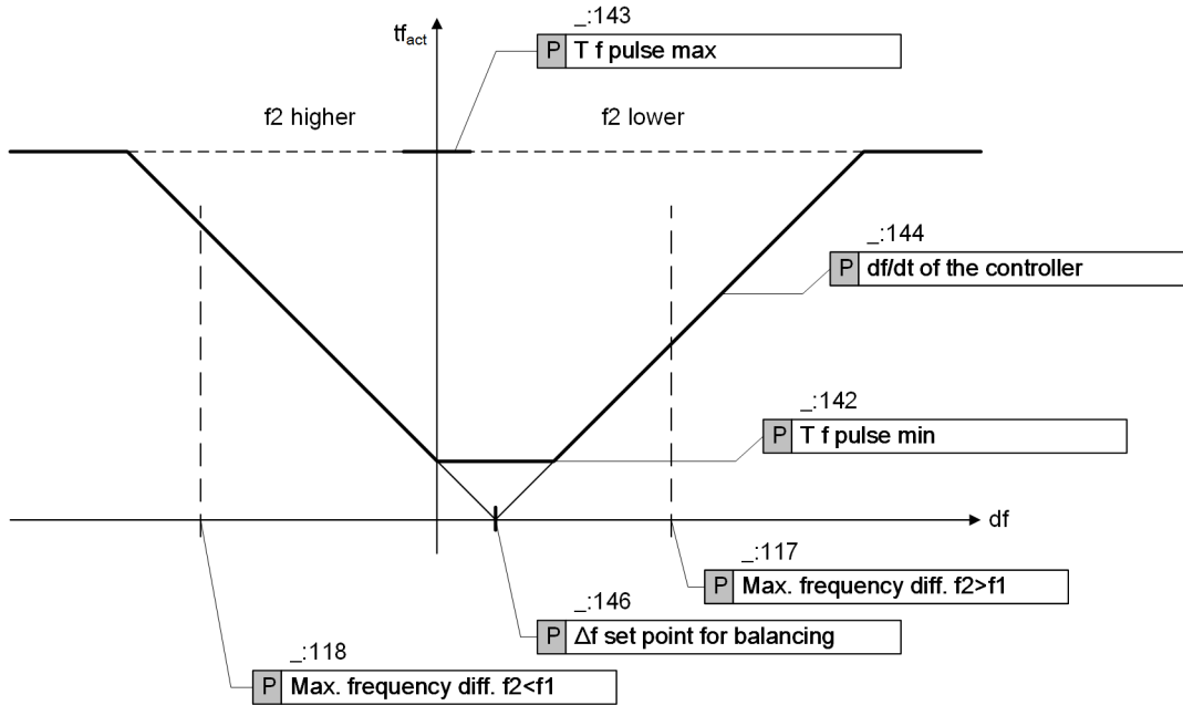
[dw_build_frequency-adjusting-com, 2, en_US] Figure 9-68 Generation of Balancing Commands for Frequency
