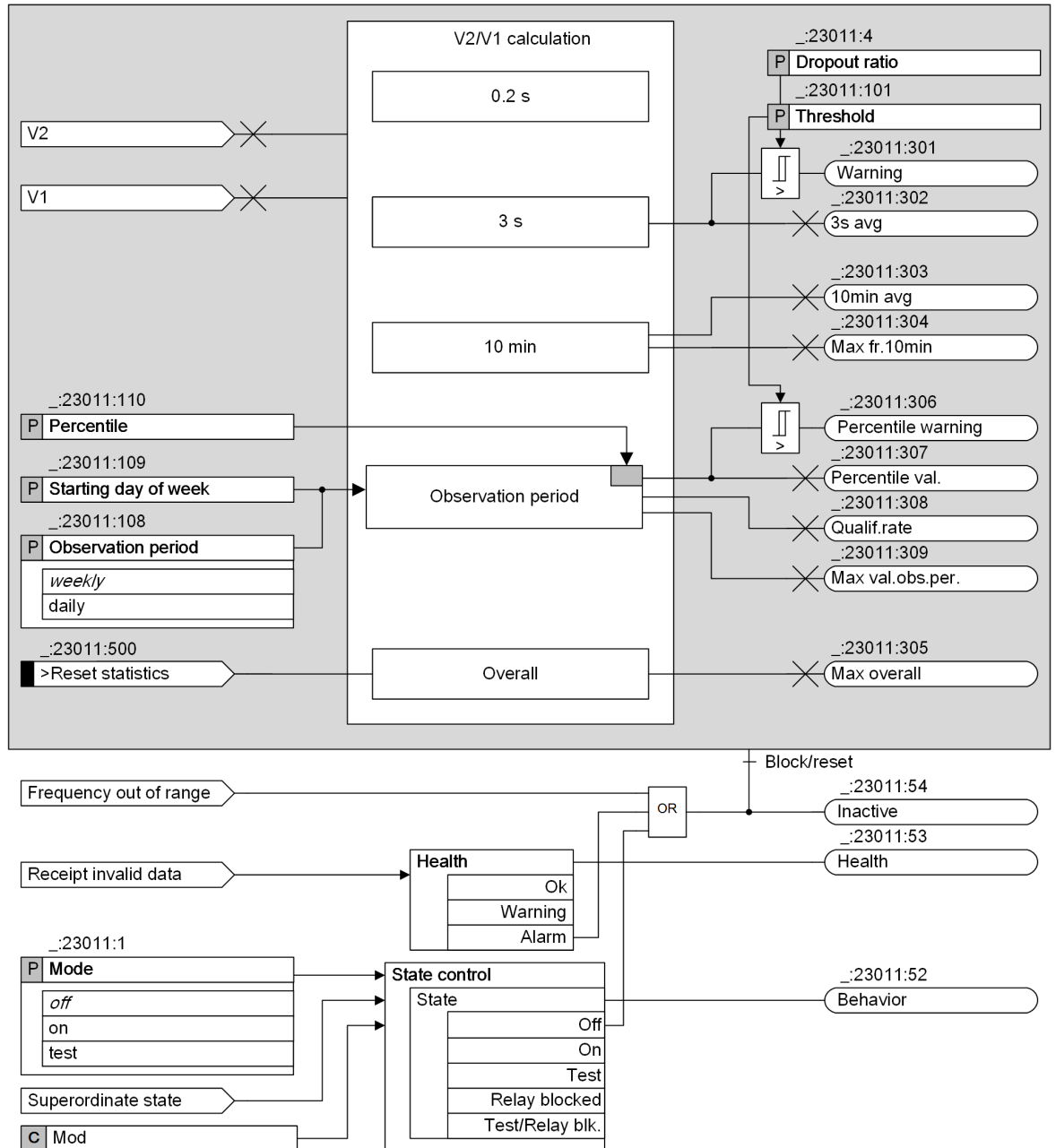
Figure 12-11 Logic Diagram of the Stage V2/V1
