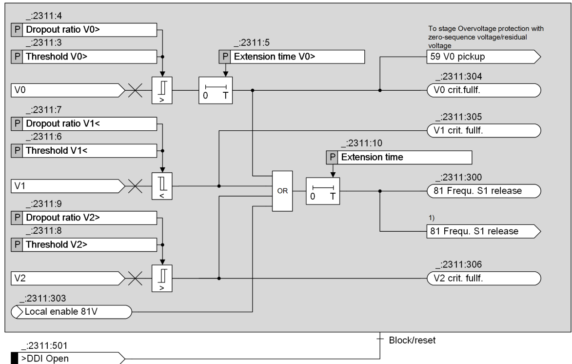
Figure 6-357 Logic Diagram of the Voltmetric Unblocking
