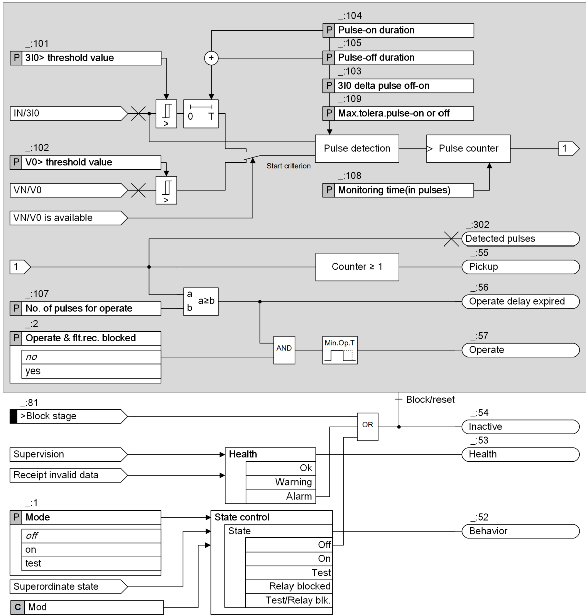
Figure 6-144 Logic Diagram of the Pulse-Pattern Detection Stage
