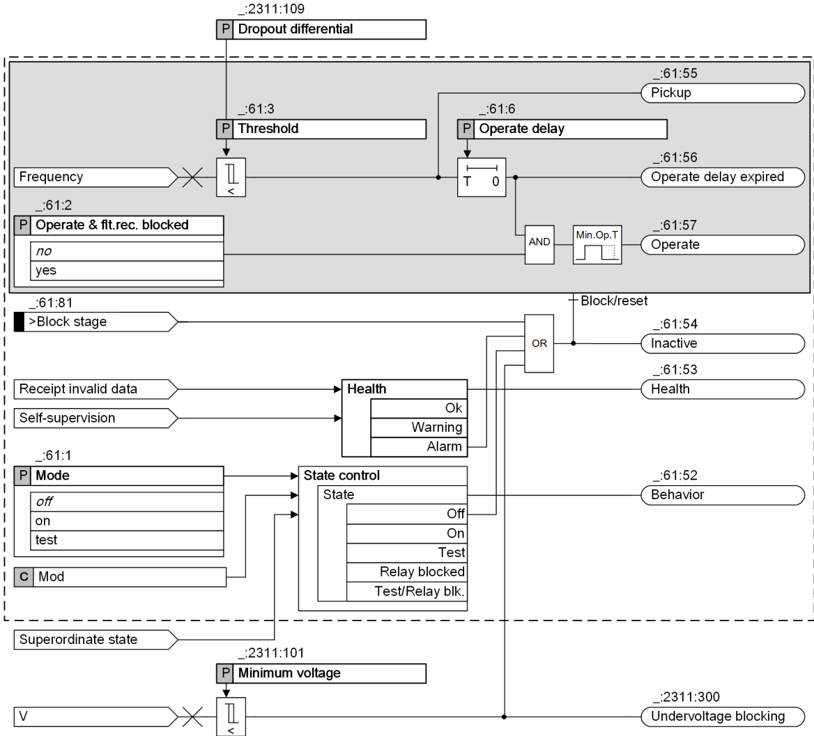
Figure 6-213 Logic Diagram of the Underfrequency-Protection Stage
