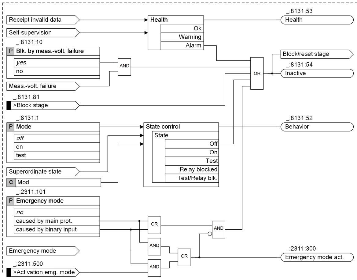
Figure 6-39 Stage-Control Logic Diagram
