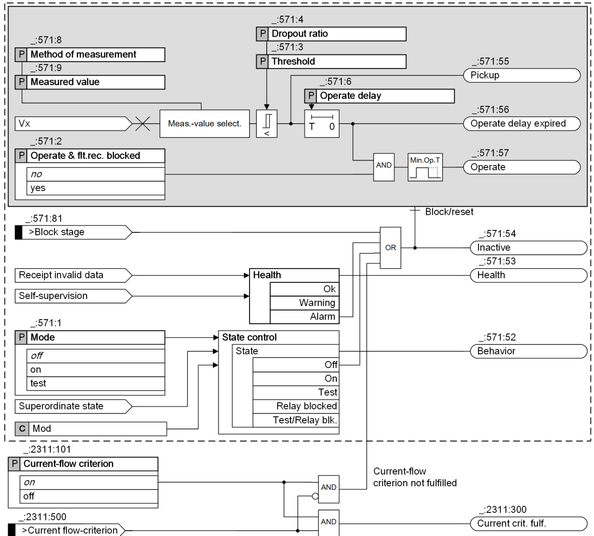
Figure 6-206 Logic Diagram of a Stage: Undervoltage Protection with Any Voltage
