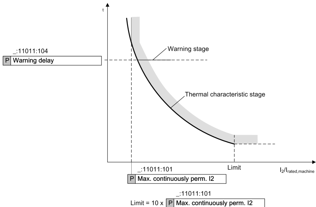
Figure 6-175 Operate Curve of the Unbalanced-Load Protection
