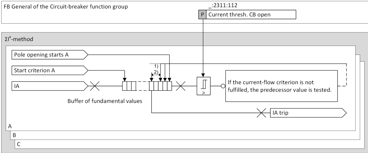
Figure 11-9 Logic of the Determination of the Tripping Current Value
