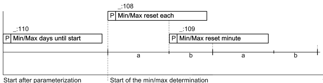
Figure 11-3 Minimum and Maximum-Value Formation
