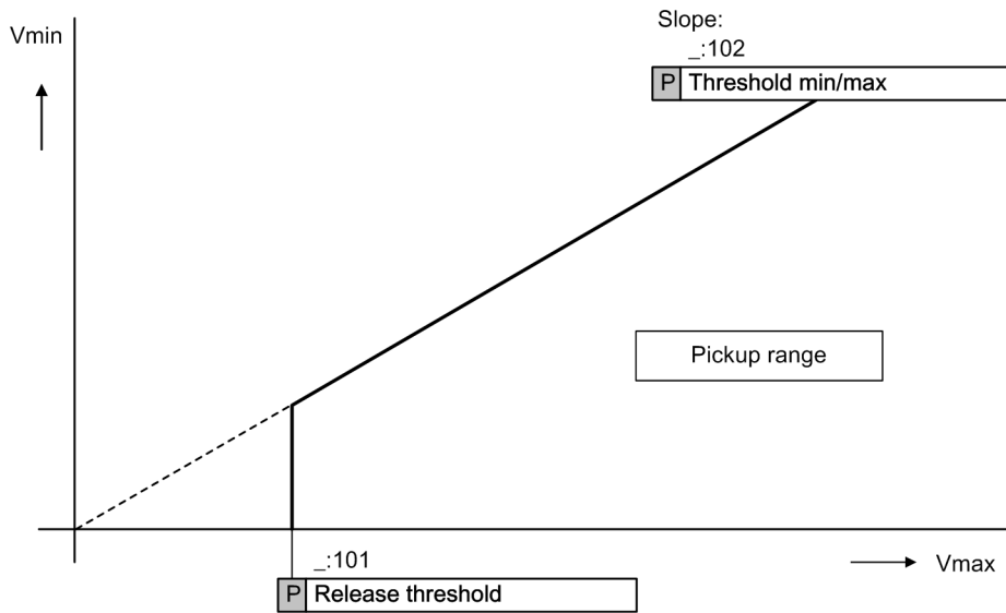
Figure 10-16 Characteristic of the Voltage-Balance Supervision
