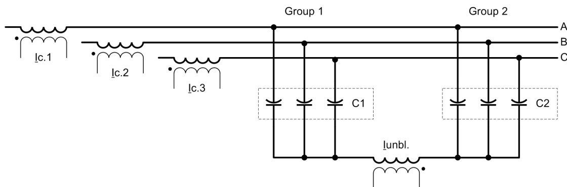
Figure 8-9 Definition for the Fault-Location Information
