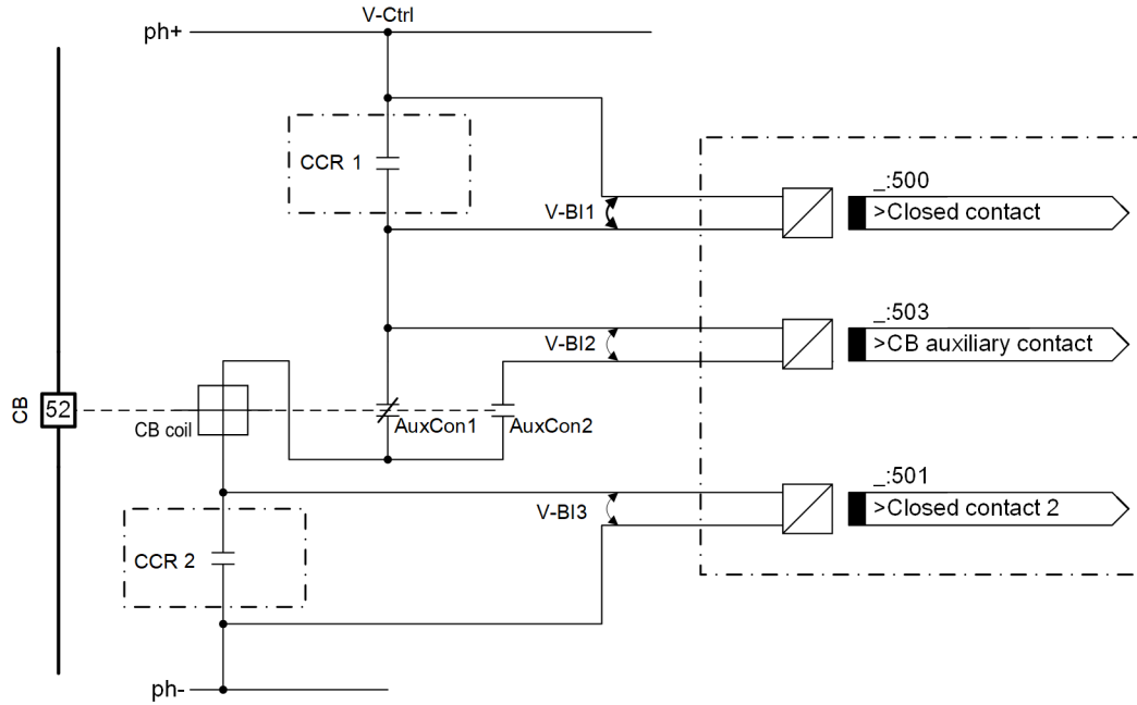
Figure 10-42 Principle of the Closing-Circuit Supervision with 3 Binary Inputs
