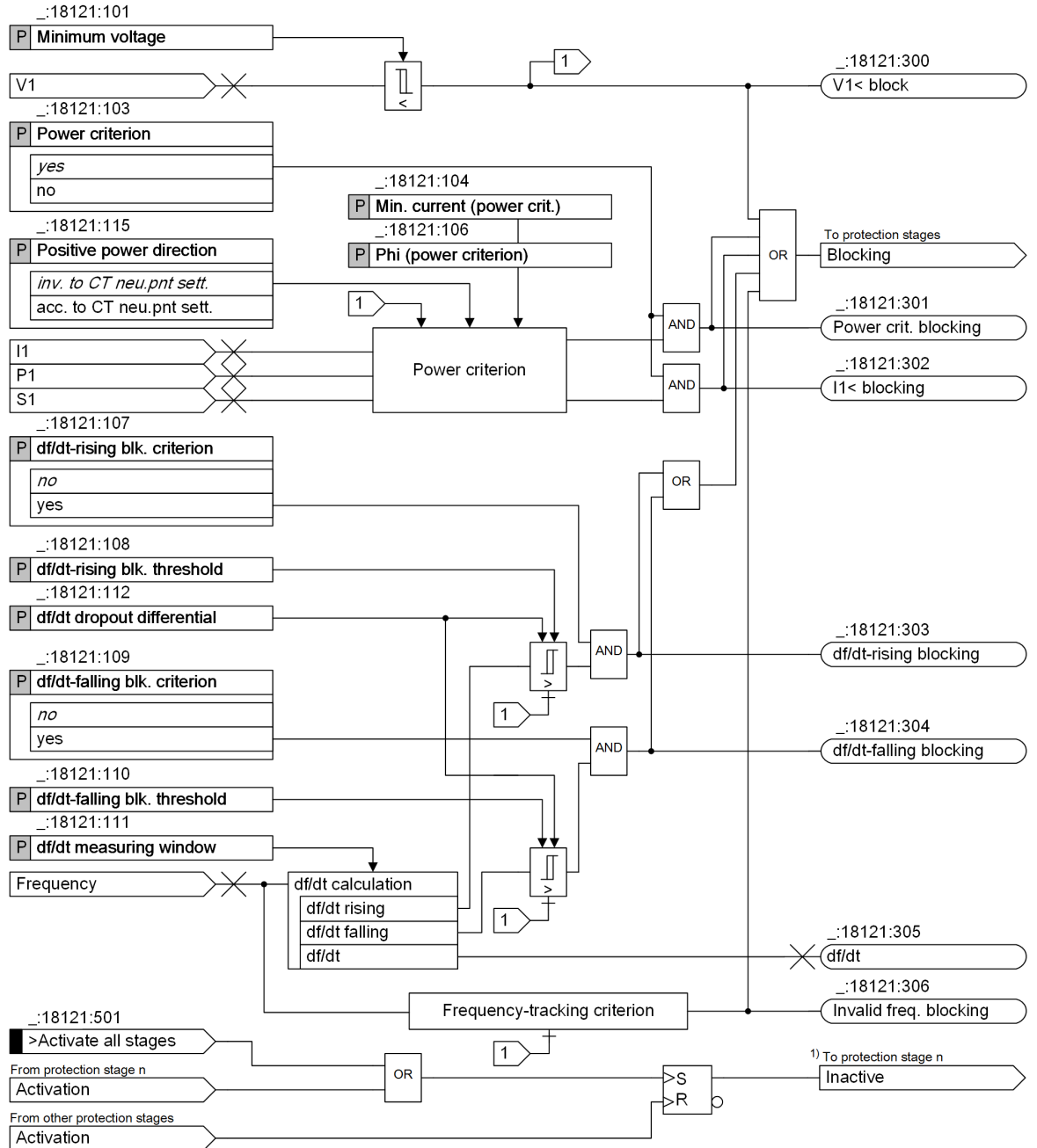
Figure 6-215 Logic Diagram of the General Functionality
