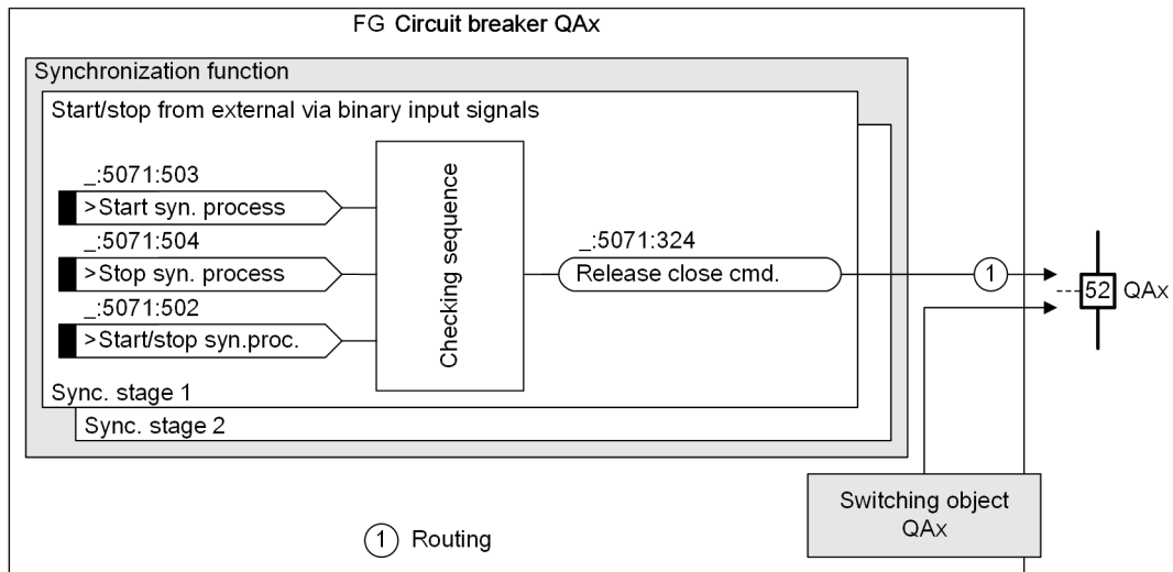
Figure 9-80 Interaction of the Synchronization Function with External Control
