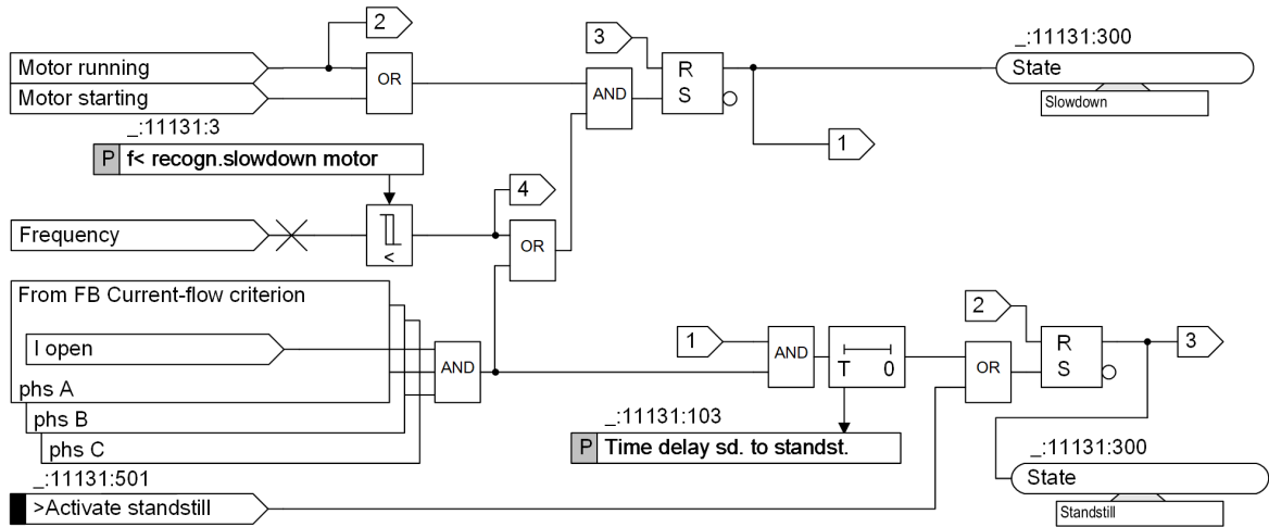
Figure 5-24 Logic Diagram of the Motor-State Detection, Part 1
