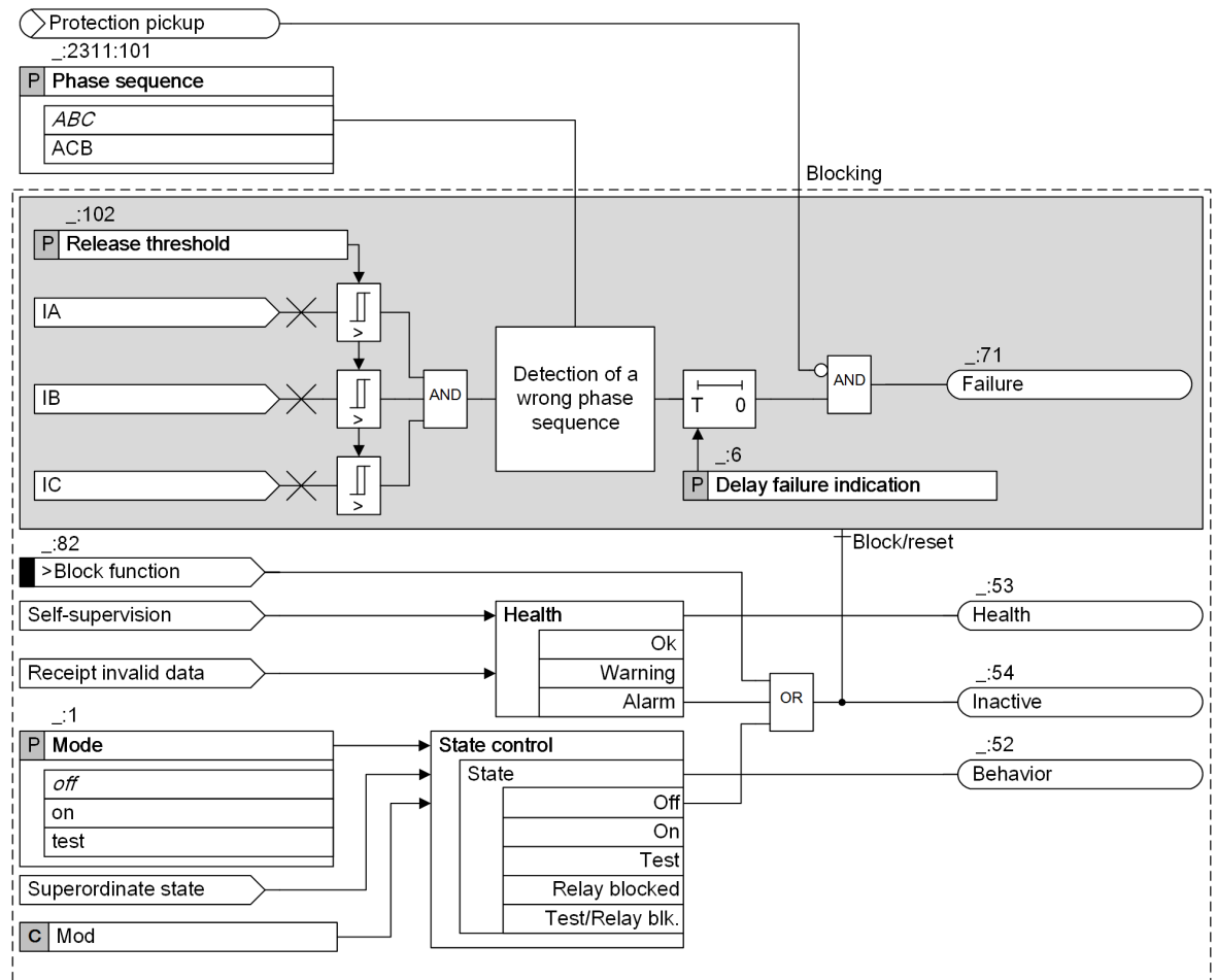
Figure 10-35 Logic Diagram of the Current Phase-Rotation Supervision
