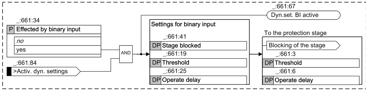
Figure 6-21 Influence of the Binary Input on the Overcurrent-Protection Stage
