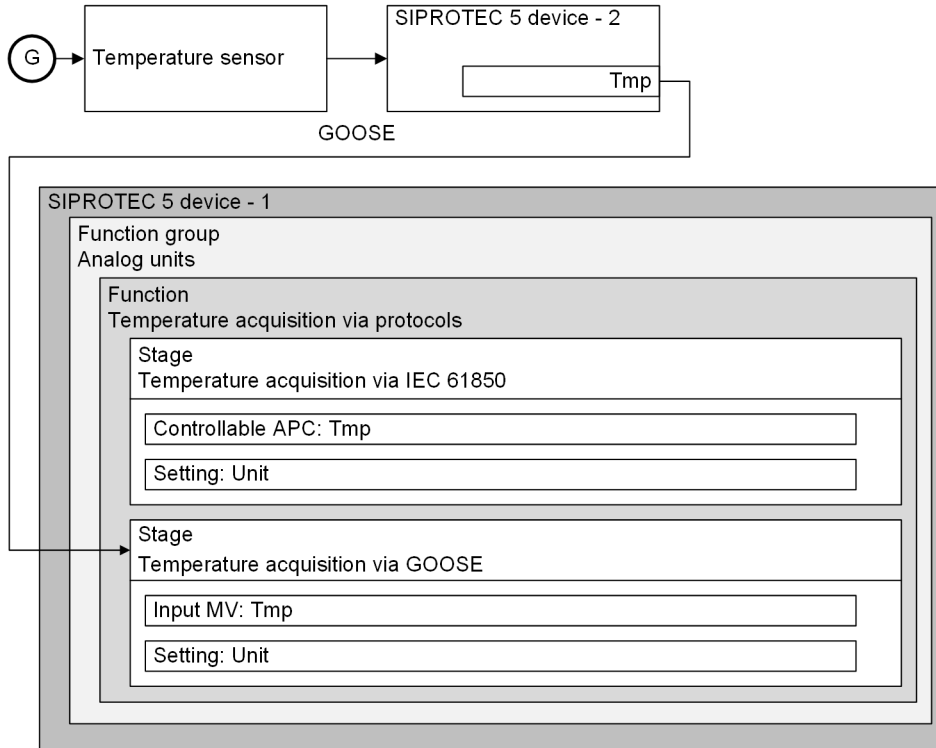
Figure 5-83 Application Example
