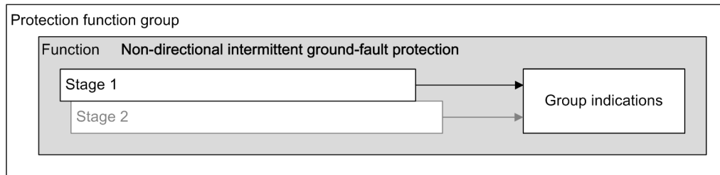
Figure 6-103 Structure/Embedding of the Function
