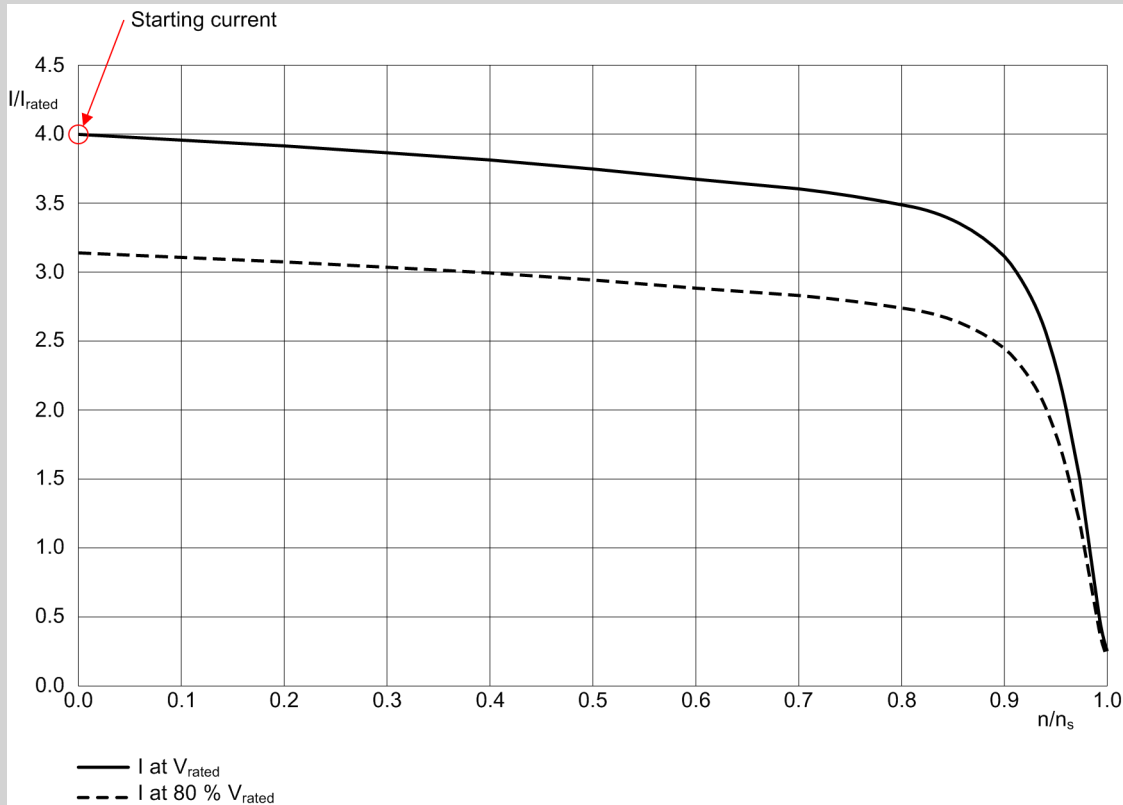
Figure 5-31 Starting-Data Diagram
