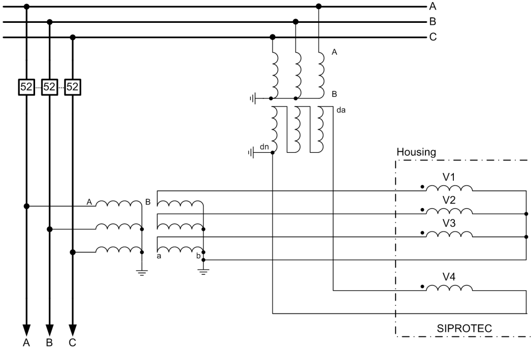
Voltage transformer 3-phase: connection = 3 phase-to-ground volt. + VN
