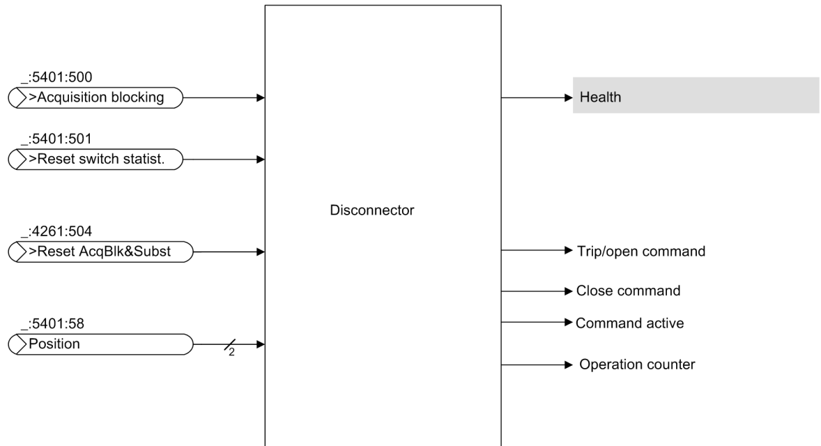
Figure 9-9 Logical Inputs and Outputs of the Disconnecter Function Block
