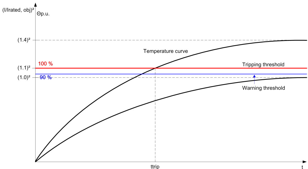
Figure 6-163 Temperature History for Different Overload Currents ( K-factor = 1.1)
