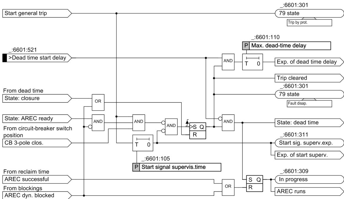
[do_gistar_1_en_US] Figure 6-299 Logic for Function Block Start
