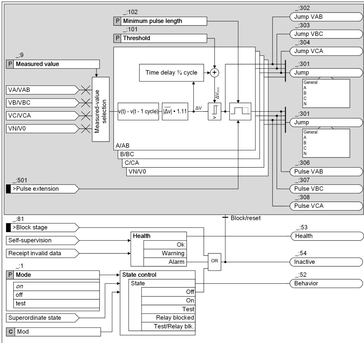
Figure 6-348 Voltage-Jump Detection Logic
