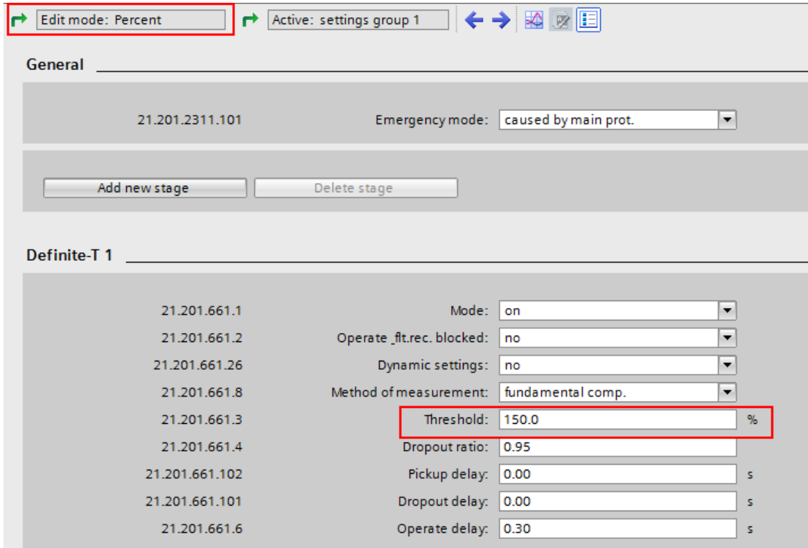
Figure 3-72 Example of the Threshold Value of the Definite-Time Overcurrent Protection Stage (Edit Mode: Percent)
