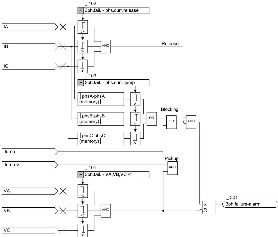
Figure 10-7 Logic Diagram 3-Phase Measuring-Voltage Failure
