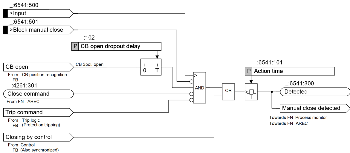
Figure 5-119 Logic for Manual Closure Detection
