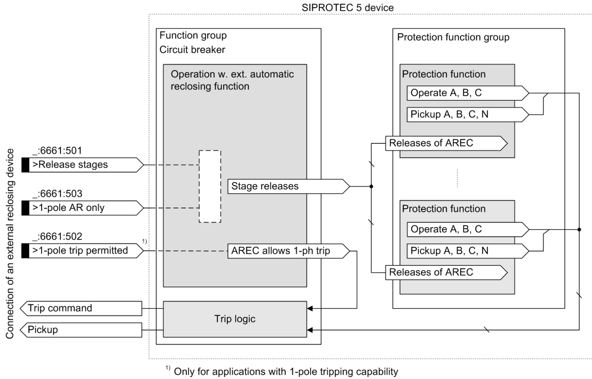
Figure 6-319 Connection of an External Automatic Reclosing Function
