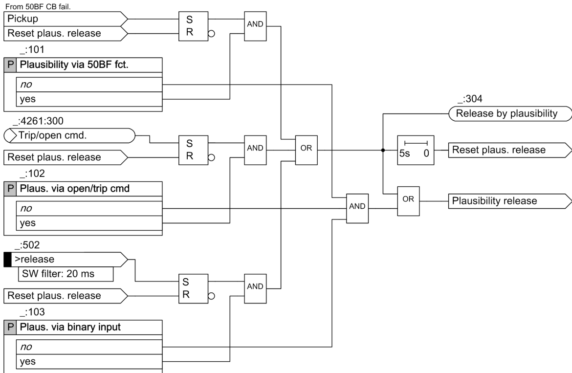
Figure 6-259 Logic Diagram for the Plausibility Release of the Circuit-Breaker Restrike Protection
