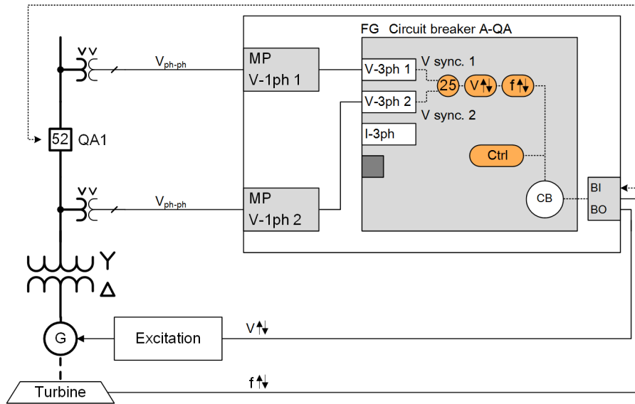
Figure 9-72 Connection of Two 1-Phase Voltage Transformers (Phase-to-Phase Voltage)
