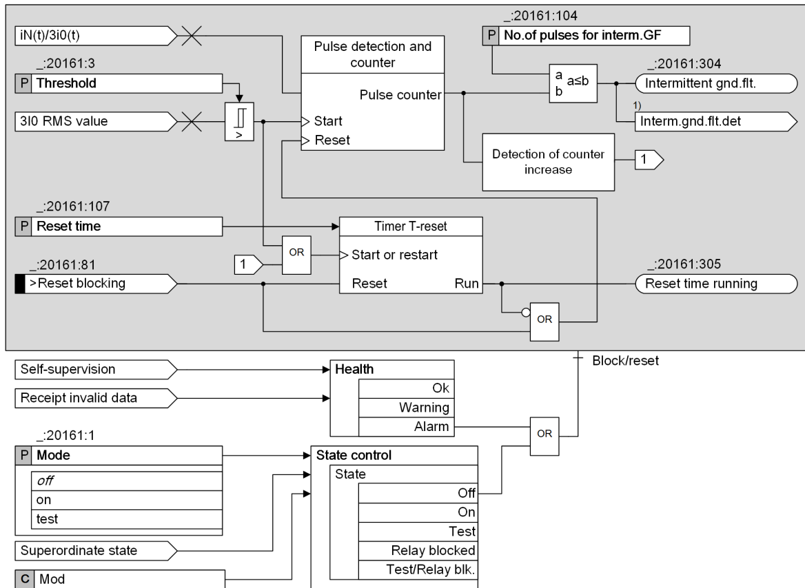
Figure 6-146 Logic Diagram of the Intermittent Ground-Fault Blocking Stage
