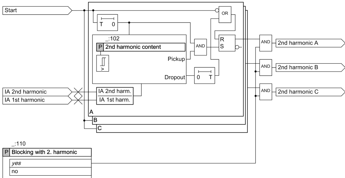
[file_inrush_10_1_en_US] Figure 6-72 Logic of the Harmonic Analysis Function (T = 1 Period)
