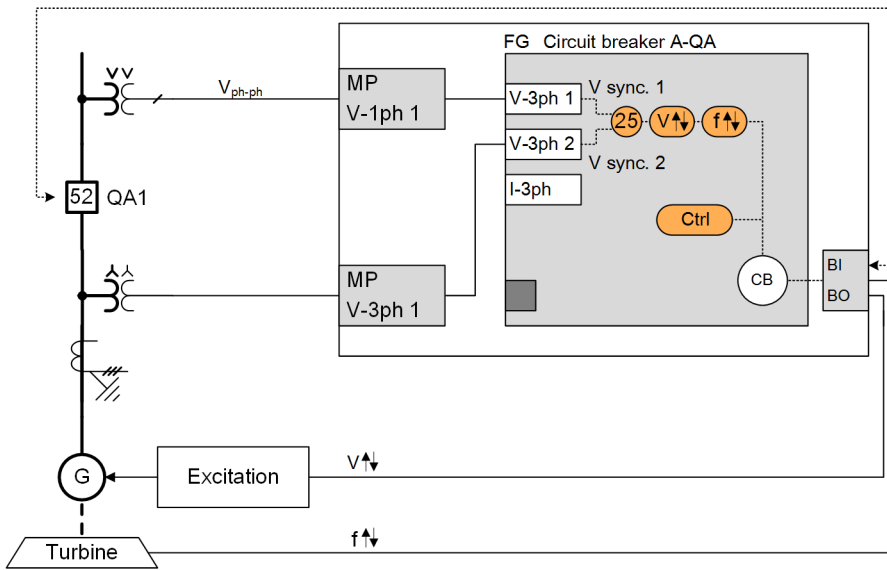
Figure 9-71 Connection of a 3-Phase and a 1-Phase Voltage Transformer (Phase-to-Phase Voltage)
