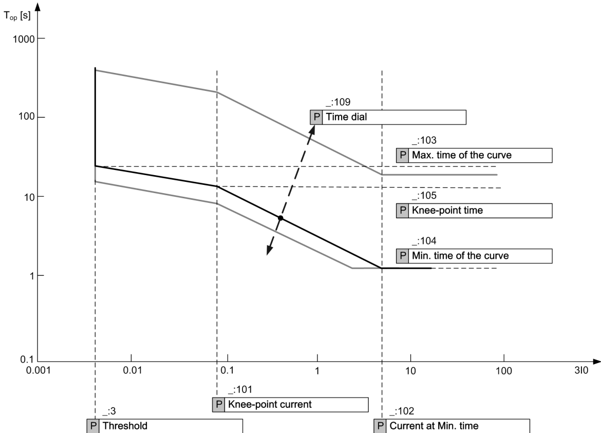
Figure 6-67 Operate Curve of the Logarithmic Inverse Time with Knee-Point Characteristic (In the Example of Threshold = 0.004 A )
