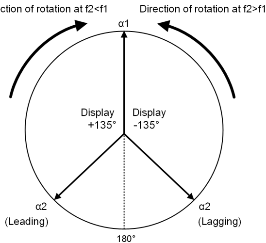
Figure 9-51 Phase-Angle Difference Representation d\alpha
