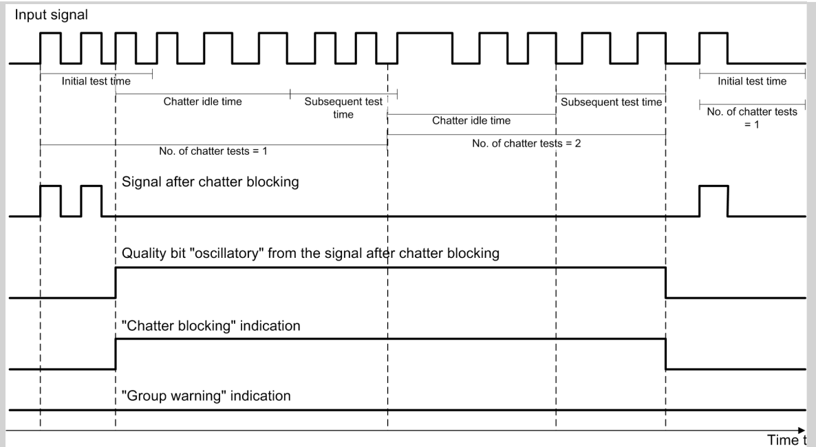
Figure 3-56 Signal Change during Chatter Blocking with Permissible Number of Signal State Changes During 2nd Subsequent Test Time
