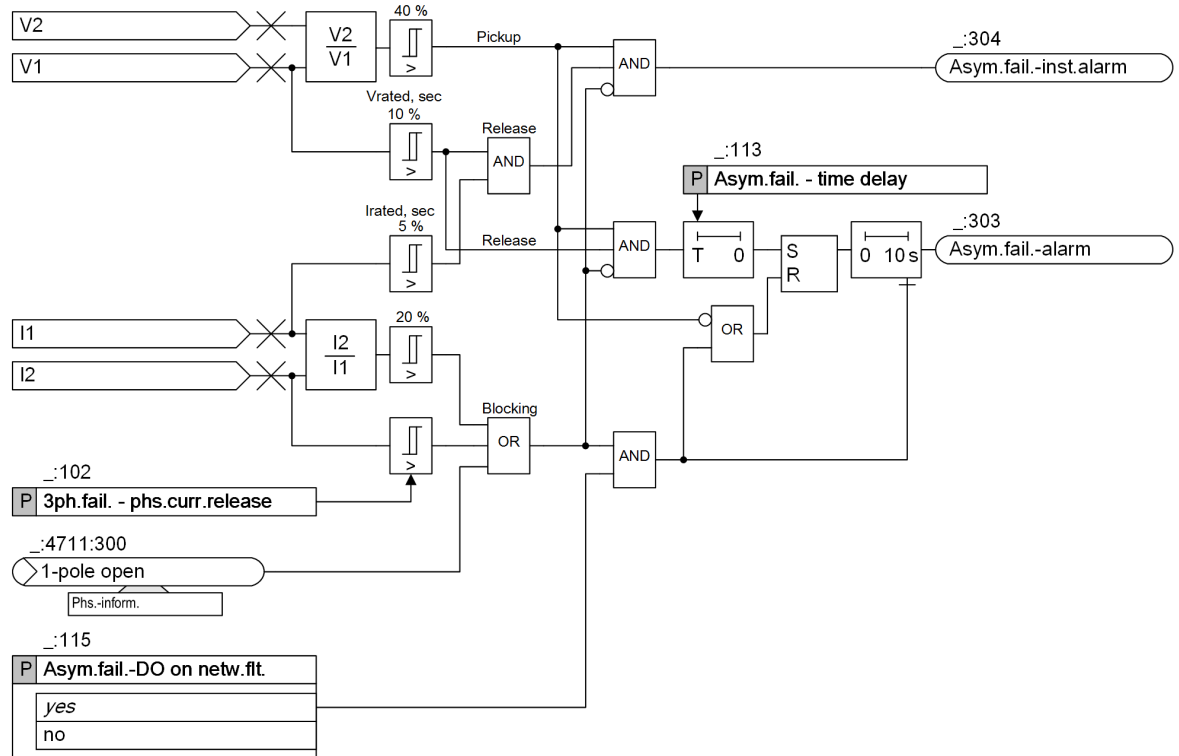
Figure 10-6 Logic Diagram Unbalanced Measuring-Voltage Failure Detection
