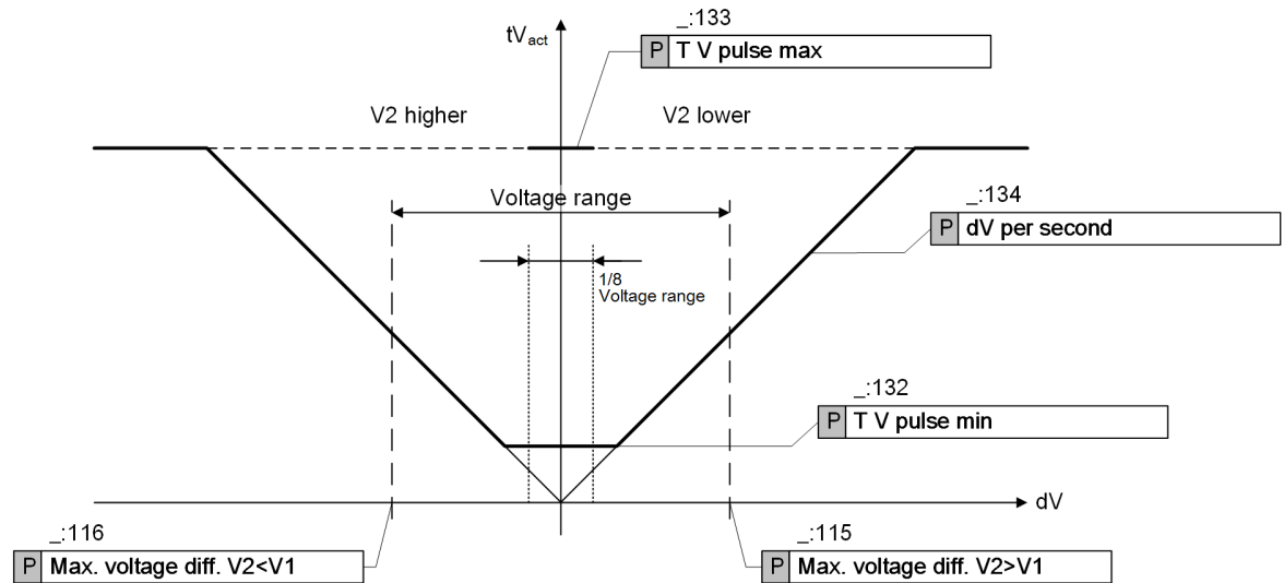
Figure 9-67 Generation of Balancing Commands for Voltage
