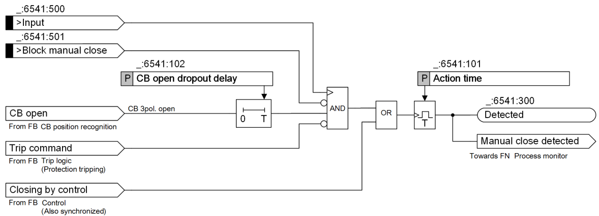
Figure 5-135 Logic for Manual Closure Detection
