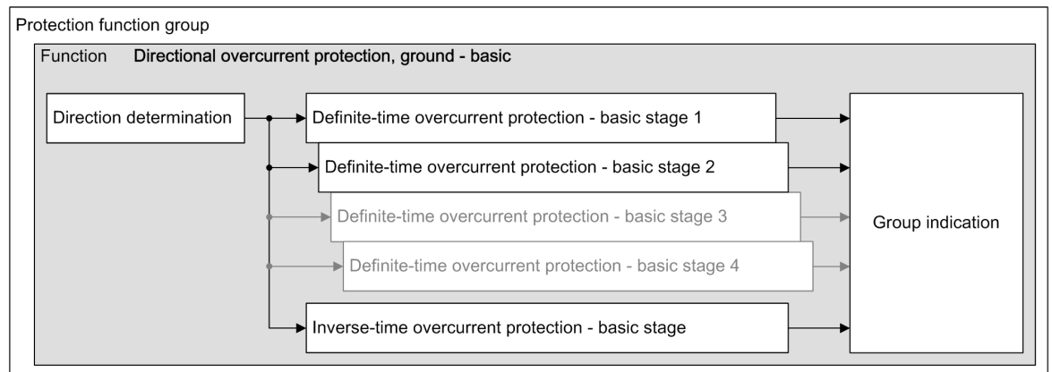
Figure 6-52 Structure/Embedding of the Function Directional Overcurrent Protection, Ground – Basic
