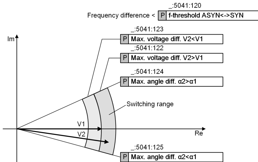
Figure 9-60 Connecting Under Synchronous System Conditions
