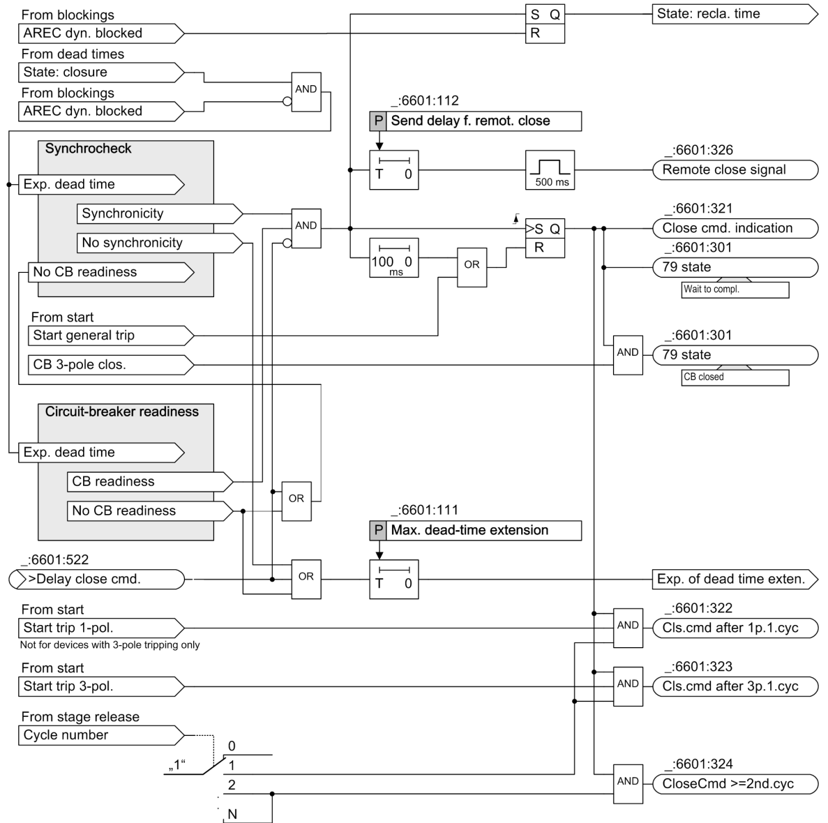
Figure 6-310 Cyclic Automatic Reclosing: Logic for the Closing Indication
