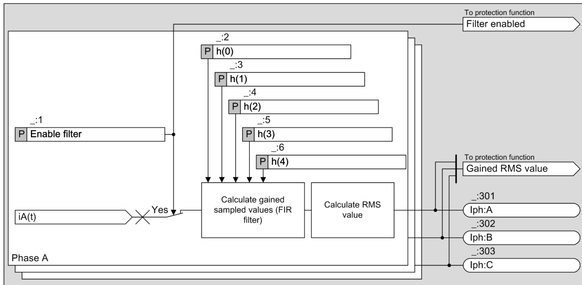
Figure 6-8 Logic Diagram of the Function Block Filter
