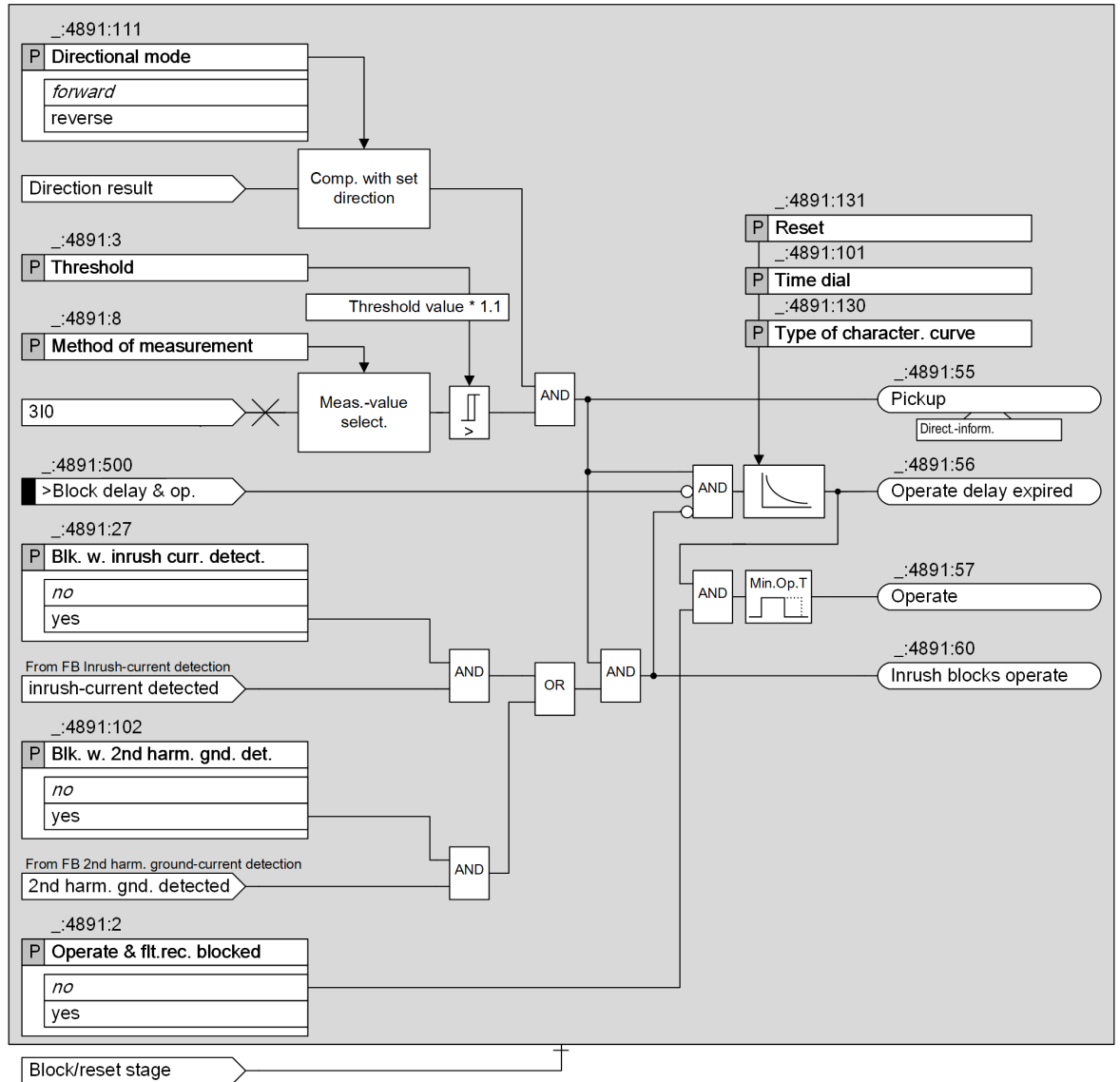
Figure 6-61 Logic Diagram of the Directional Inverse-Time Overcurrent Protection, Ground – Basic
