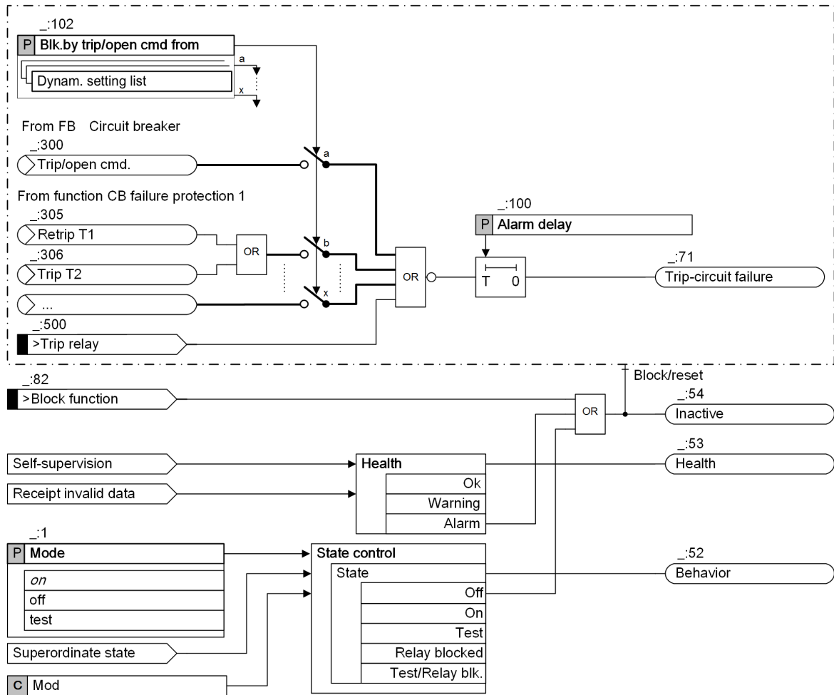
Figure 10-40 Logic Diagram of Trip-Circuit Supervision with 1 Binary Input
