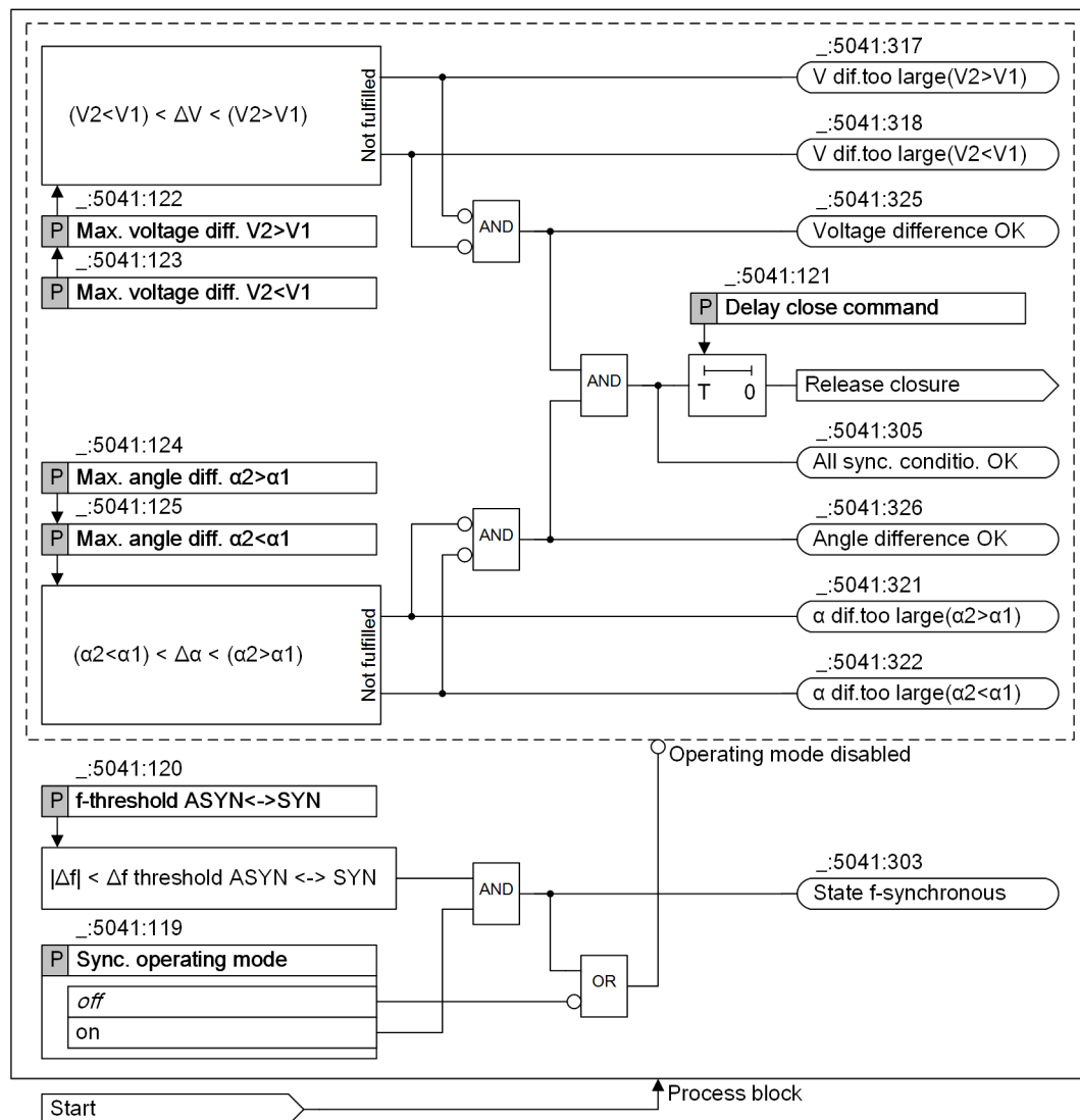
Figure 9-59 Closing Conditions when Switching Synchronous Systems
