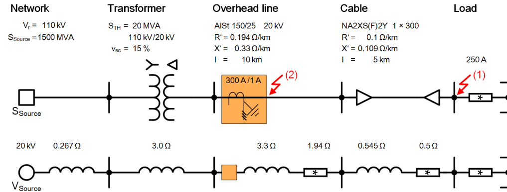
Figure A-4 Example for a System Design
