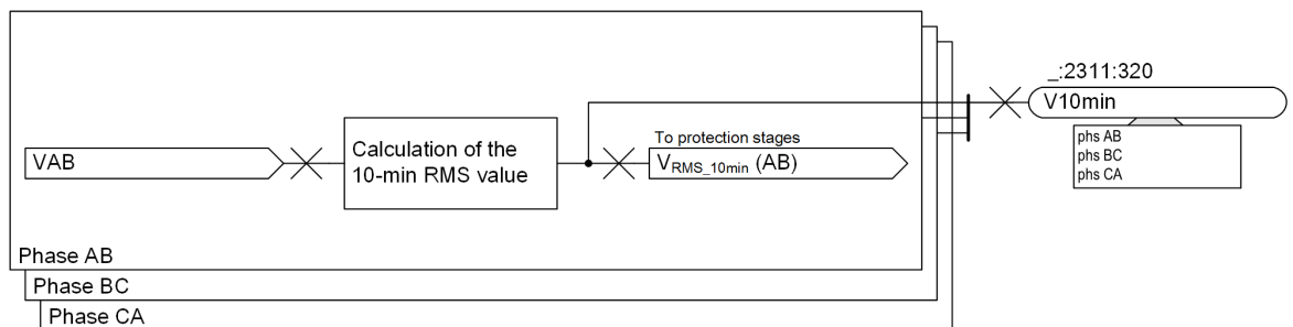
Figure 6-353 Logic Diagram of the General Functionality
