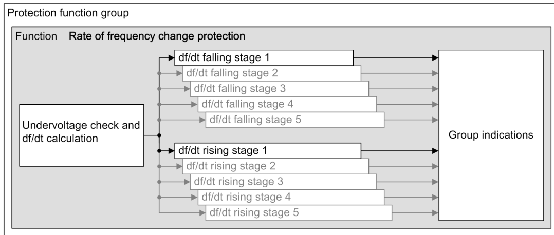
Figure 6-220 Structure/Embedding of the Function
