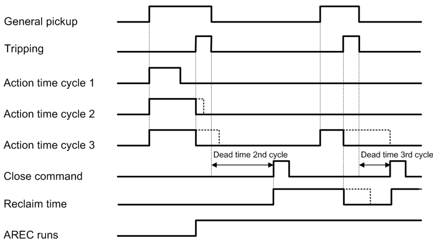
Figure 6-292 Operating-Mode Signal Examples: With Tripping/With Action Time
