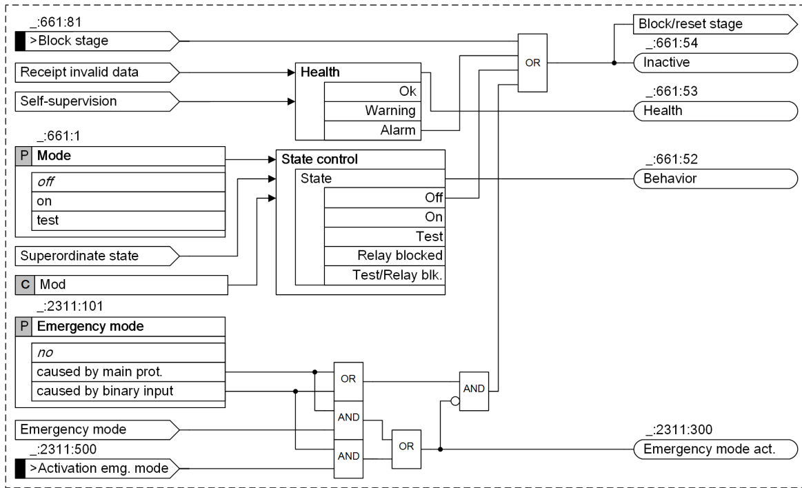
Figure 6-10 Logic Diagram of the Stage Control
