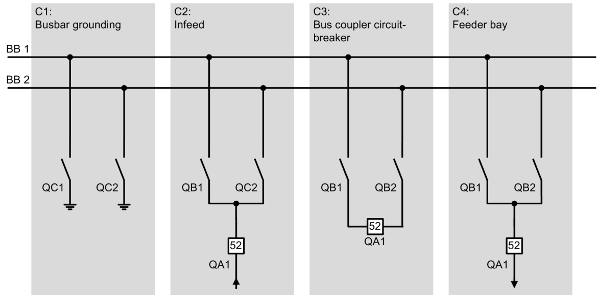
Figure 9-89 Example of a Substation
