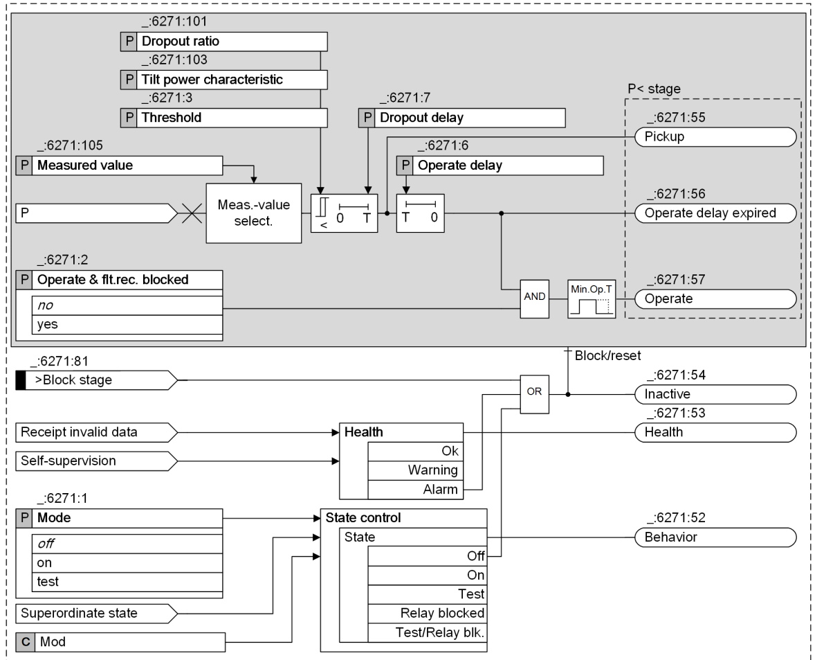
Figure 6-231 Logic Diagram of the Active Power Stage (Stage Type: Power P<)
