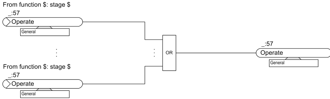
Figure 5-19 Generation of the Operate Indication of the Motor Function Group
