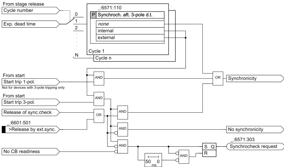
Figure 6-312 Cyclic Reclosing Function: Logic for the Query of the Synchronism
