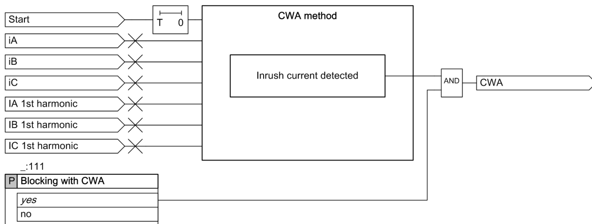
Figure 6-74 Logic of the CWA-Method Function (T = 1 Period)
