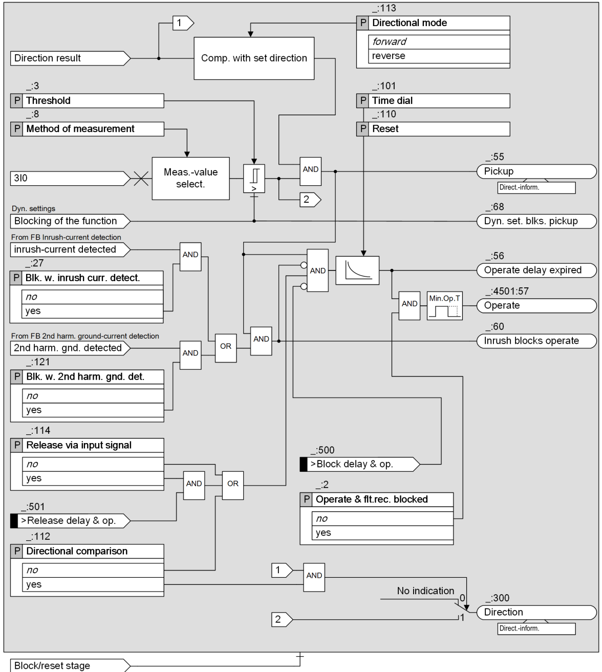
Figure 6-68 Logic Diagram of the Directional User-Defined Characteristic Curve Overcurrent Protection, Ground
