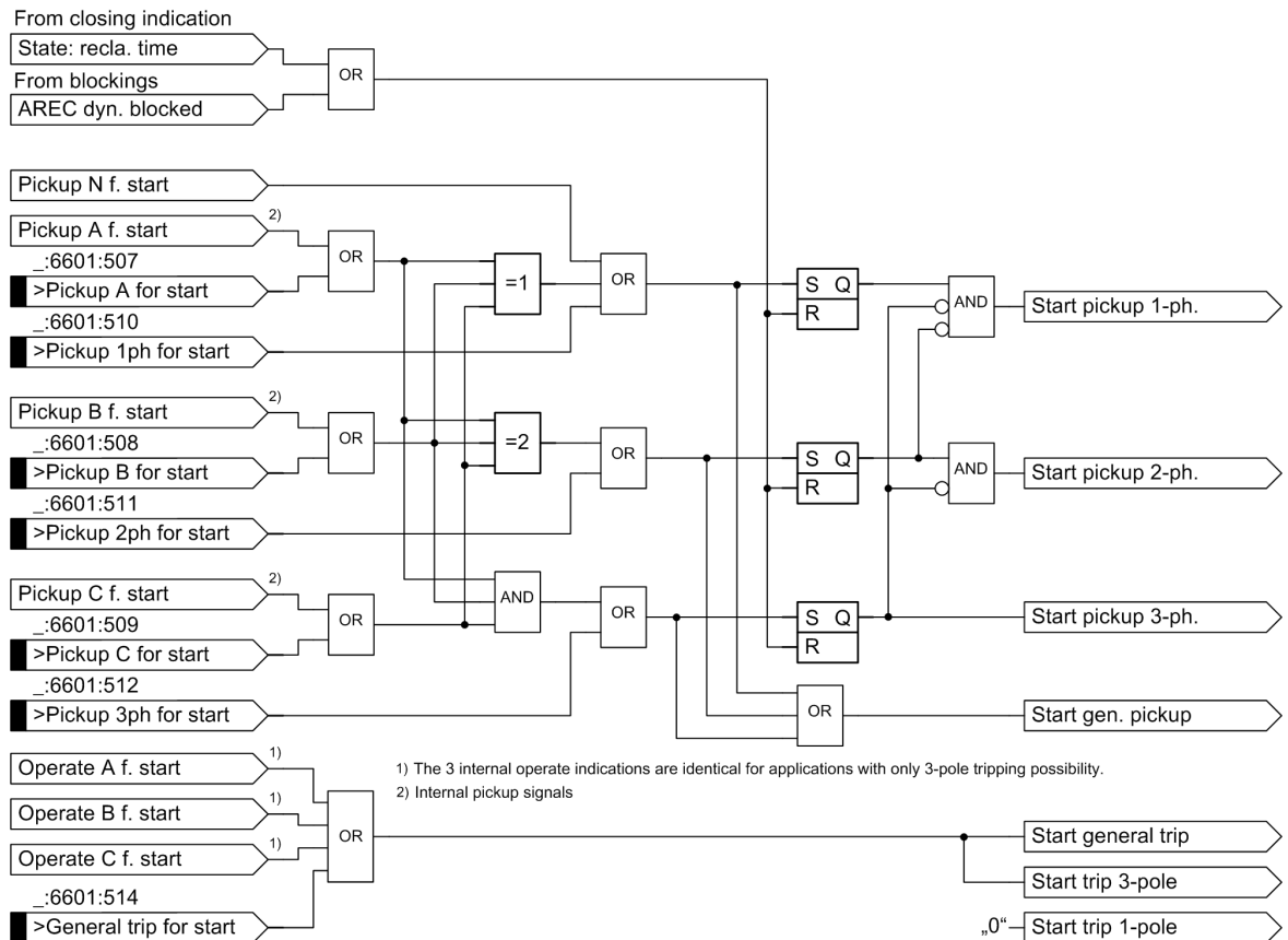
Figure 6-298 Input Logic for Operating Modes: With Pickup
