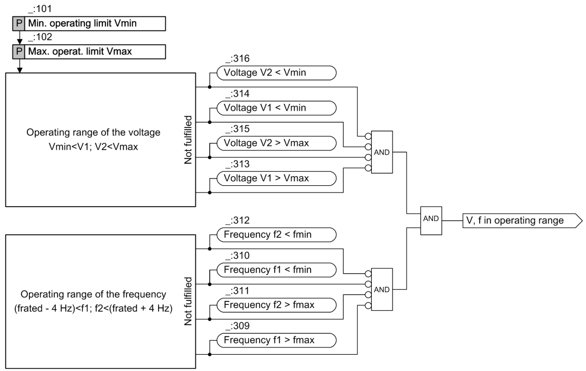
Figure 9-53 Logic of the Operating Ranges
