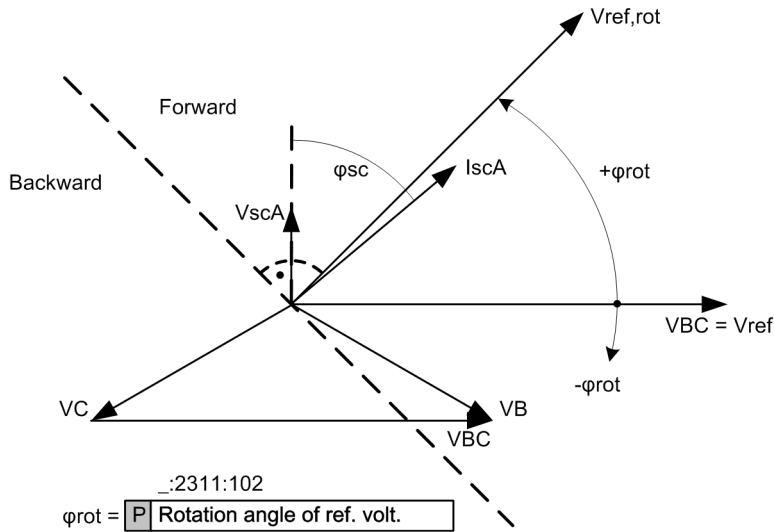
Figure 6-47 Rotation of the Reference Voltage, Phase-Measuring Element
