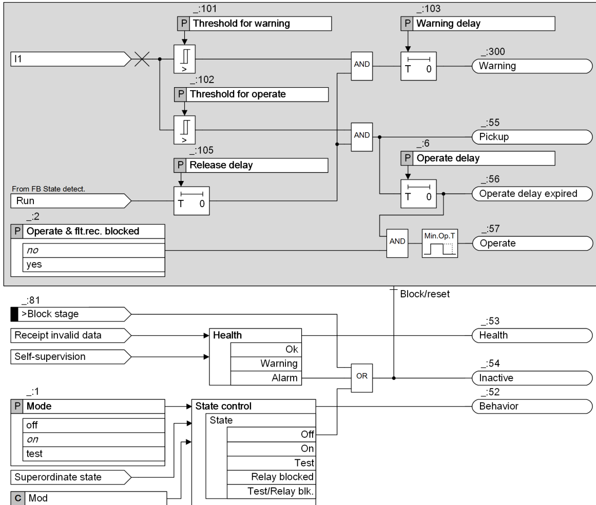
Figure 7-17 Logic Diagram of Load-Jam Protection
