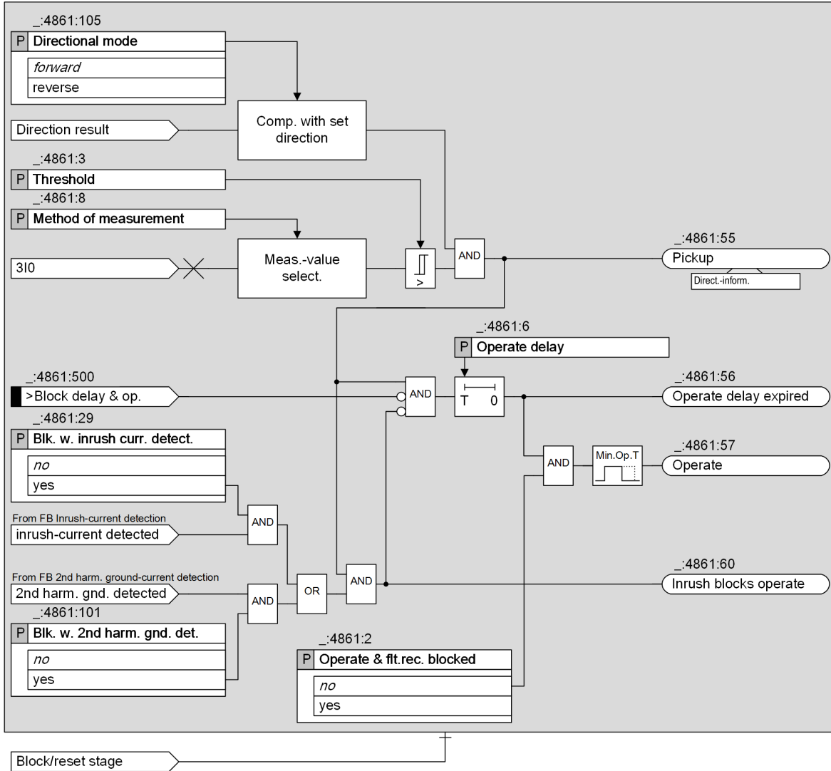
Figure 6-59 Logic Diagram of the Directional Definite-Time Overcurrent Protection, Ground – Basic
