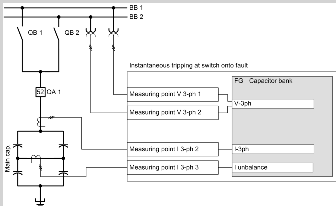
Figure 6-349 Double Busbar with Capacitor Bank
