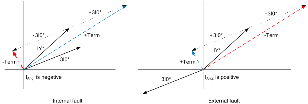
Figure 6-268 Angle Decision in Internal and External Faults
