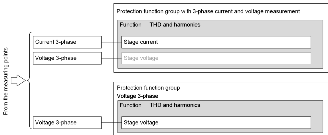
Figure 11-2 Structure/Embedding of the Function
