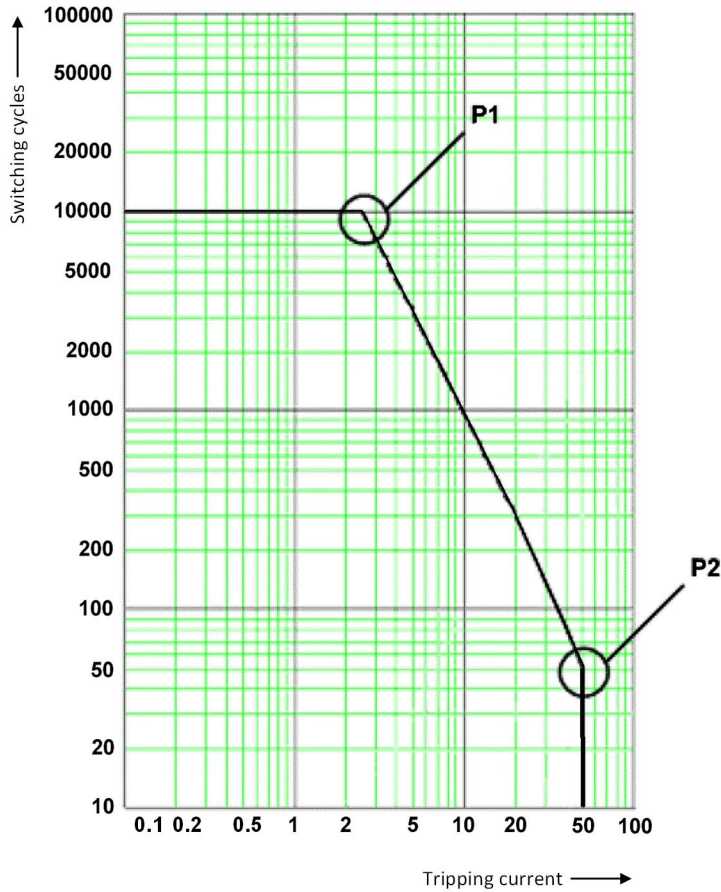
[dw_CB_WOpC, 2, en_US] Figure 11-11 Diagram of Switching Cycles for the 2P Method
