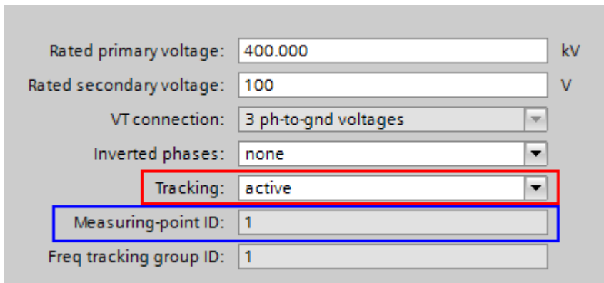
Figure 3-31 Using the Measuring Point to Determine the Sampling Frequency
