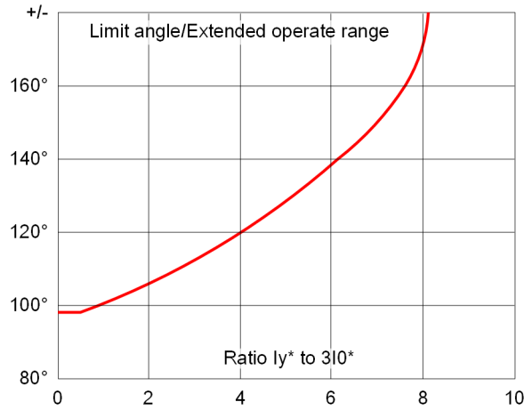
Figure 6-269 Ratio I_Y^* to 3I_0^*
