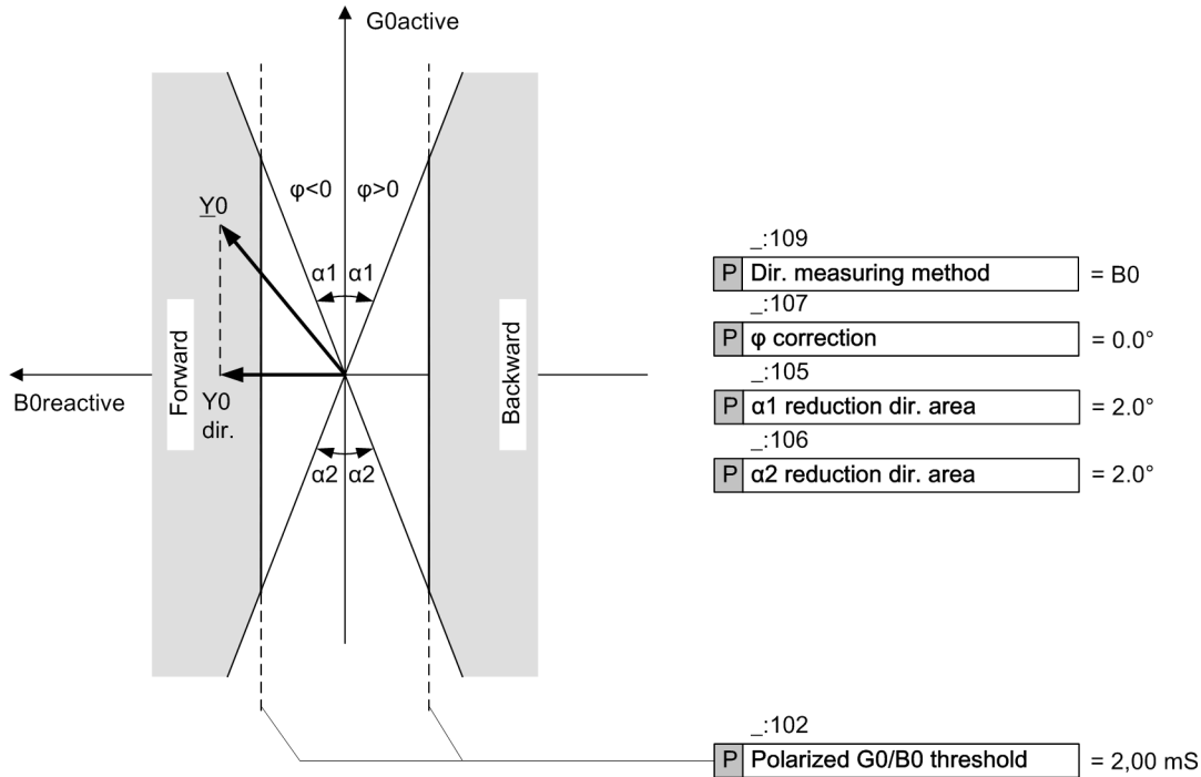
[dw_sl_co_Y0_1_en_US] Figure 6-134 Direction-Characteristic Curve for the B0 Measurement
