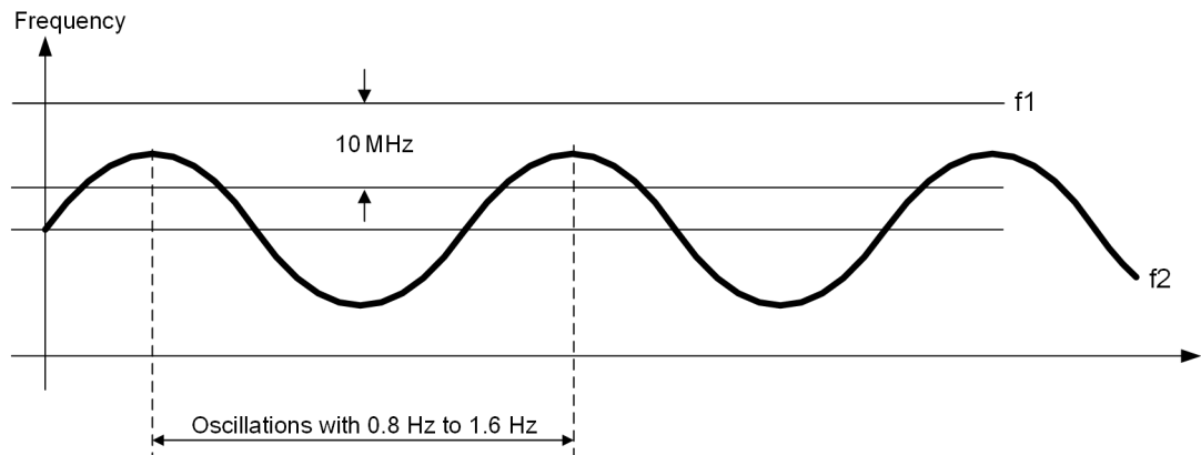
Figure 9-76 Example: Frequency Difference between the Constant Frequency f_1 and the Sinusoidal Oscillating Frequency f_2
