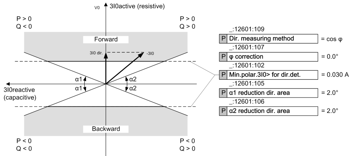
Figure 6-121 Direction-Characteristic Curve with Cos \phi Measurement
