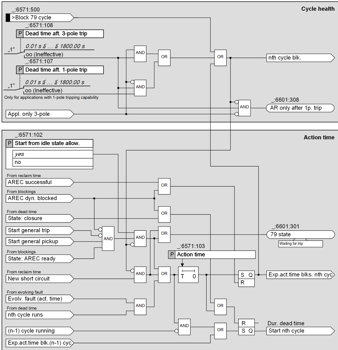
Figure 6-300 Cycle Control with Operating Mode: With Tripping/With Action Time
