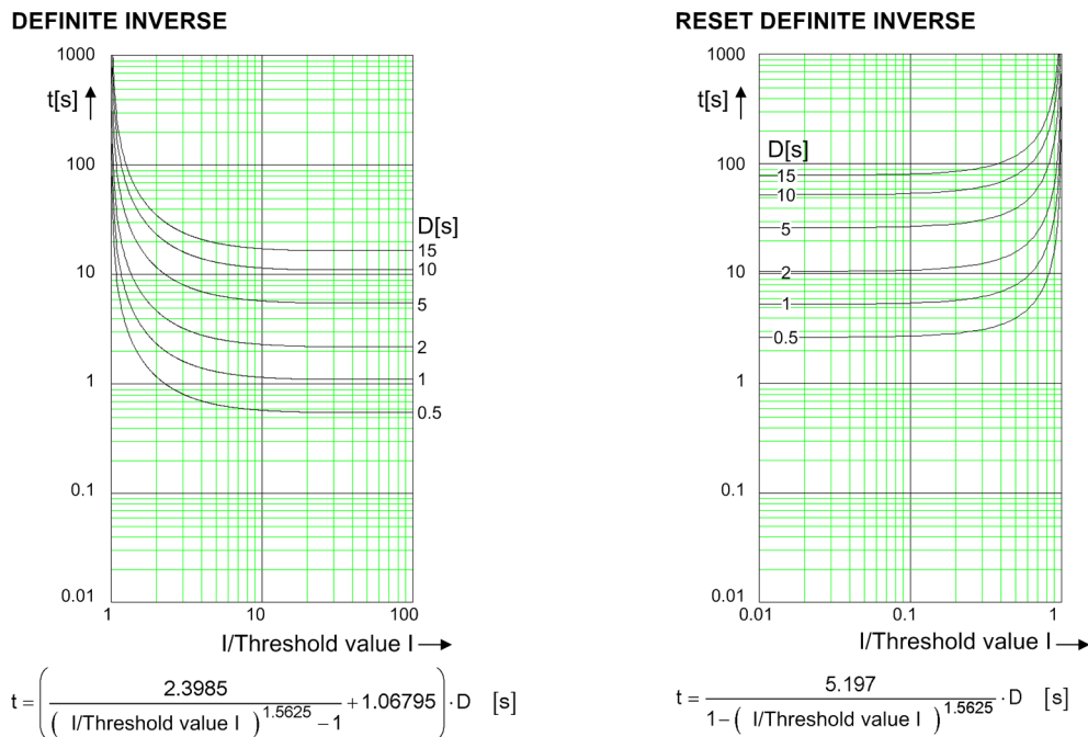
Figure 14-7 Operate Curves and Dropout-Time Characteristic Curves According to ANSI/IEEE
