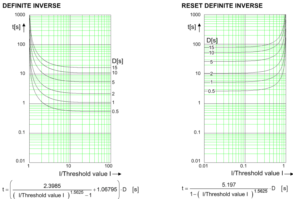
Figure 14-18 Operate Curves and Dropout-Time Characteristic Curves According to ANSI/IEEE
