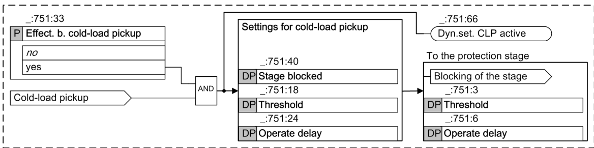
Figure 6-37 Influence of the Cold-Load Pickup Detection on the Overcurrent-Protection Stage
