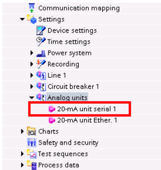
Figure 5-55 Insertion of the Function 20-mA Unit Serial 1
