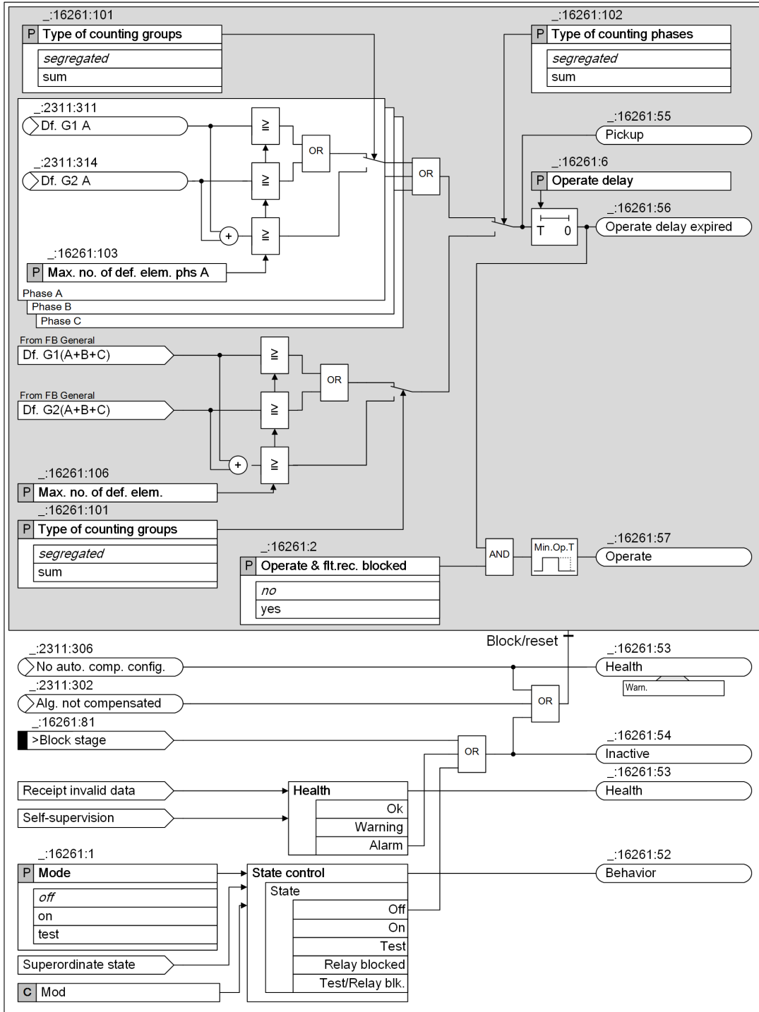
Figure 8-10 Logic Diagram of the Counter Stage
