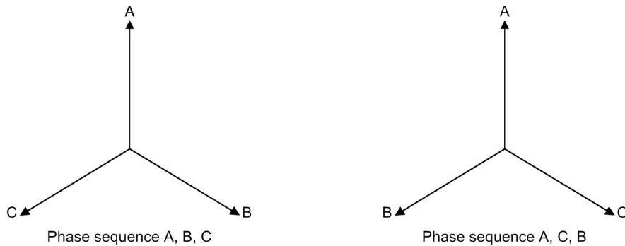
Figure 6-341 Vector with Different Phase Sequences
