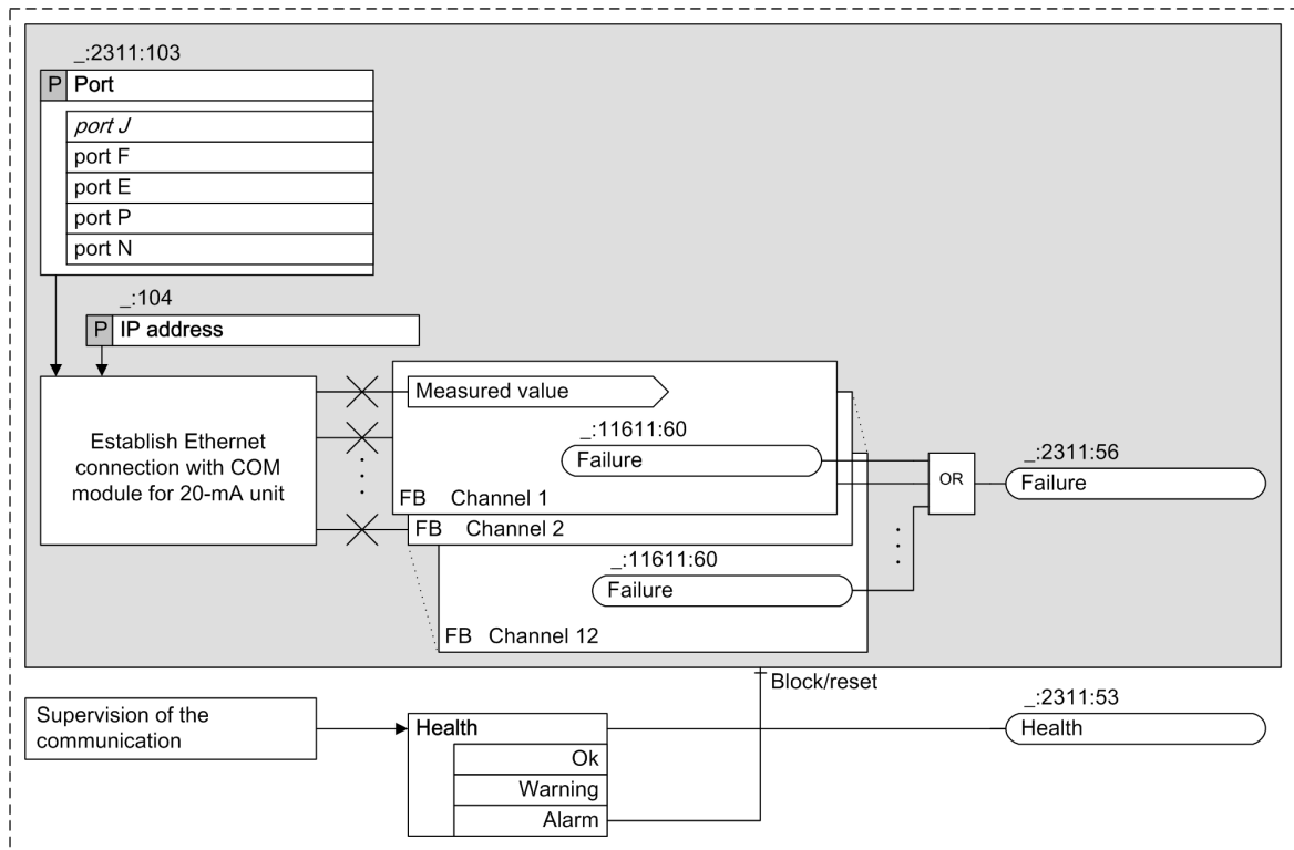
Figure 5-46 Logic of the Function 20-mA Unit Ethernet
