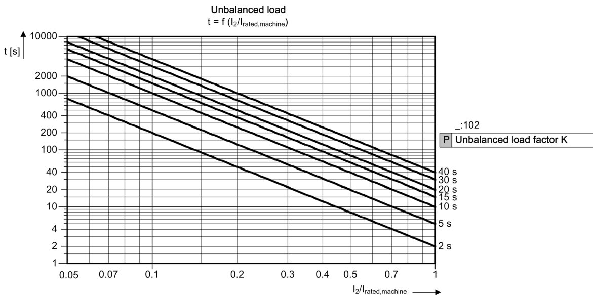
Figure 14-11 Thermal Characteristic for Unbalanced Load Protection
