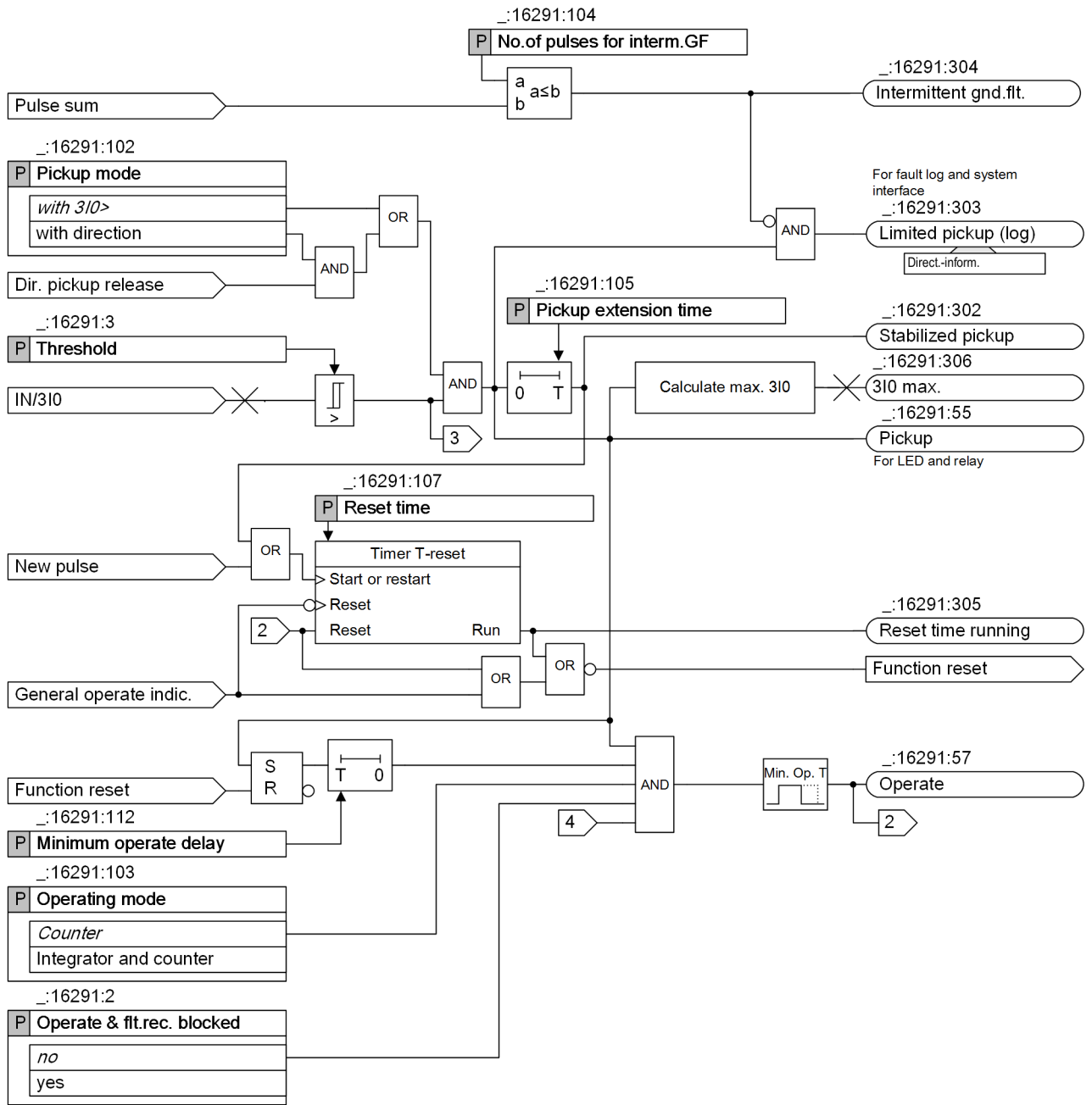
Figure 6-110 Pickup, Operate, and Reset Logic in Operating Mode Counter
