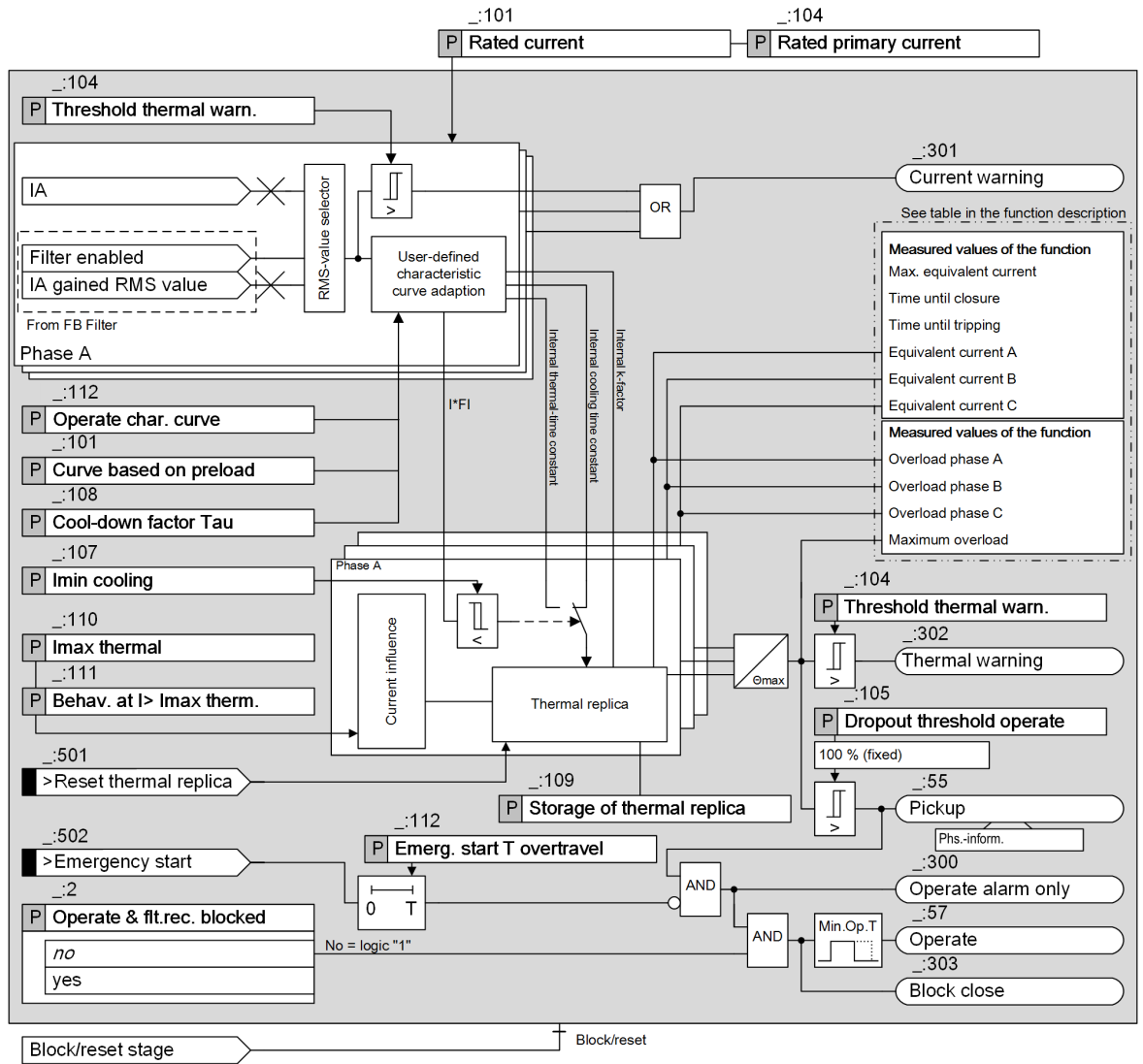
Figure 6-165 Logic Diagram of the Thermal Overload Protection, User-Defined Characteristic Curve Function
