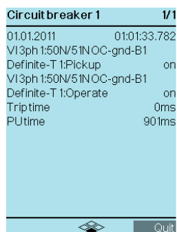
Figure 3-29 Spontaneous Fault Display on the Device
