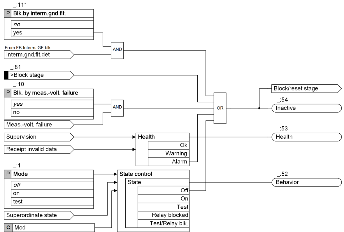
Figure 6-127 Logic Diagram of the Stage Control
