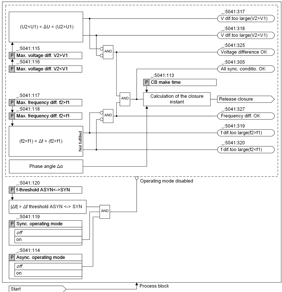
Figure 9-61 Closing Conditions when Switching Asynchronous Systems
