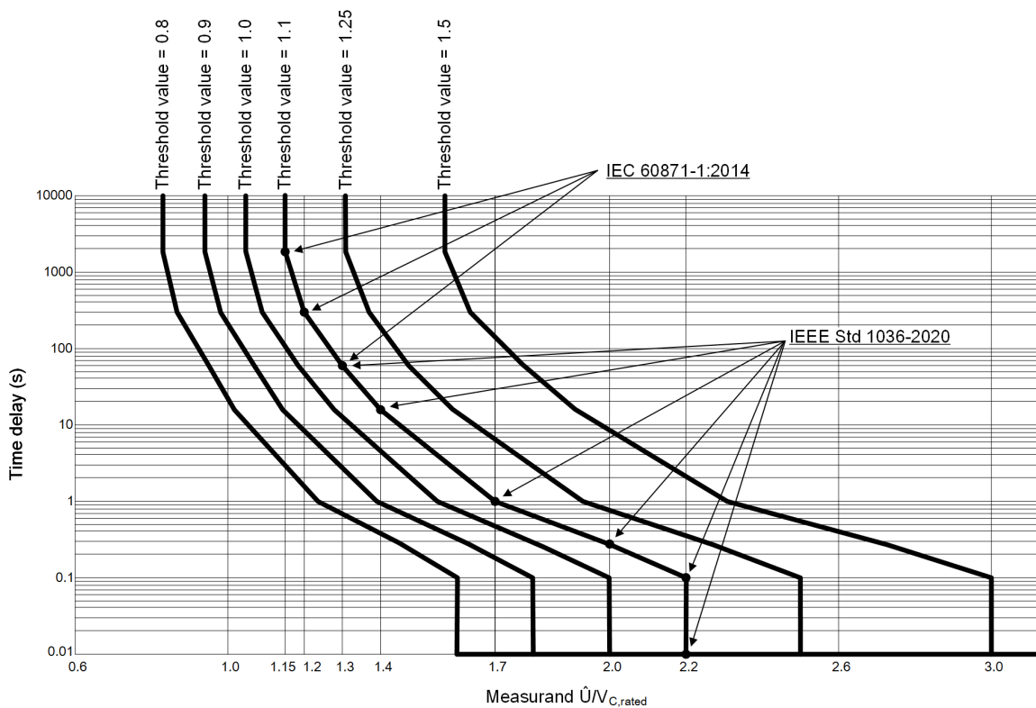
Figure 14-19 Inverse-Time Characteristic Curve
