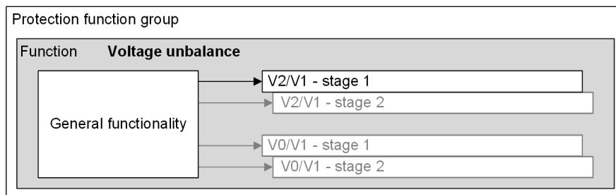
Figure 12-10 Structure/Embedding of the Function
