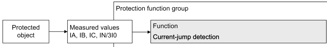
Figure 6-345 Structure/Embedding of the Function
