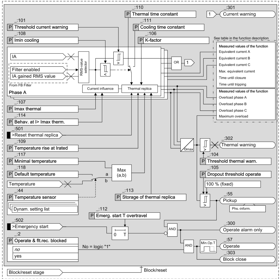
Figure 6-161 Logic Diagram of the Thermal Overload Protection, 3-Phase - Advanced Stage
