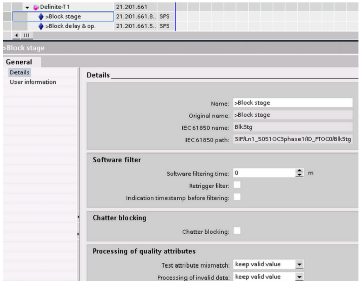
Figure 3-44 Influence Options for a Binary Input Signal (SPS Input Signal)
