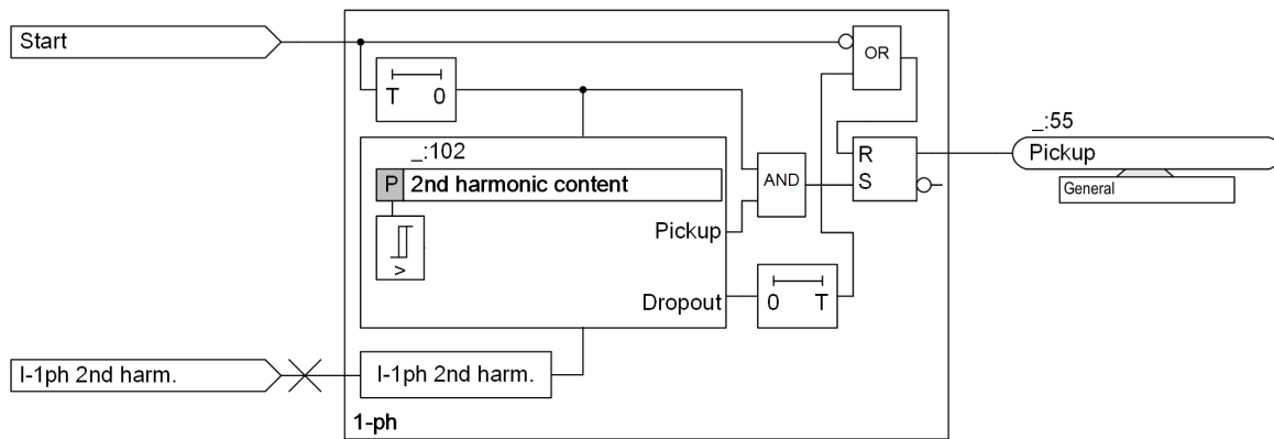
Figure 6-79 Logic of the Harmonic Analysis Function
