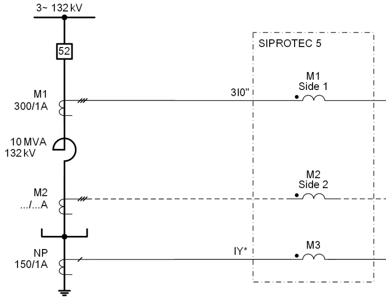
Figure 6-280 Application with Neutral Reactor
