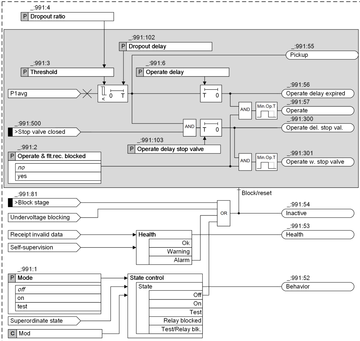
Figure 6-237 Logic Diagram of the Reverse-Power Protection Stage
