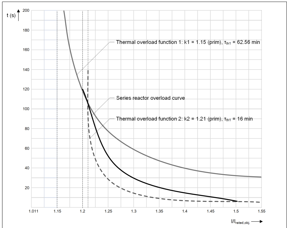
Figure 6-167 User-Defined Characteristic Curve with Replica of Standard Characteristics
