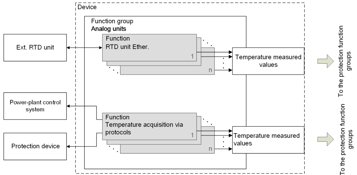
Figure 5-44 Structure of the Function Group Analog Unit
