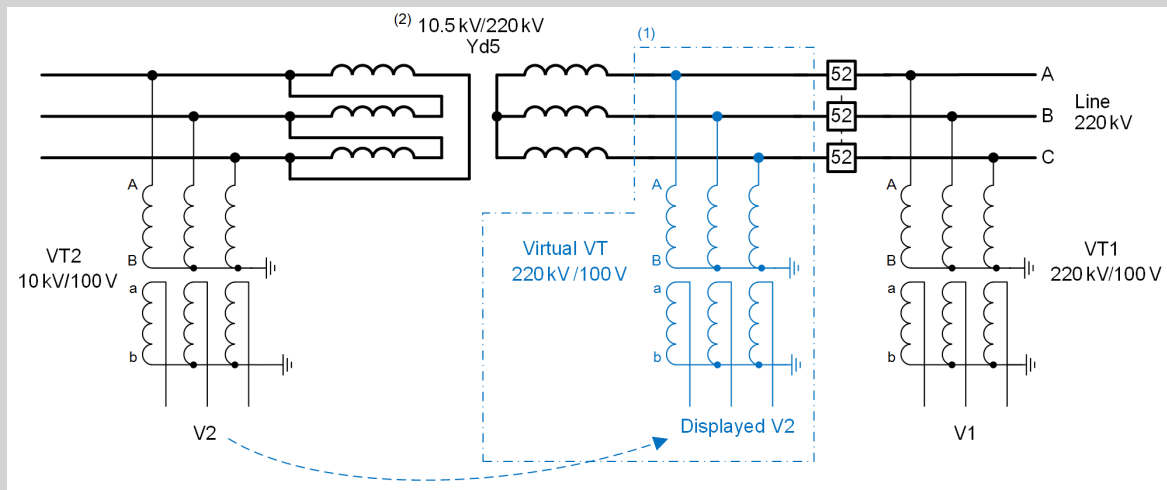
Figure 9-55 Example: the Electrical Power System with a Power Transformer
