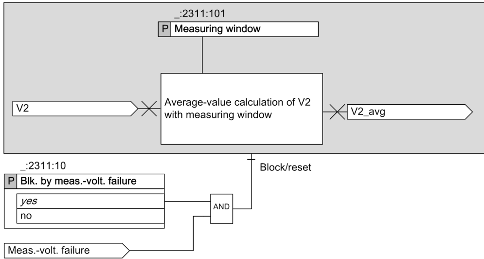
Figure 6-186 Logic Diagram of the General Functionality
