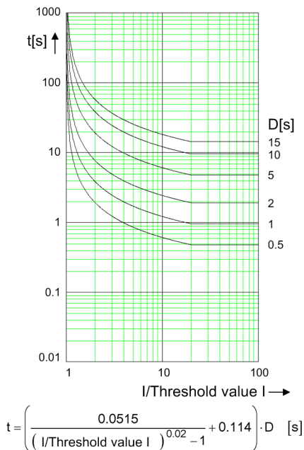
Figure 14-5 Operate Curves and Dropout-Time Characteristic Curves According to ANSI/IEEE
