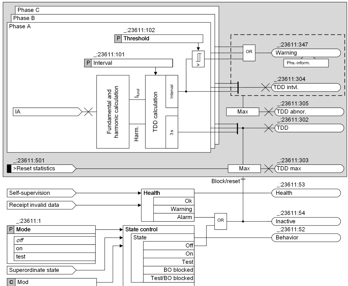
Figure 12-18 Logic Diagram of the Stage Current
