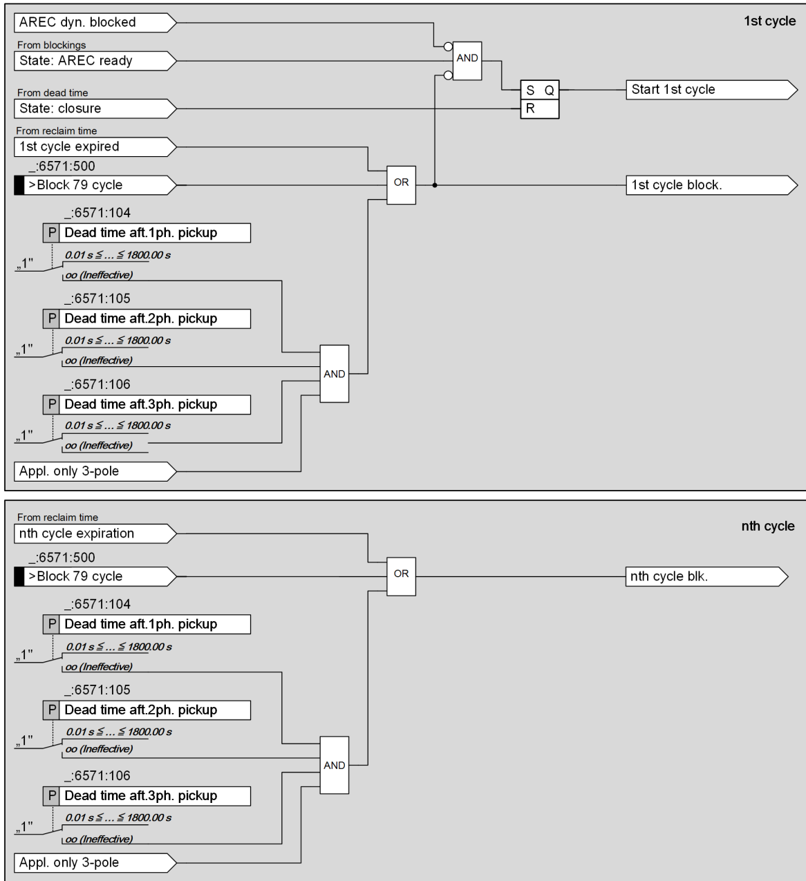
Figure 6-303 Cycle Control with Operating Mode: With Pickup/Without Action Time
