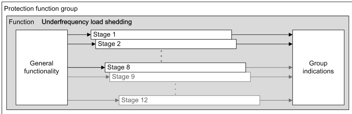
Figure 6-214 Structure/Embedding of the Function
