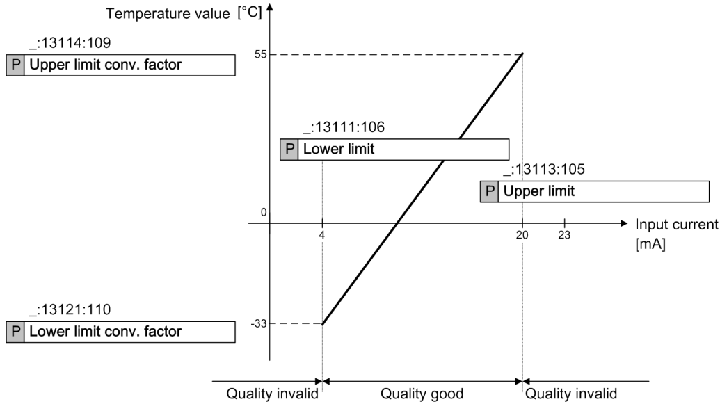
[dw_knges2_1_en_US] Figure 5-51 Characteristic Curve of a 20-mA Unit (Example 2)
