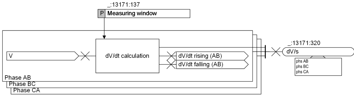
Figure 6-208 Logic Diagram of the General Functionality
