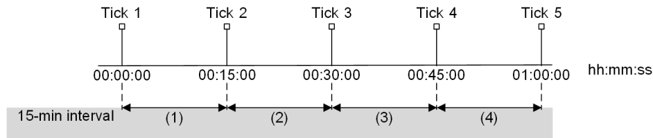
Figure 12-19 Ticks and 15-Min Intervals in an Hour
