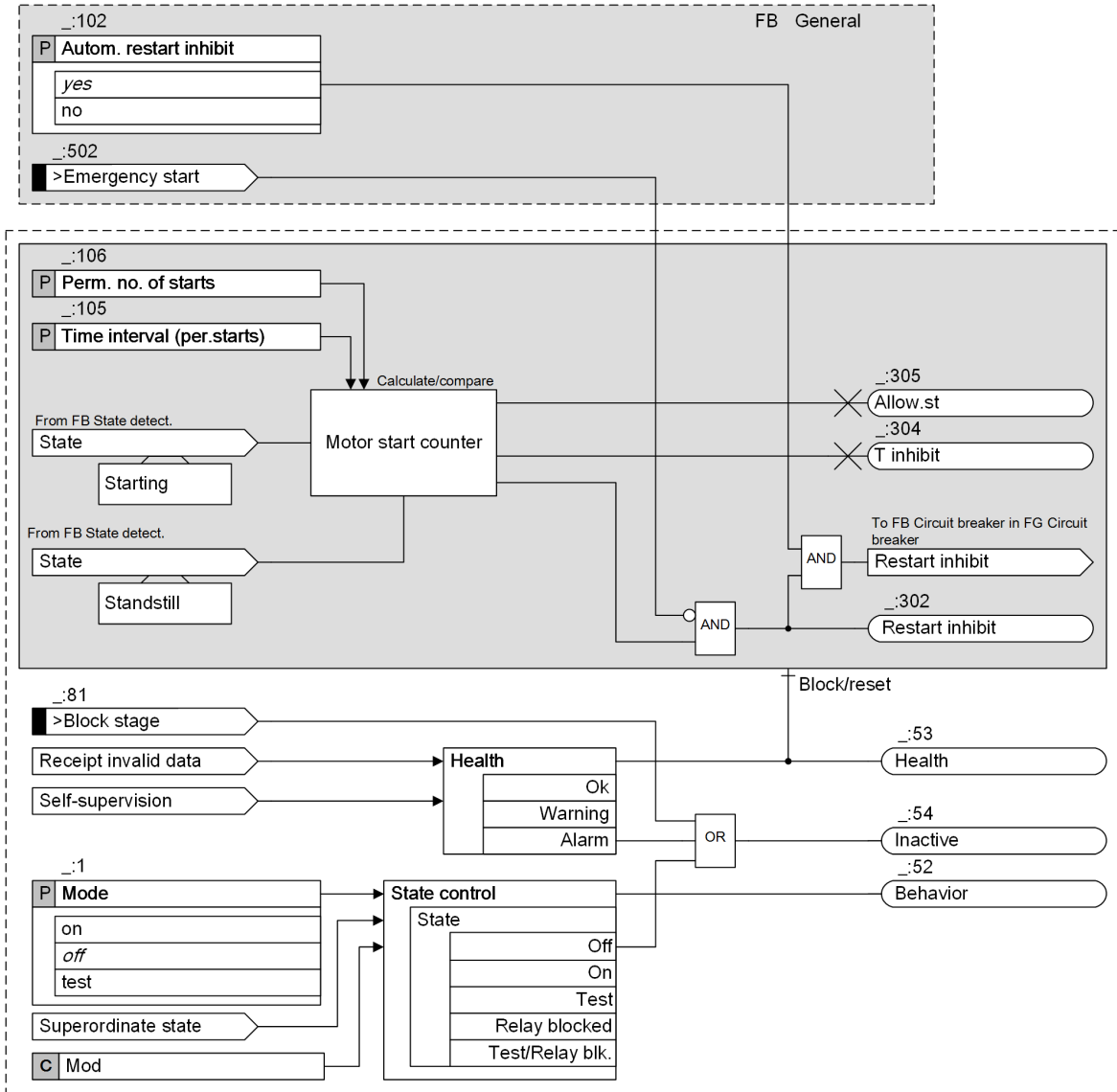
Figure 7-12 Logic Diagram of the Counter Stage
