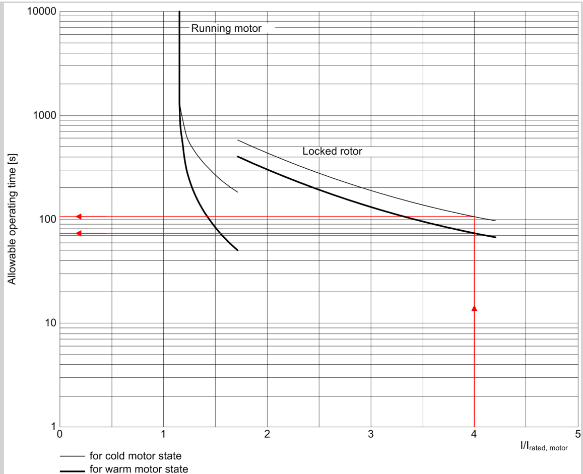
Figure 7-5 Thermal-Limit Curve
