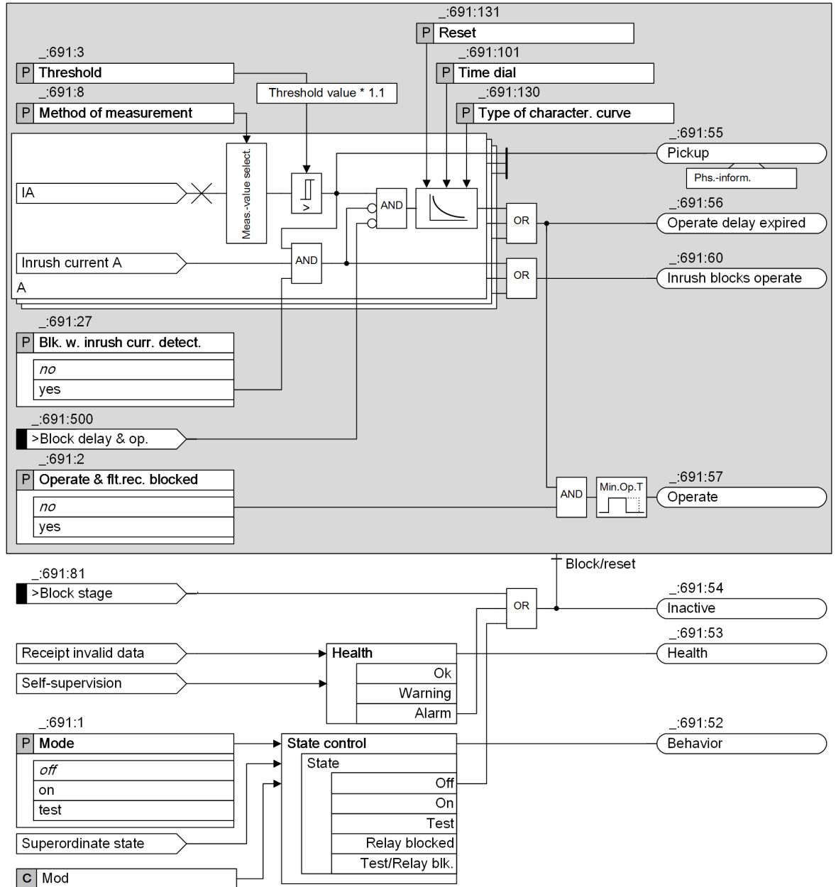
Figure 6-13 Logic Diagram Inverse-Time Overcurrent Protection (Phases) – Basic
