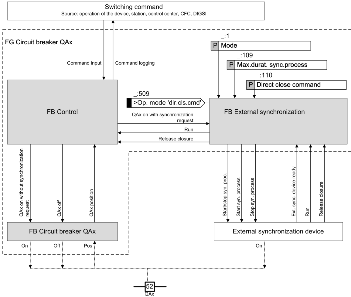
[dw_extsyn-02, 1, en_US] Figure 9-82 Interaction between Control and External Synchronization
