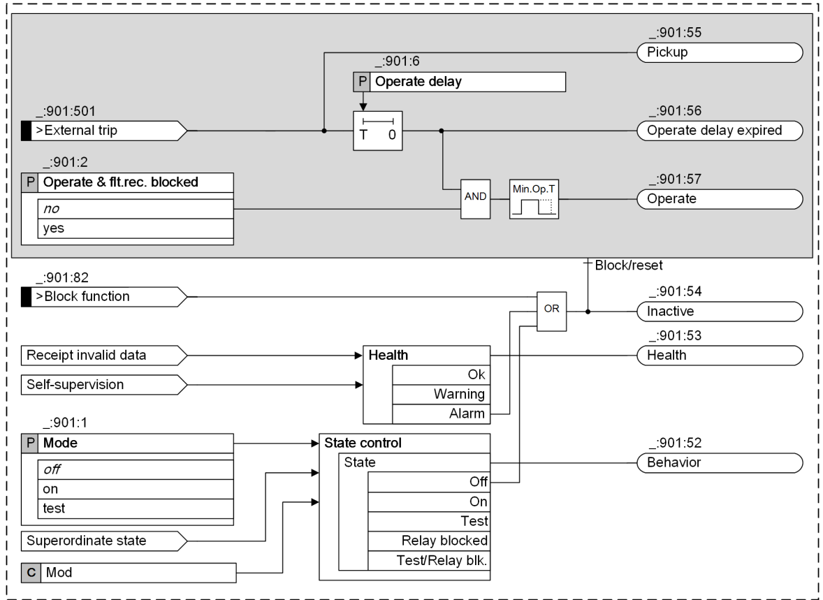
Figure 6-282 Logic Diagram for the External Trip-Initiation Stage
