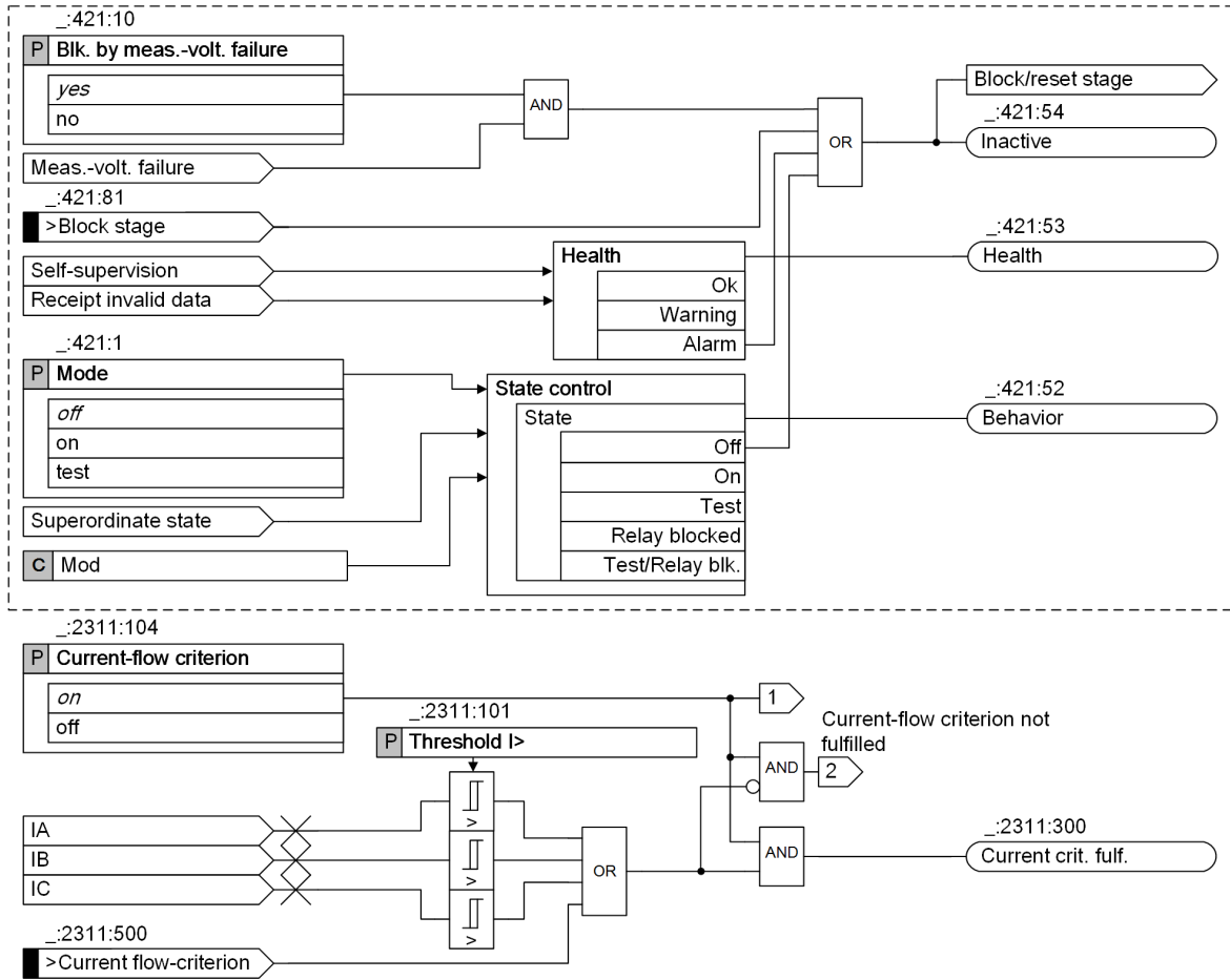
Figure 6-198 Logic Diagram Stage Control
