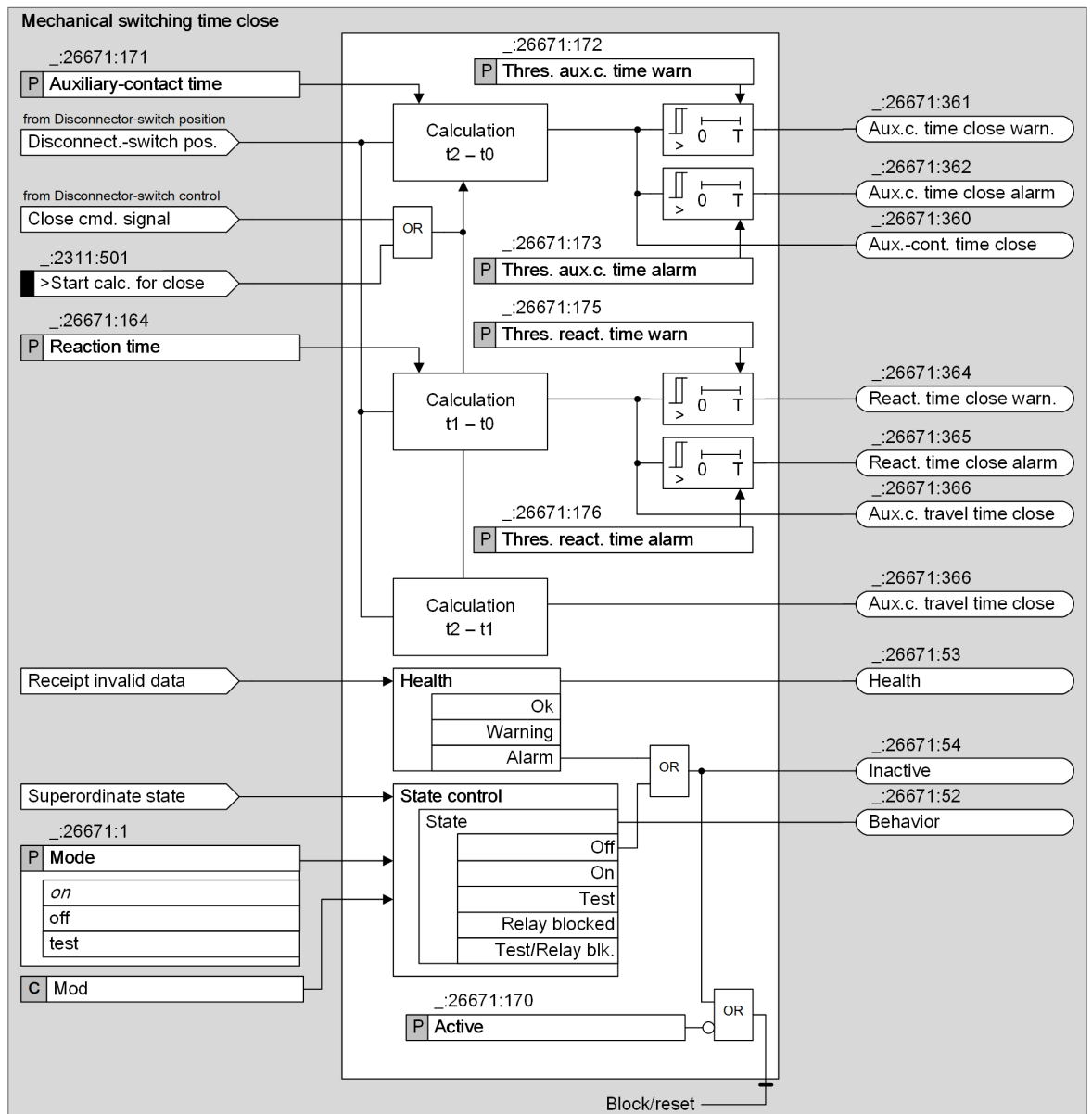
Figure 11-23 Logic of the Stage Mechanical Switching Time Close for Disconnecter
