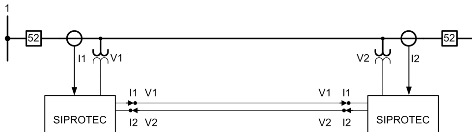
Figure 6-332 Data Exchange for 2 Devices, Each With Protection Communication
