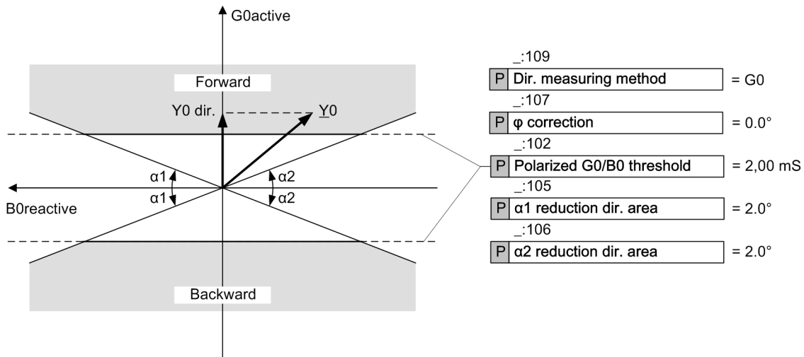
[dw_Y0_dir.1_en_US] Figure 6-132 Direction-Characteristic Curve for the G0 Measurement
