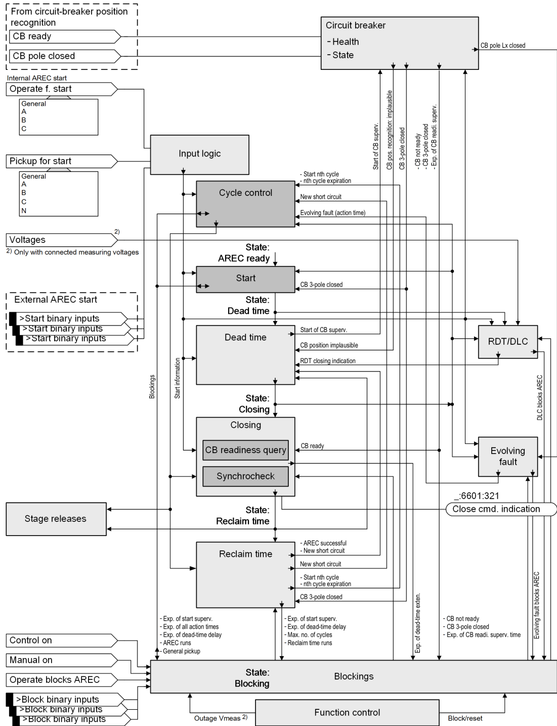
[to_zyk_aws_2_en_US] Figure 6-296 Cyclic Automatic Reclosing: Block Diagram of Automatic Reclosing
