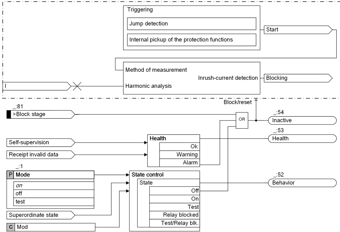
Figure 6-78 Logic of 2nd Harmonic Detection 1-Phase
