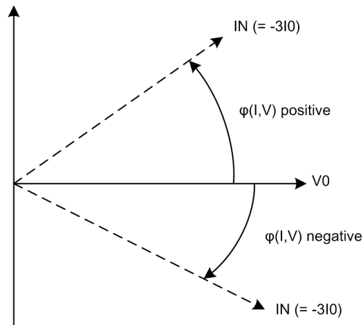
Figure 6-55 Measured-Value Definition
