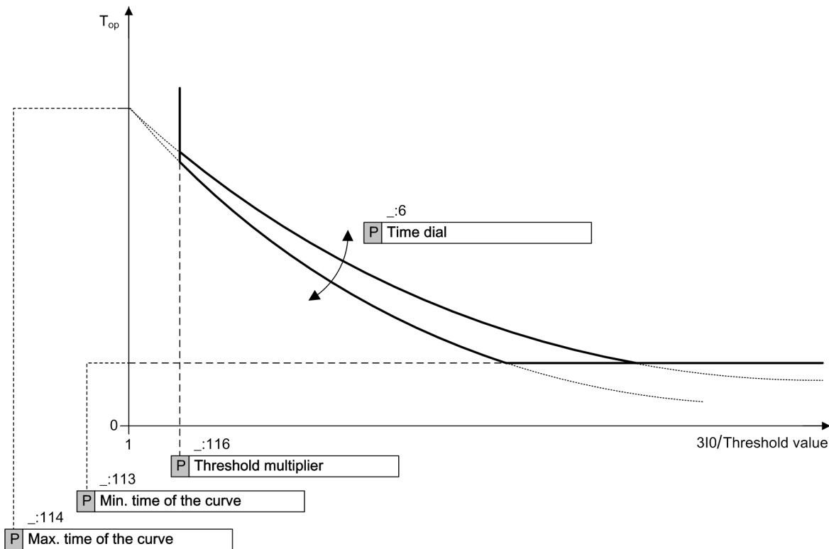
Figure 14-8 Operate Curve of Logarithmic Inverse-Time Characteristic
