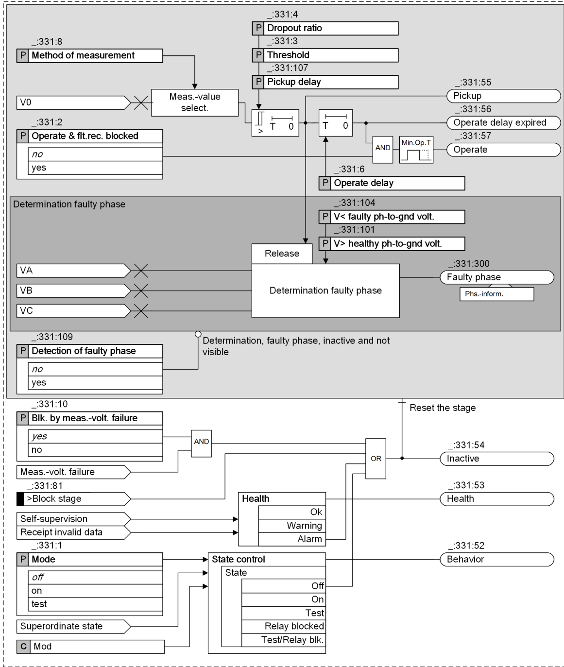
Figure 6-182 Logic Diagram of the Definite-Time Overvoltage Protection with Zero-Sequence Voltage/Residual Voltage
