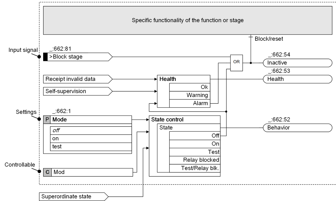
[[io_steurg, 2, en_US] Figure 2-4 General Control of a Function
