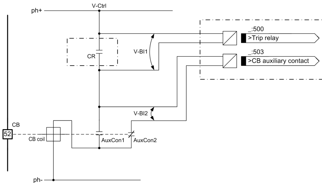
Figure 10-37 Principle of Trip-Circuit Supervision with 2 Binary Inputs
