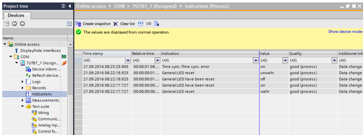
Figure 3-27 Displaying Spontaneous Device Indications in DIGSI 5
