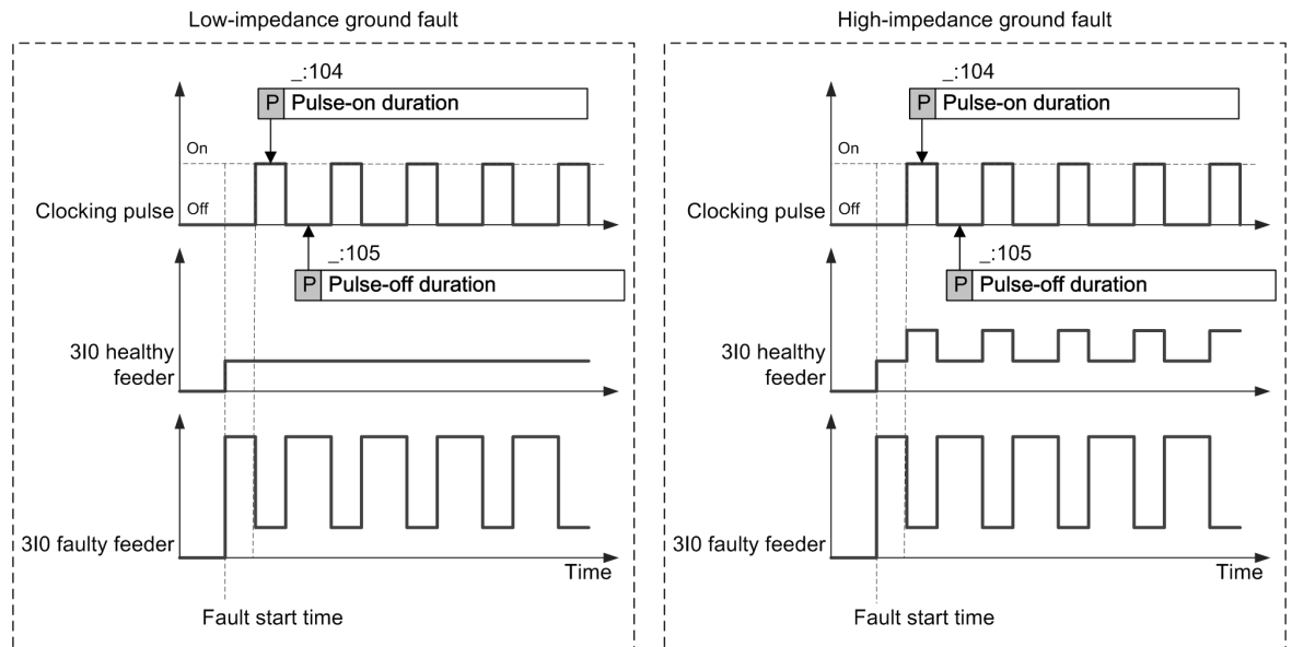
Figure 6-143 Current Pulse Pattern in the Overcompensated System
