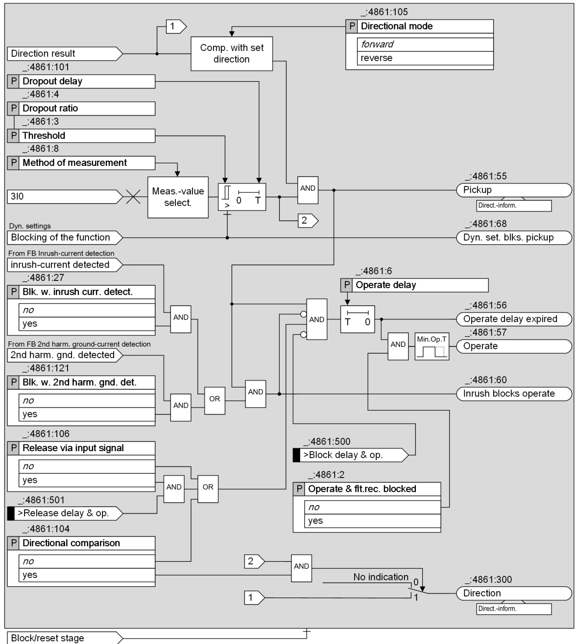
Figure 6-60 Logic Diagram of the Directional Definite-Time Overcurrent Protection, Ground – Advanced
