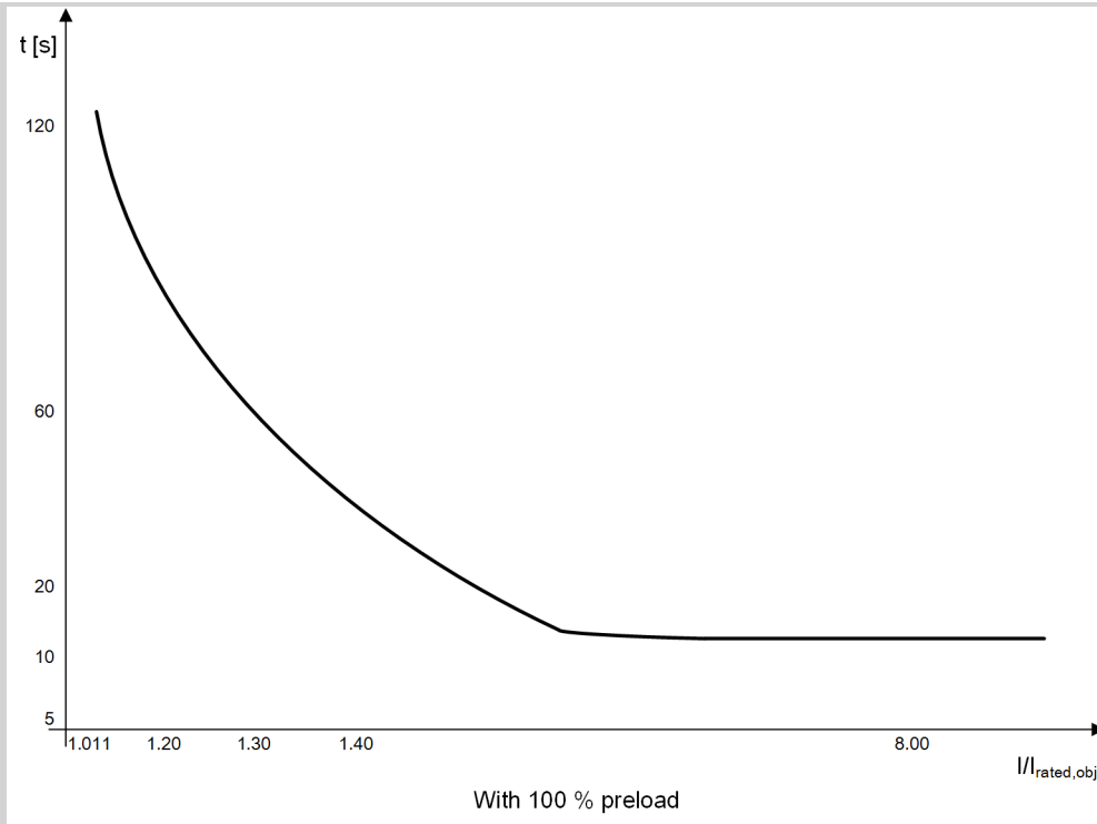
Figure 6-169 Example of the User-Defined Characteristic Curve
