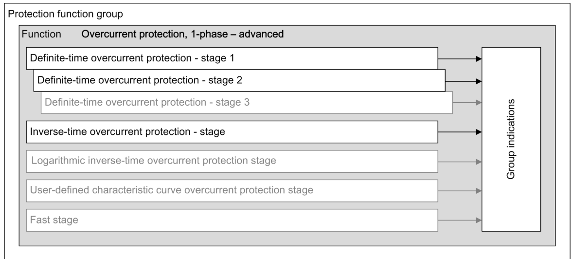
Figure 6-84 Structure/Embedding the Function Overcurrent Protection, 1-Phase – Advanced
