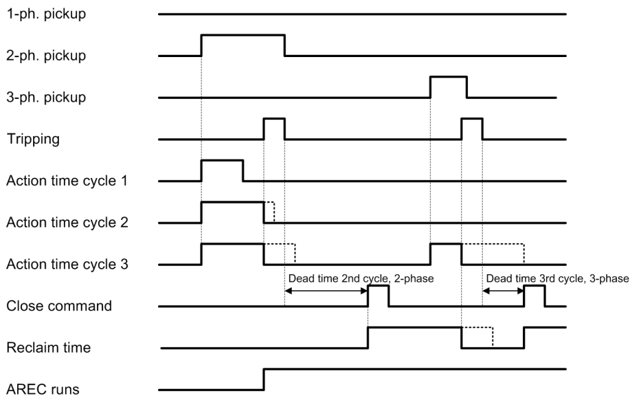
Figure 6-293 Operating-Mode Signal Examples: With Pickup/With Action Time
