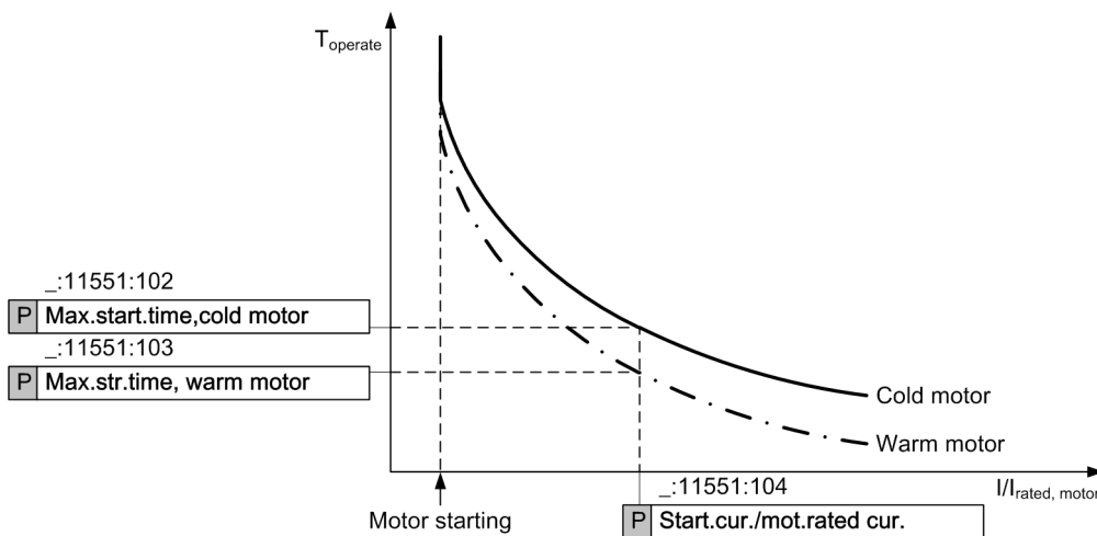
Figure 7-3 Thermal Characteristic Curve with Starting Current
