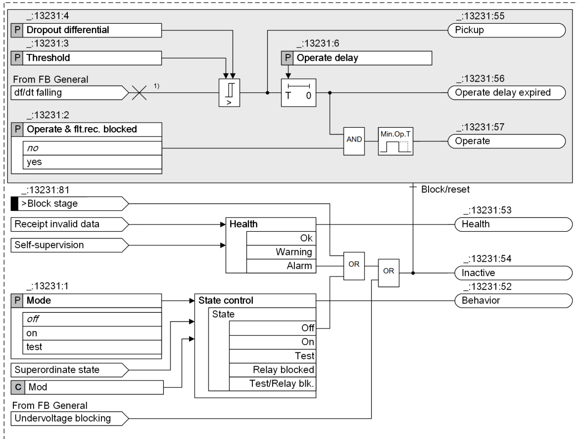
Figure 6-222 Logic Diagram of Rate of Frequency Change Protection
