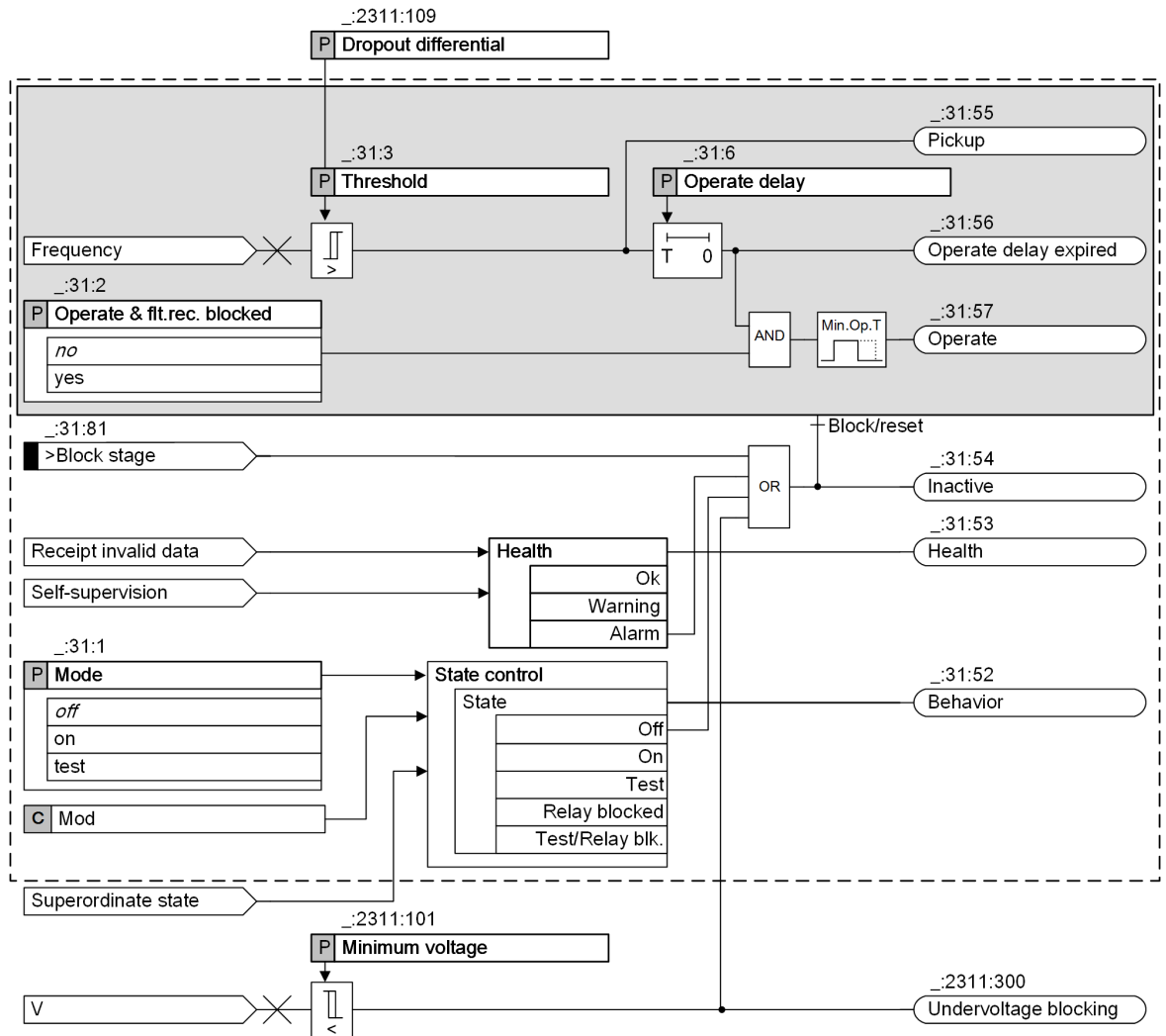
Figure 6-211 Logic Diagram of the Overfrequency-Protection Stage
