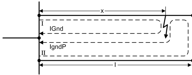
[dwparkomnw-161013, 1, en_US] Figure 6-337 Radius of Parallel-Line Compensation at II
