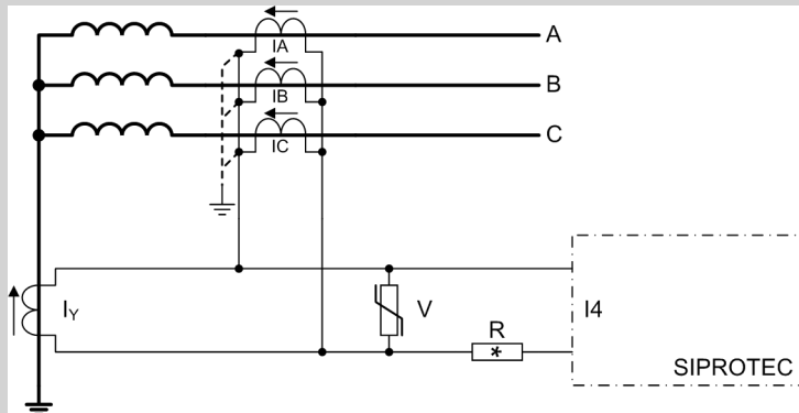
Figure 6-97 Connection Diagram of the Restricted Ground-Fault Protection According to the High-Impedance Principle
