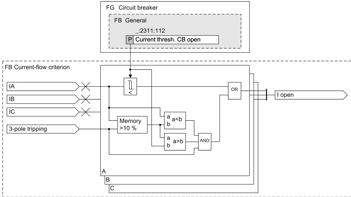
Figure 5-21 Logic Diagram of the Current-Flow Criterion Function Block
