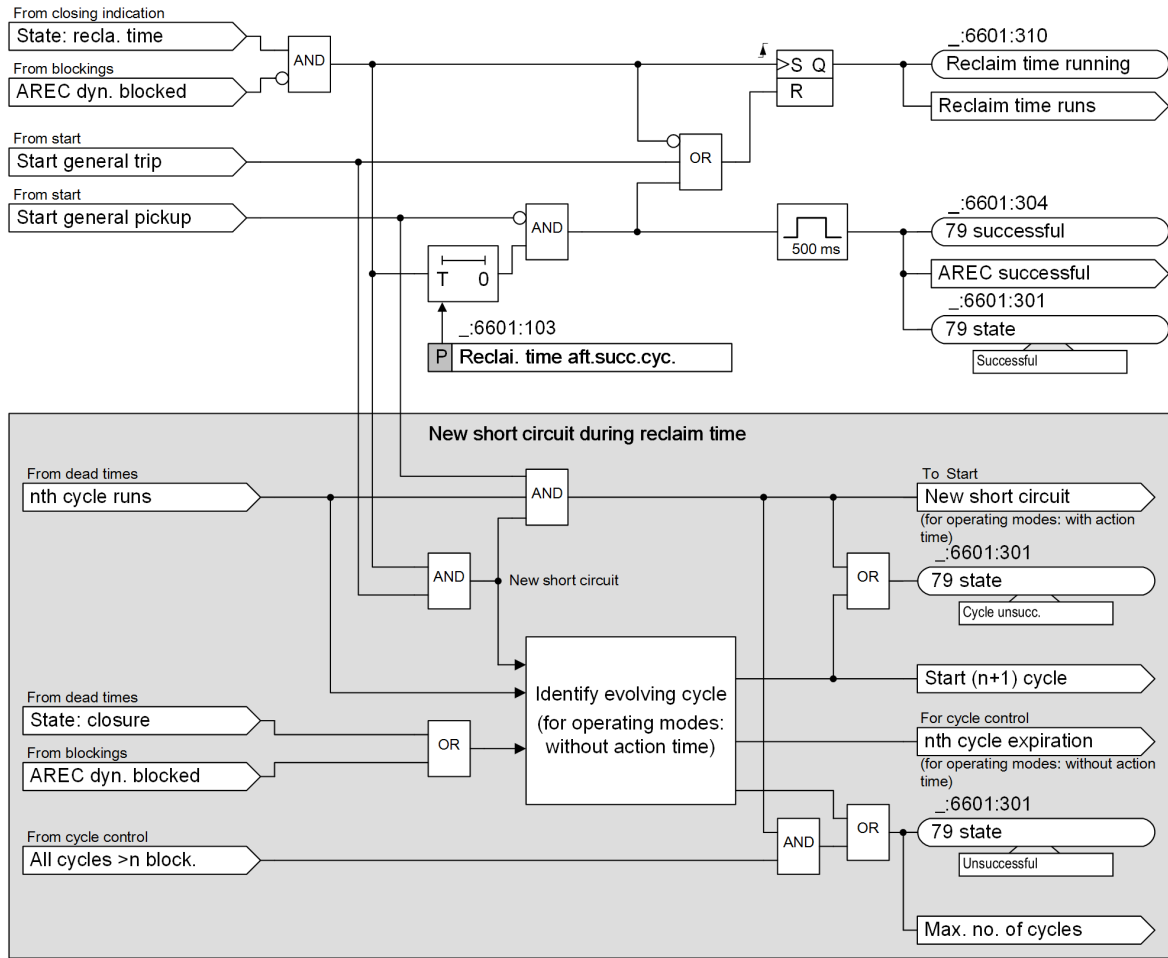
Figure 6-313 Cyclic Automatic Reclosing: Logic for the Reclaim Time
