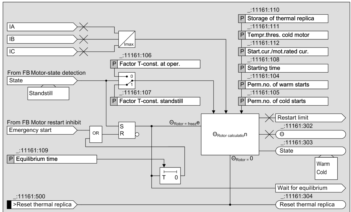
Figure 5-29 Logic Diagram of the Thermal Replica Rotor Function Block
