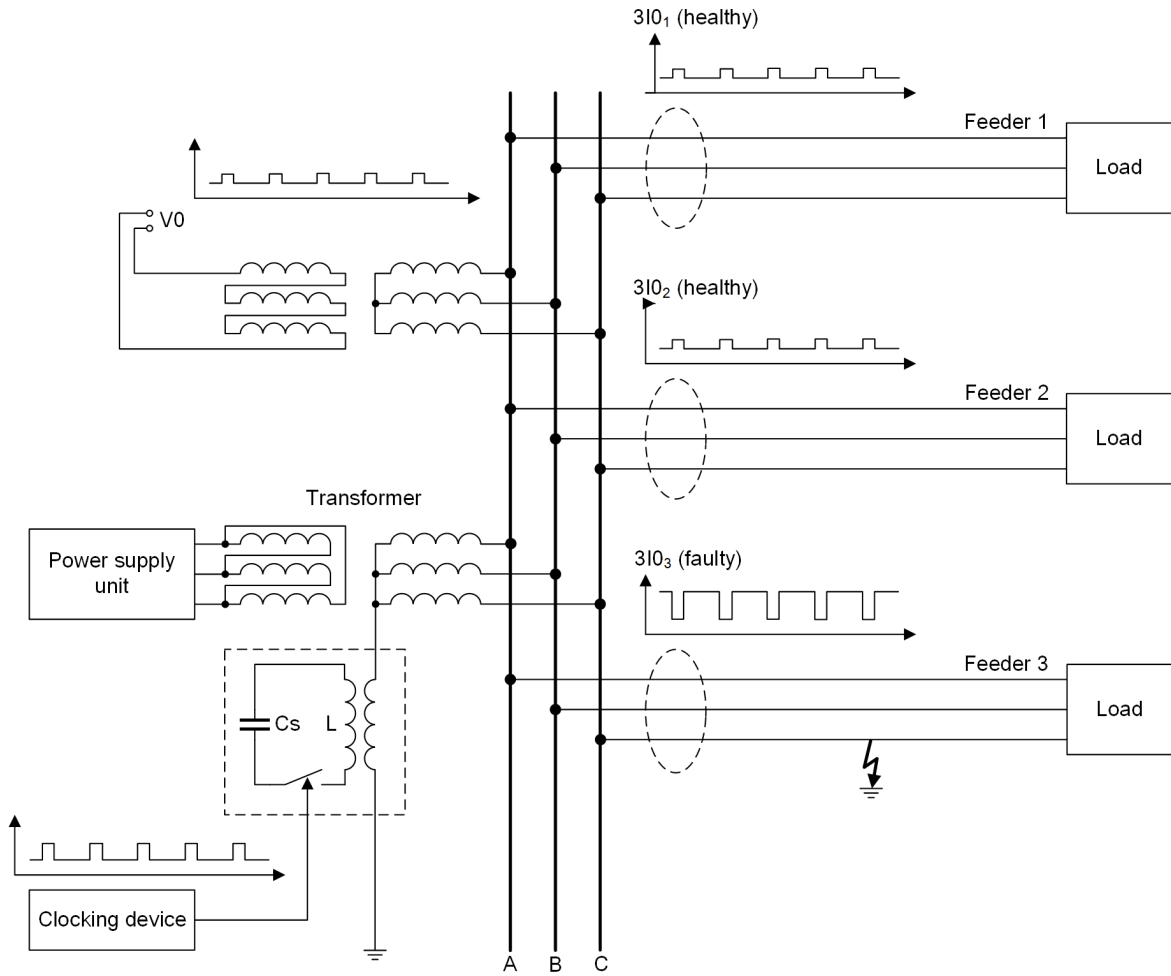
[dw_pulse detection network, 2, en_US] Figure 6-142 Network that Uses the Pulse-Pattern Detection
