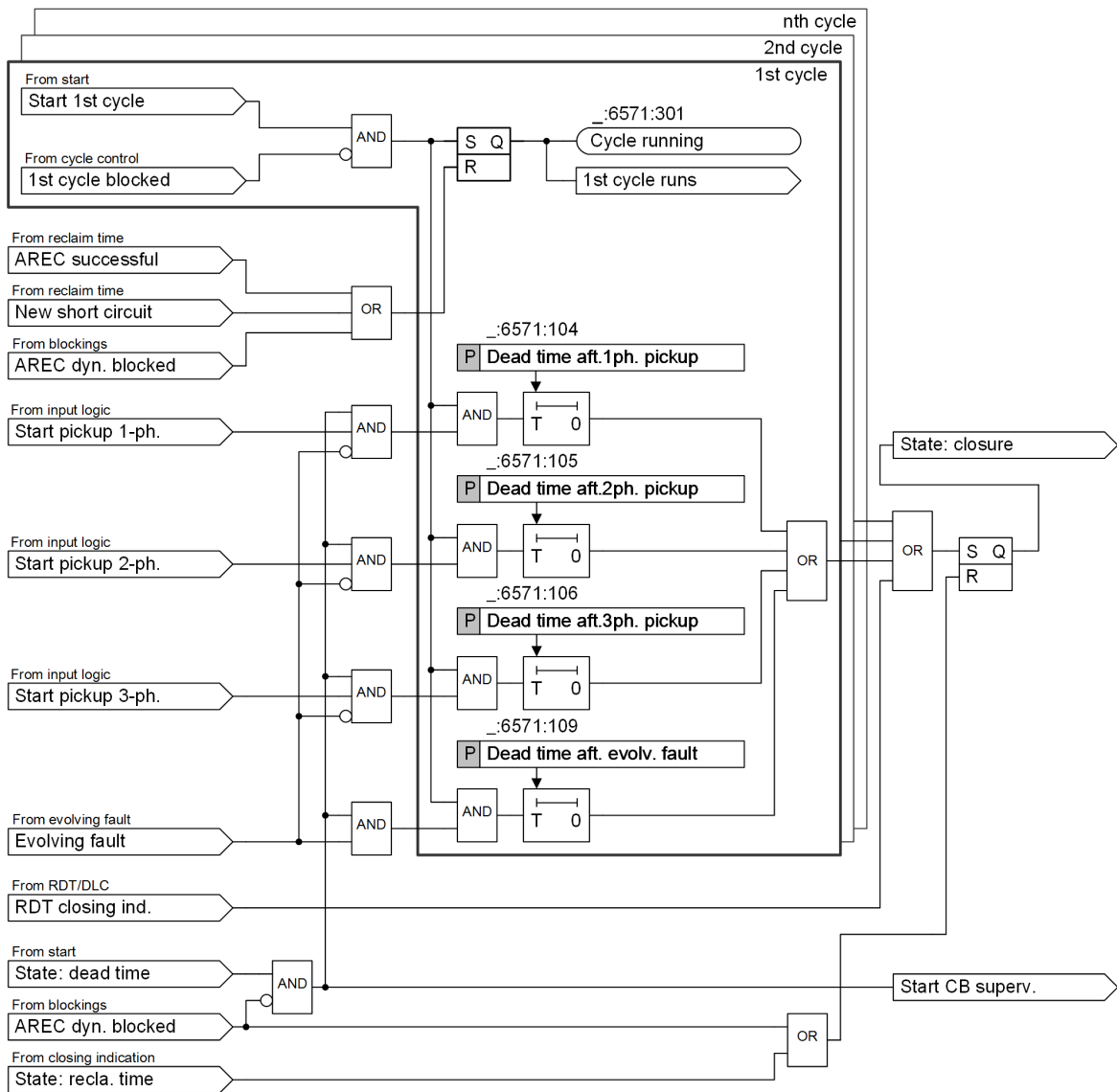
Figure 6-307 Cyclic Automatic Reclosing Function – Logic of the Dead Time for the Operating Modes: With Pickup
