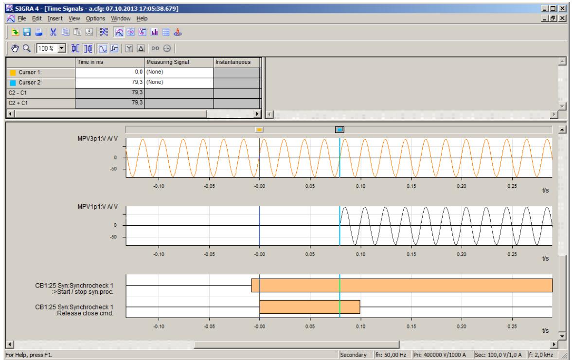
Figure 13-12 Measurement of the Circuit-Breaker Make Time
