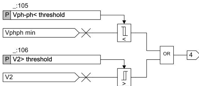
Figure 6-28 Logic Diagram of the Definite-Time Overcurrent Protection, Voltage-Released Undervoltage Seal-in, Part 2
