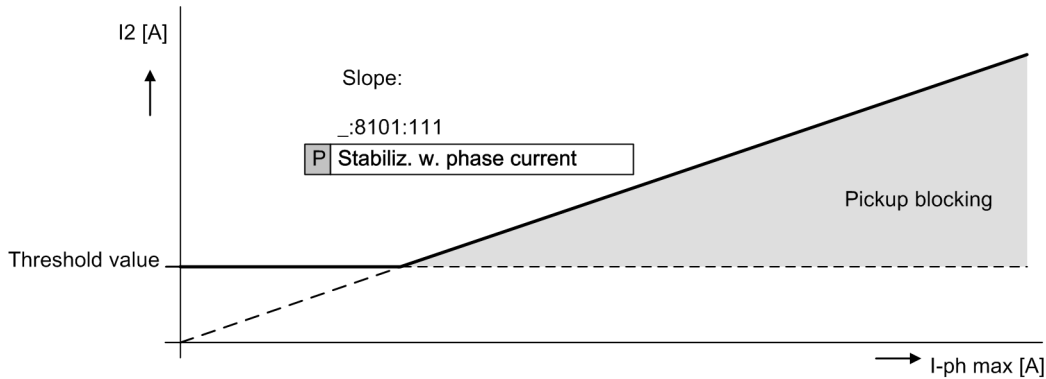
Figure 6-156 Stabilization with Phase Currents
