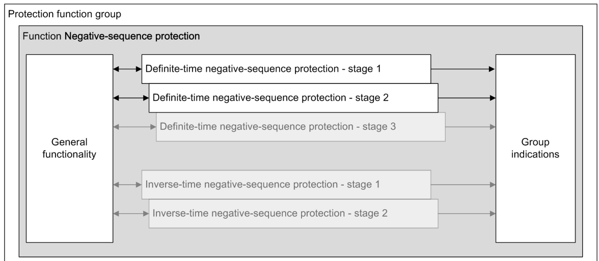
Figure 6-149 Structure/Embedding of the Function
