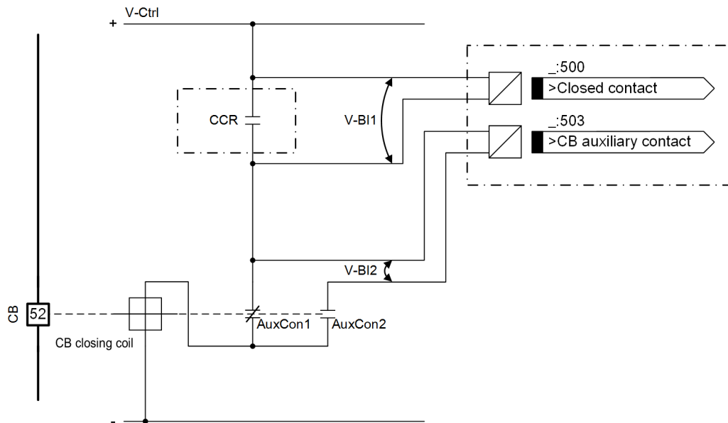
Figure 10-45 Principle of the Closing-Circuit Supervision with 2 Binary Inputs
