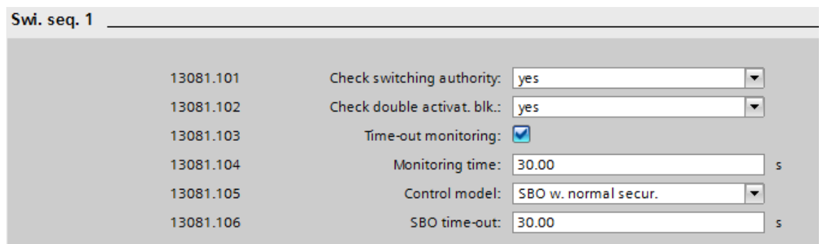
[sc_ccs4pa, 1, en_US] Figure 9-87 Settings of the Switching Sequence Function Block
