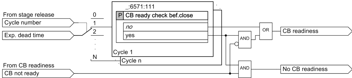
Figure 6-311 Cyclic Reclosing Function: Logic for the Query of the Circuit-Breaker Readiness Directly before Closing
