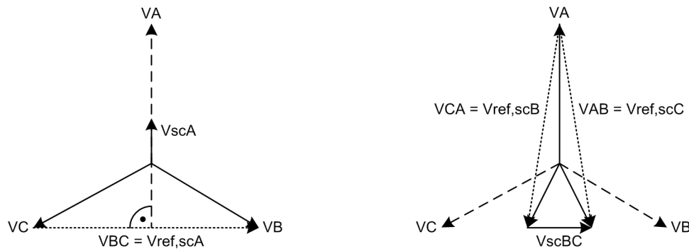
Figure 6-46 Cross-Polarized Voltages for Direction Determination
