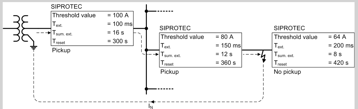
Figure 6-106 Example of Selectivity Criteria of the Intermittent Ground-Fault Protection
