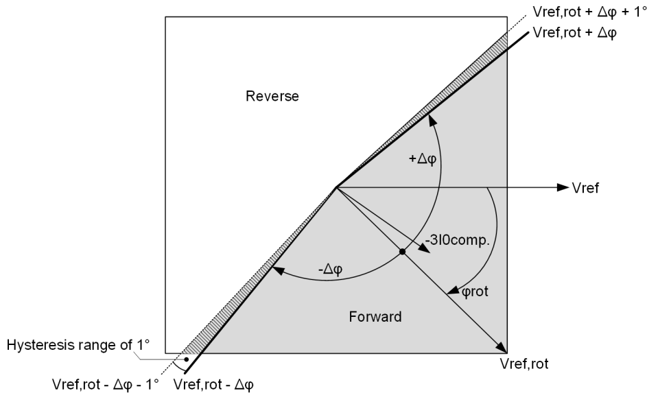
Figure 6-129 Directional Characteristic in Forward Mode
