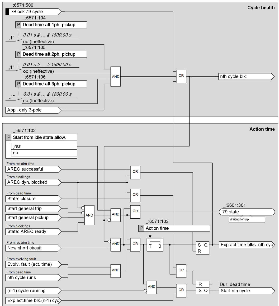
Figure 6-301 Cycle Control with Operating Mode: With Pickup/With Action Time
