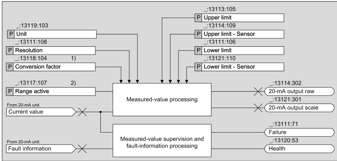
Figure 5-47 Logic Diagram of the Function 20-mA Channel
