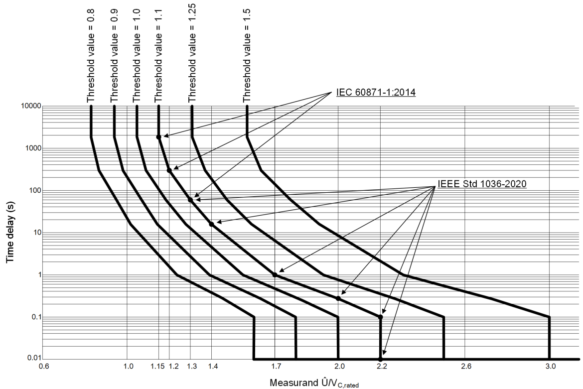
Figure 8-13 Inverse-Time Characteristic Curve
