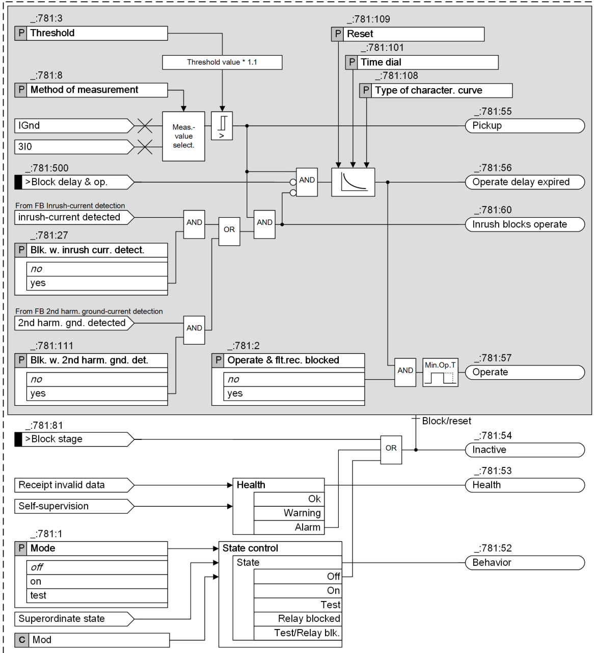
Figure 6-32 Logic Diagram Inverse-Time Overcurrent Protection (Ground) – Basic
