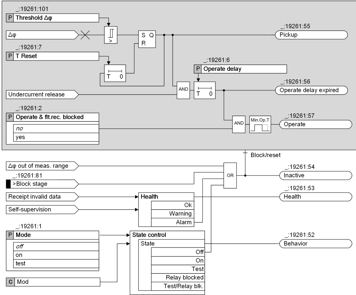
Figure 6-227 Logic Diagram of the Δφ Stage
