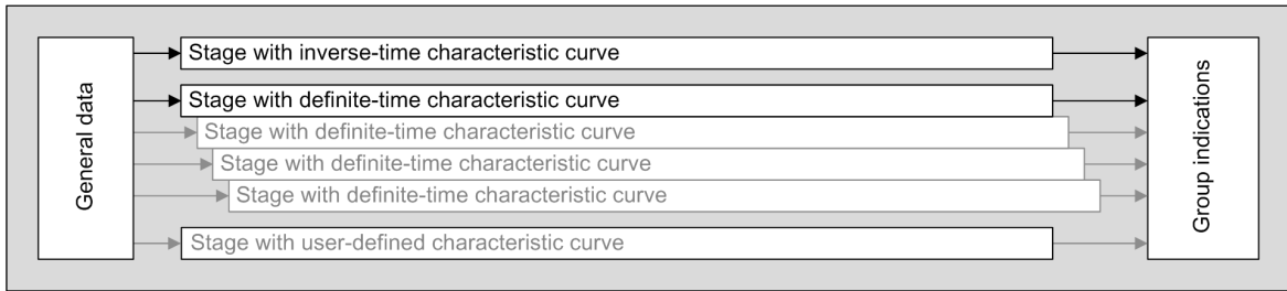
Figure 8-11 Structure/Embedding of the Function
