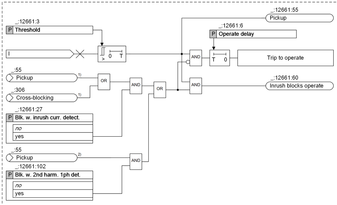
Figure 6-92 Part-Logic Diagram on the Influence of Inrush-Current Detection Exemplified by the 1st Definite-Time Overcurrent Protection Stage
