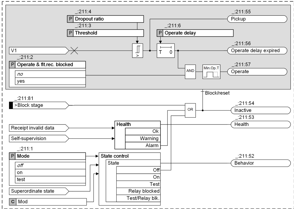
Figure 6-184 Logic Diagram of a Stage: Overvoltage Protection with Positive-Sequence Voltage
