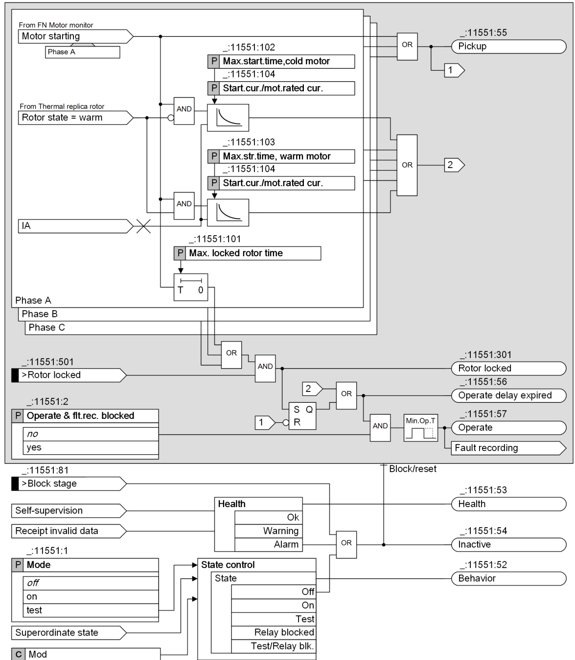
Figure 7-2 Logic Diagram of Motor-Starting Time Supervision with Inverse-Time Characteristic Curve
