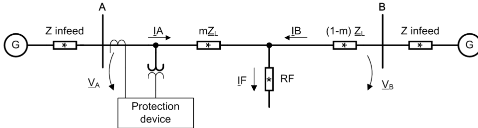
Figure 6-326 Fault Currents and Voltages of a Line Fed on Both Sides (1-Pole Display)
