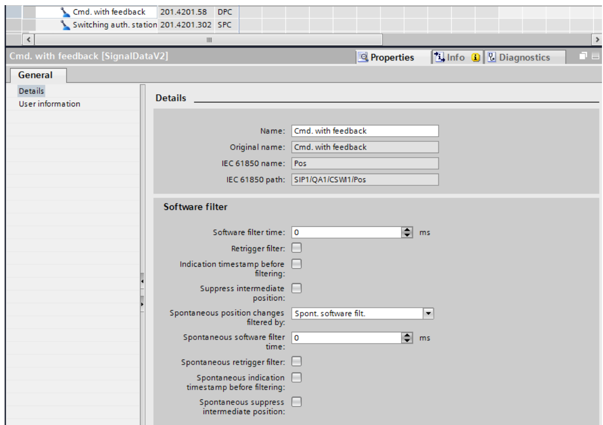
Figure 3-53 Settings for Circuit-Breaker Switch Position
