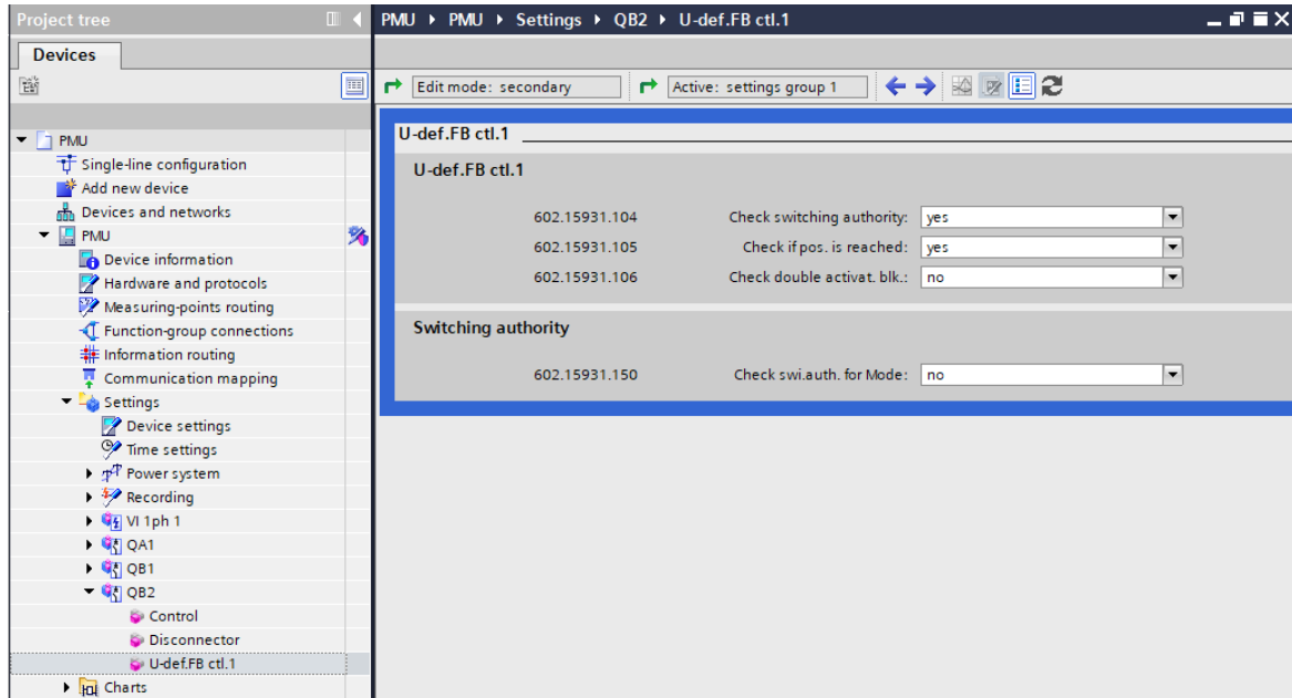
Figure 9-92 Parameterization Options of the User-Defined Function Block [Control]
