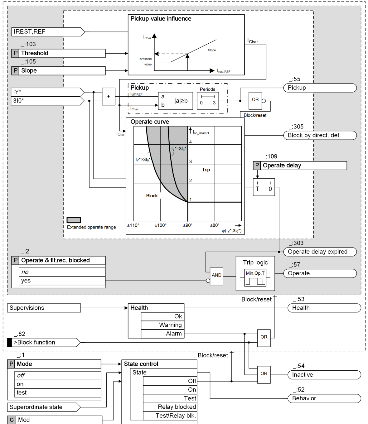
Figure 6-264 Logic Diagram of the Restricted Ground-Fault Protection Function
