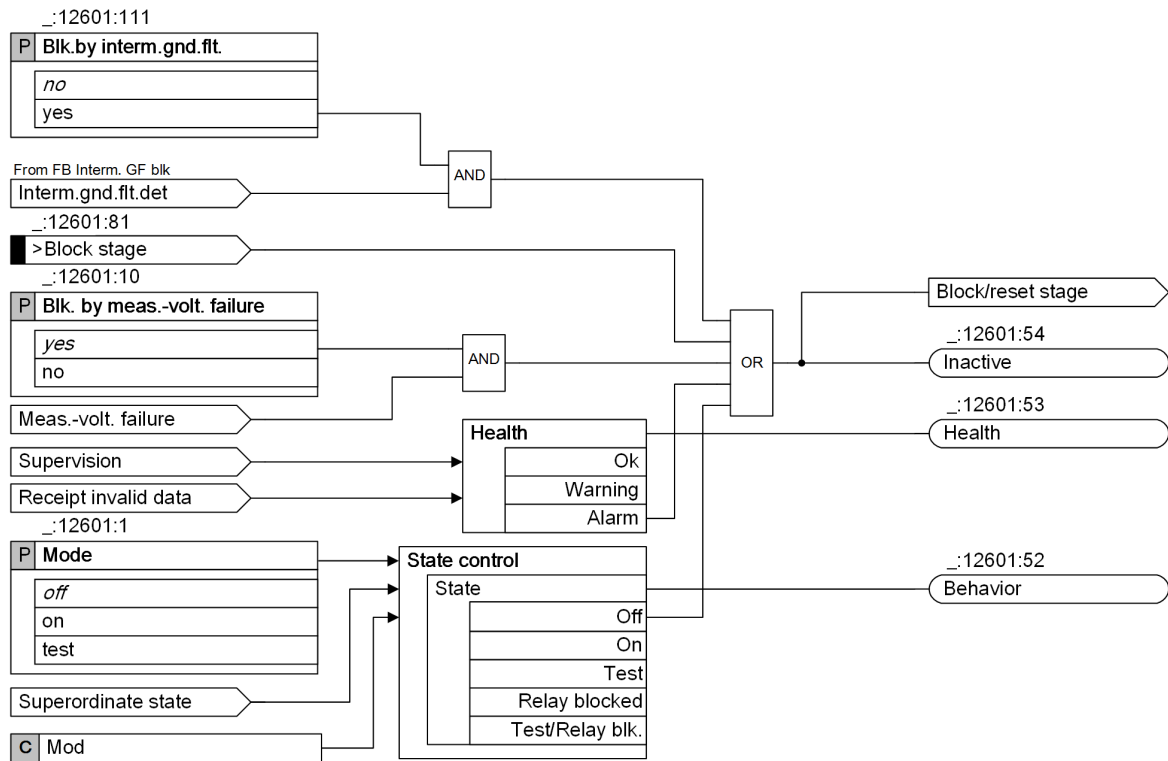
Figure 6-119 Logic Diagram of the Stage Control
