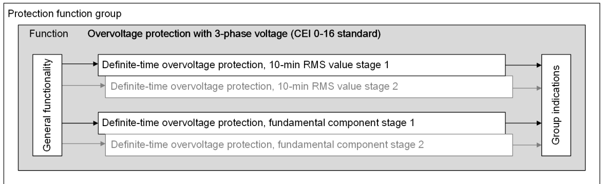
Figure 6-352 Structure/Embedding of the Function
