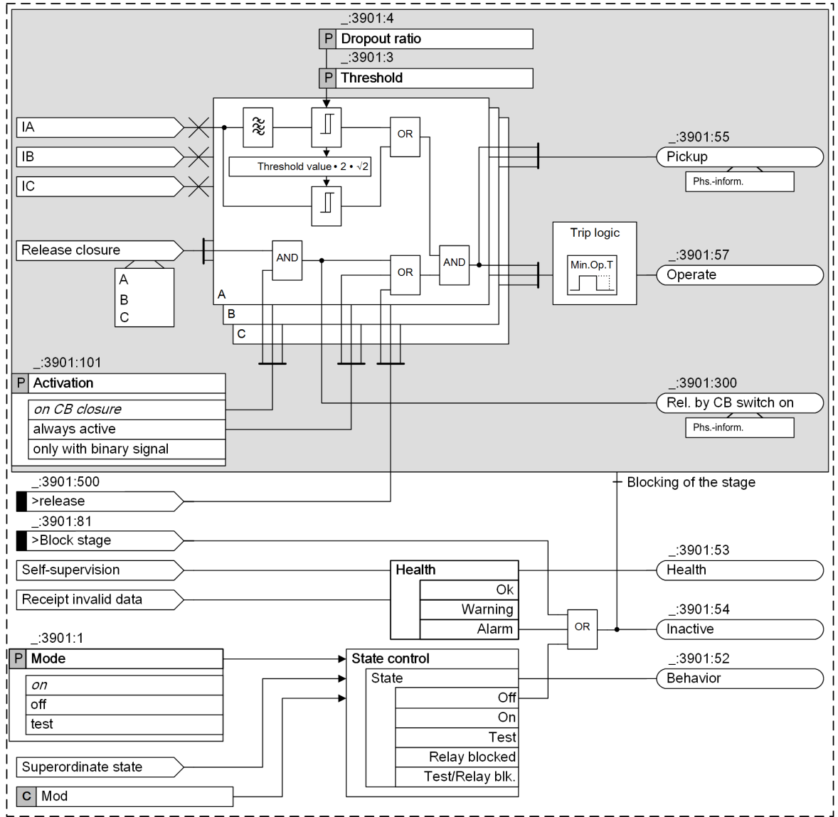
Figure 6-81 Logic Diagram of Instantaneous High-Current Tripping with Standard Release Method
