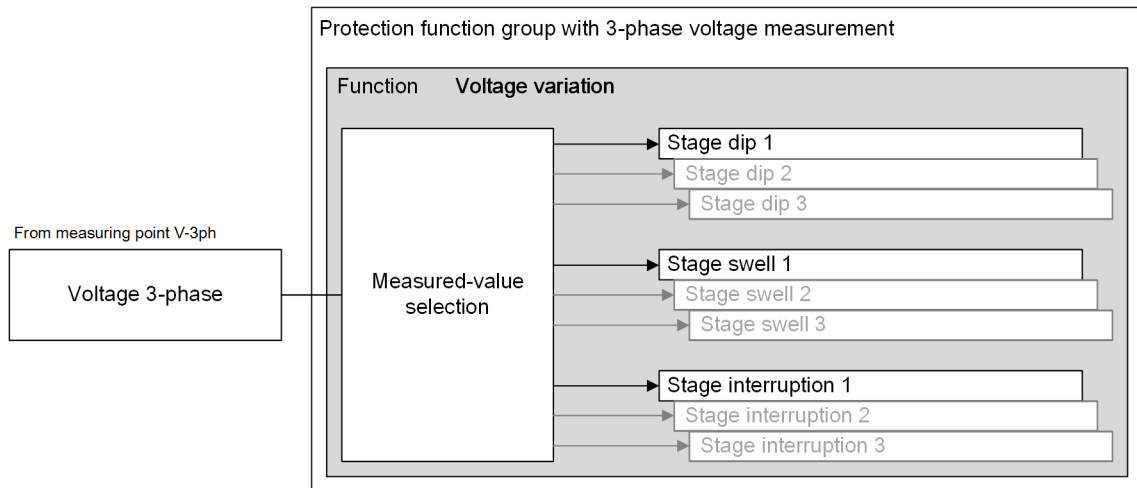
Figure 12-1 Structure/Embedding of the Function
