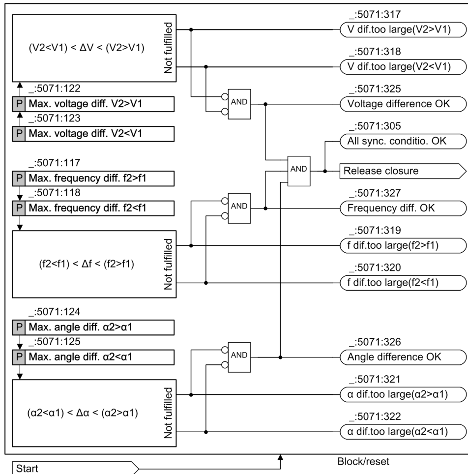
Figure 9-58 Closing Conditions for the Synchrocheck Function
