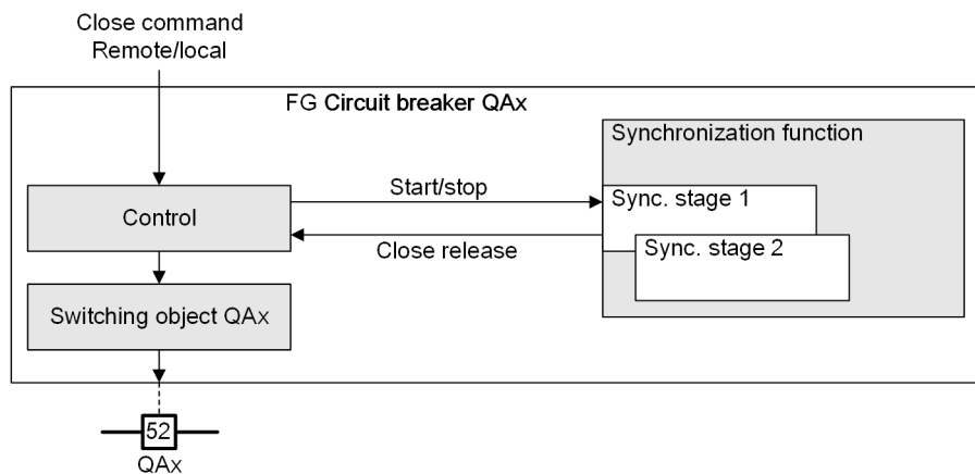
Figure 9-79 Interaction of the Control with the Synchronization Function
