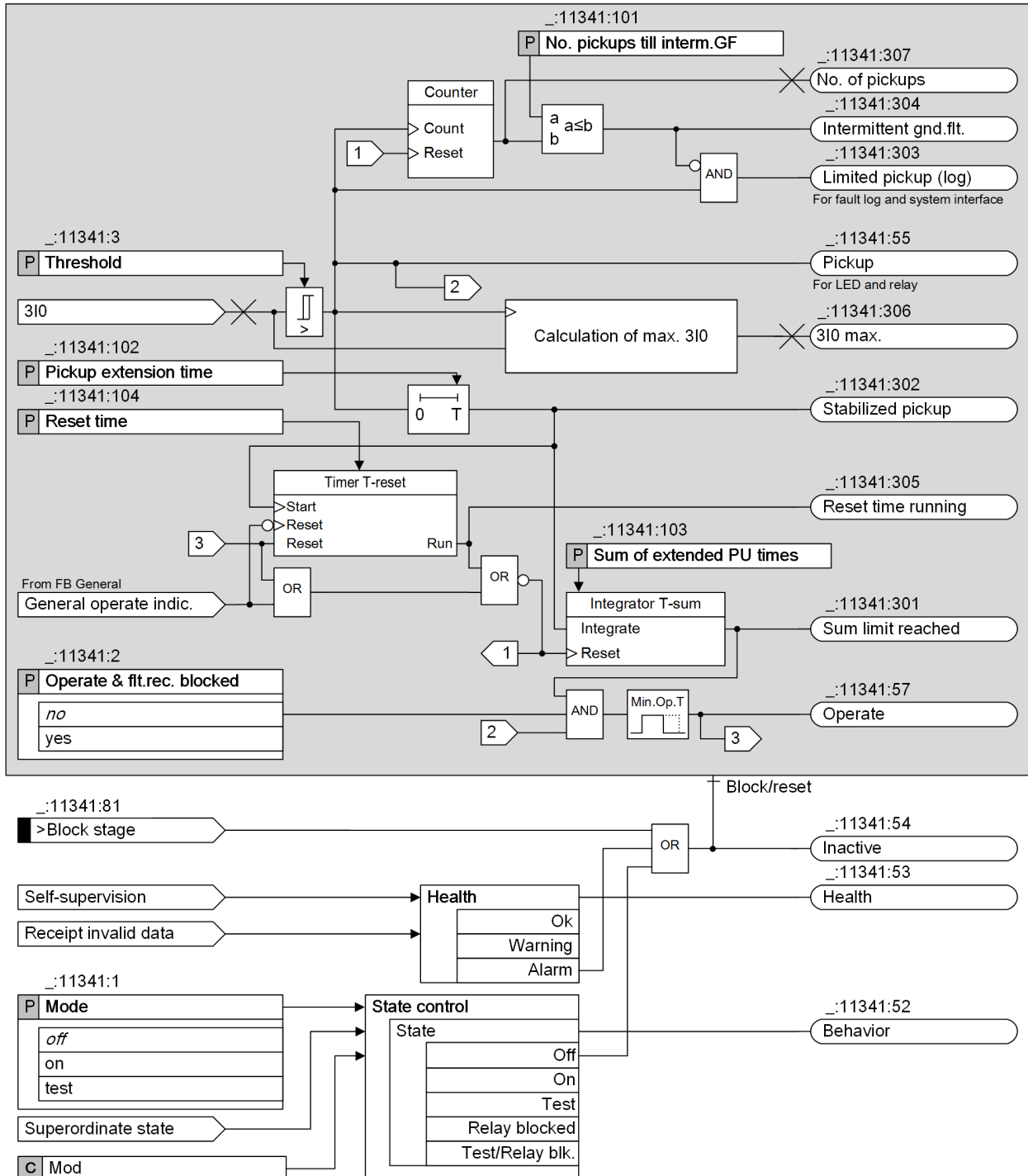
Figure 6-104 Logic of the Non-Directional Intermittent Ground-Fault Protection
