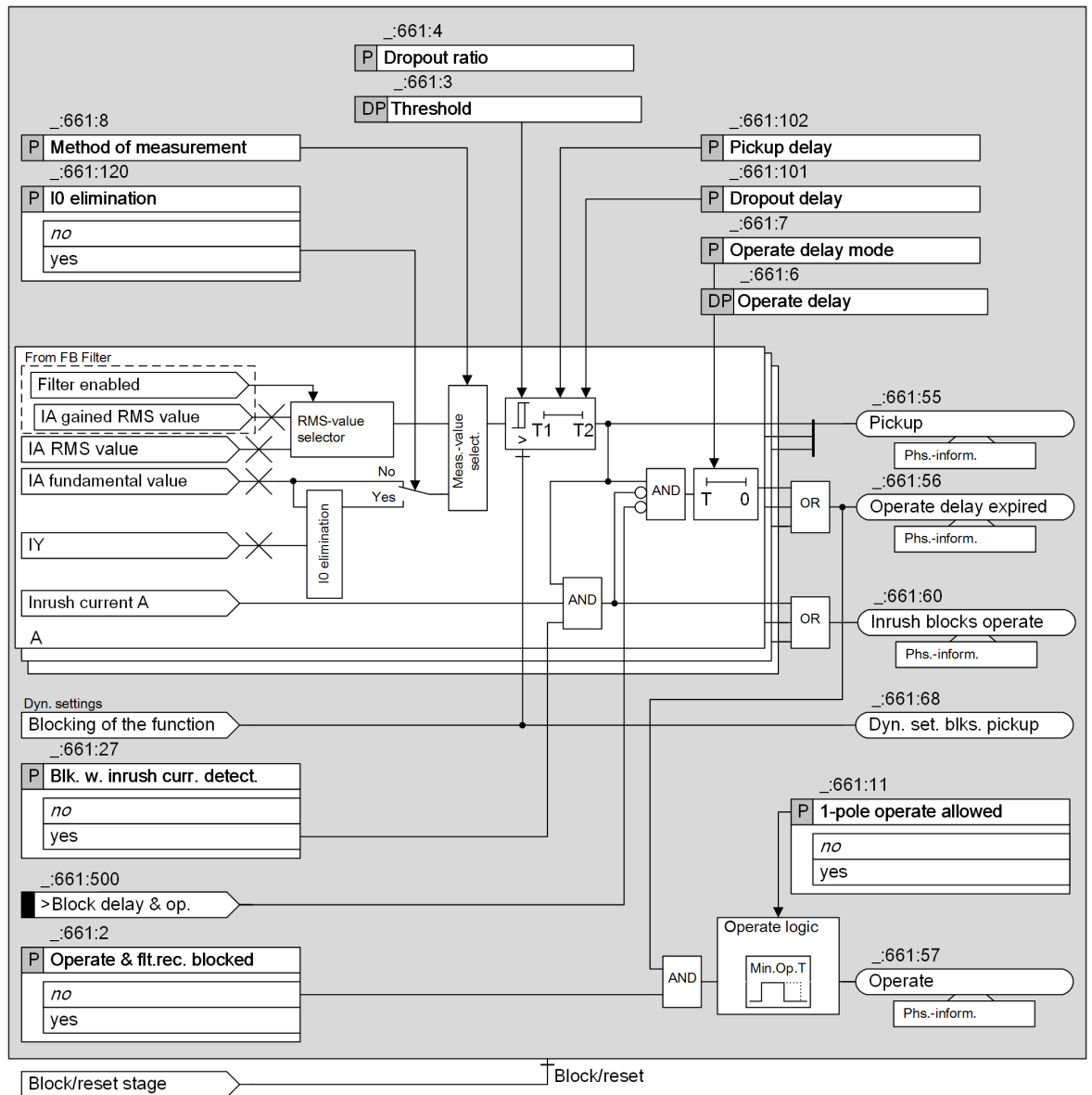
Figure 6-11 Logic Diagram of the Definite-Time Overcurrent Protection (Phases) – Advanced
