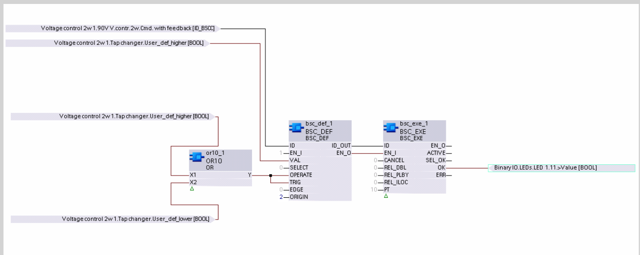
Figure 9-96 CFC Chart
