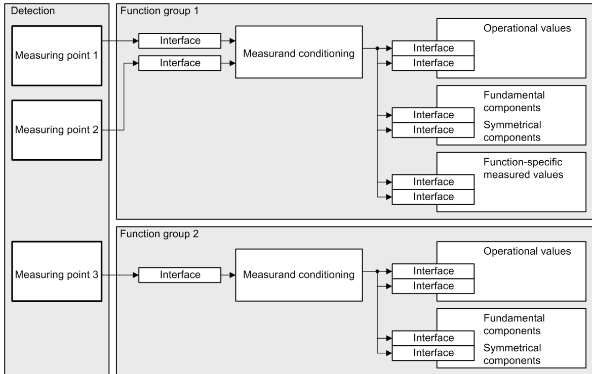
Figure 11-1 Structure of Measured-Value Acquisition and Processing
