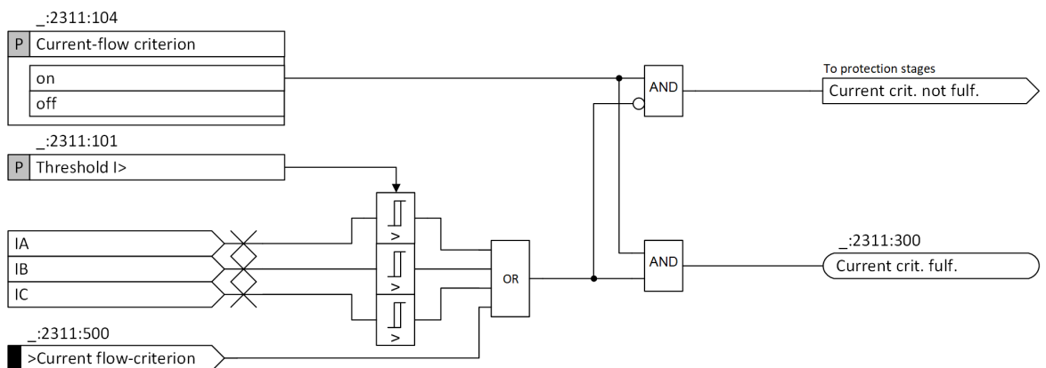
Figure 6-367 Logic Diagram of the General Functionality
