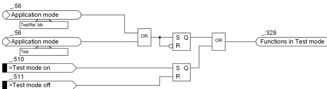
Figure 13-1 Logic Diagram: Enabling/Disabling the Test Mode for the Entire Device
