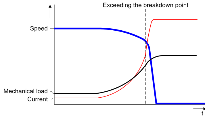
Figure 7-16 Example of the Time Characteristic Curve for Mechanical Rotor Locking
