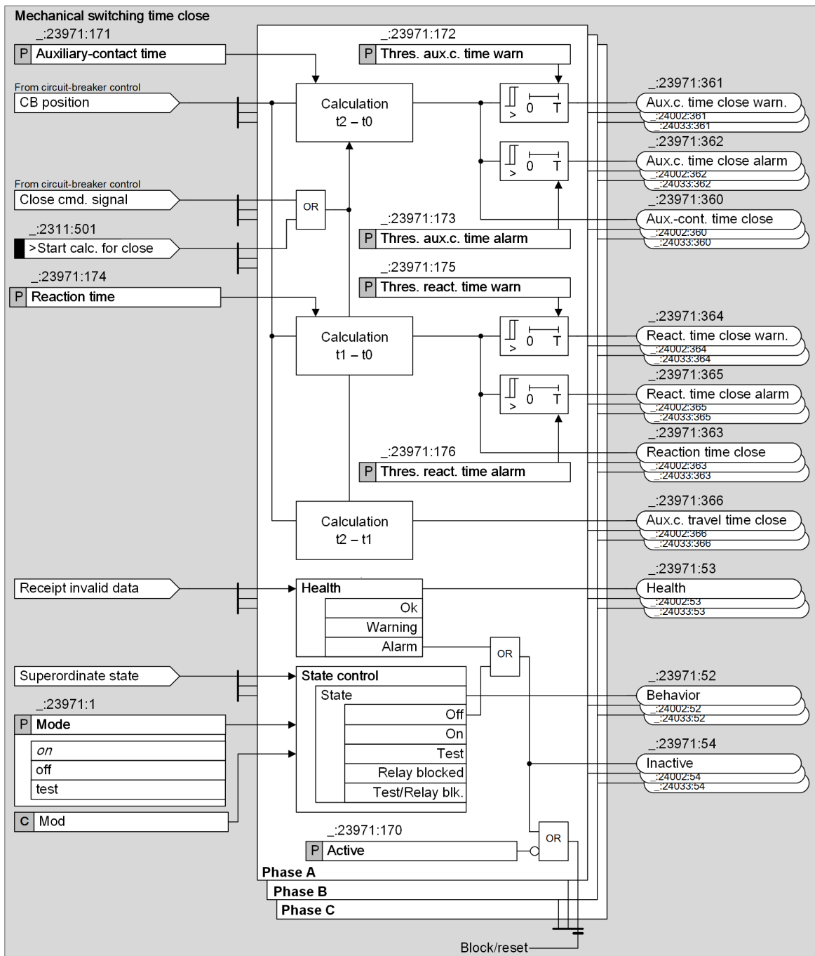
Figure 11-21 Logic of the Stage Mechanical Switching Time Close for Circuit Breakers 1-Pole
