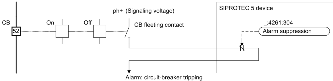
Figure 5-117 Circuit-Breaker Tripping Alarm Suppression
