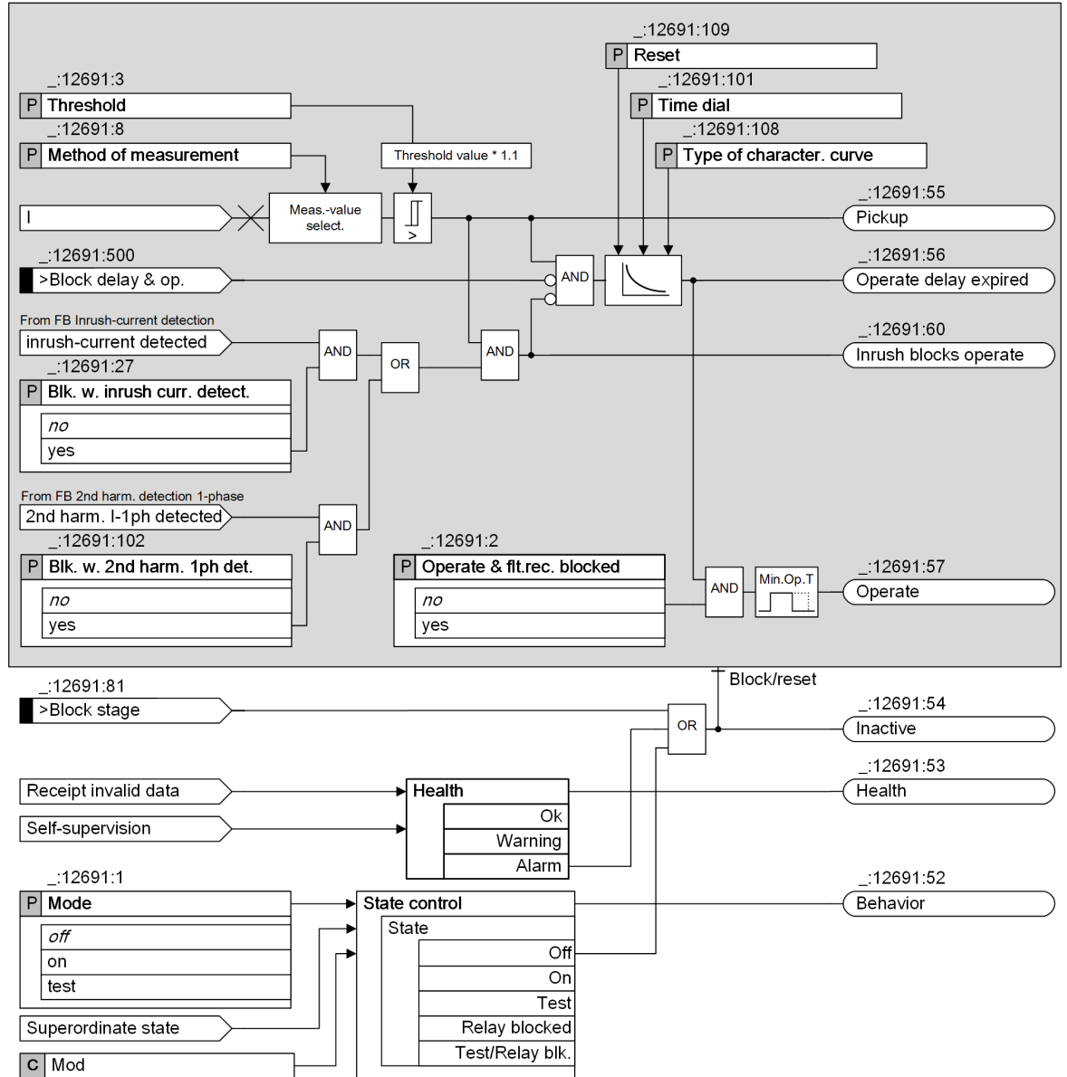
Figure 6-87 Logic Diagram of the Inverse-Time Overcurrent Protection (1-Phase)
