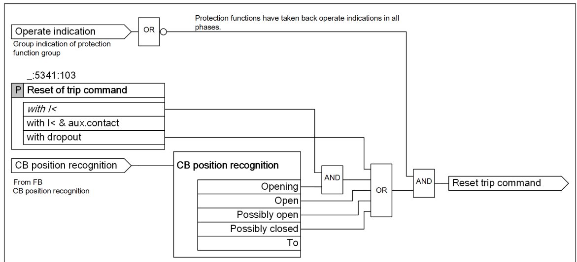
Figure 5-109 Trip-Command Reset
