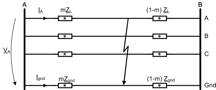
Figure 6-325 Short Circuit of a Phase-to-Ground Loop
