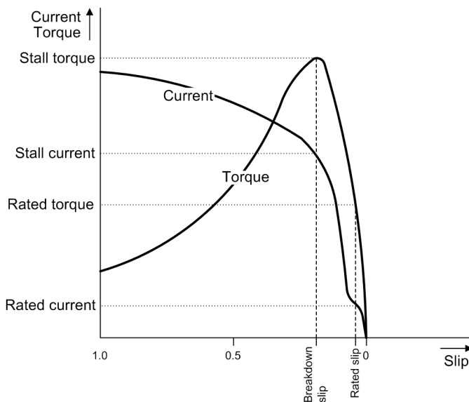
Figure 7-15 Typical Characteristic Curve of an Asynchronous Squirrel-Cage Motor
