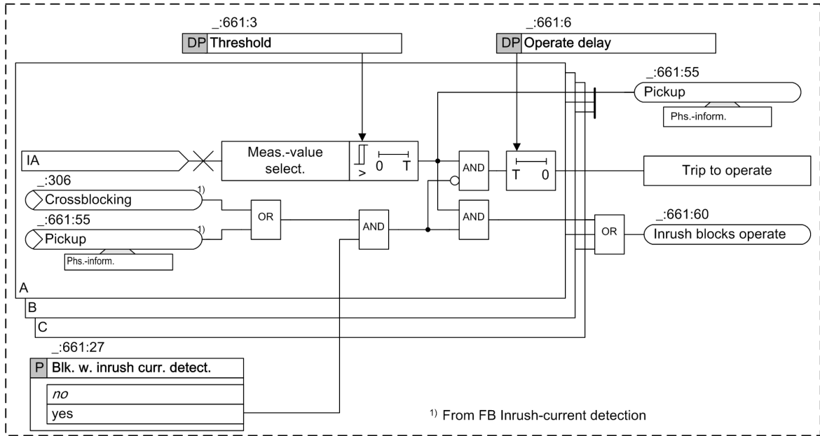
Figure 6-19 Part-Logic Diagram on the Influence of Inrush-Current Detection Exemplified by the 1st Definite-Time Overcurrent Protection Stage
