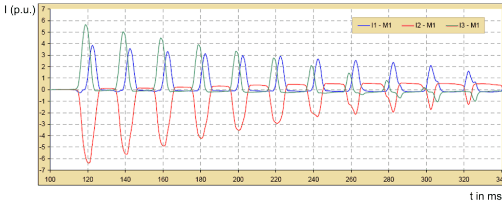
[dvw_inrush_03_1_en_US] Figure 6-73 Inrush-Current Characteristic
