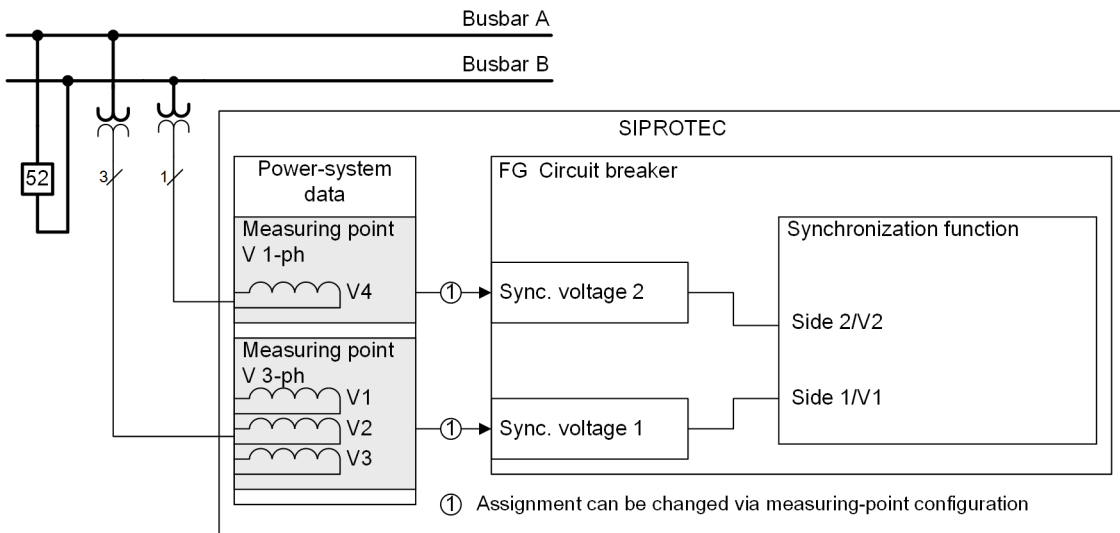
Figure 9-50 Synchronization of 2 Busbars via Cross-Coupling, Connection via 4 Voltage Inputs
