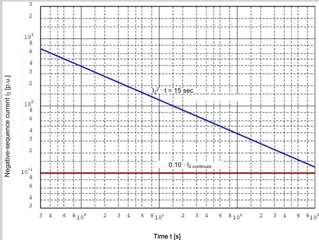
Figure 6-176 Example of an Unbalanced-Load Characteristic Specified by the Machine Manufacturer
