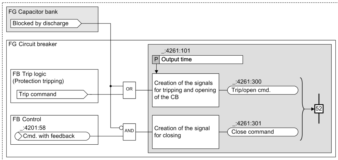
Figure 5-40 Logic Diagram of Processing the Blocked by Discharge Signal
