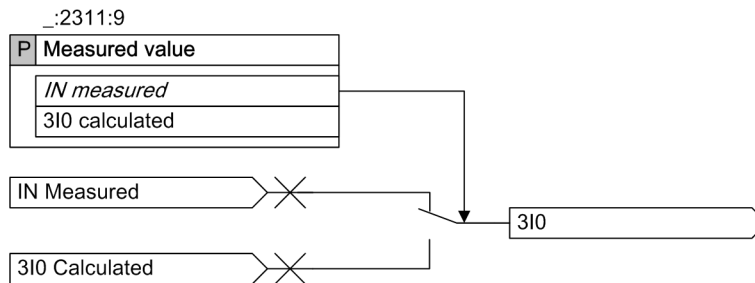
Figure 6-29 Logic Diagram of Measured-Value Selection
