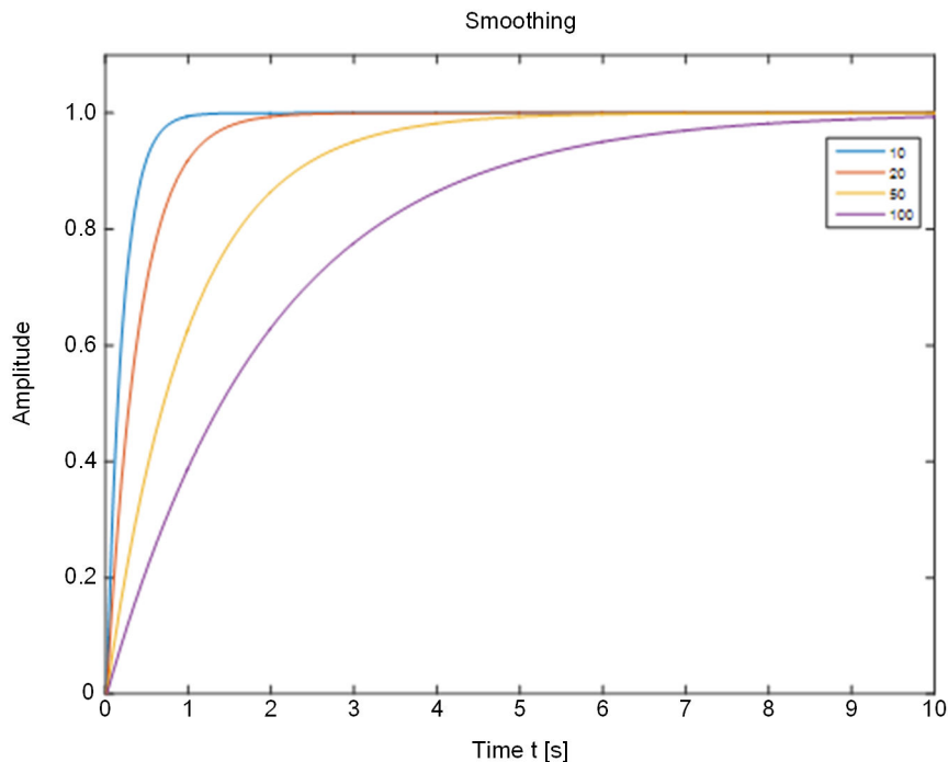
Figure 9-75 Effect of Smoothing Depending on the Set Parameter
