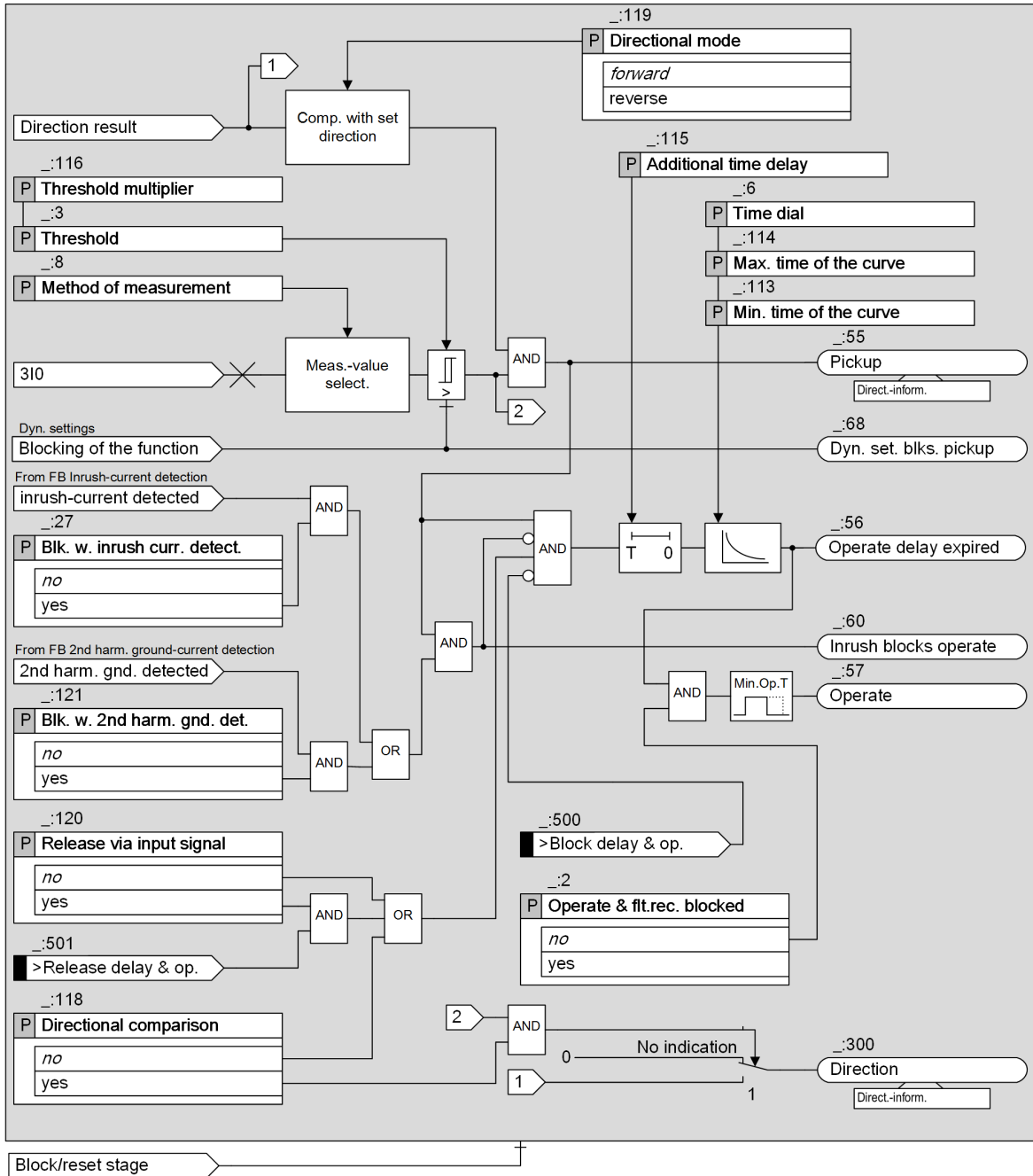
Figure 6-64 Logic Diagram of the Directional Logarithmic Inverse-Time Overcurrent Protection, Ground
