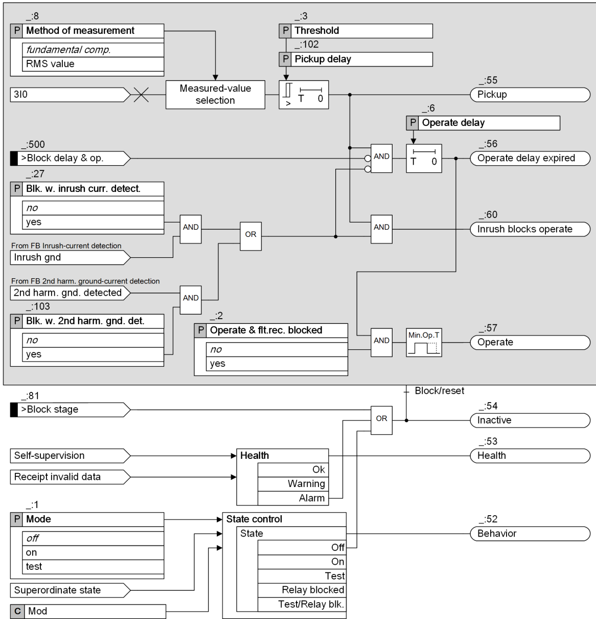
Figure 6-139 Logic Diagram of the Non-Directional 3I0 Stage
