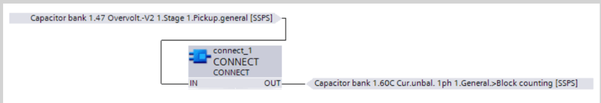
Figure 8-5 CFC for Blocking the Counting
