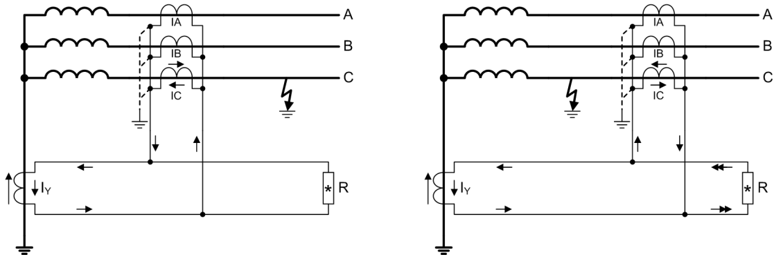
Figure 6-94 Principle of the Restricted Ground-Fault Protection According to the High-Impedance Principle
