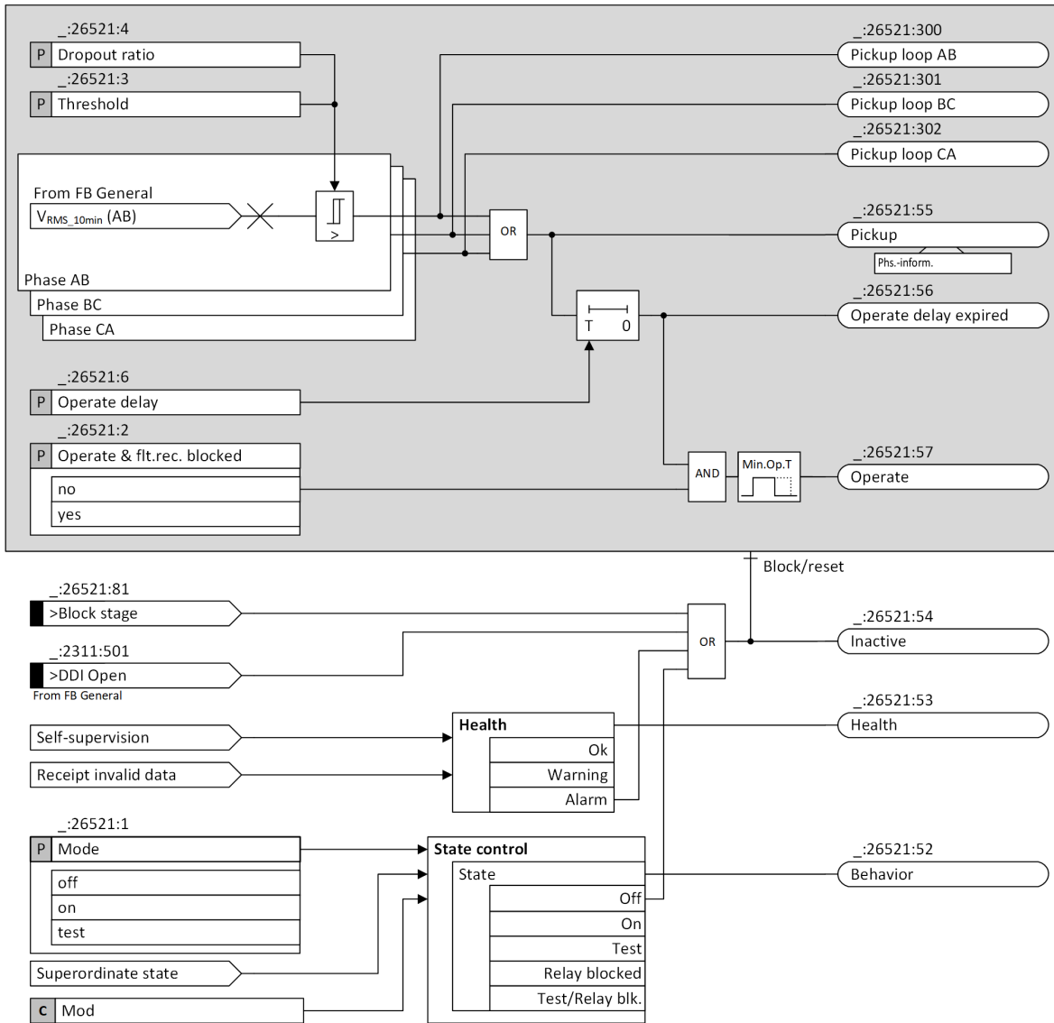
Figure 6-354 Logic Diagram of the Stage with Definite-Time Characteristic Curve, 10-Min RMS Value
