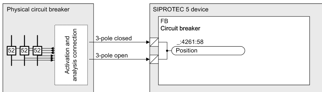
Figure 5-131 Recommended Analysis of the Circuit-Breaker Switch Position
