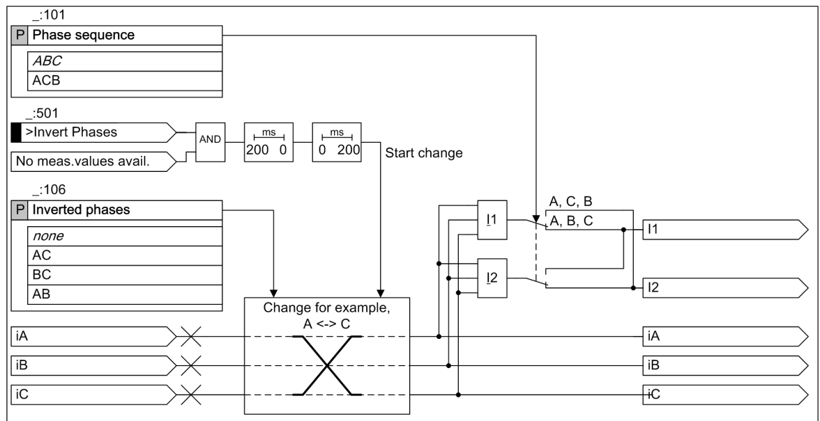
Figure 6-344 Measured Values for Changed-Over Phases
