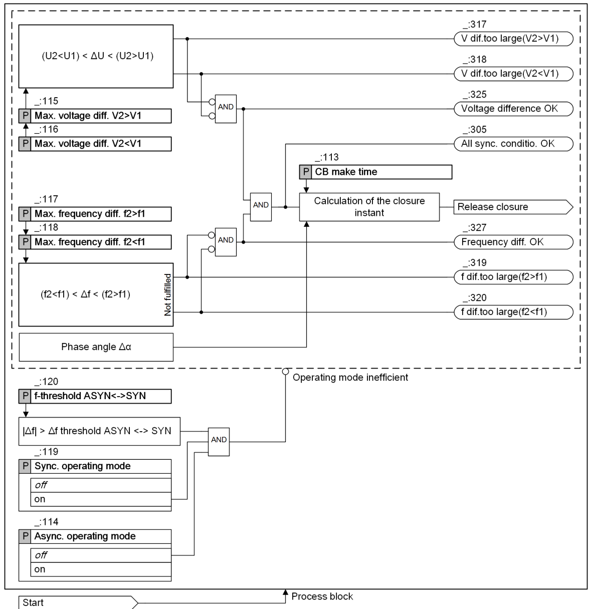
Figure 9-65 Closing Conditions when Switching Asynchronous Systems
