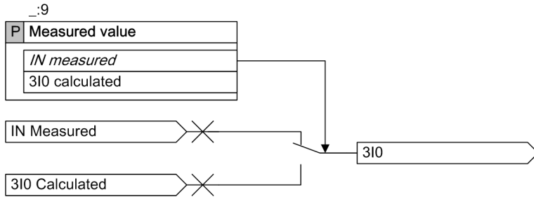
Figure 6-53 Logic Diagram of Measured-Value Selection
