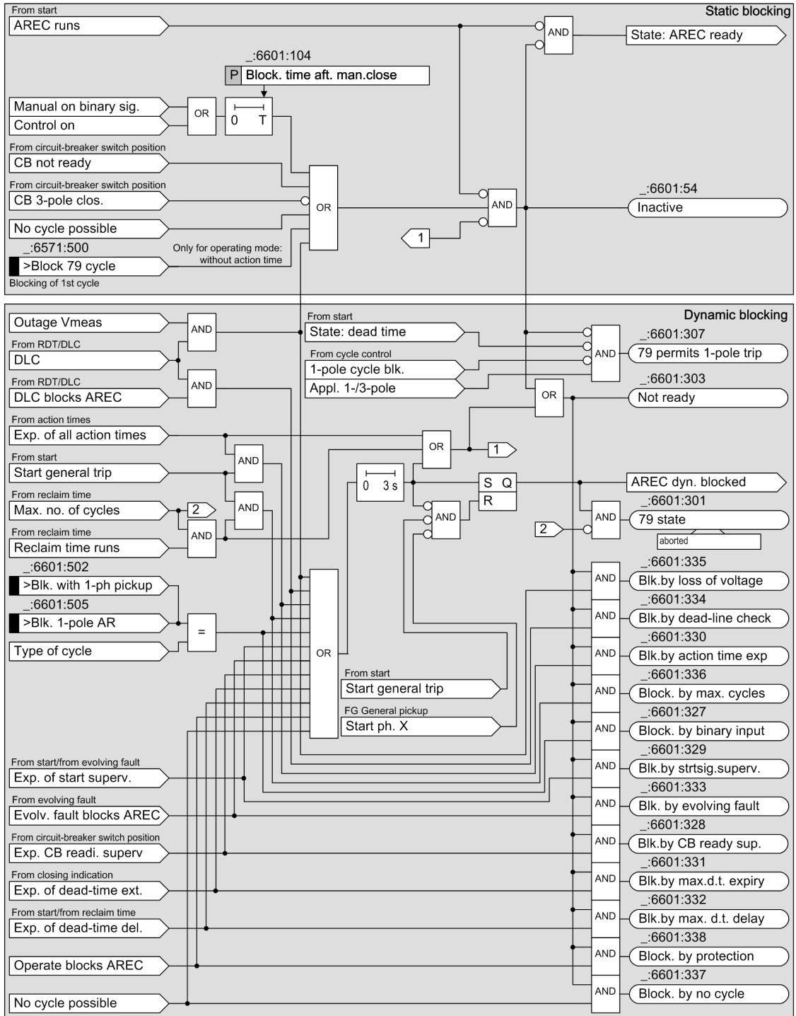
Figure 6-316 Cyclic Automatic Reclosing: Blocking Logic in the Example for a 1-Pole Cycle (Static and Dynamic Blocking)
