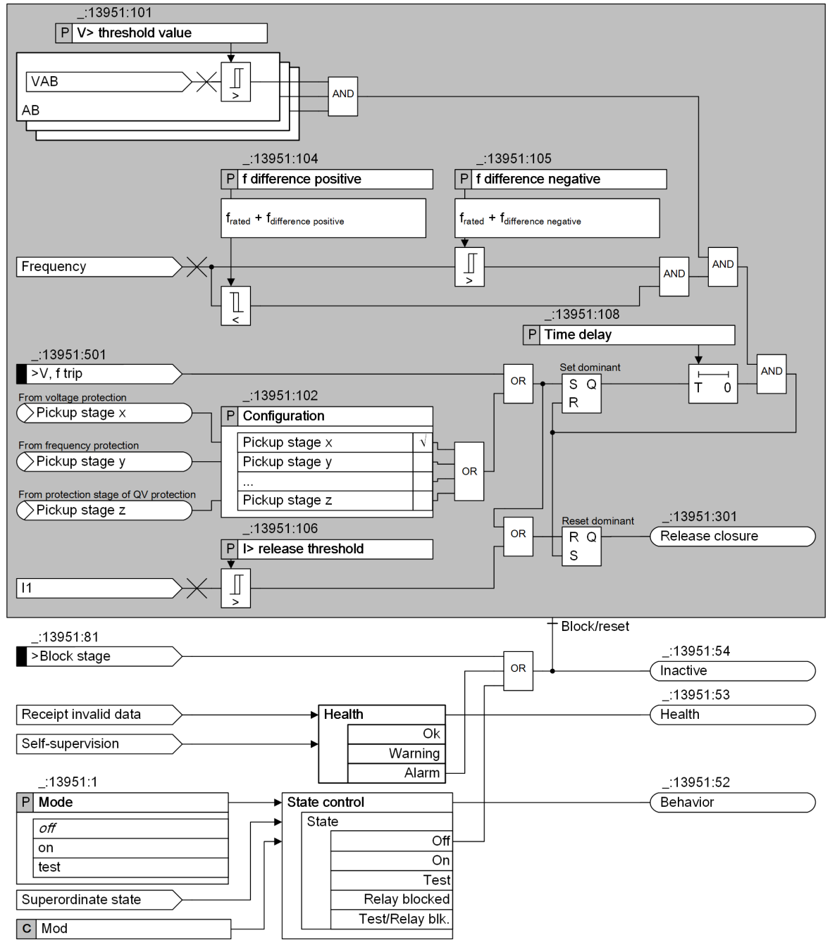
Figure 6-246 Logic Diagram of Reclosure Stage in Undervoltage-Controlled Reactive-Power Protection
