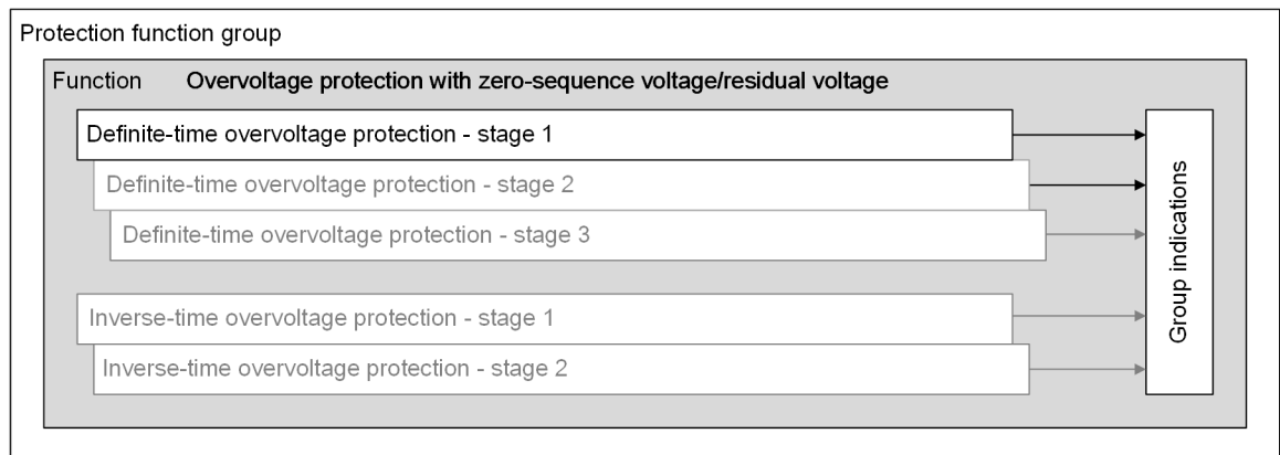
Figure 6-181 Structure/Embedding of the Function
