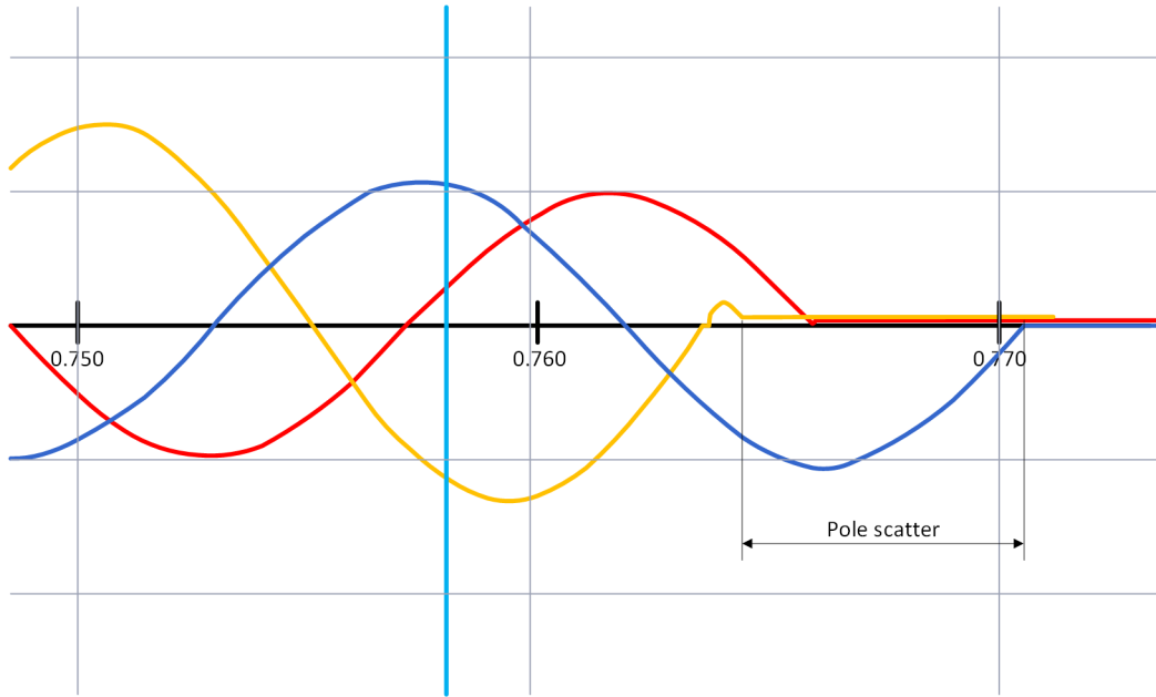
Figure 11-17 Pole Scatter Time
