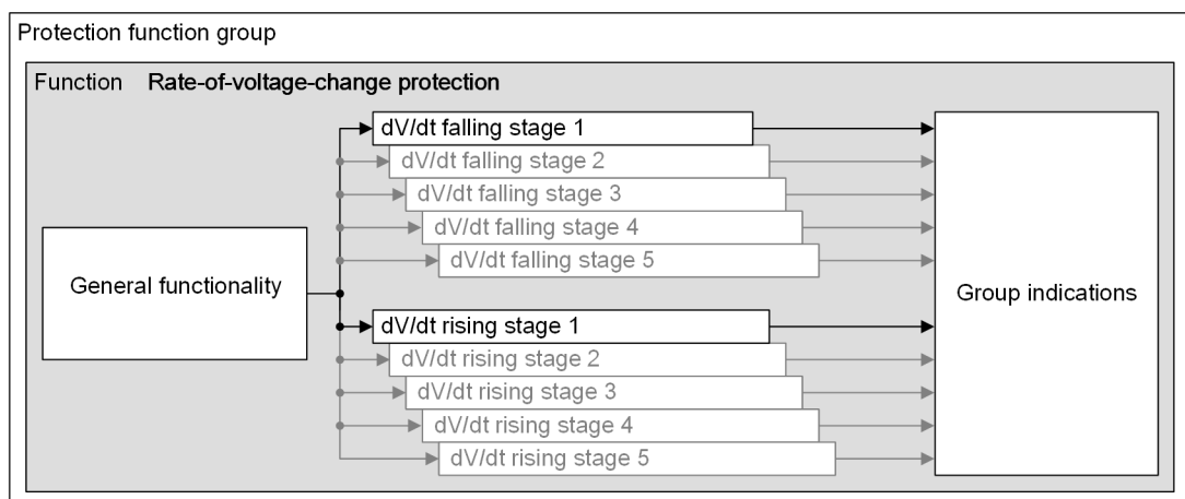
Figure 6-207 Structure/Embedding of the Function
