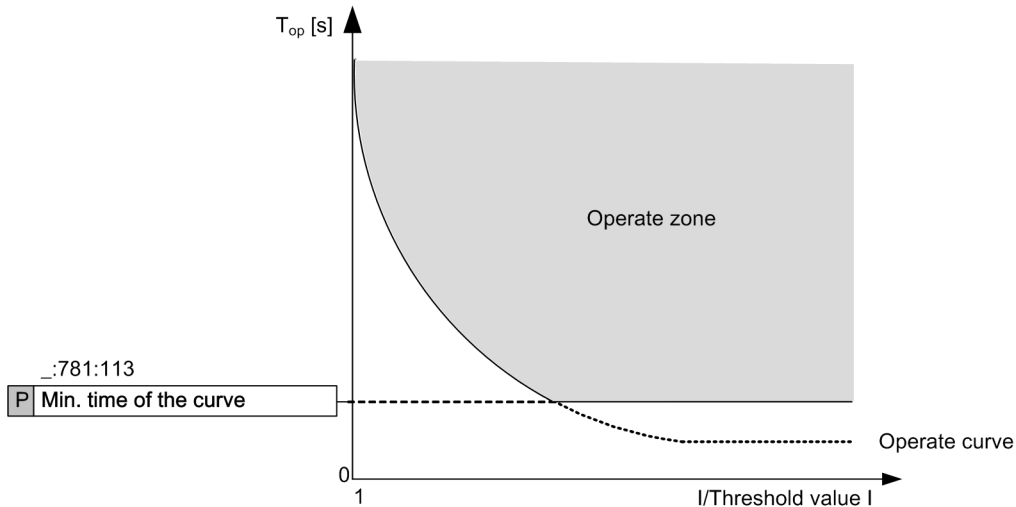
[dw_ocp_gr3_mi_1_en_US] Figure 6-34 Minimum Operating Time of the Curve
