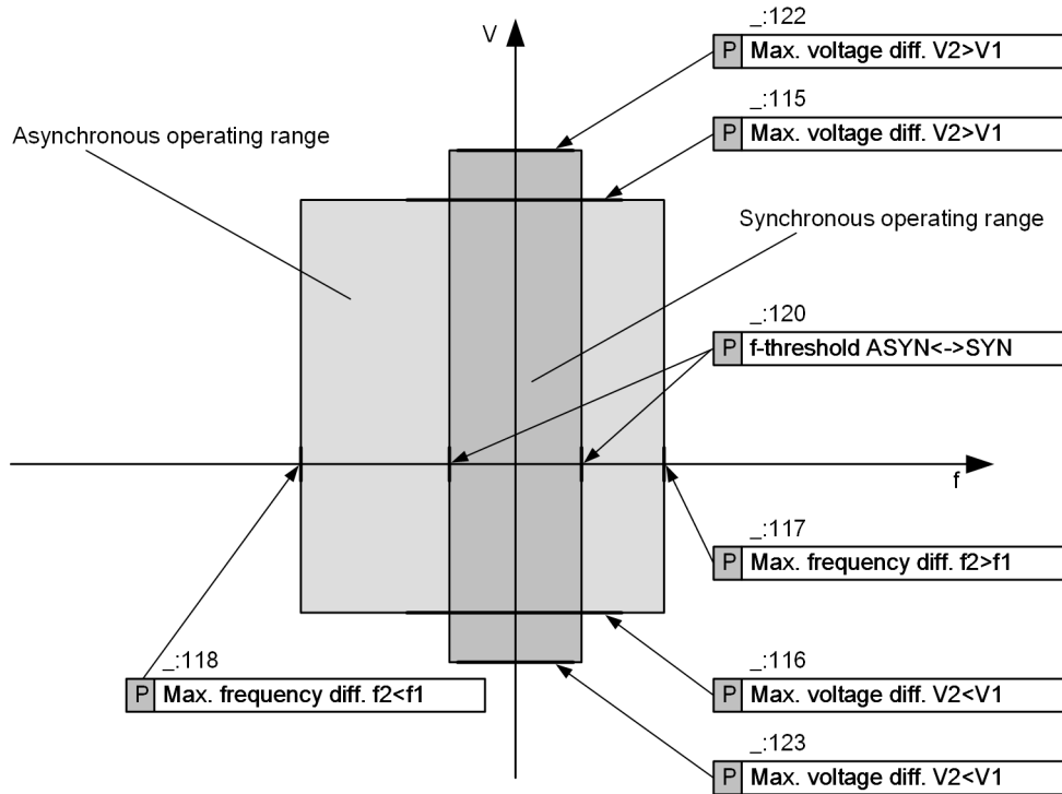
Figure 9-66 Operating Range under Synchronous and Asynchronous Conditions for Voltage (V) and Frequency (f)
