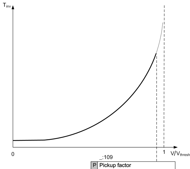
Figure 6-202 Inverse-Time Characteristics for Undervoltage Protection
