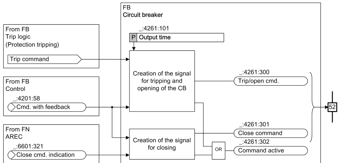
Figure 5-110 Tripping, Opening, and Closing the Circuit Breaker
