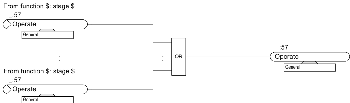
Figure 5-42 Generation of the Operate Indication of the Capacitor Bank Function Group
