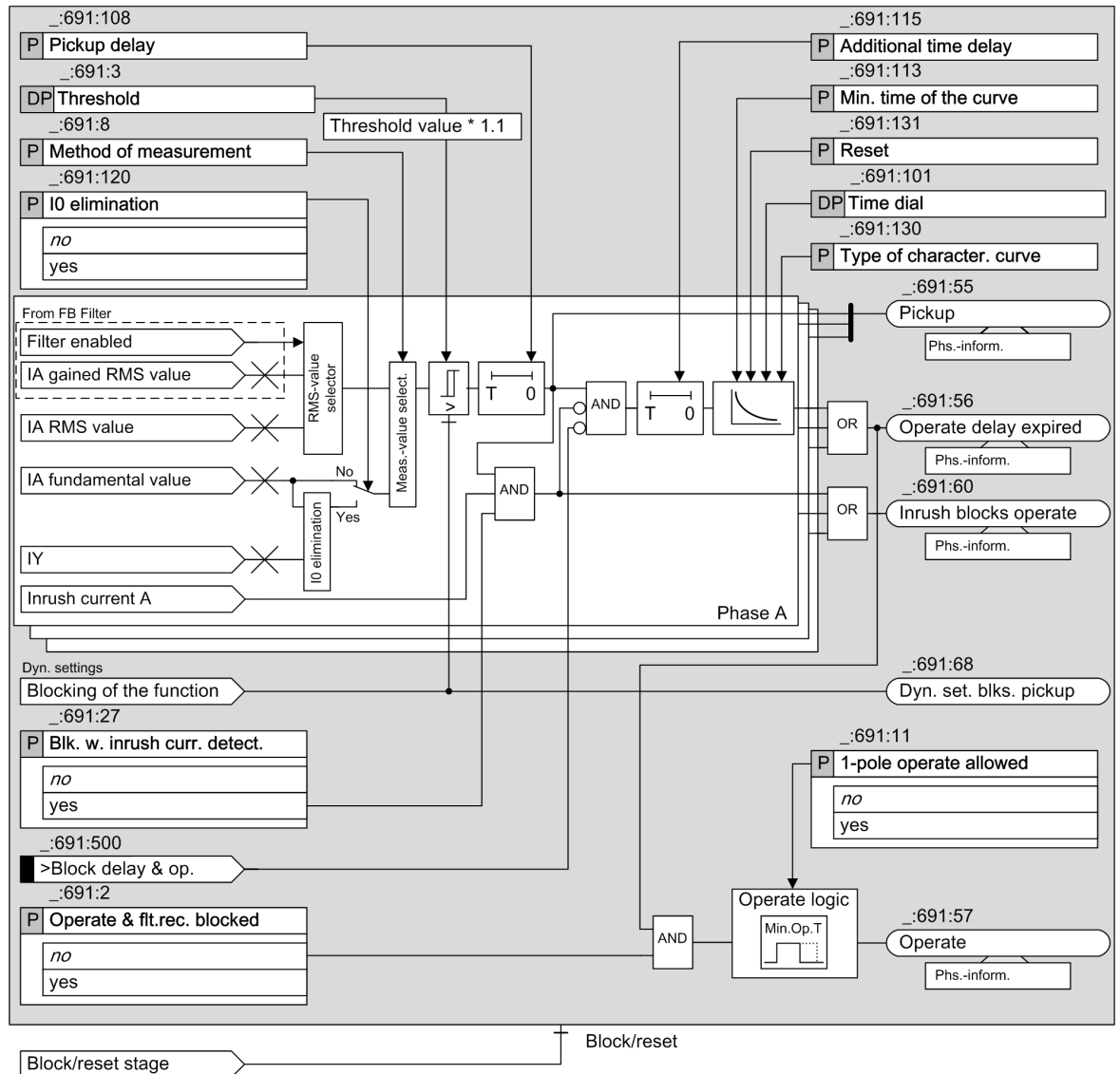
Figure 6-15 Logic Diagram Inverse-Time Overcurrent Protection (Phases) – Advanced
