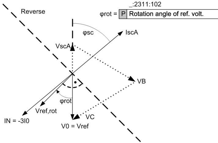
[ldw_r0reze, 2, en_US] Figure 6-56 Rotation of the Reference Voltage, Directional Overcurrent Protection, Ground Function with Zero-Sequence Values
