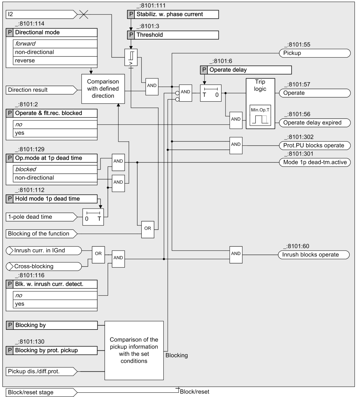
Figure 6-155 Logic Diagram of the Function Directional Negative-Sequence System Protection with Current-Independent Time Delay
