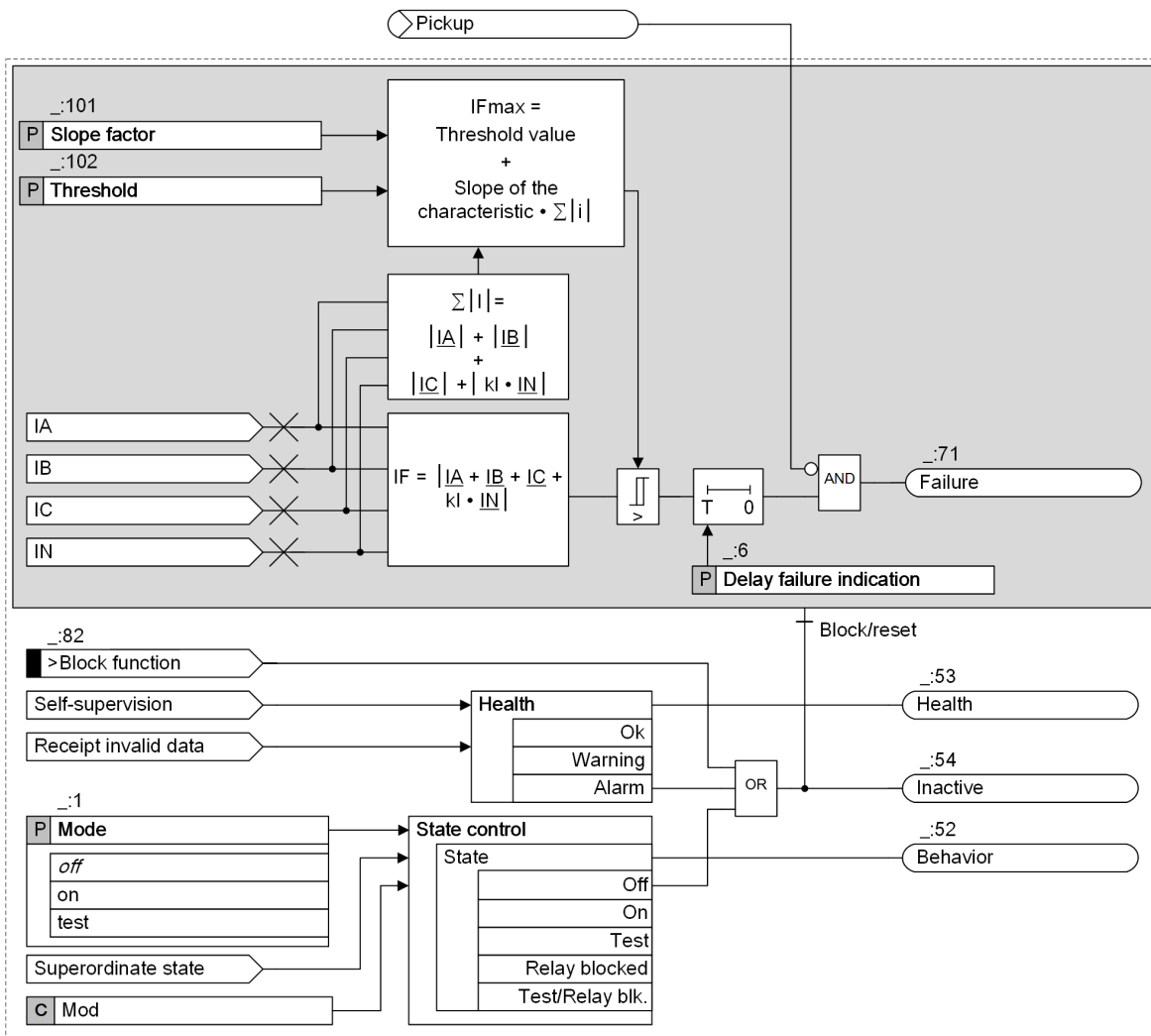
Figure 10-33 Logic Diagram of the Current-Sum Supervision
