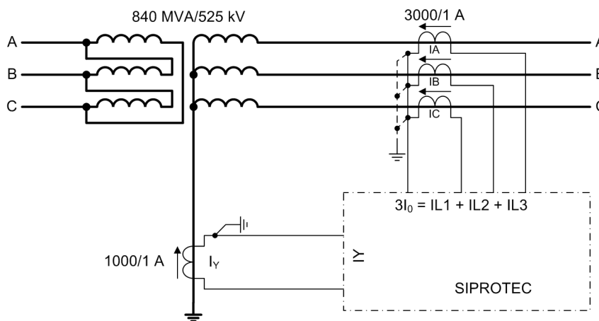
Figure 6-270 Application Star Side
