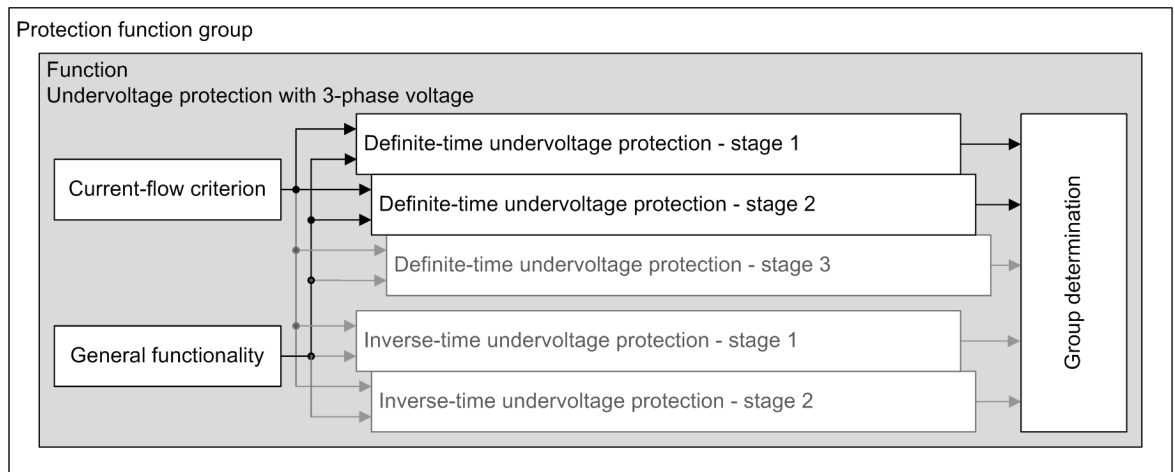
Figure 6-197 Structure/Embedding of the Function
