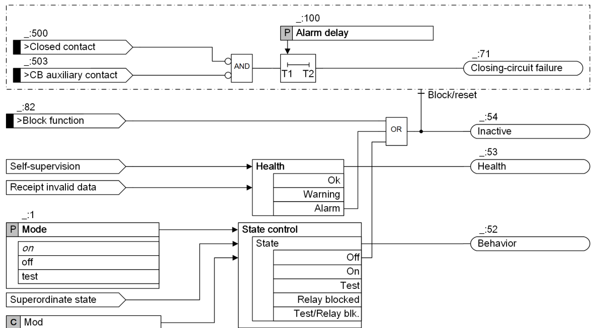
Figure 10-46 Logic Diagram of the Stage Closing-Circuit Supervision with 2 Binary Inputs
