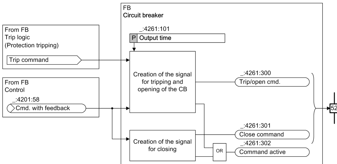
Figure 5-125 Tripping, Opening, and Closing the Circuit Breaker
