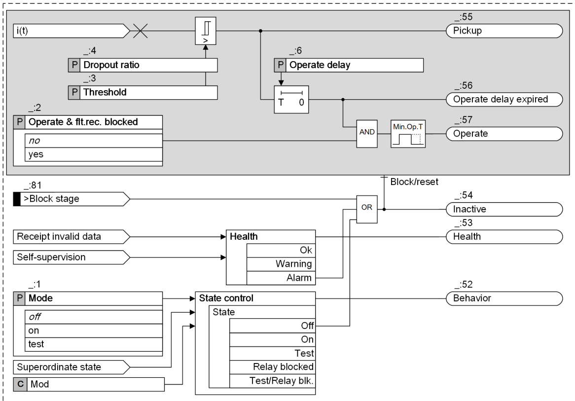
Figure 6-91 Logic Diagram of the Fast Stage, 1-Phase
