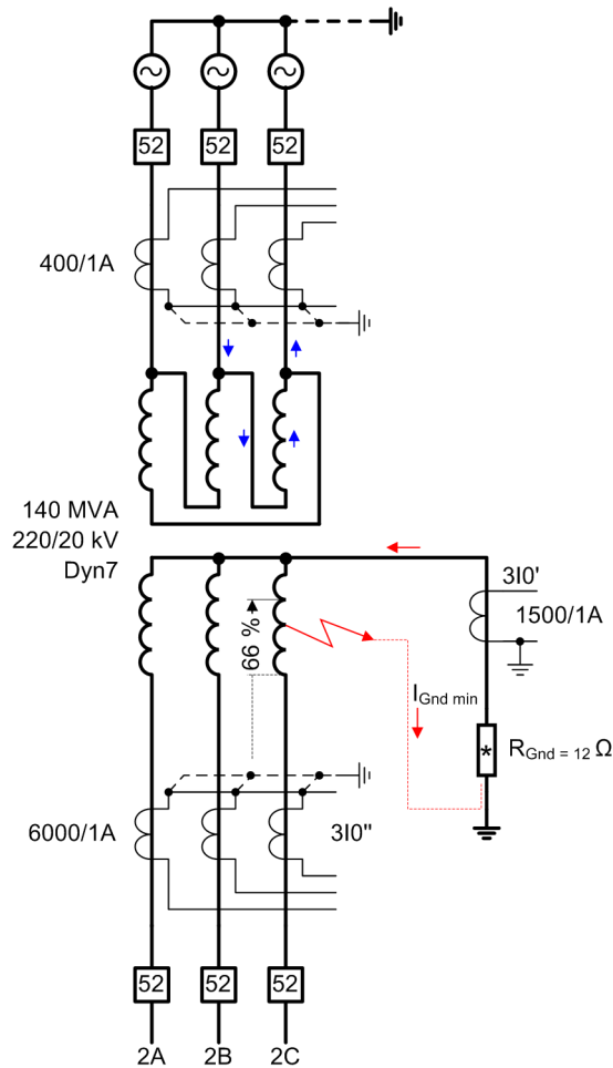
Figure 6-278 Application with Resistance-Grounded Neutral Point
