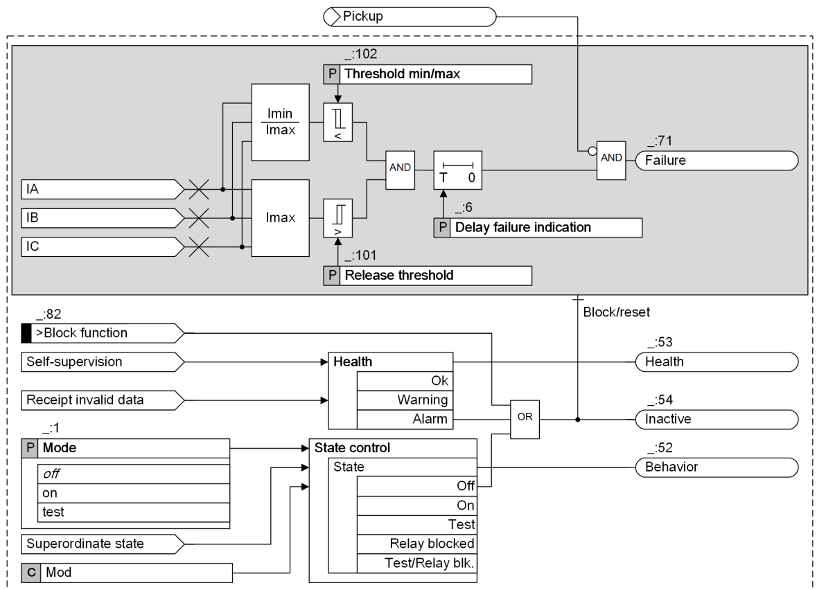
Figure 10-30 Logic Diagram of the Current-Balance Supervision
