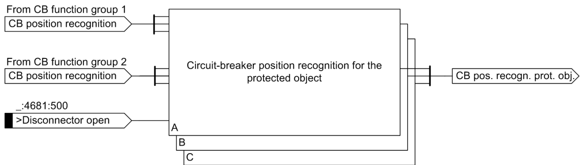
Figure 5-22 Logic Diagram of the Circuit-Breaker Condition for the Protected-Object Function Block
