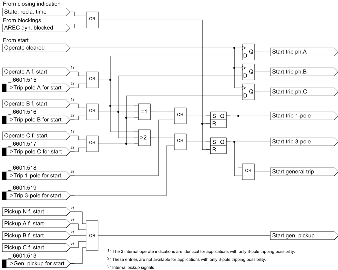
Figure 6-297 Input Logic for Operating Modes: With Tripping
