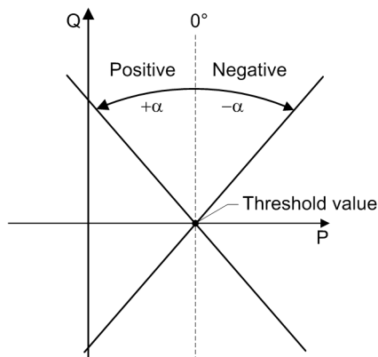
Figure 6-232 Tilt-Power Characteristic
