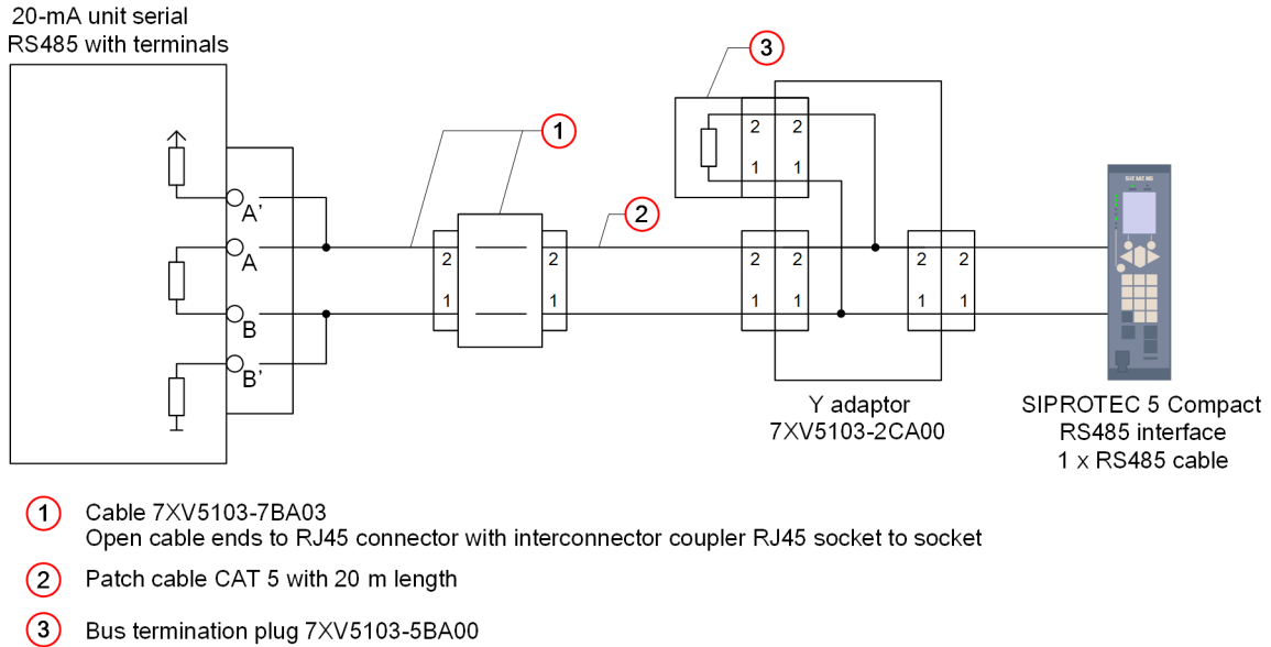
Figure 5-52 Connection of the 20-mA Unit to the SIPROTEC 5 Compact Device
