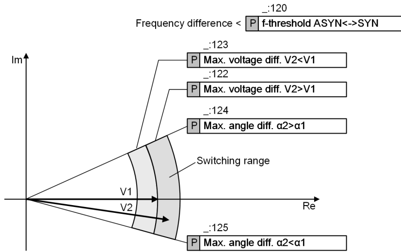
Figure 9-64 Connecting Under Synchronous System Conditions
