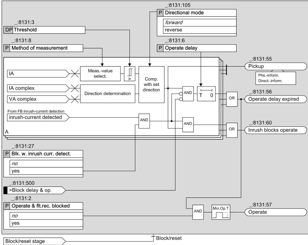
Figure 6-40 Logic Diagram of the Directional, Definite-Time Overcurrent Protection, Phases - Basic
