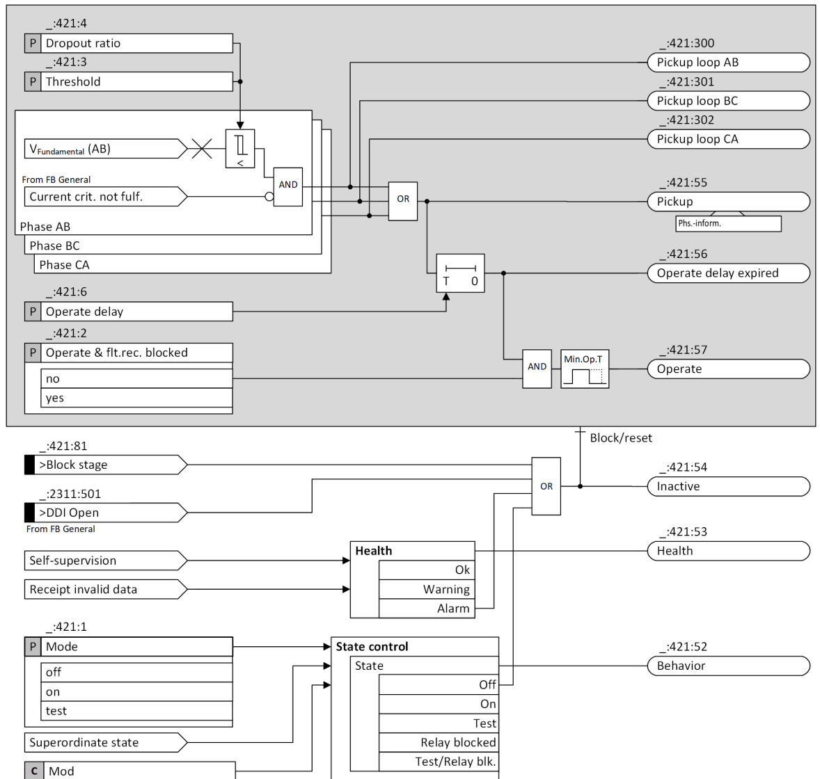
Figure 6-368 Logic Diagram of the Stage with Definite-Time Characteristic Curve, Fundamental Component
