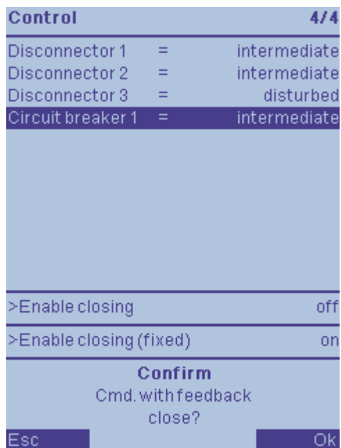
Figure 9-34 The Status of Interlocking Conditions is Visible in the Control Menu
