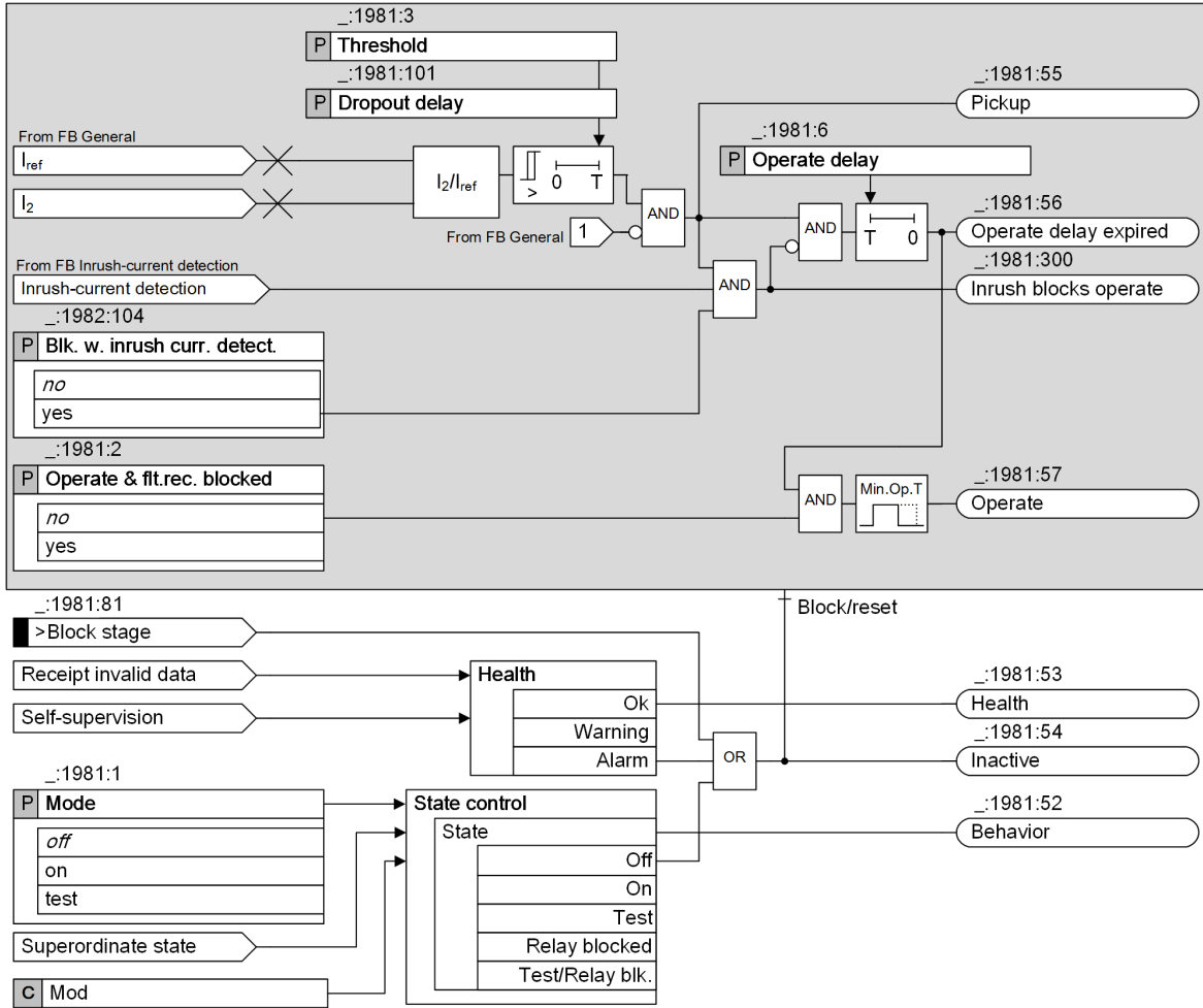
Figure 6-151 Logic Diagram of the Stage Negative-Sequence Protection with Definite-Time Characteristic Curve
