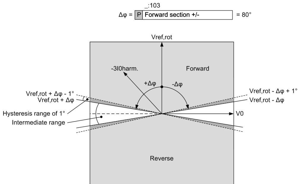
Figure 6-137 Direction Characteristic
