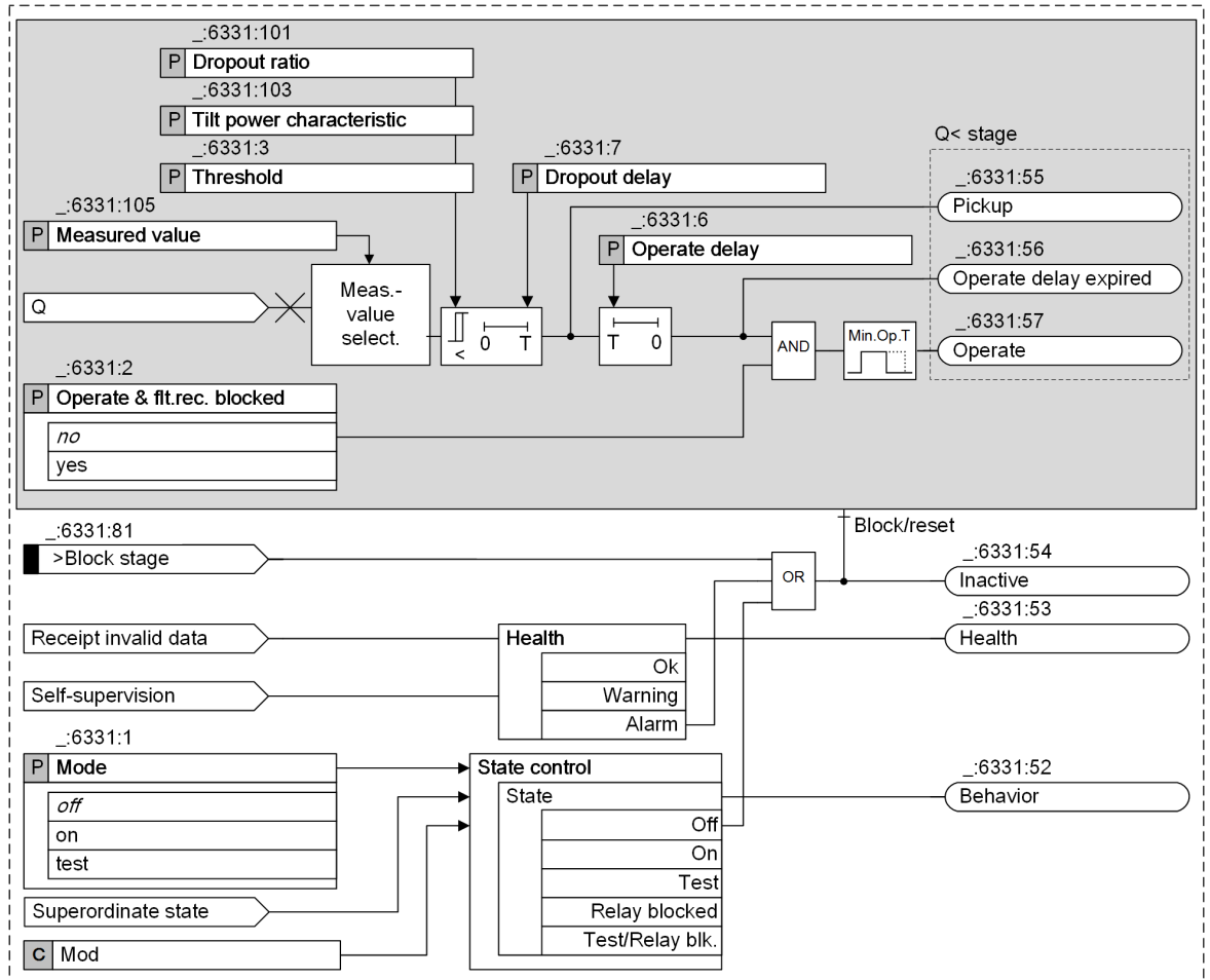
Figure 6-233 Logic Diagram of the Reactive Power Stage (Stage Type: Power Q<)
