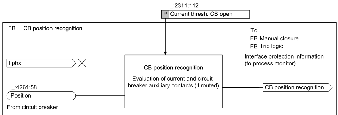
Figure 5-118 Overview of the Circuit-Breaker Condition Position Function
