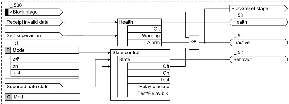
Figure 6-166 Logic Diagram of the Stage Control
