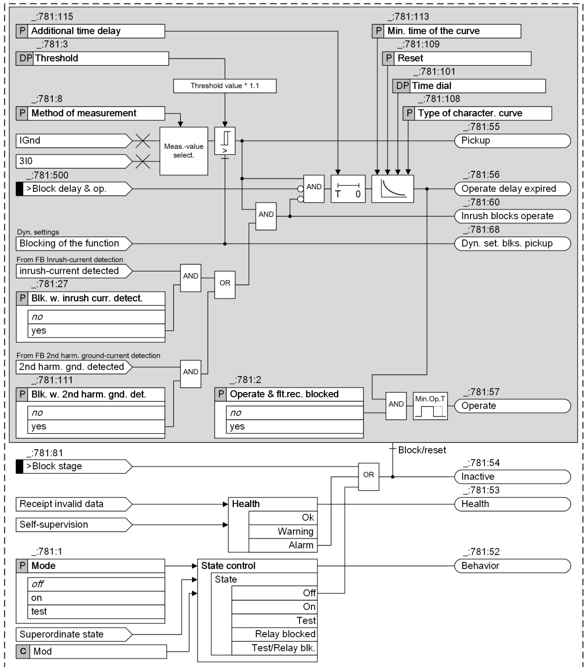
Figure 6-33 Logic Diagram Inverse-Time Overcurrent Protection (Ground) – Advanced
