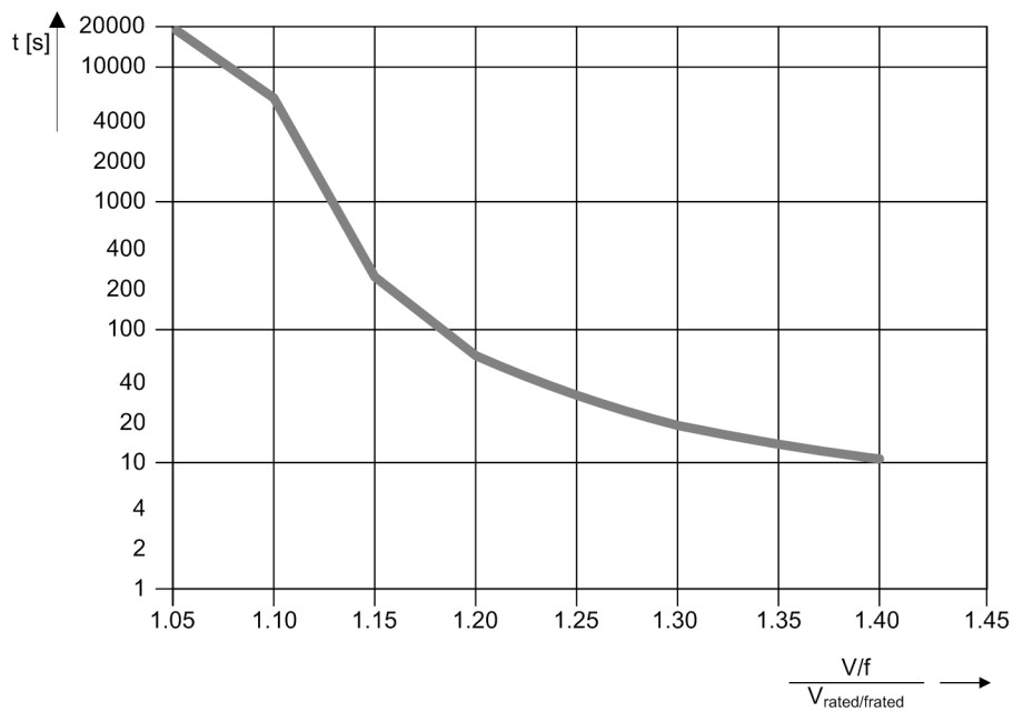
Figure 14-20 Operate Curve from the Thermal Replica of the Overexcitation Protection (Default Setting)
