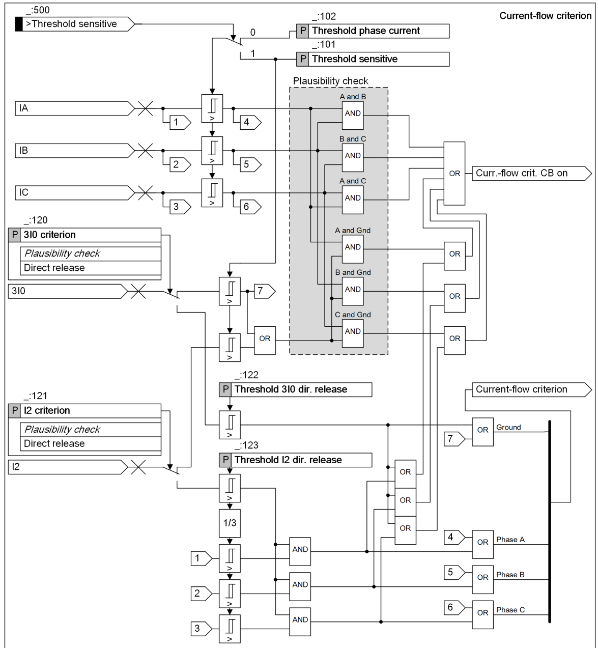
Figure 6-252 Current-Flow Criterion
