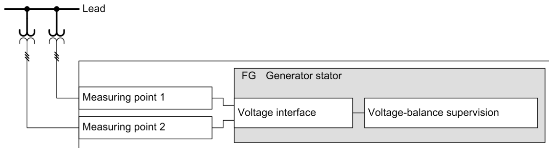
Figure 10-24 Application Example
