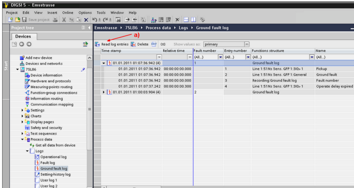
[sc_grfimd, 1, en_US] Figure 3-9 Reading the Ground-Fault Log with DIGSI 5
