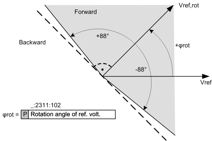
Figure 6-48 Forward Characteristic of the Directional Function, Phase-Measuring Element
