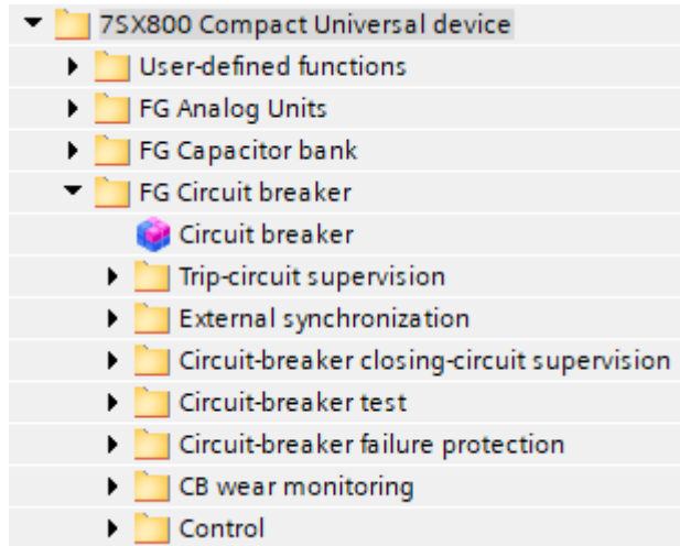
Figure 5-106 Circuit-Breaker Function Group – Example of the Functional Scope
