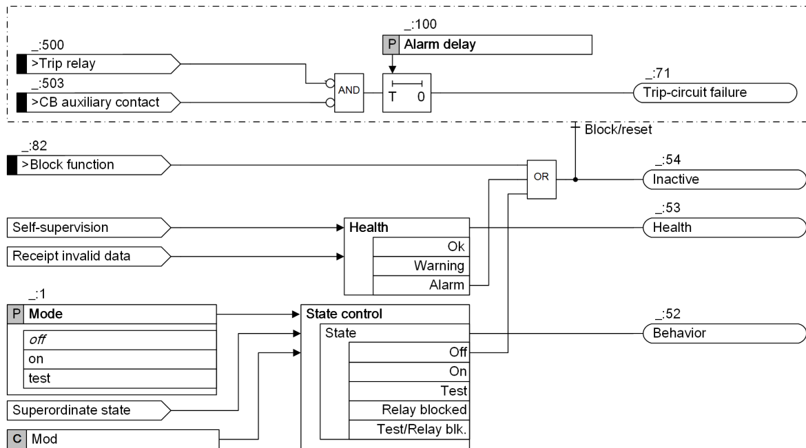
Figure 10-38 Logic Diagram of Trip-Circuit Supervision with 2 Binary Inputs
