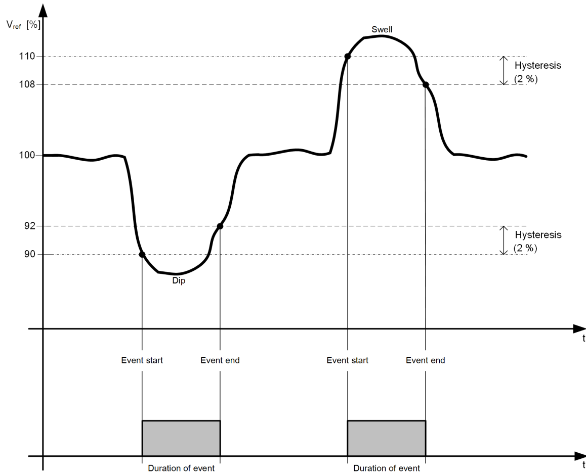
Figure 12-4 Duration of a Voltage-Dip or Voltage-Swell Event
