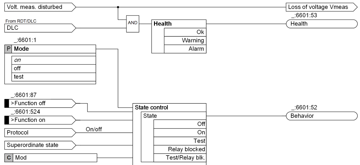
Figure 6-289 Function Control for the Automatic Reclosing Function
