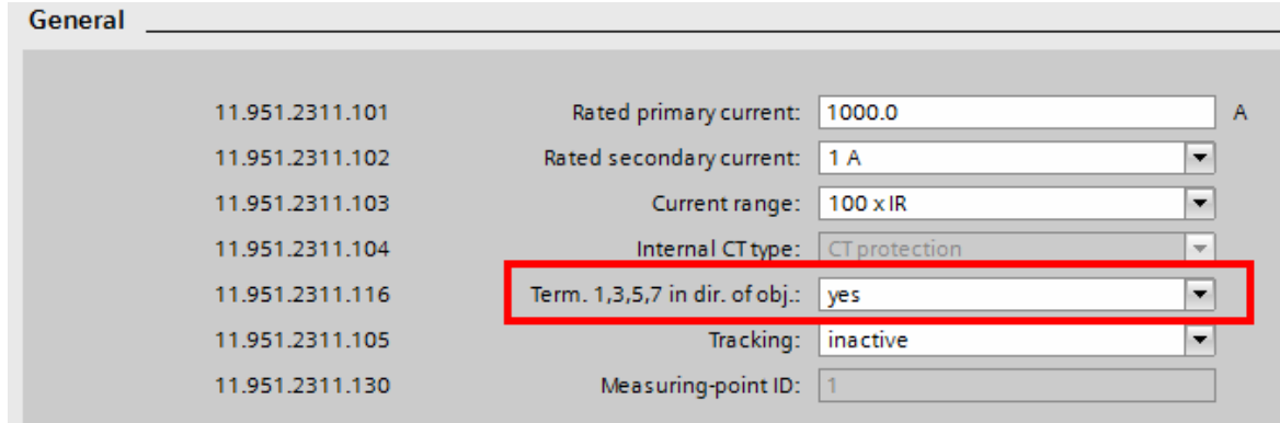
Figure 6-275 DIGSI 5 Setting
