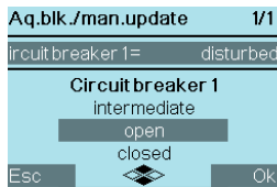
Figure 3-59 Selecting Position
