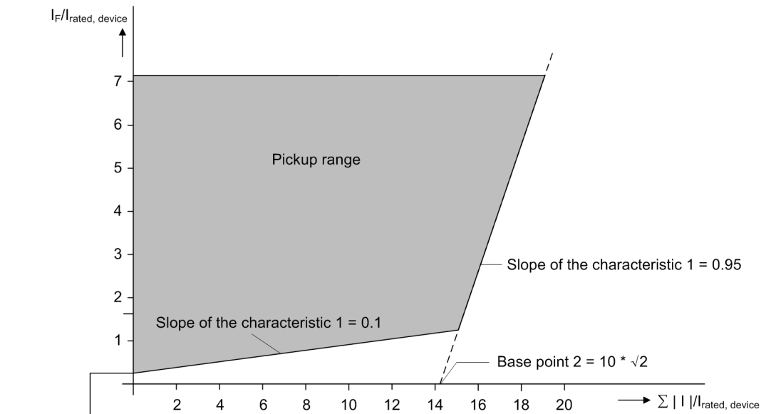
Figure 10-51 Characteristic Curve of the Supervision of the Device-Internal Analog-Digital Converters
