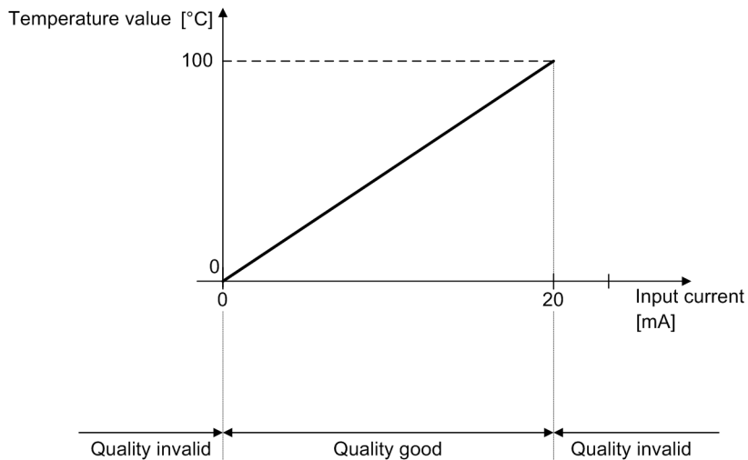
Figure 5-49 Characteristic Curve of a 20-mA Input (Example 1)
