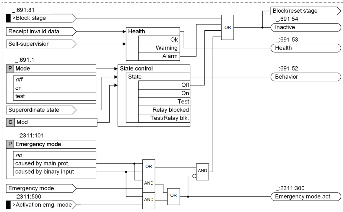
Figure 6-14 Logic Diagram Stage Control
