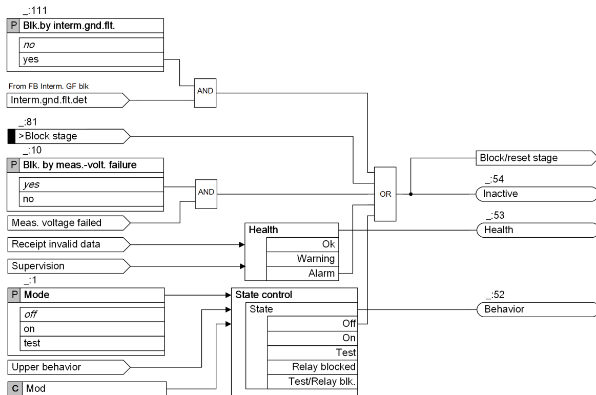
Figure 6-130 Logic Diagram of the Stage Control
