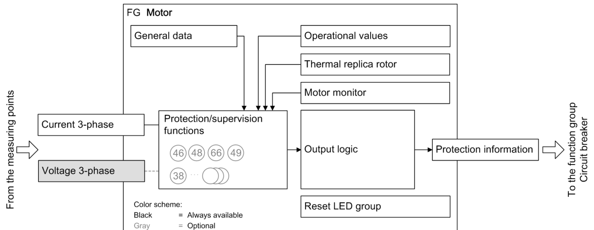
Figure 5-14 Structure of the Motor Function Group
