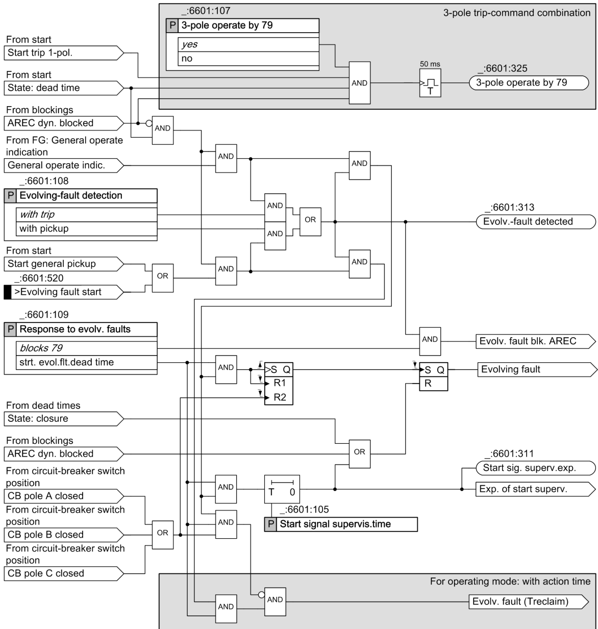
Figure 6-309 Cyclic Automatic Reclosing Function - Logic of Evolving-Fault Detection
