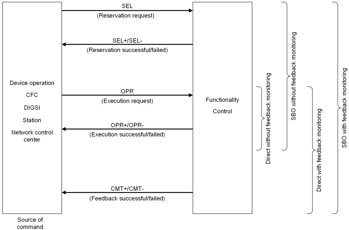
Figure 9-1 Command Sources, Command Types, and Control Models
