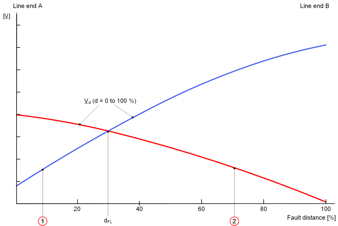
Figure 6-335 Voltage Curve, Calculated from Both Sides of the Line
