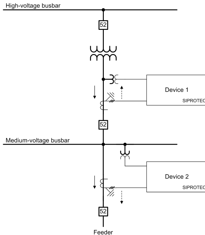
Figure 6-218 Application Scenarios
