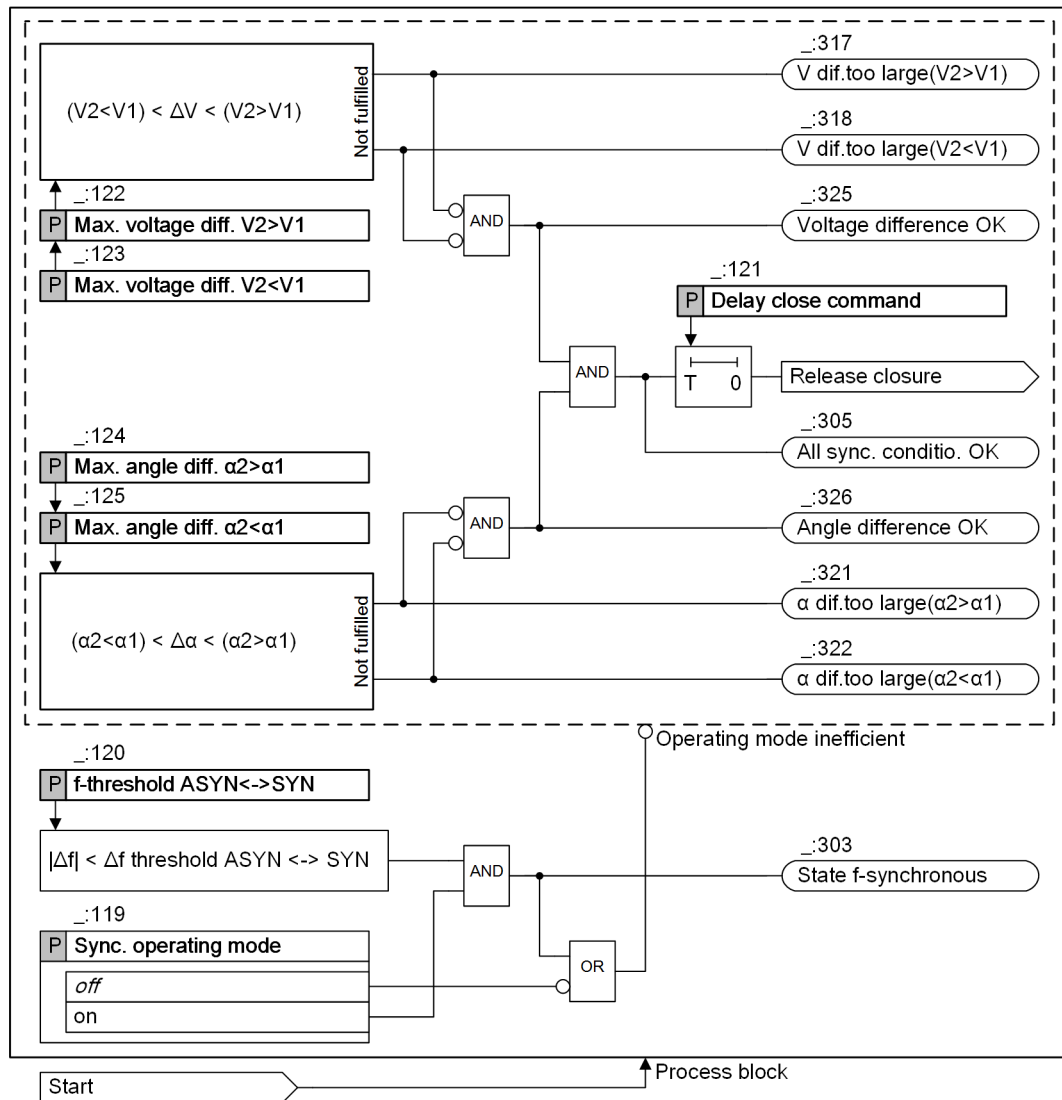
Figure 9-63 Closing Conditions when Switching Synchronous Systems
