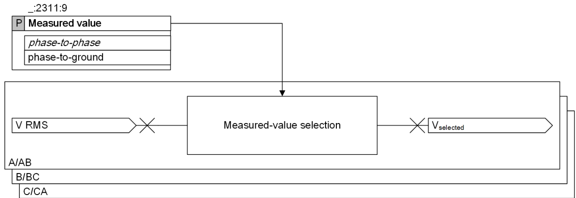
Figure 12-2 Logic Diagram of Measured-Value Selection
