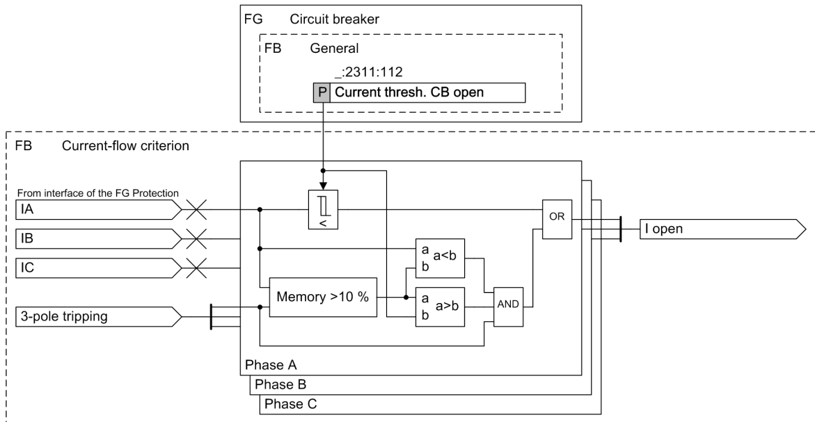
Figure 5-140 Logic Diagram of the Current-Flow Criterion Function Block
