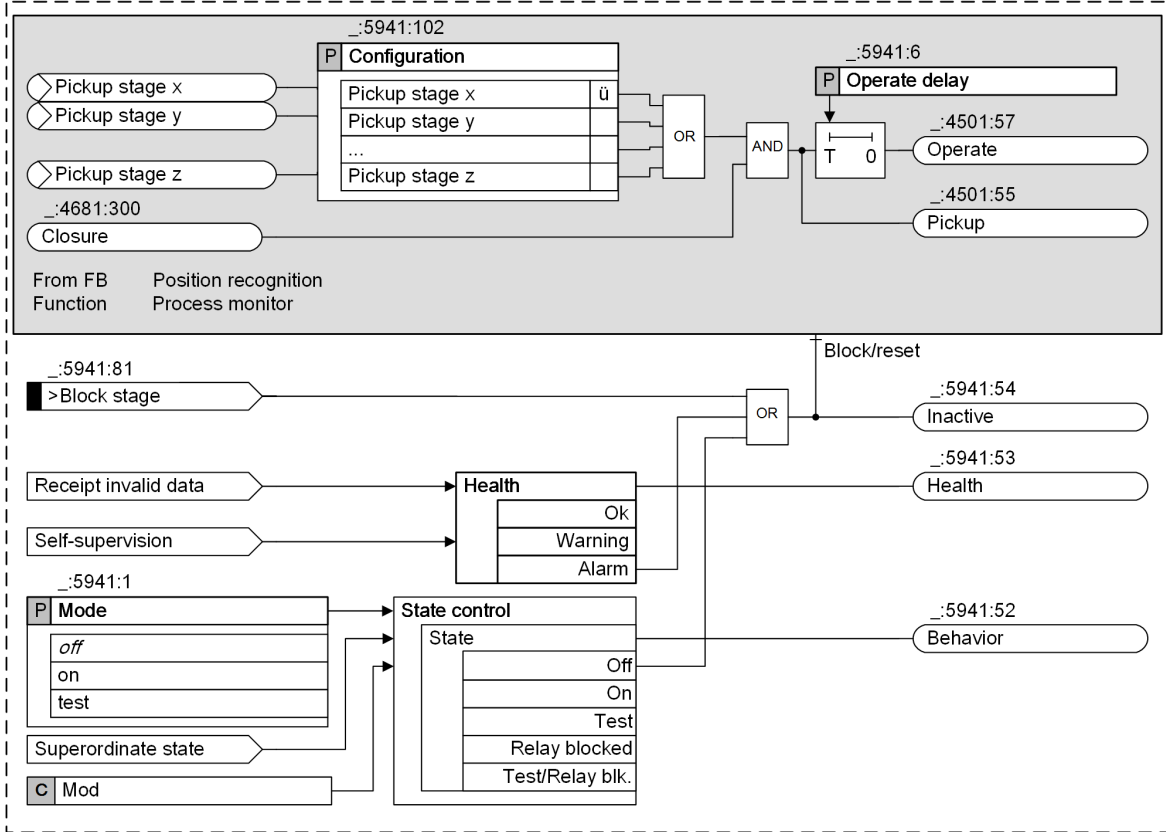
Figure 6-83 Logic Diagram of the Stage Instantaneous Tripping at Switch onto Fault
