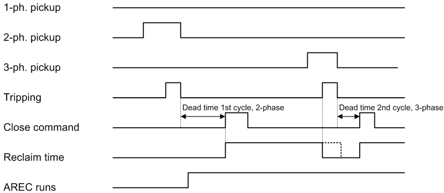
Figure 6-295 Operating-Mode Signal Examples: With Pickup/Without Action Time
