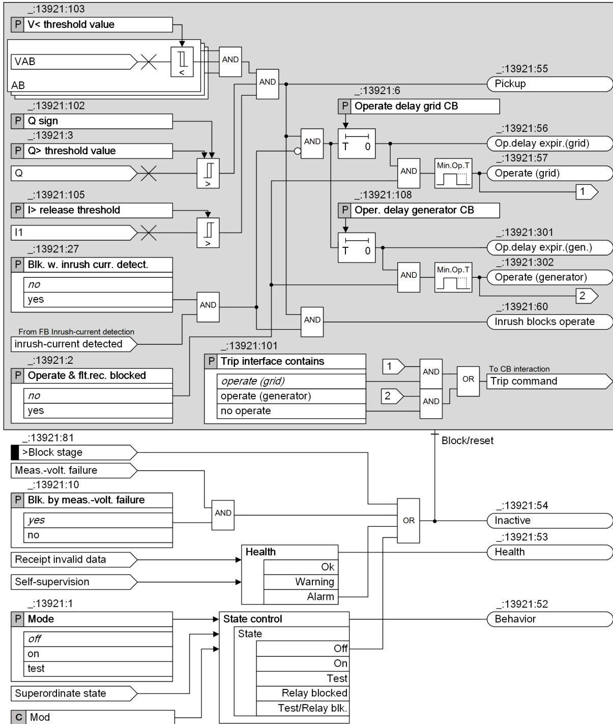
Figure 6-245 Logic Diagram of the Protection Stage of the Undervoltage-Controlled Reactive-Power Protection
