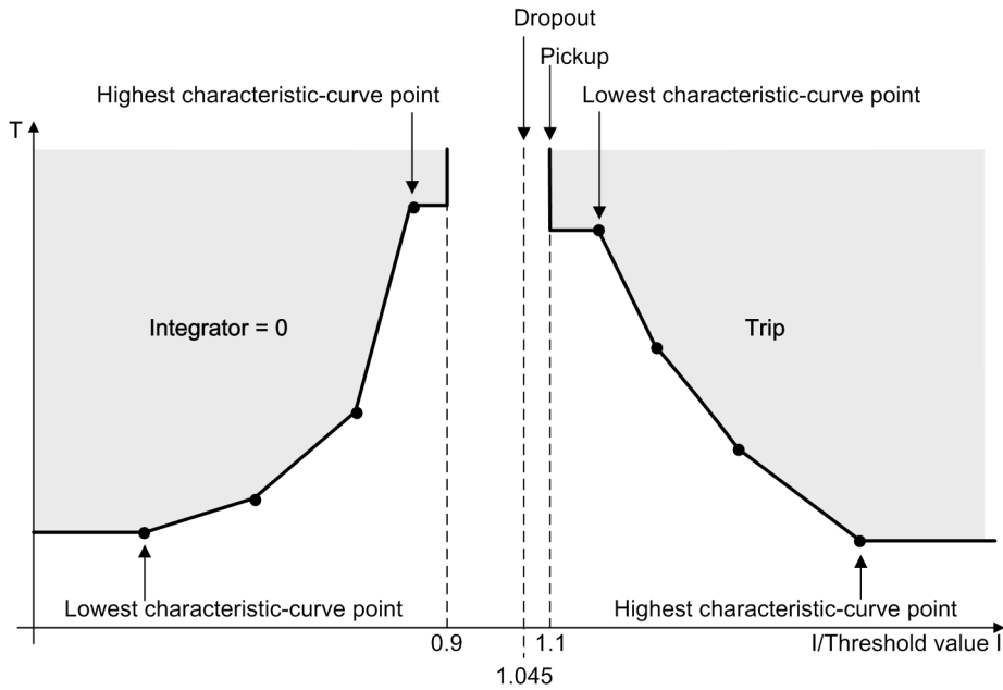
Figure 6-45 Pickup and Dropout Behaviors when Using a Directional User-Defined Characteristic Curve
