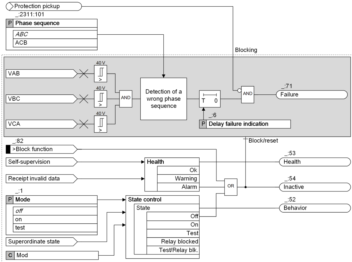
[lo_volt-phas-rotation-supervision, 5, en_US] Figure 10-22 Logic Diagram of the Voltage Phase-Rotation Supervision
