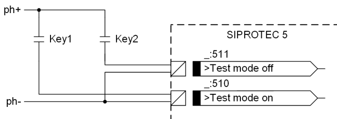
Figure 13-2 External Wiring of Push-Buttons for Enabling/Disabling the Test Mode for the Entire Device
