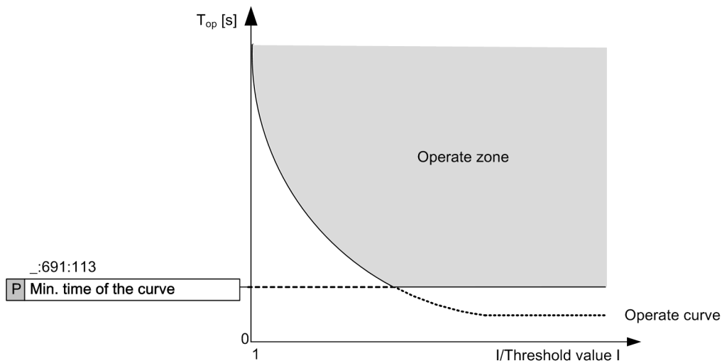
[idw_ocp_3_mi_1_en_US] Figure 6-16 Minimum Operating Time of the Curve
