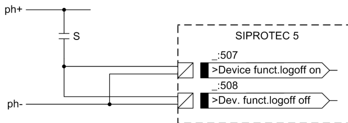
Figure 3-66 External Switch Wiring for Logging off the Device
