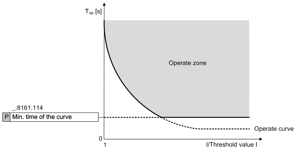
[idw_docp_01_1_en_US] Figure 6-44 Minimum Operating Time of the Curve
