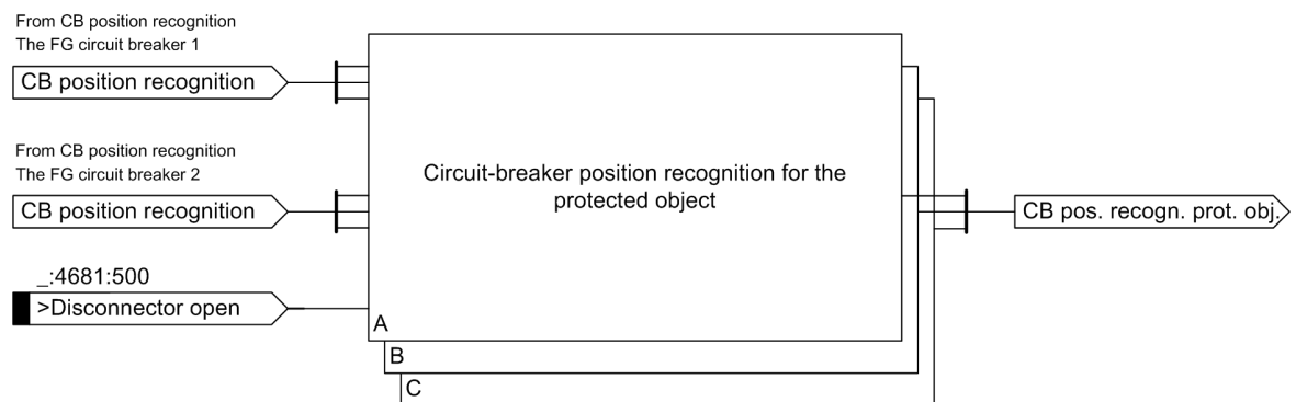
Figure 5-141 Logic Diagram of the Circuit-Breaker Condition for the Protected-Object Function Block
