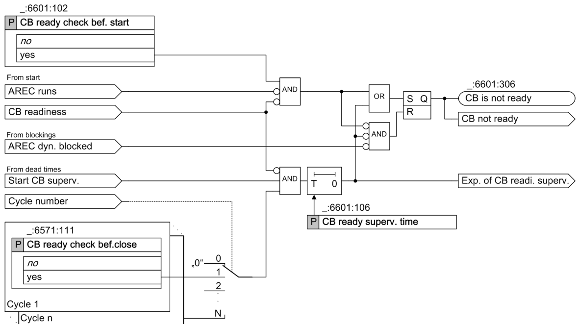
Figure 6-314 Cyclic Automatic Reclosing: Logic for the Circuit-Breaker Readiness
