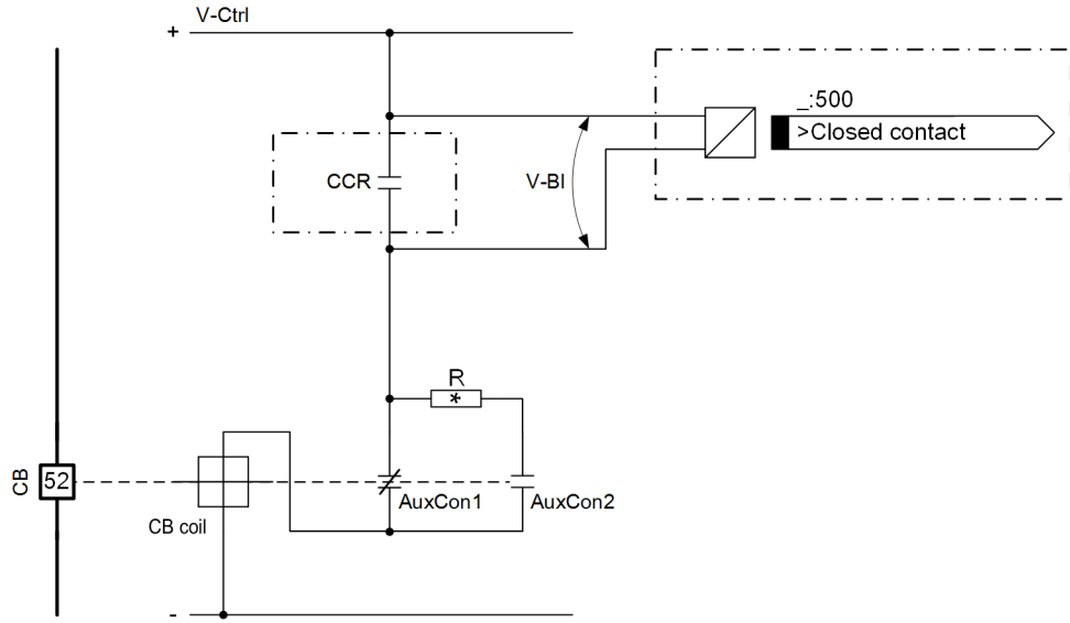
Figure 10-47 Principle of the Closing-Circuit Supervision with 1 Binary Input
