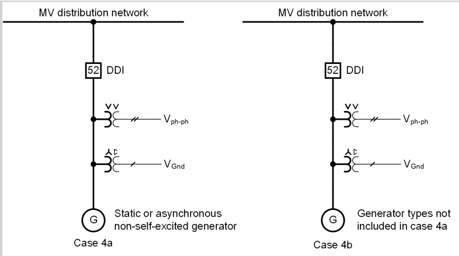
Figure 6-362 Application Example of Voltage-Transformer Positions: Case 4
