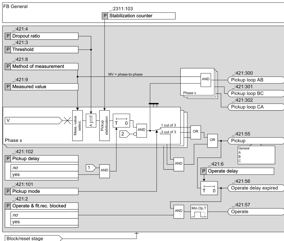
Figure 6-199 Logic Diagram of the Definite-Time Undervoltage Protection with 3-Phase Voltage
