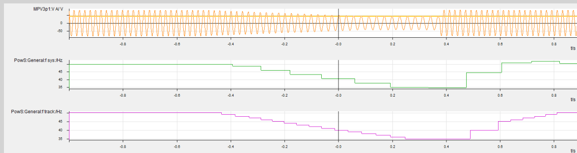
Figure 3-34 Example of Frequency Tracking and Reaction to a Step Change in the Input Variable
