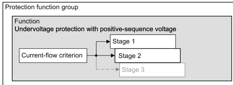
Figure 6-203 Structure/Embedding of the Function
