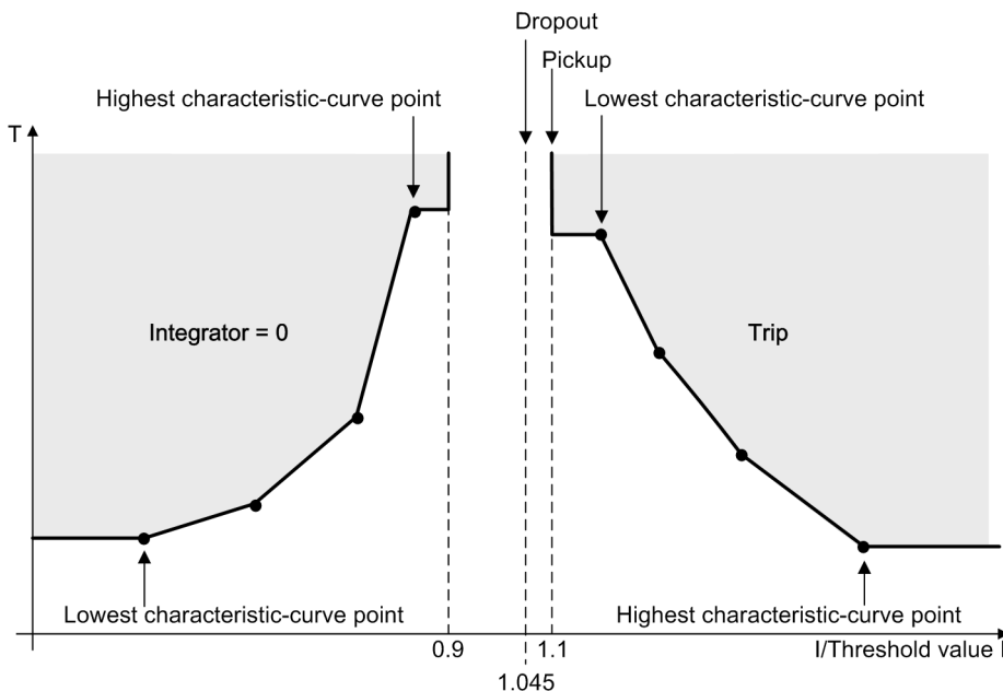
Figure 6-18 Pickup Behavior and Dropout Behavior when Using a User-Defined Characteristic Curve
