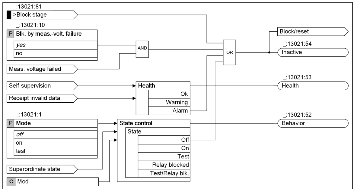
Figure 6-124 Logic Diagram of the Stage Control
