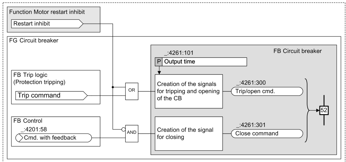
Figure 7-11 Processing the Restart Inhibit Signal
