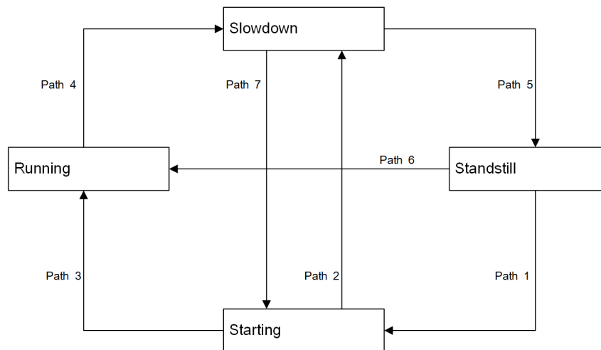
Figure 5-26 Motor State Machine
