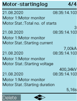
Figure 3-25 Reading the Motor-Starting Log on the On-Site Operation Panel of the Device
