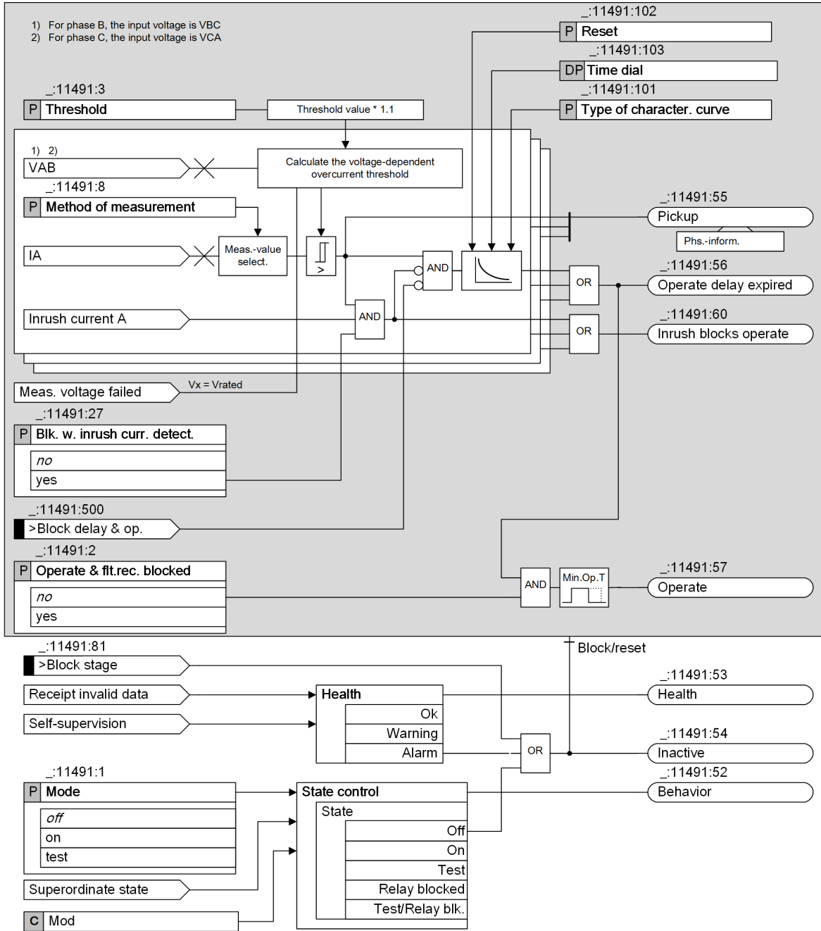
Figure 6-23 Logic Diagram of the Inverse-Time Overcurrent Protection, Voltage-Dependent
