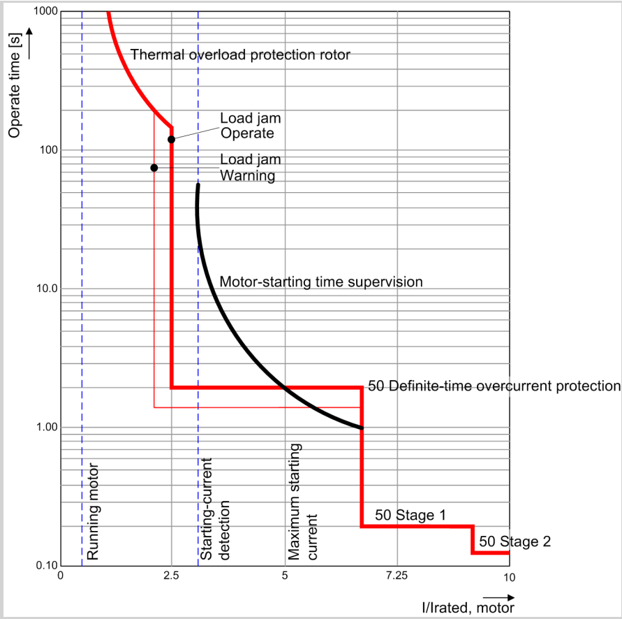
Figure 7-18 Example of a Complete Motor-Protection Characteristic Curve
