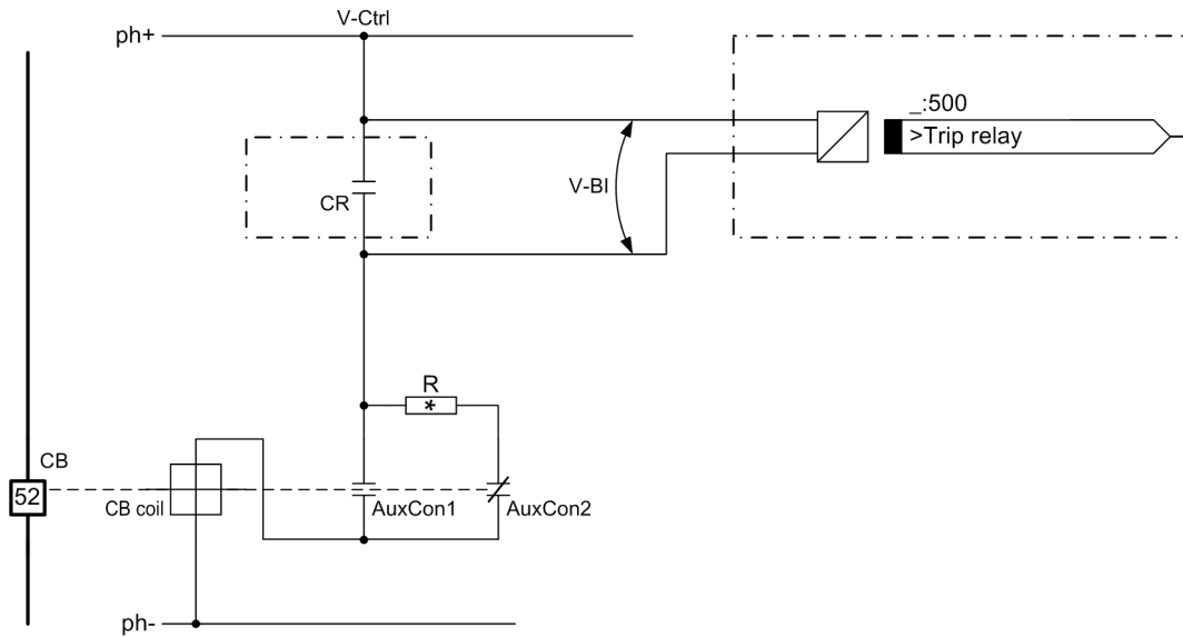
Figure 10-39 Principle of Trip-Circuit Supervision with 1 Binary Input
