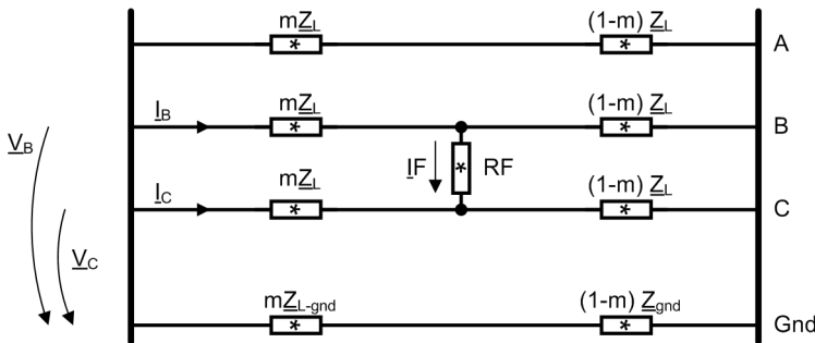
Figure 6-328 Short Circuit of a Phase-to-Phase Loop
