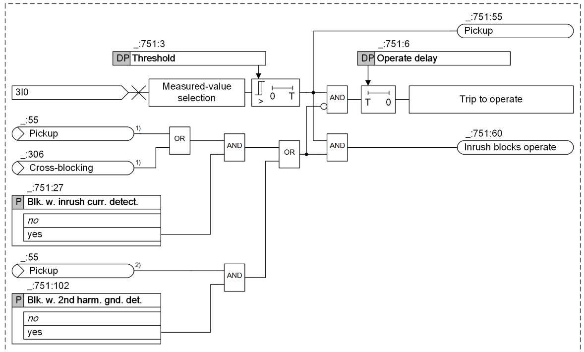
Figure 6-36 Part-Logic Diagram on the Influence of Inrush-Current Detection Exemplified by the 1st Definite-Time Overcurrent Protection Stage
