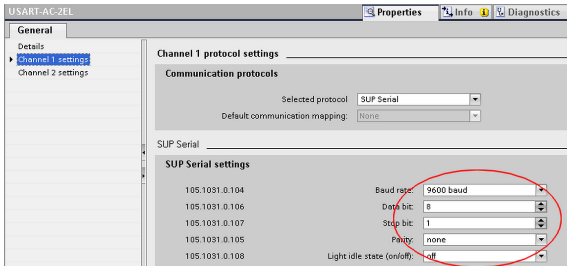
Figure 5-67 Making the Communication Settings
