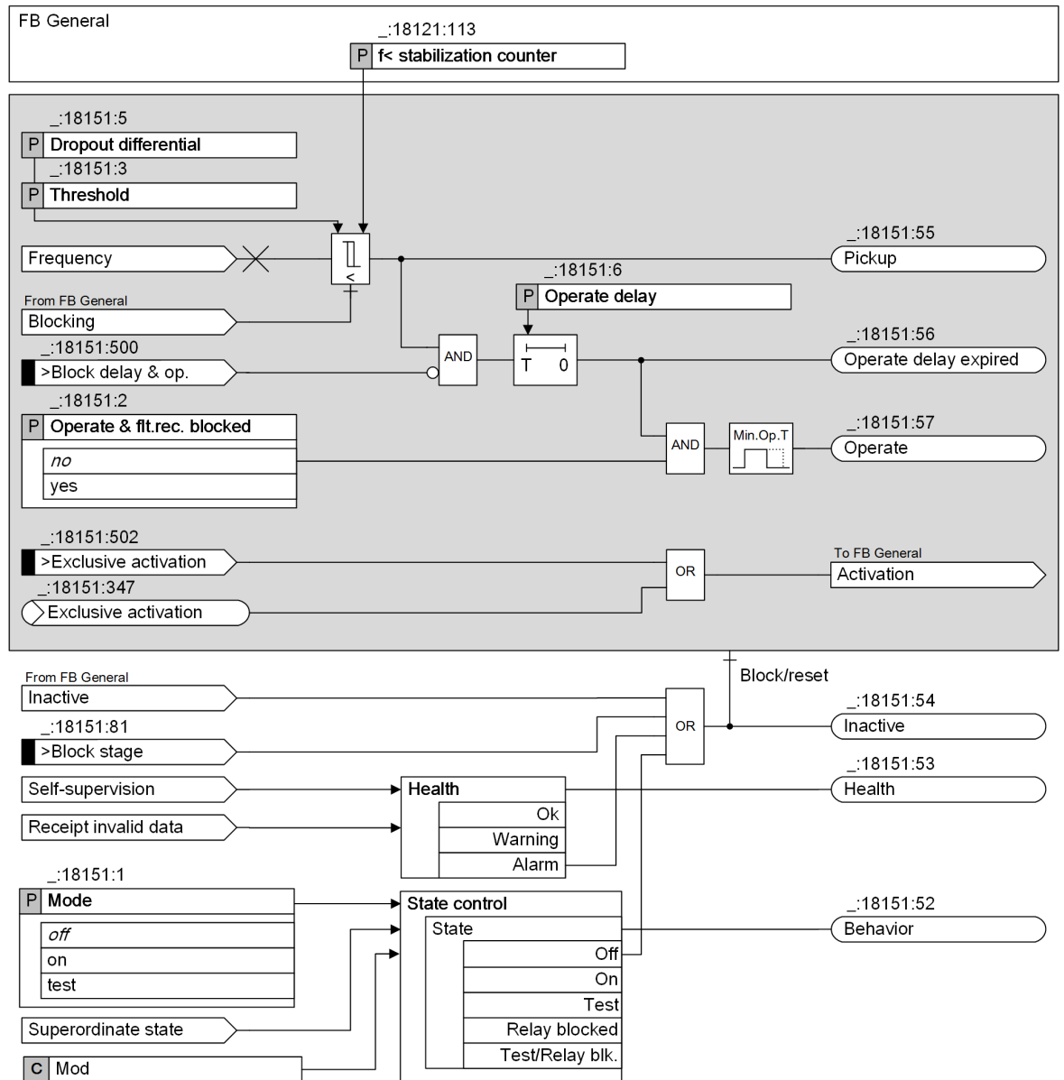
Figure 6-219 Logic Diagram of the Underfrequency Load Shedding Stage
