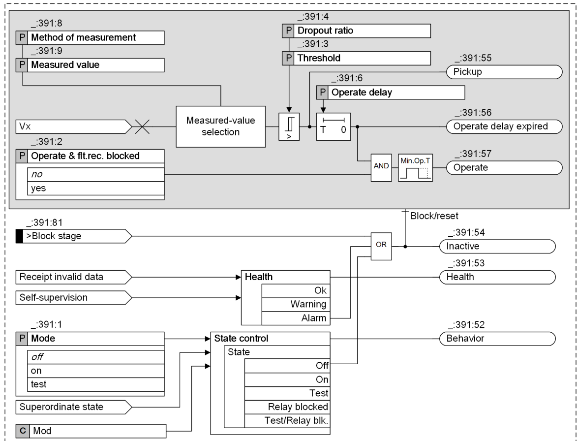
Figure 6-191 Logic Diagram of a Stage: Overvoltage Protection with Any Voltage
