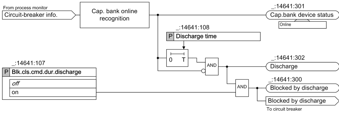
Figure 5-39 Logic Diagram of Capacitor Bank Device Status and Blocking of Circuit-breaker Closing during Discharging
