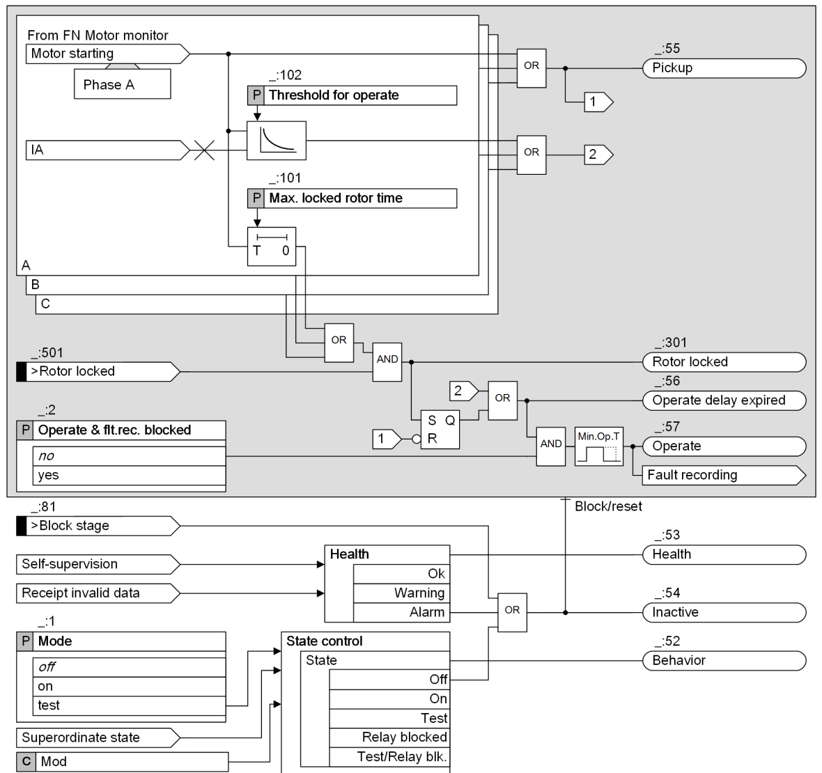
Figure 7-6 Logic Diagram of Motor-Starting Time Supervision with User-Defined Characteristic Curve
