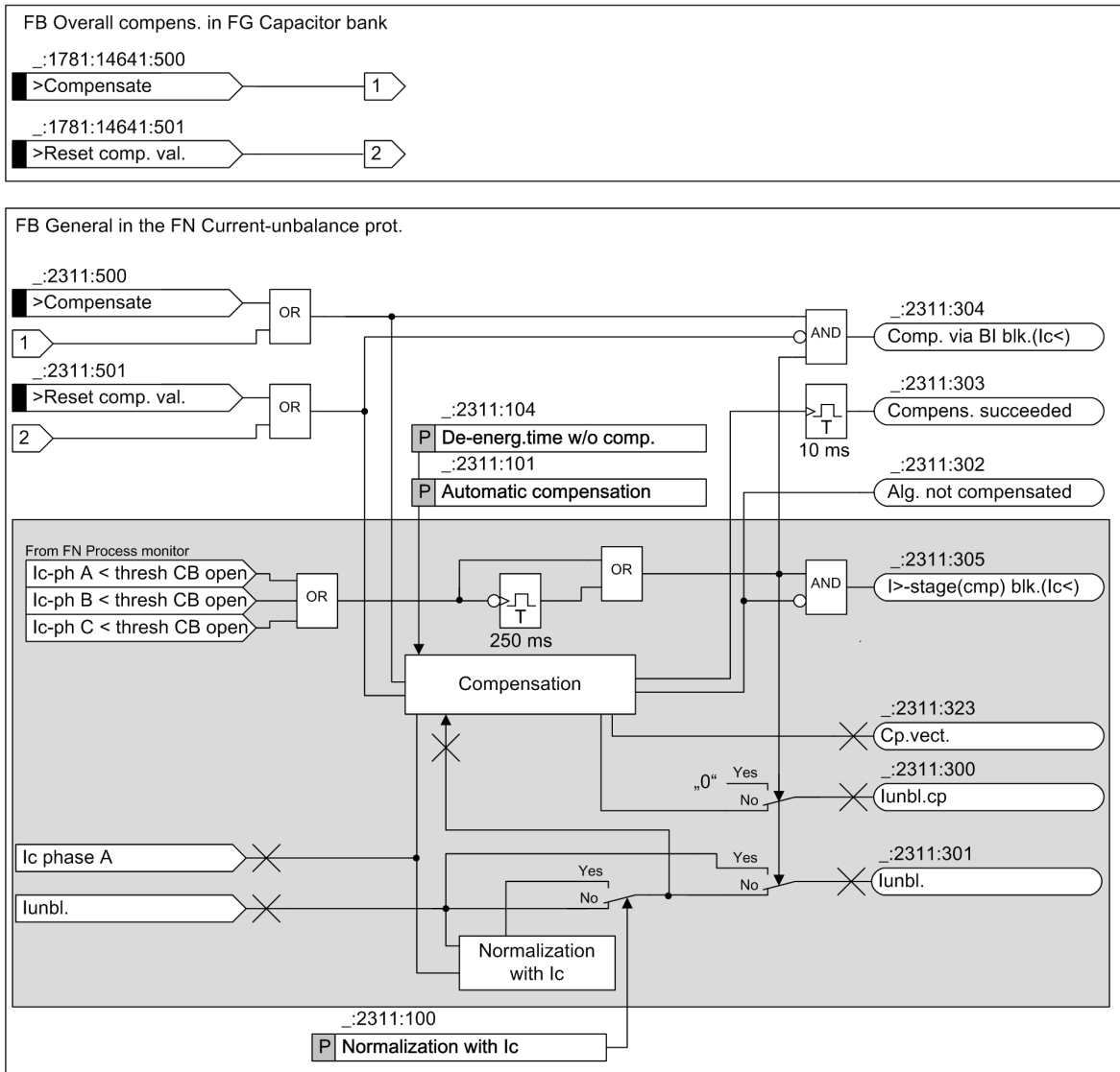
Figure 8-2 Cross-Stage Functionality
