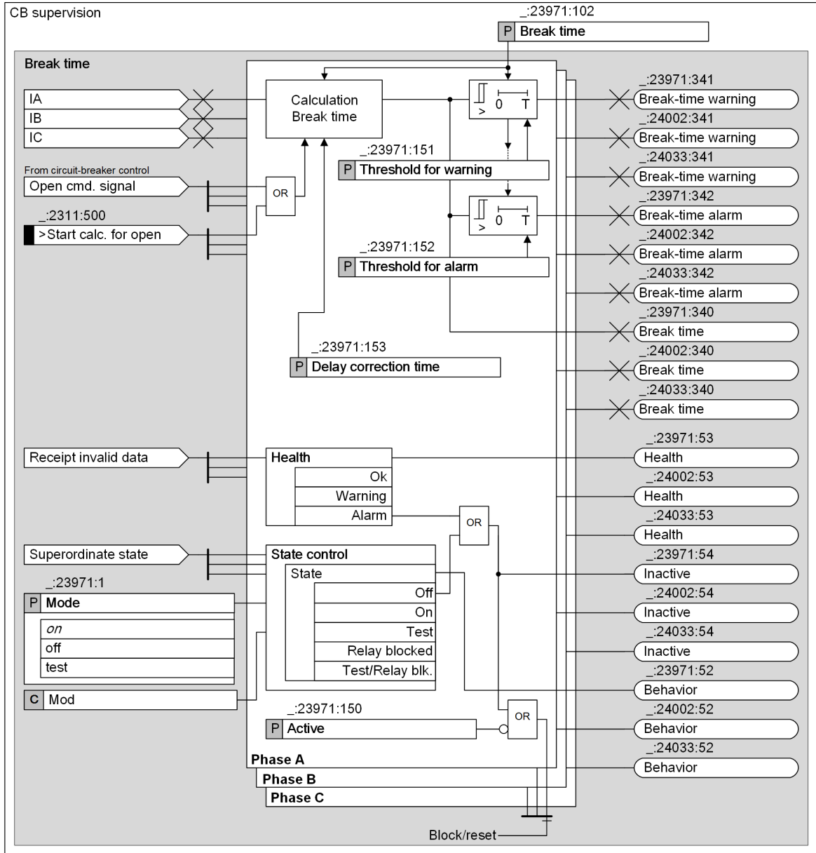
Figure 11-15 Logic of the Break Time
