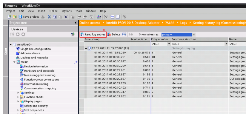
Figure 3-11 Reading the Setting-History Log with DIGSI 5
