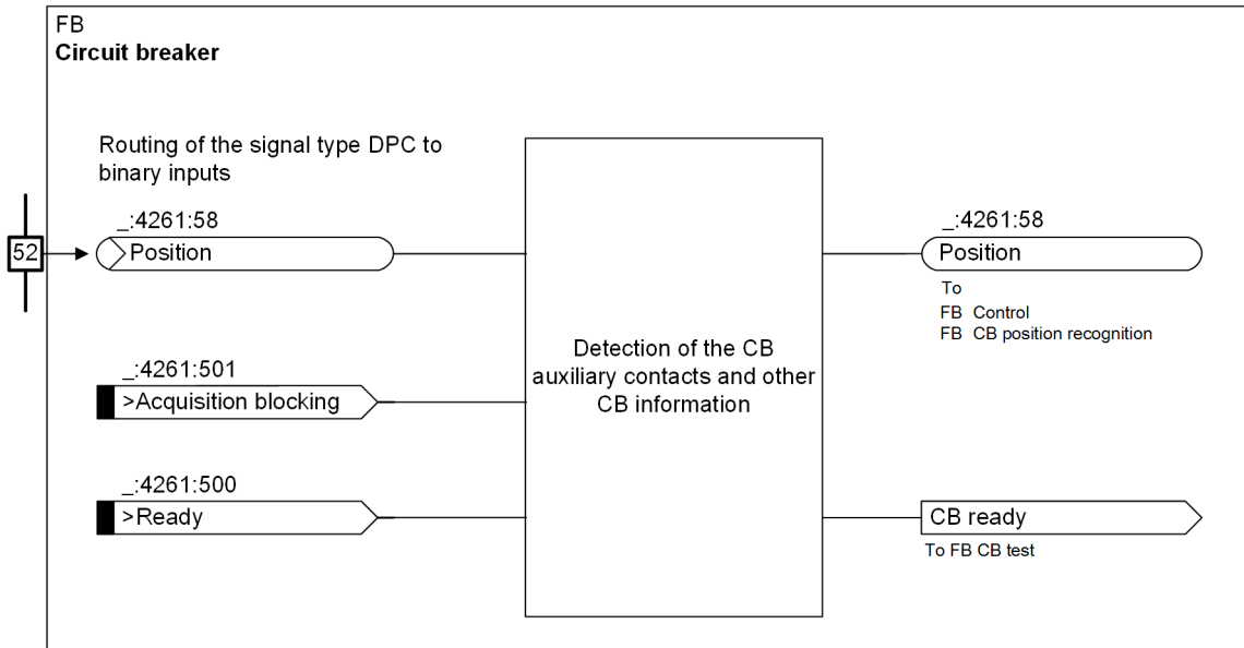
Figure 5-126 Acquisition of the Circuit-Breaker Information
