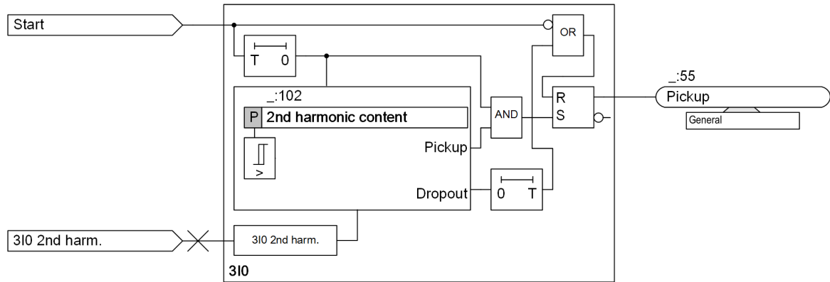
Figure 6-77 Logic of the Harmonic Analysis Function
