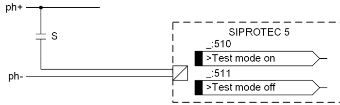
Figure 13-3 External Wiring of Switches for Enabling/Disabling the Test Mode for the Entire Device
