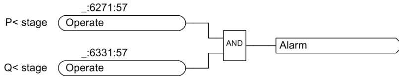
Figure 6-230 Logical Combination of Operate Indications in CFC
