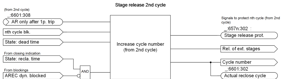
Figure 6-305 Stage Release for Protection Functions Starting With the 2nd Automatic Reclosing Cycle
