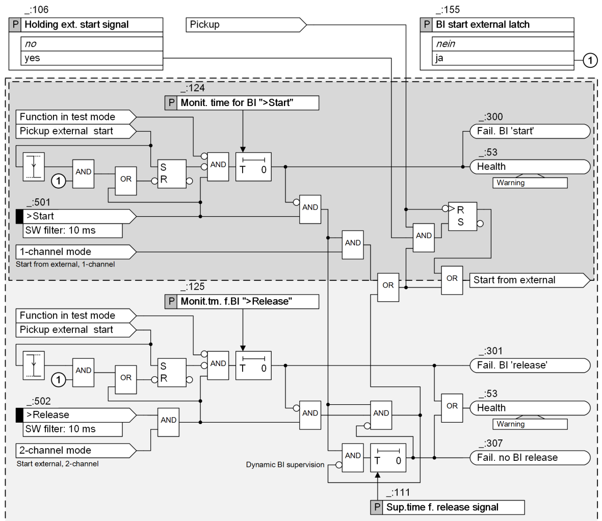
Figure 6-251 External Start of the Circuit-Breaker Failure Protection Function, Logic
