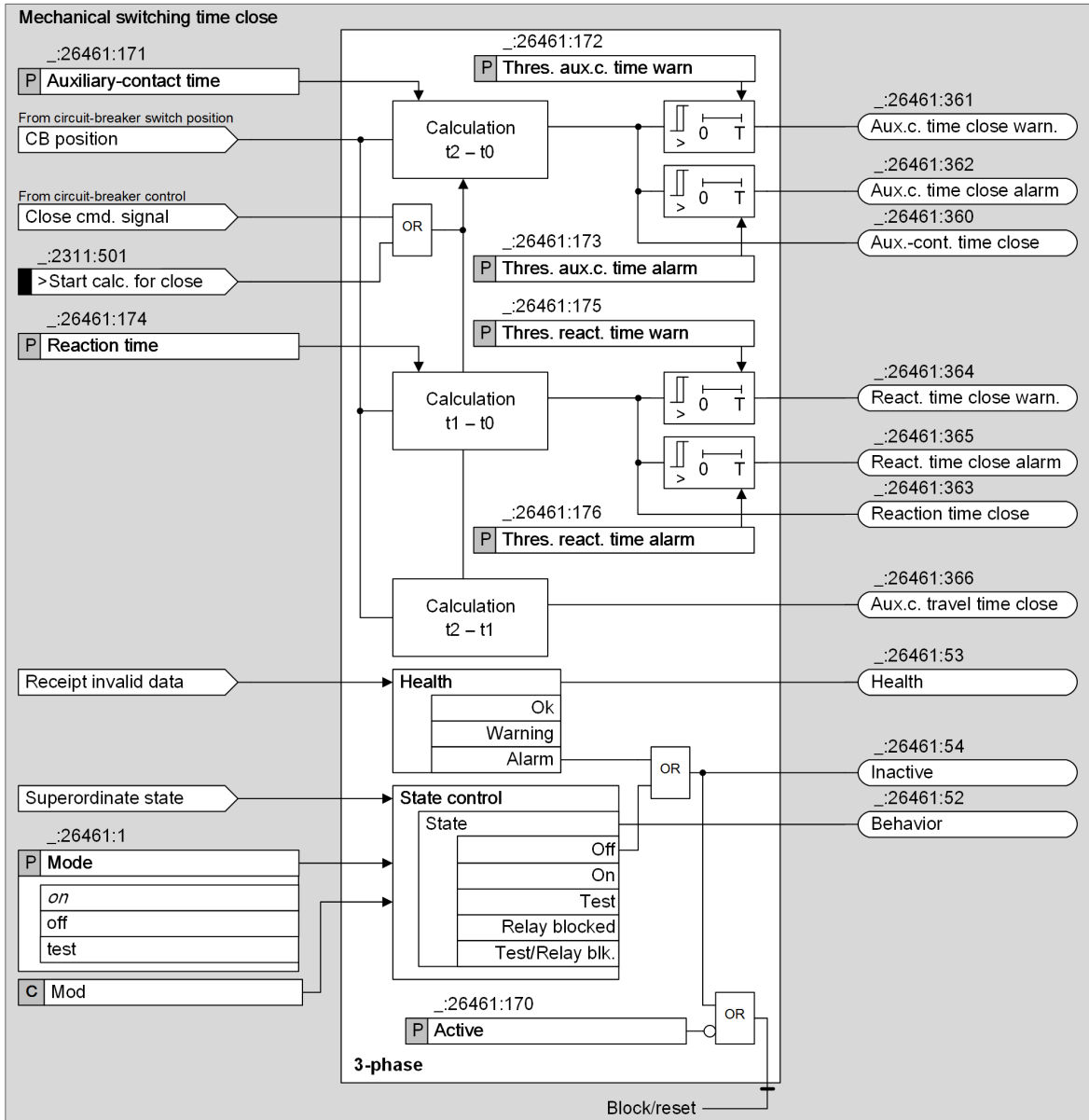
Figure 11-20 Logic of the Stage Mechanical Switching Time Close for Circuit Breakers 3-Pole
