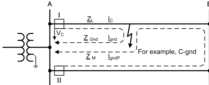
Figure 6-329 Ground Fault on a Double Line
