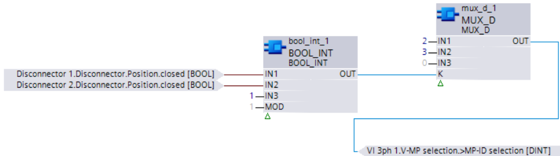
Figure 6-351 Logic Block Chart: Voltage Selection Using Measuring Point ID
