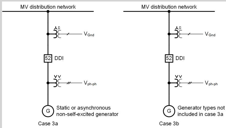
Figure 6-361 Application Example of Voltage-Transformer Positions: Case 3
