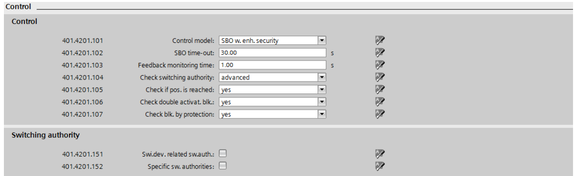
Figure 9-25 Additional Parameters for Switching Authorities in the Parameters of a Switching Device
