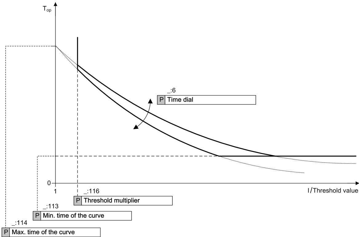
Figure 14-10 Operate Curve of Logarithmic Inverse-Time Characteristic
