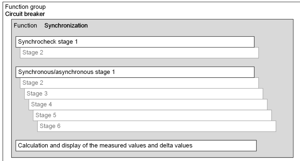
Figure 9-48 Structure/Embedding of the Function
