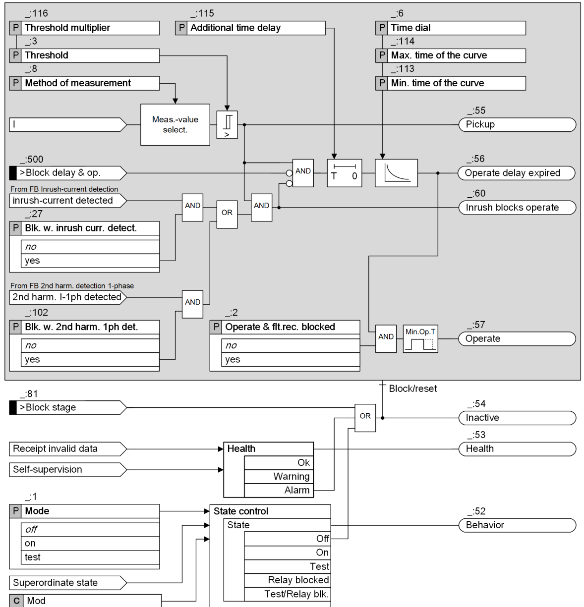
Figure 6-88 Logic Diagram of the Logarithmic Inverse-Time Overcurrent Protection (1-Phase)
