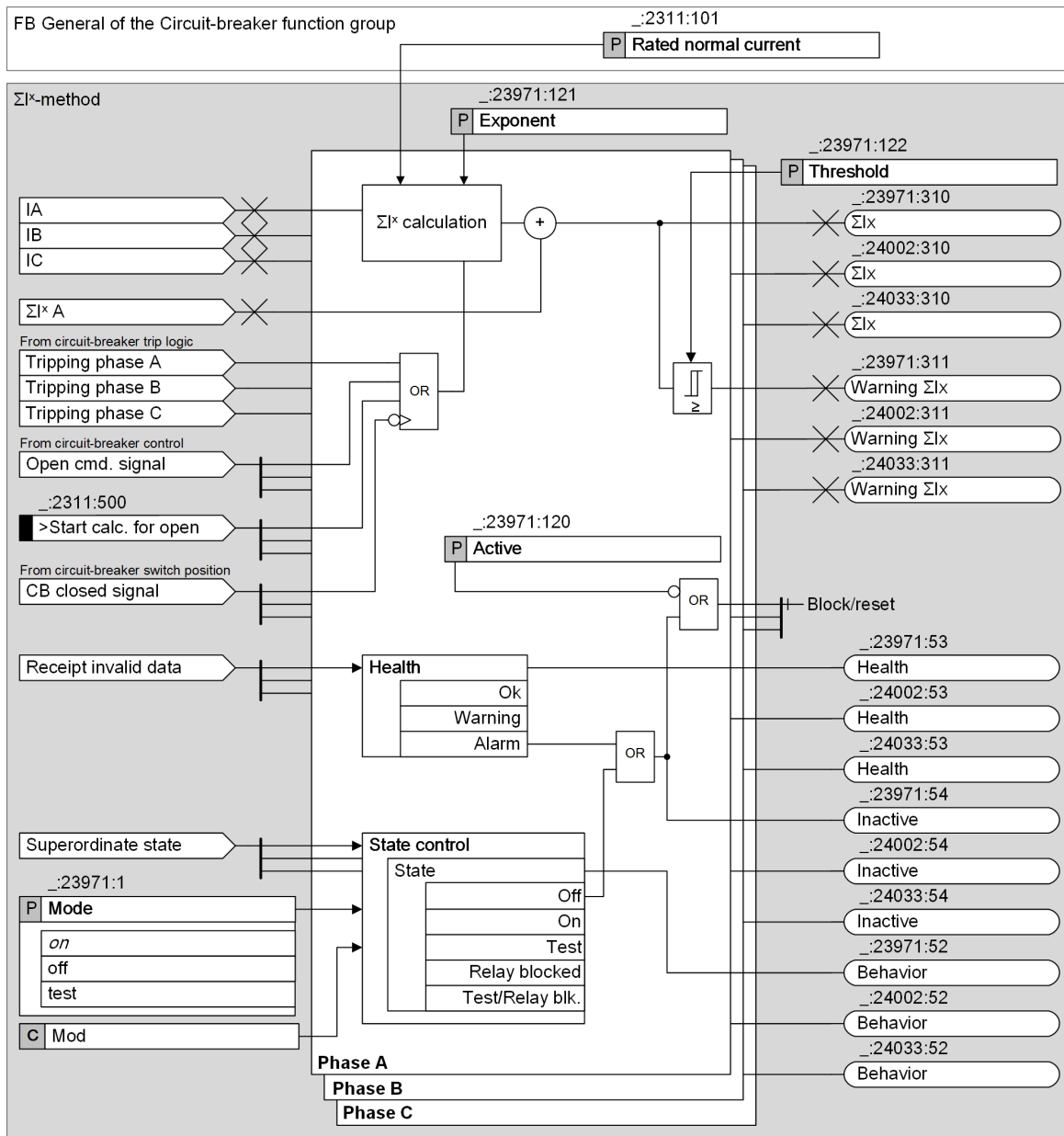
Figure 11-8 Logic of the \Sigma I^x Method
