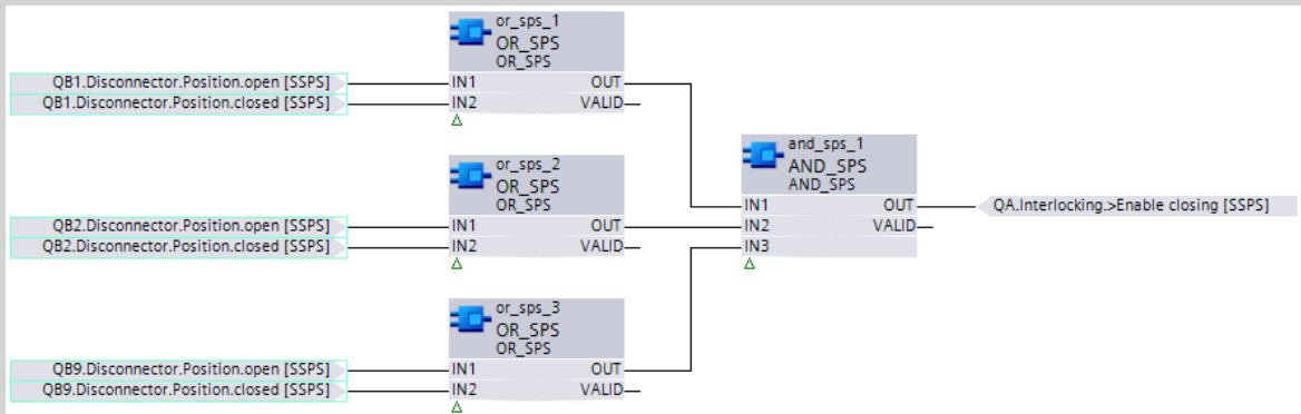
Figure 9-36 Interlocking Chart for Bay Interlocking
