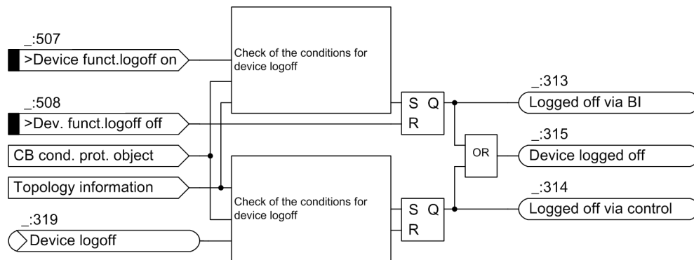
Figure 3-63 Logic for Logging off the Device
