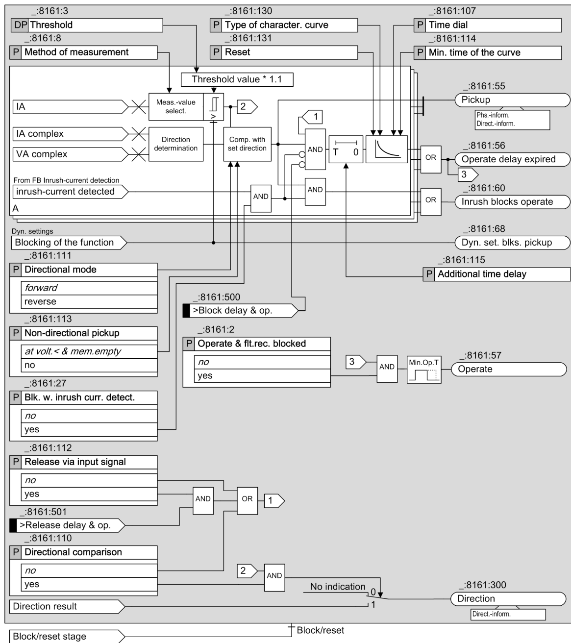
Figure 6-43 Logic Diagram of the Directional, Inverse-Time Overcurrent Protection, Phases - Advanced
