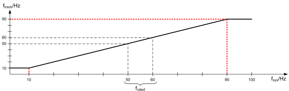
Figure 3-32 Operating Range of Sampling-Frequency Tracking
