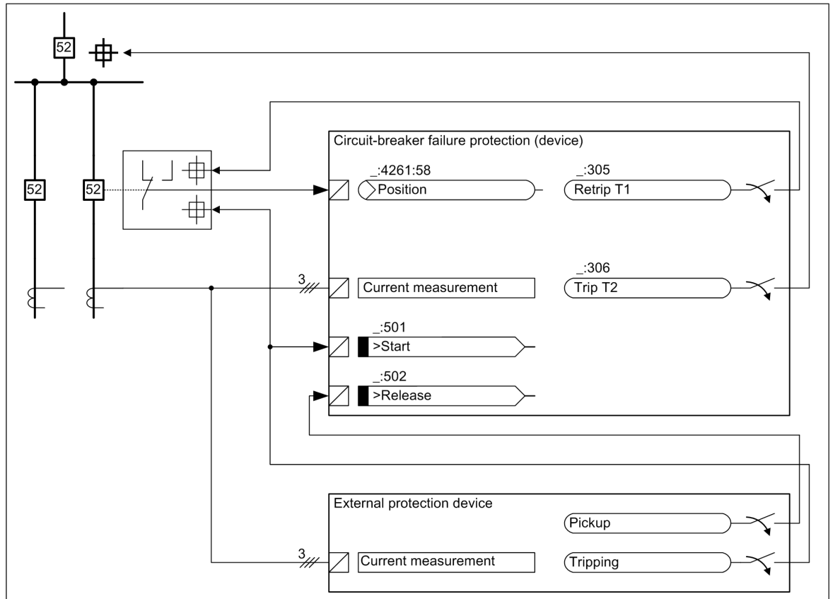
Figure 6-256 Circuit-Breaker Failure Protection with External Start, Tripping Repetition, and 3-Pole Tripping (T2)
