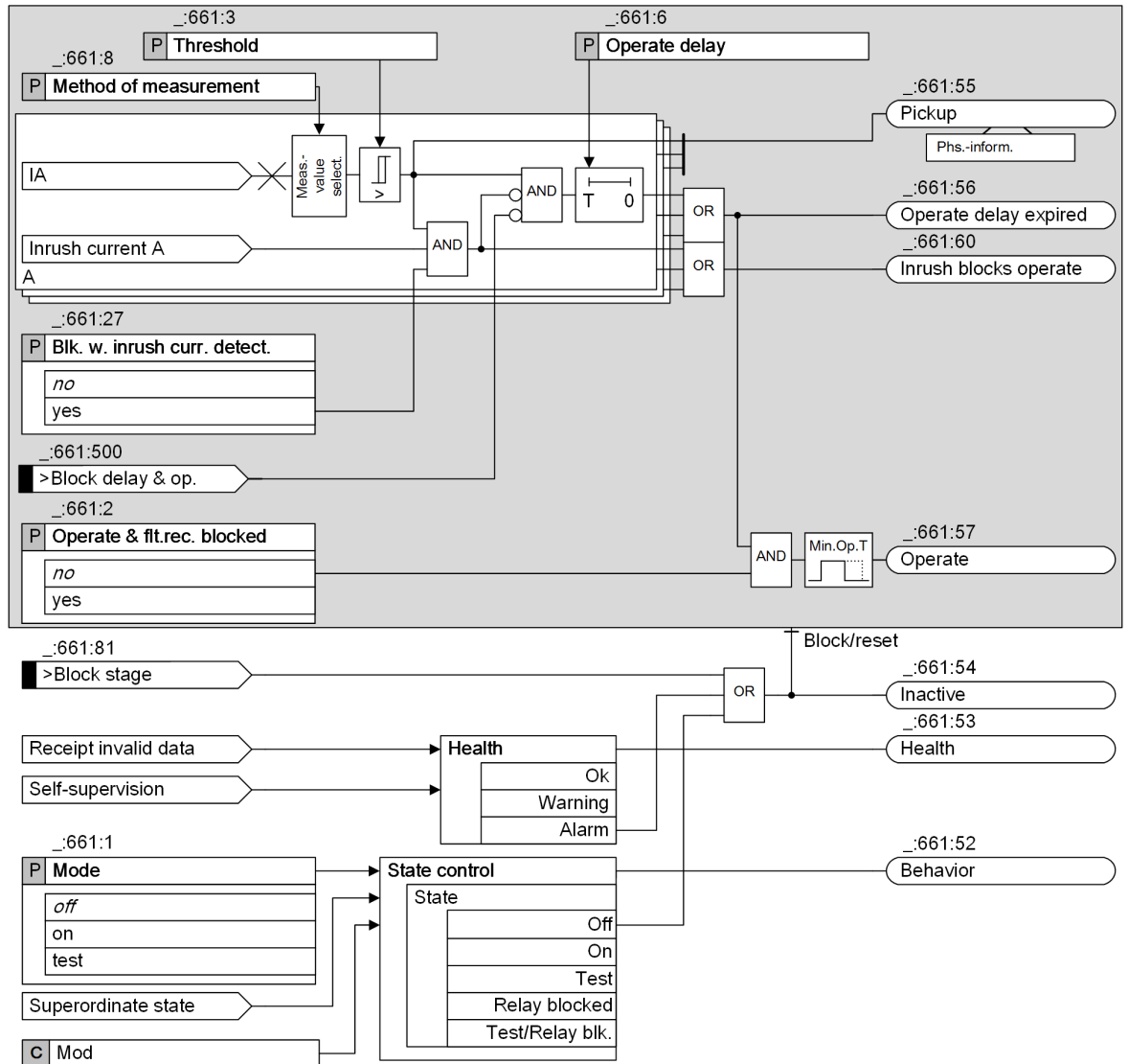
Figure 6-9 Logic Diagram of the Definite-Time Overcurrent Protection (Phases) – Basic
