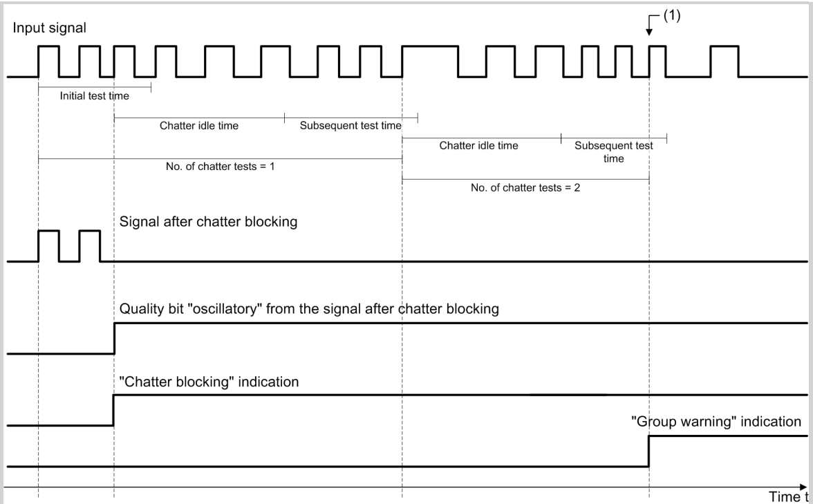
Figure 3-55 Signal Change during Chatter Blocking with too Important Number of Signal State Changes During 2nd Subsequent Test Time
