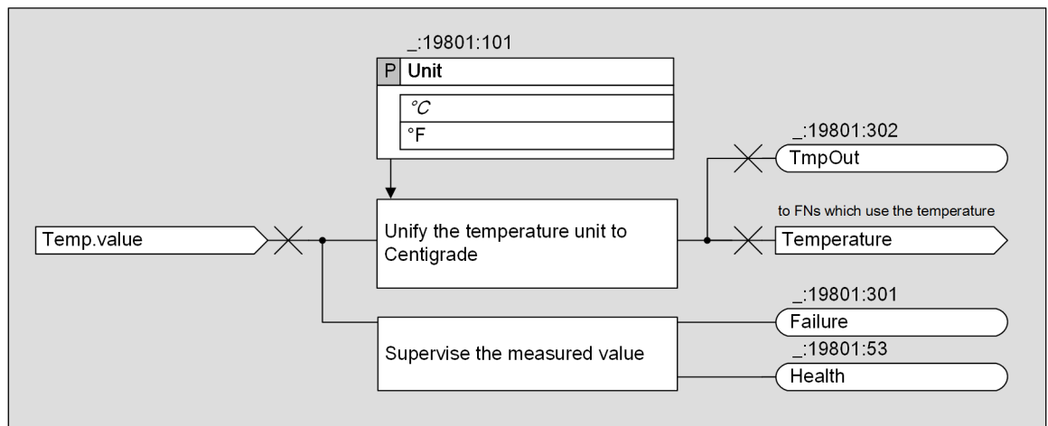
Figure 5-82 Logic Diagram of the Stage
