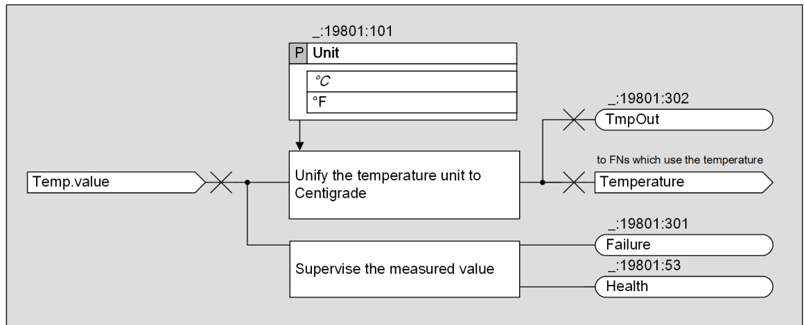
Figure 5-75 Logic Diagram of the Stage
