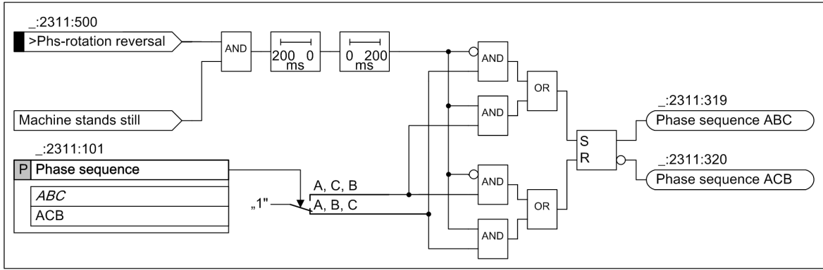
[ldw_phrrpsys1, 2, en_US] Figure 6-342 Phase Sequence Switchover
