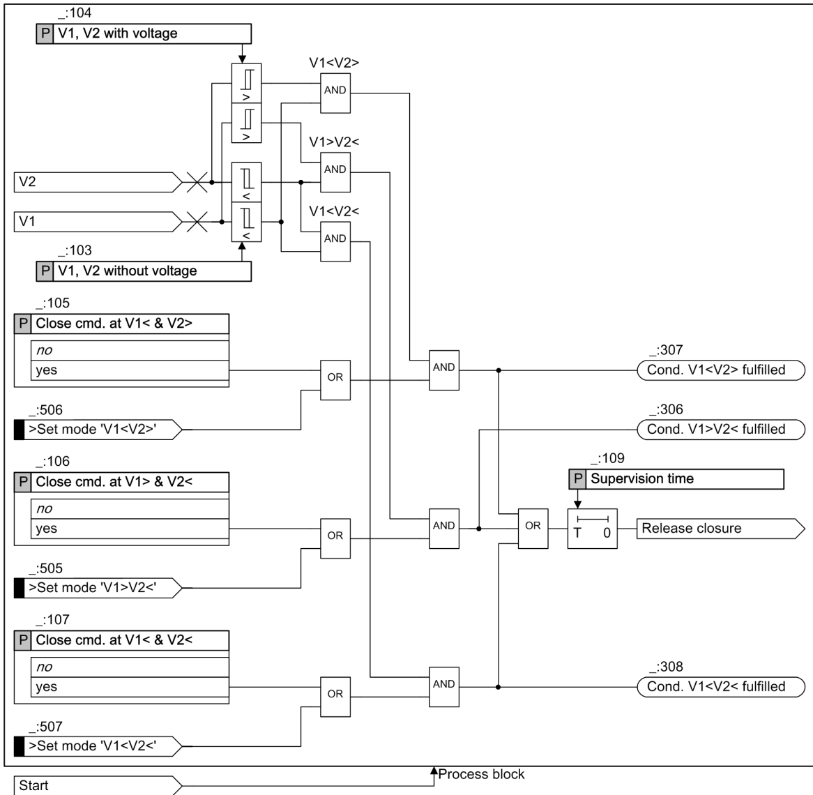
Figure 9-77 Release Conditions for Switching to De-Energized Line/Busbar
