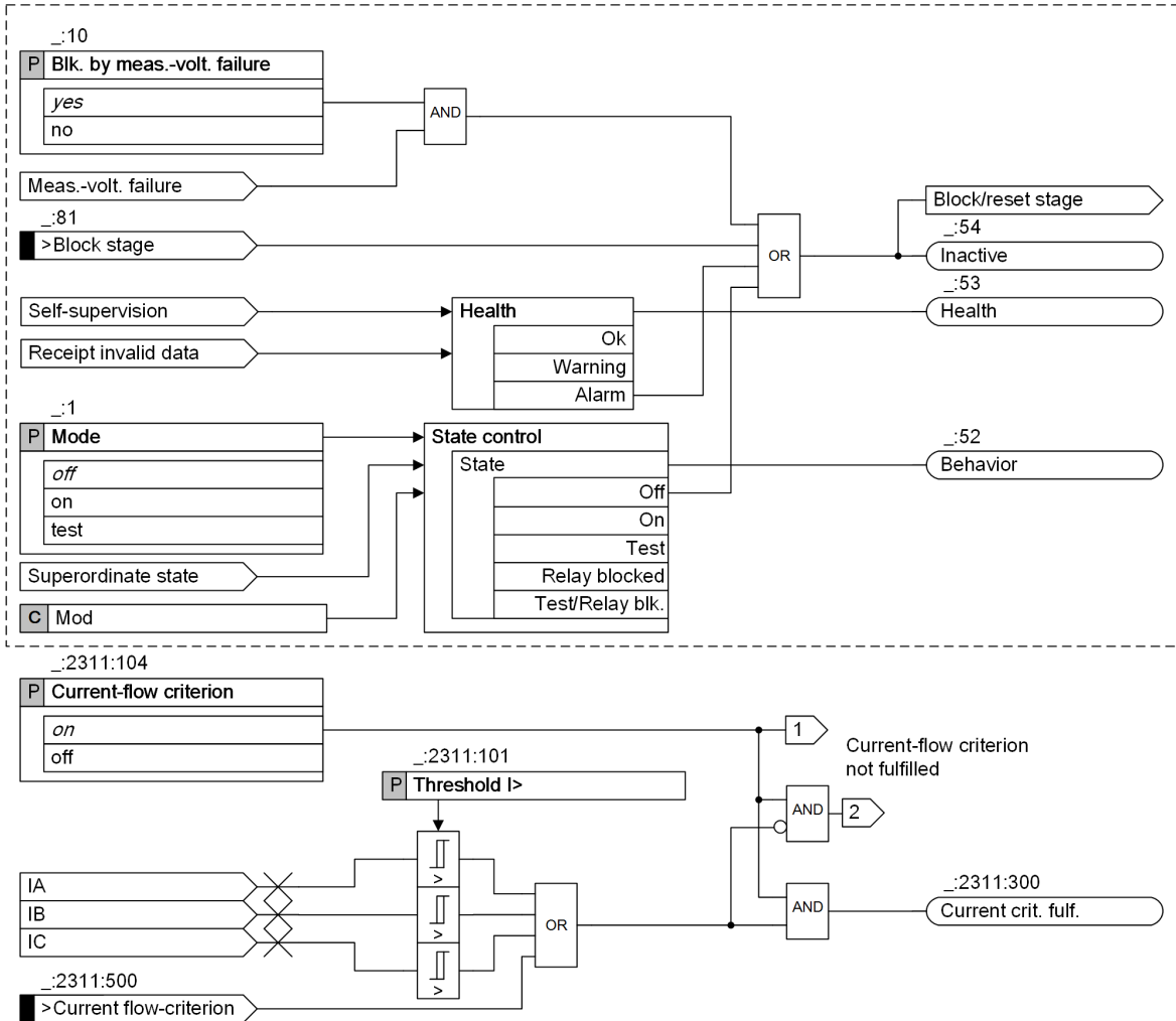
Figure 6-200 Logic Diagram of the Stage Control
