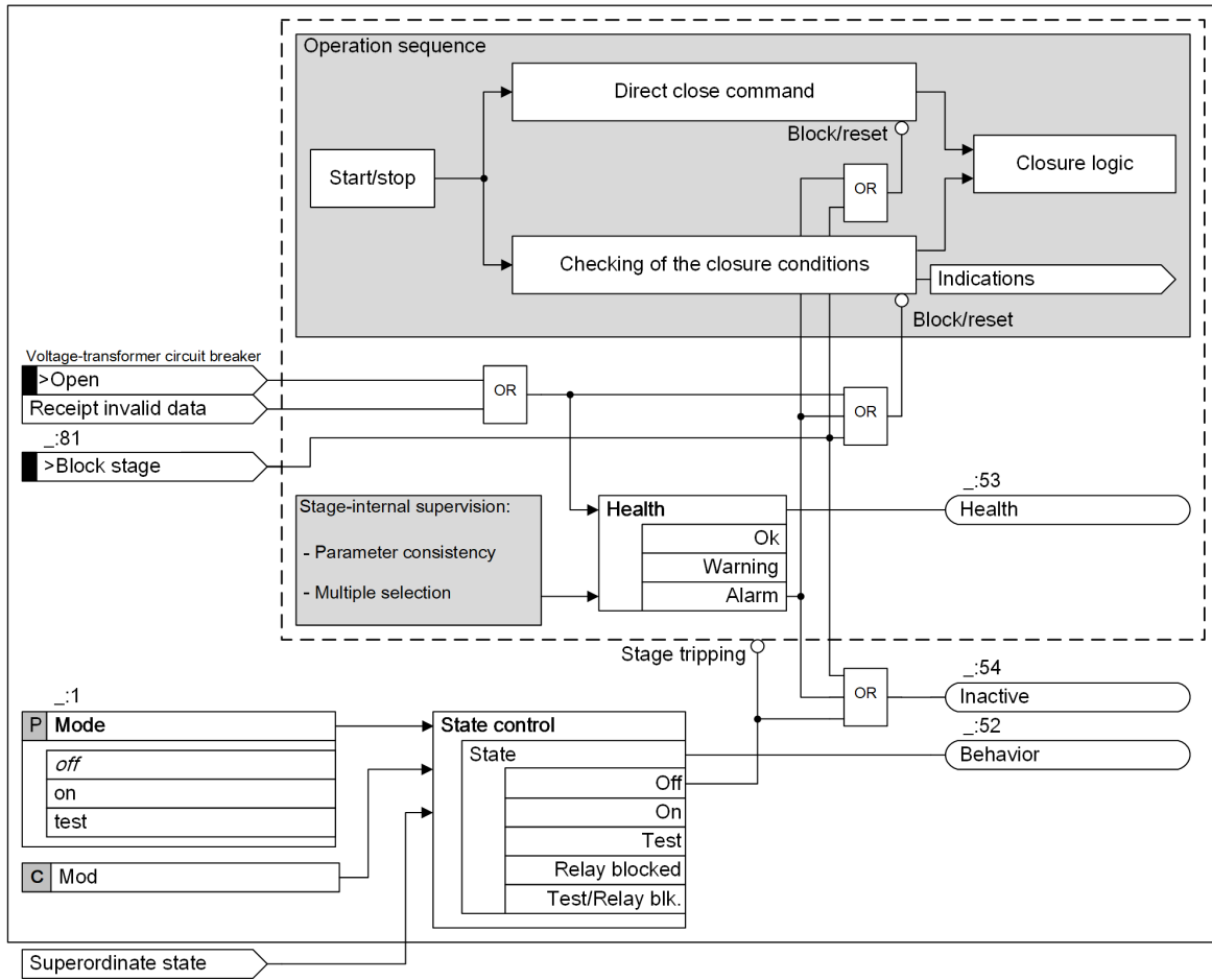
Figure 9-52 Overview of the Stage Logic
