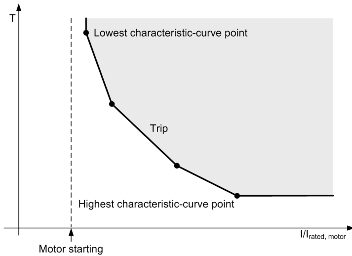
Figure 7-7 Example of User-Defined Characteristic Curve
