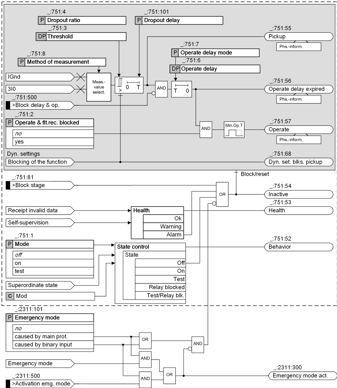
Figure 6-31 Logic Diagram Definite-Time Overcurrent Protection (Ground) – Advanced
