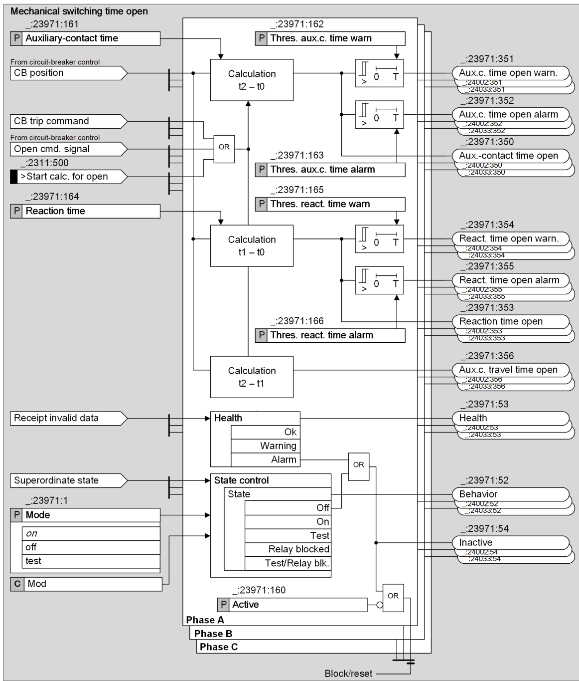
Figure 11-19 Logic of the Stage Mechanical Switching Time Open for Circuit Breakers 1-Pole
