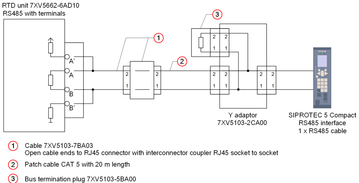
Figure 5-65 Connection of the RTD Unit to the SIPROTEC 5 Compact Device
