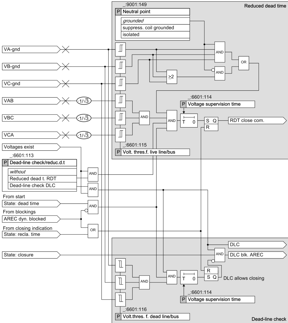
Figure 6-317 Cyclic Reclosing Function: Logic for the Functions of Reduced Dead Time and Dead-Line Check
