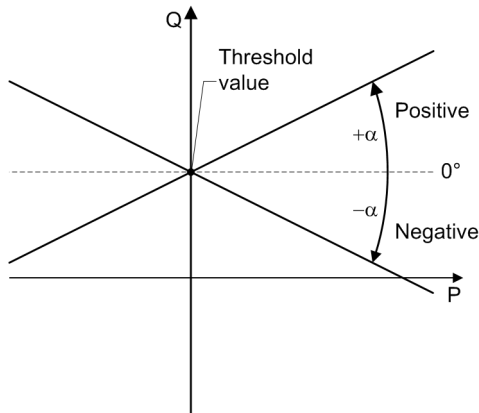
Figure 6-234 Tilt-Power Characteristic
