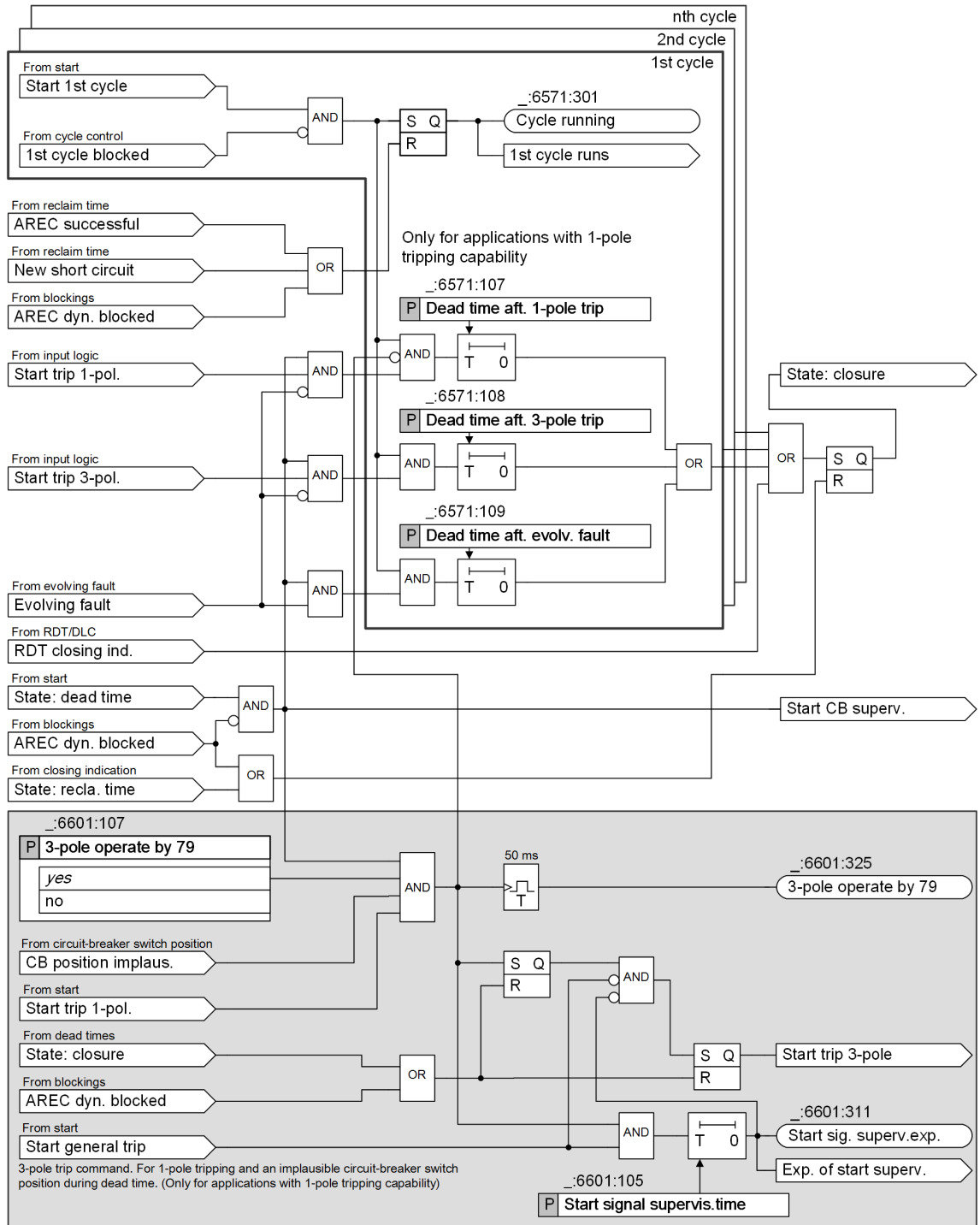
Figure 6-306 Cyclic Automatic Reclosing Function – Logic of the Dead Time for the Operating Modes: With Tripping
