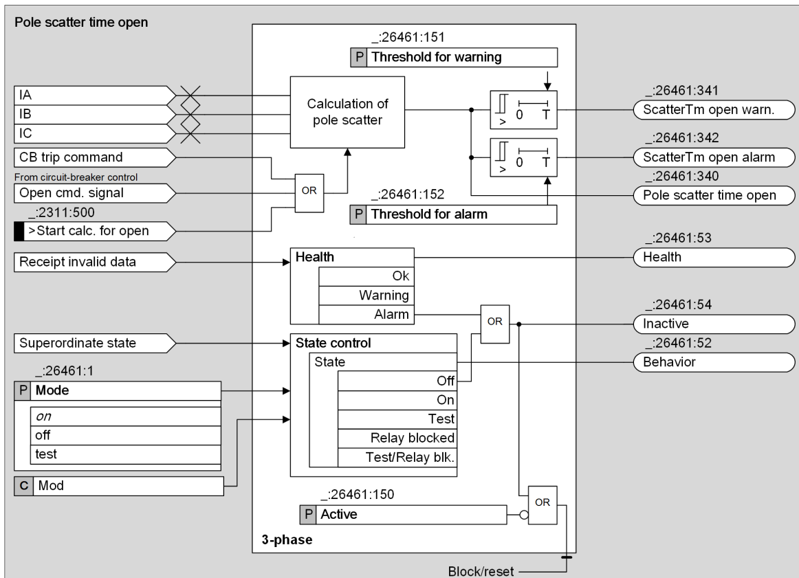
Figure 11-16 Logic of the Stage Pole Scatter Time Open
