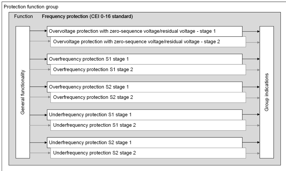
Figure 6-356 Structure/Embedding of the Function
