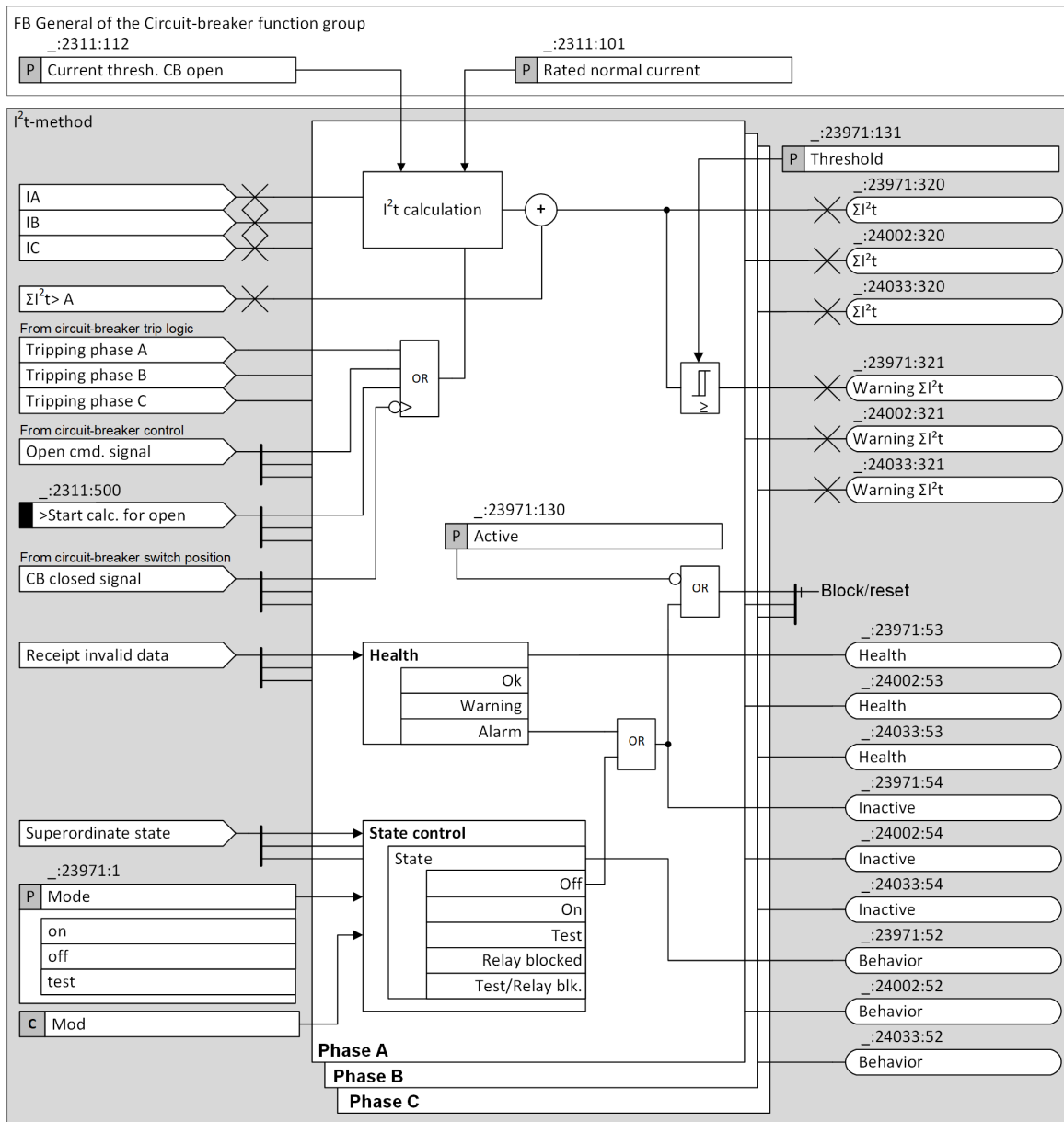
Figure 11-13 Logic of the I 2 t Method
