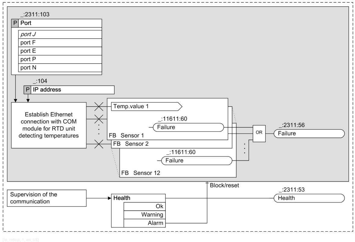
Figure 5-62 Logic of the RTD Unit Ether. Function
