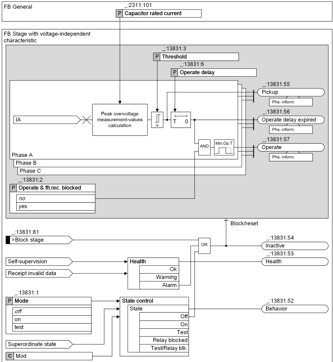
Figure 8-15 Logic Diagram of the Stage with Definite-Time Characteristic Curve
