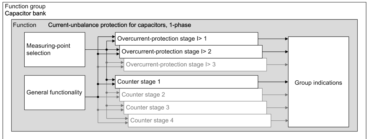
Figure 8-1 Structure/Embedding of the Function
