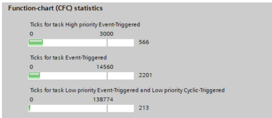
Figure 10-3 CFC Statistics
