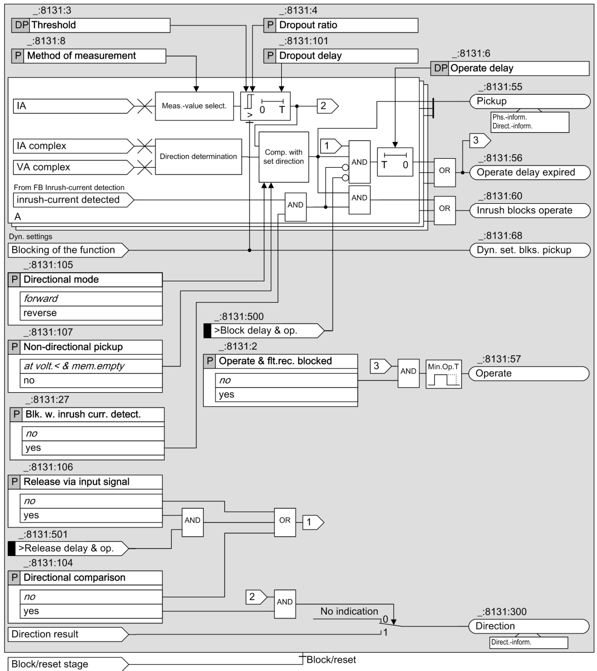
Figure 6-41 Logic Diagram of the Directional, Definite-Time Overcurrent Protection, Phases - Advanced
