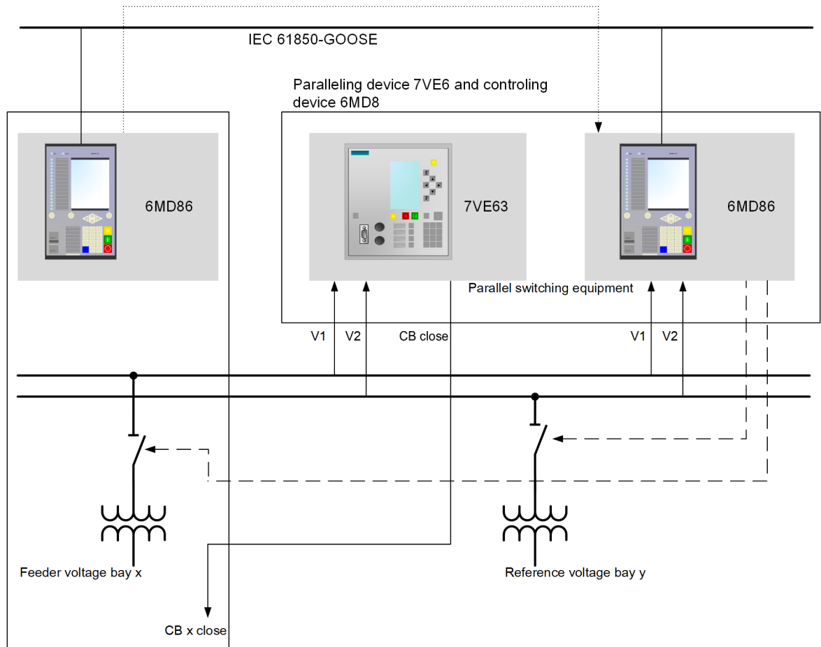
Figure 9-81 Triggering an External Synchronization Device
