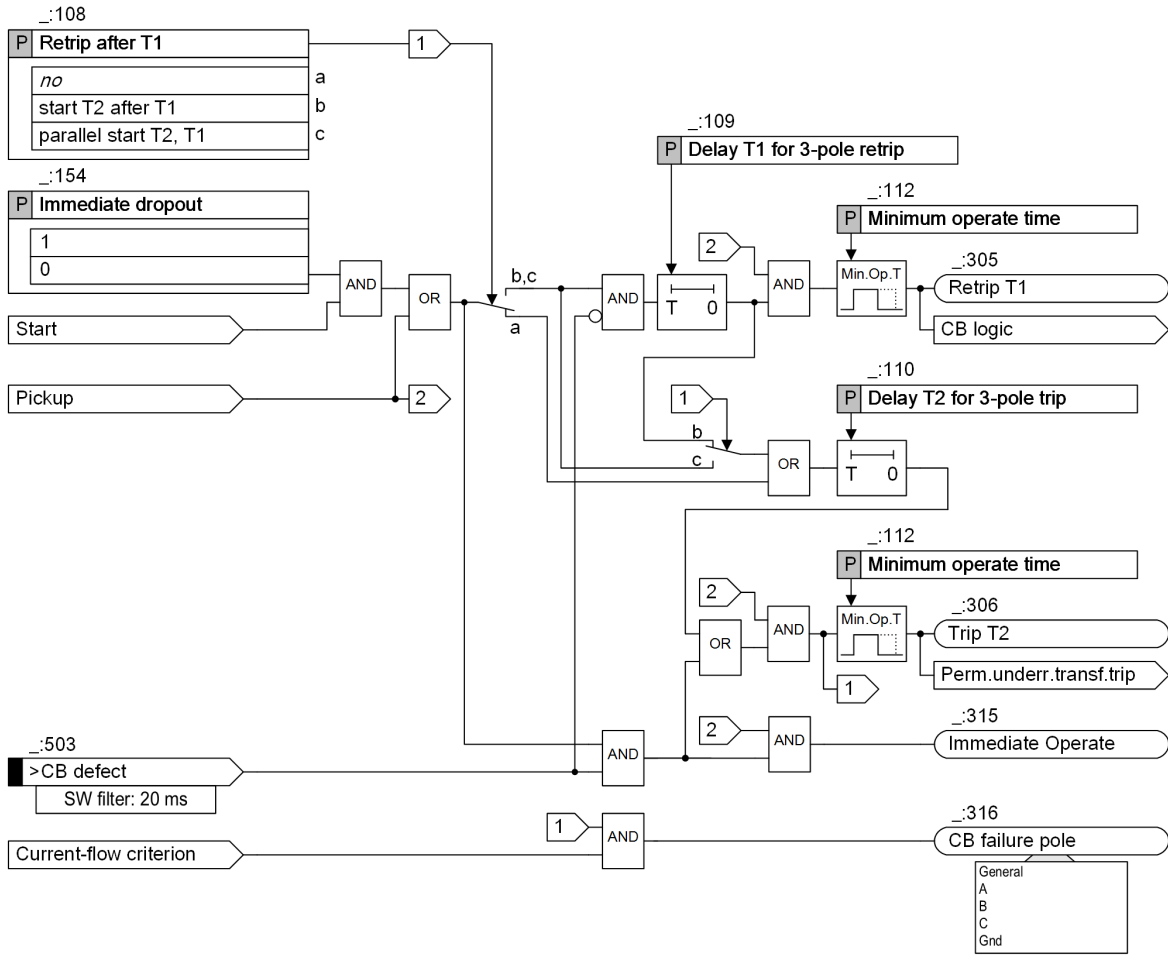
Figure 6-255 Delay/Tripping of the Circuit-Breaker Failure Protection Function
