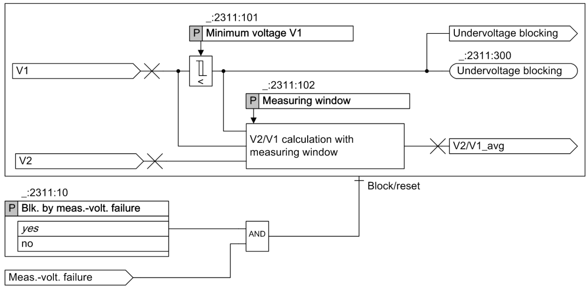
Figure 6-193 Logic Diagram of the General Functionality
