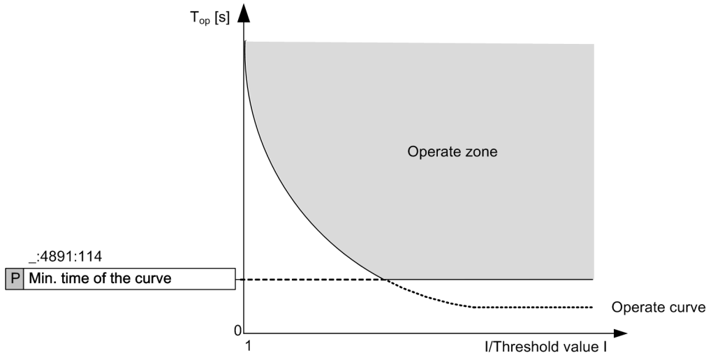
[dw_min_time_1_en_US] Figure 6-63 Minimum Operating Time of the Curve
