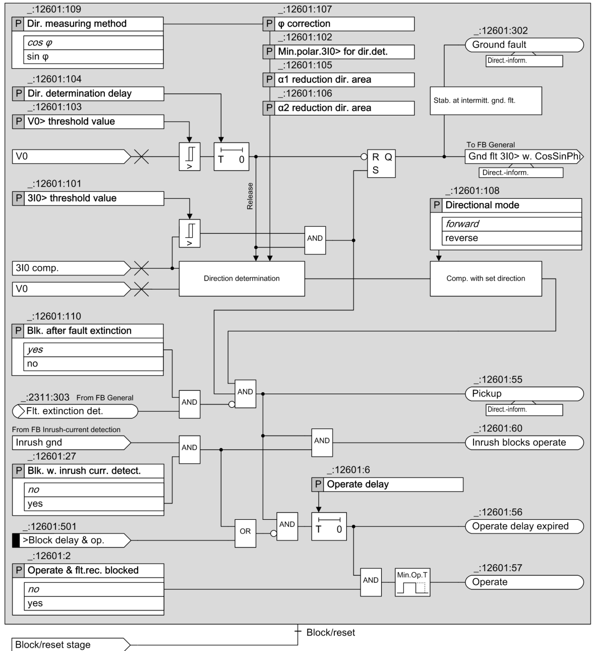
Figure 6-120 Logic Diagram of the Directional 3I0 Stage with Cos φ or Sin φ Measurement
