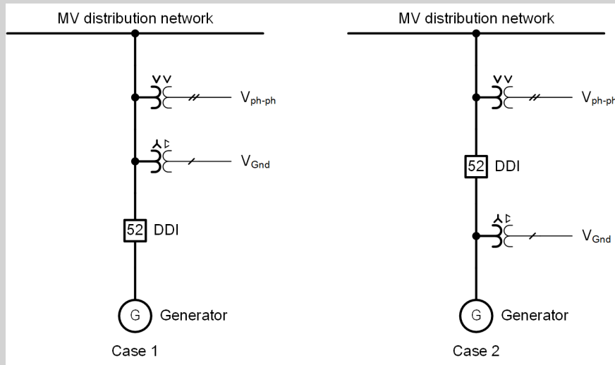
Figure 6-360 Application Example of Voltage-Transformer Positions: Case 1 and Case 2
