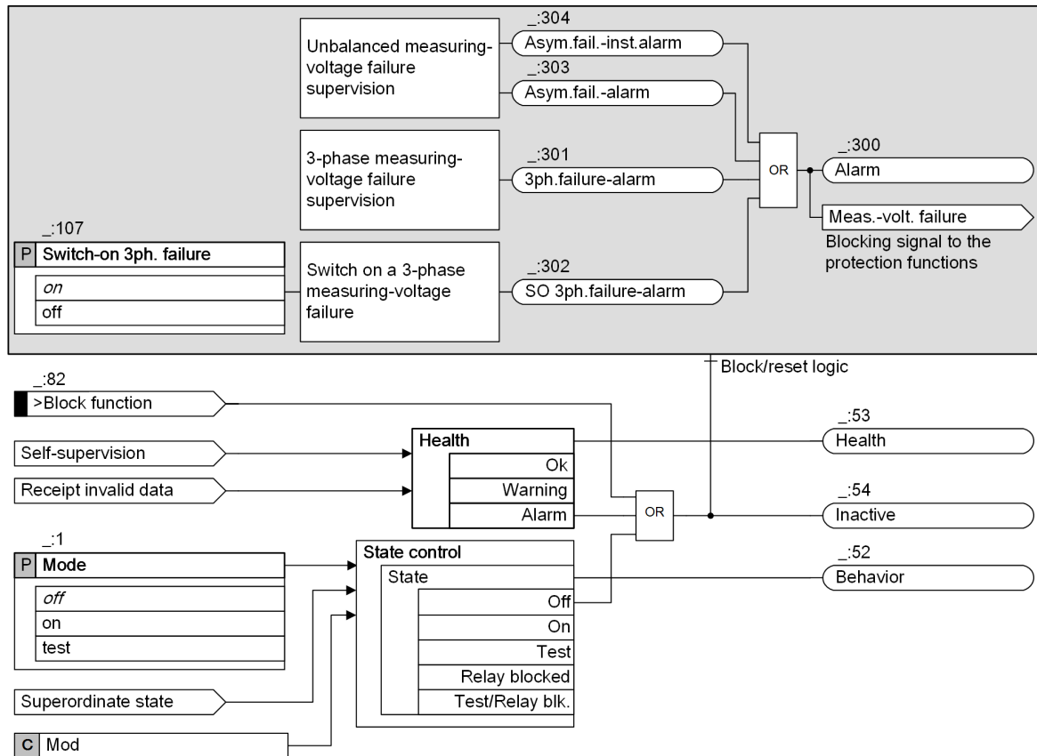
Figure 10-5 Breakdown of the Measuring-Voltage Failure Detection Function
