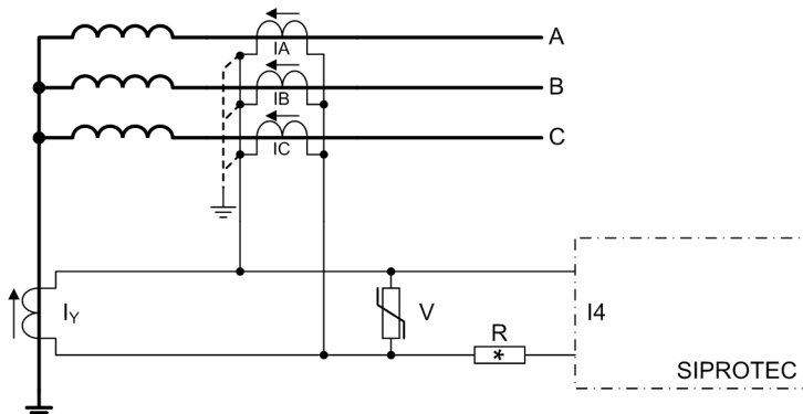
Figure 6-95 Connection Diagram of the Restricted Ground-Fault Protection According to the High-Impedance Principle
