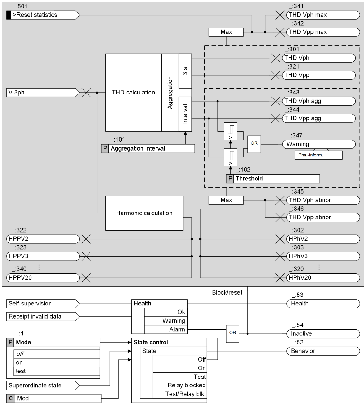
Figure 12-15 Logic Diagram of the stage Voltage
