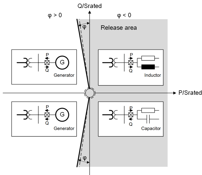
Figure 6-217 Power-Criterion Checking at \Phi (power criterion) > 0 (according to VDE-AR-N 4142:2020-04)
