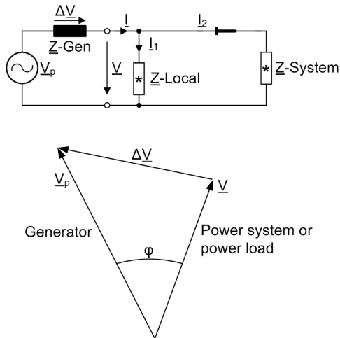
Figure 6-224 Voltage Vector of the Steady State
