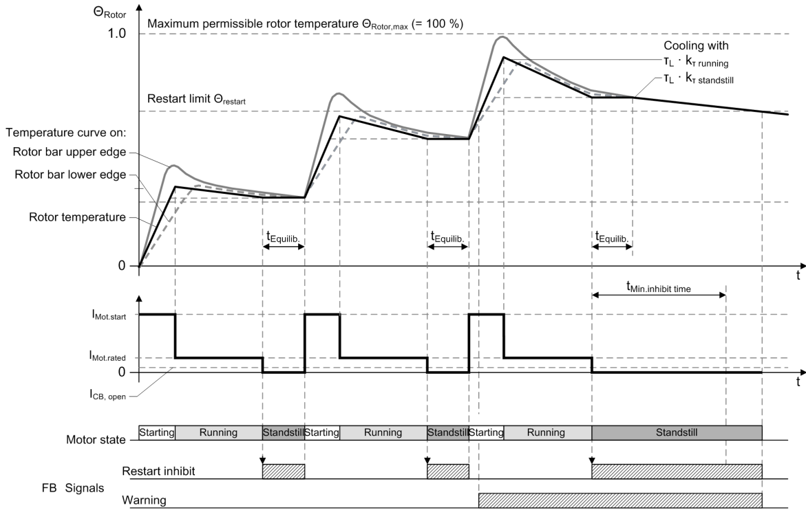
Figure 7-10 Rotor-Temperature Curve and Repeated Motor-Starting Attempts
