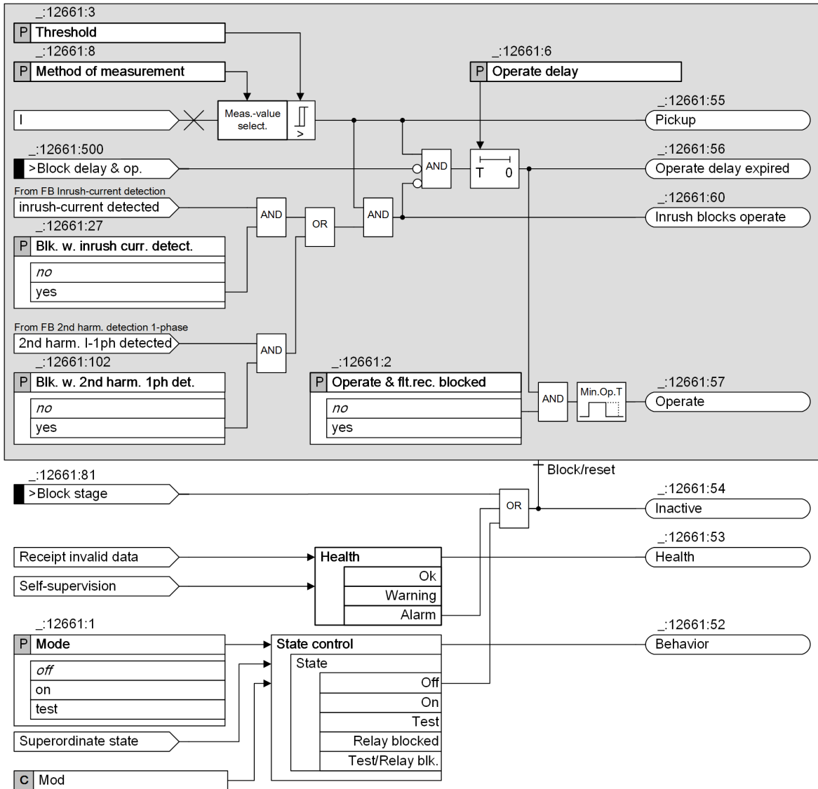
Figure 6-86 Logic Diagram of the Definite-Time Overcurrent Protection, 1-Phase
