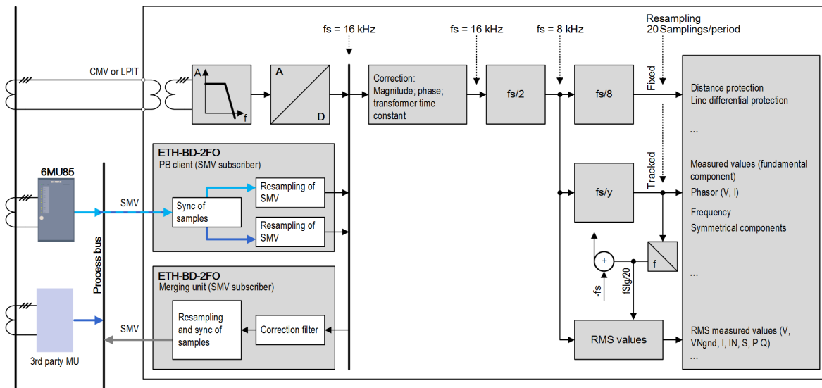
Figure 3-30 Measured-Value Acquisition Chain
