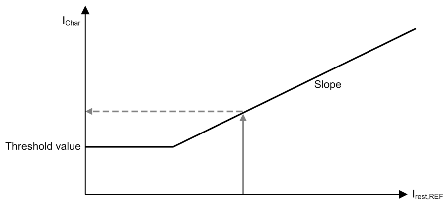
Figure 6-266 Stabilized Characteristic Curve
