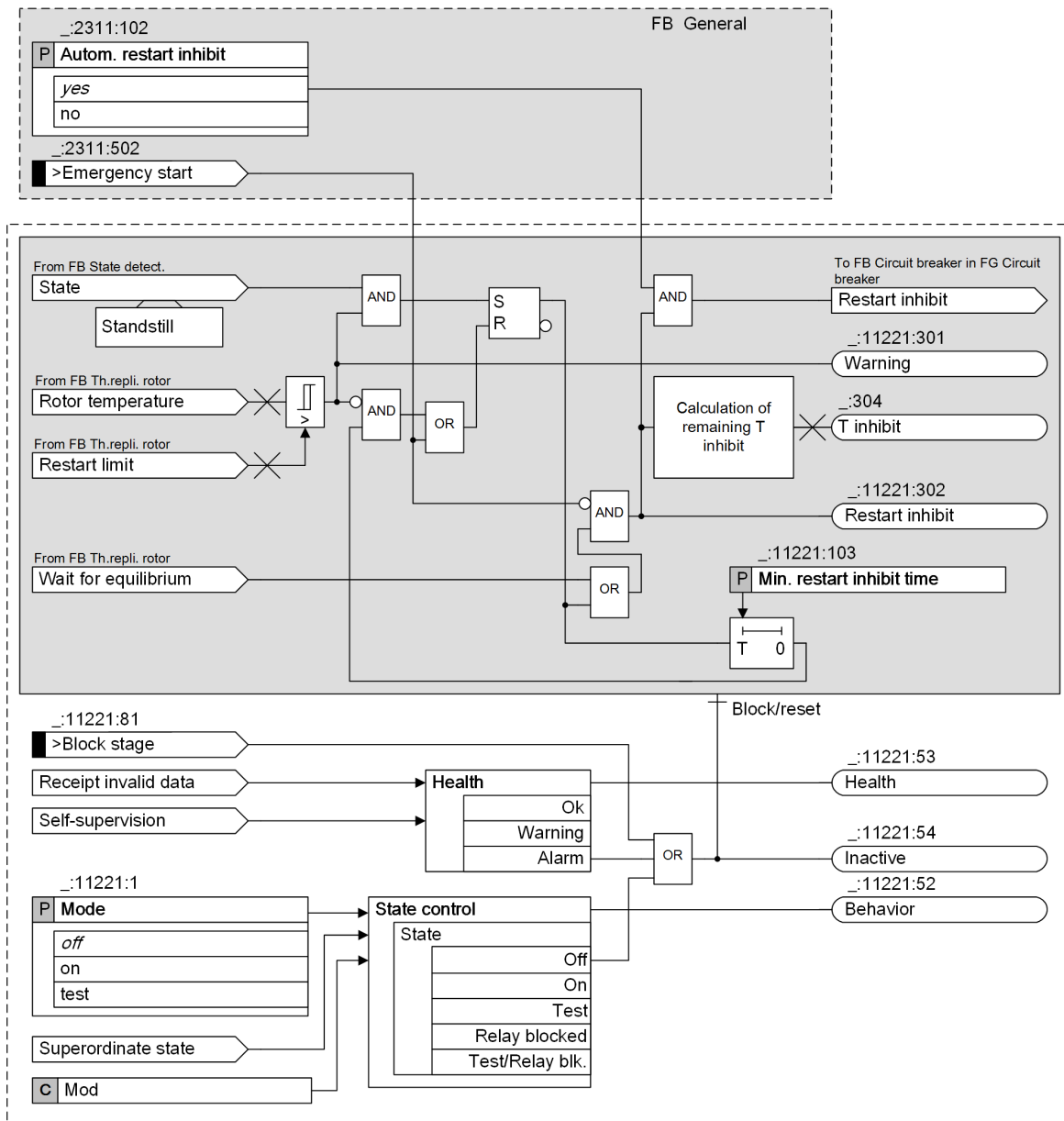
Figure 7-9 Logic Diagram of the Thermal Stage
