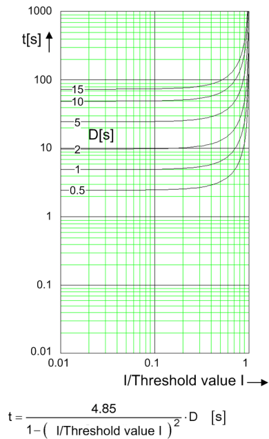
Figure 14-5 Operate Curves and Dropout-Time Characteristic Curves According to ANSI/IEEE
