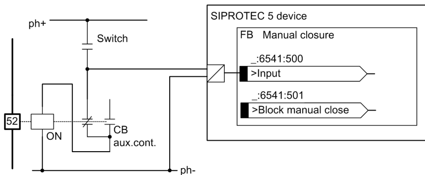
Figure 5-136 Connection of the Input Signal to the Control Circuit of the Circuit-Breaker Closing Coil
