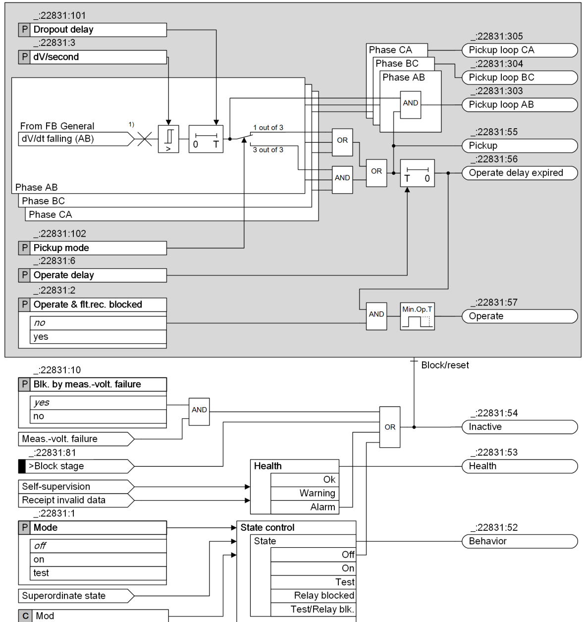
Figure 6-209 Logic Diagram of the dV/dt Falling Stage
