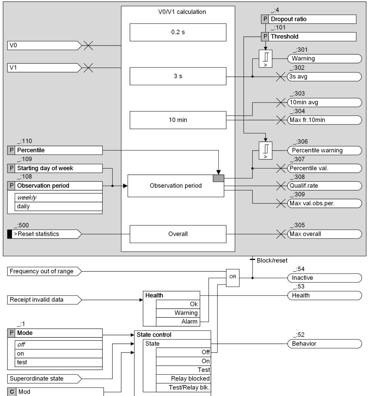
Figure 12-13 Logic Diagram of the Stage V0/V1
