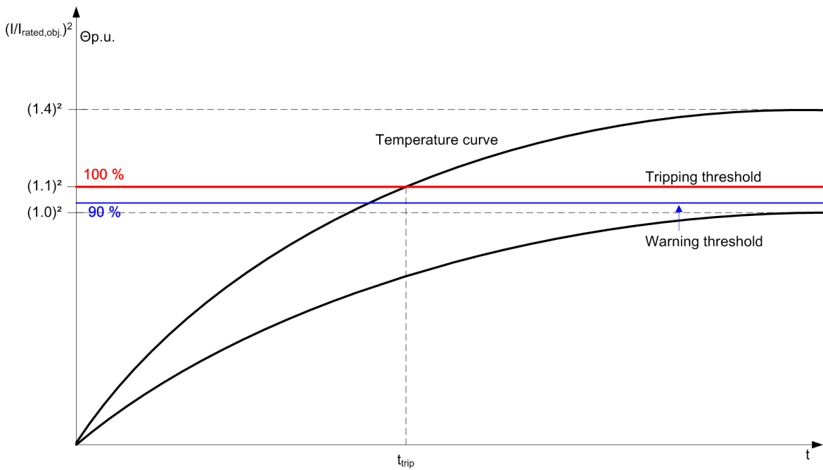
Figure 6-168 Temperature History for Different Overload Currents ( K-factor = 1.1 )
