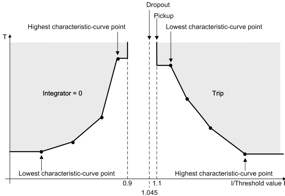
Figure 6-35 Pickup Behavior and Dropout Behavior when Using a User-Defined Characteristic Curve
