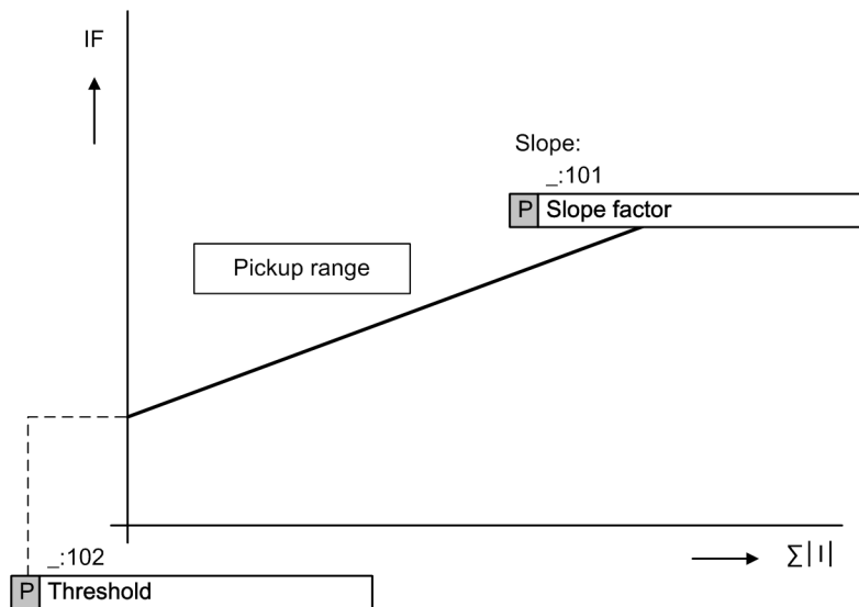
Figure 10-32 Characteristic of the Current-Sum Supervision
