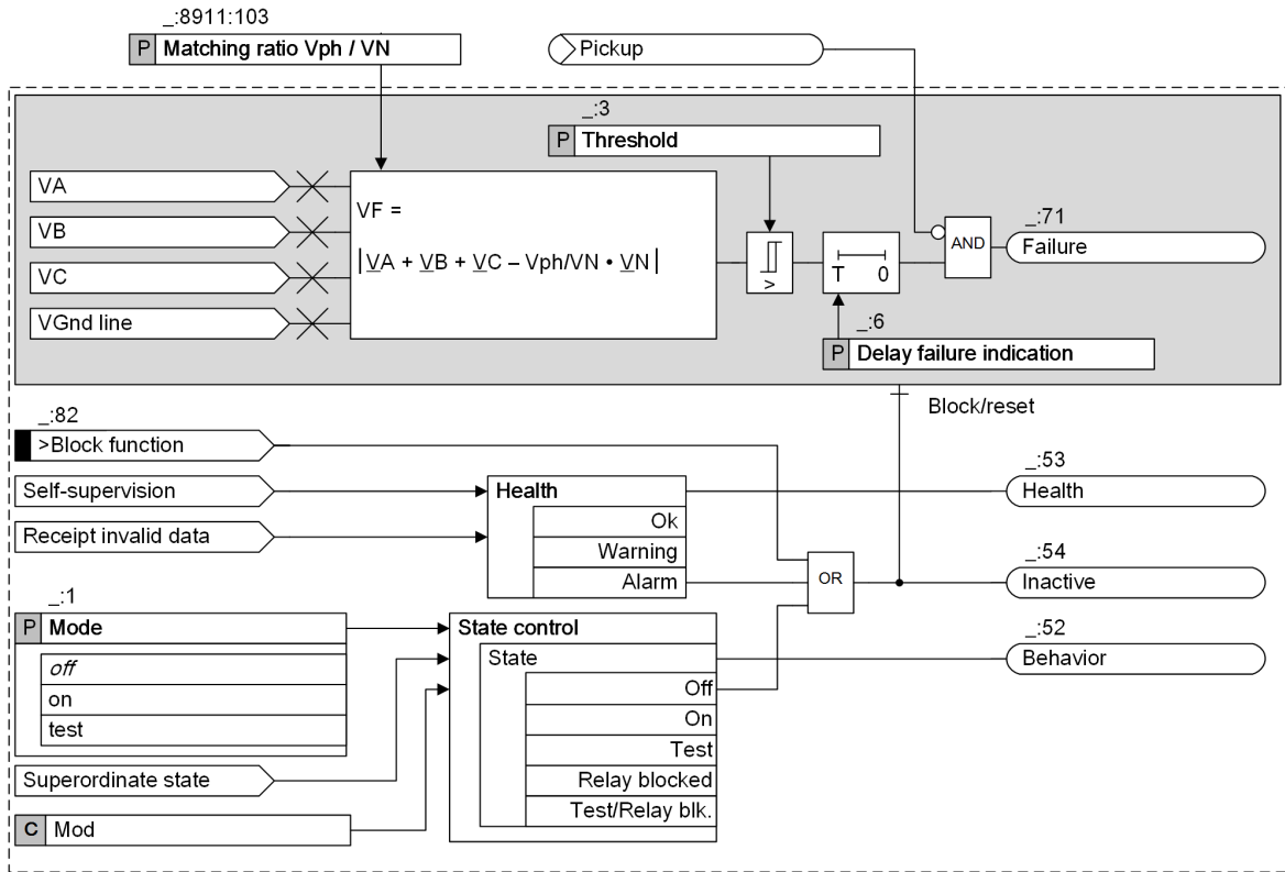
Figure 10-20 Logic Diagram of the Voltage-Sum Supervision
