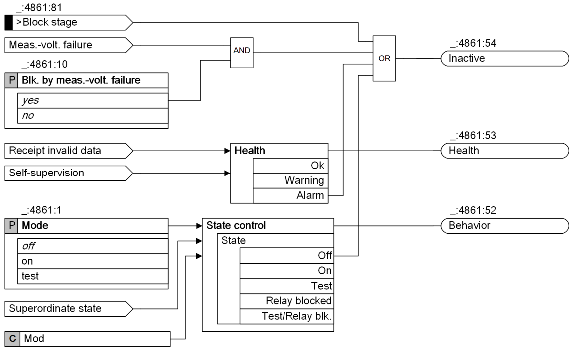
Figure 6-58 Logic Diagram of the Stage Control
