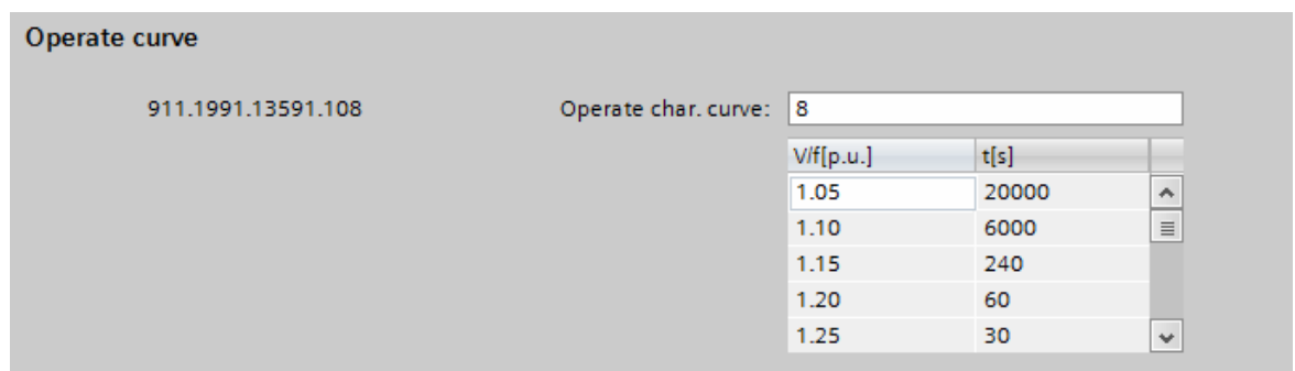
Figure 6-240 Data Sheet for Adjustment of Thermal Characteristic Curve
