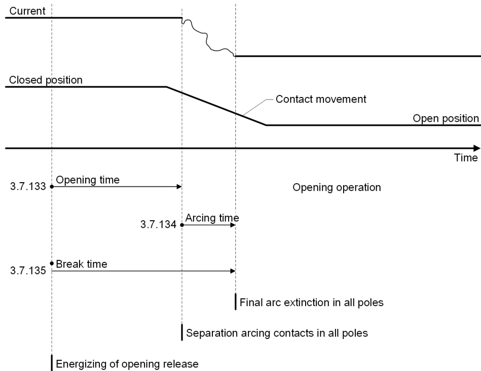
Figure 11-7 Circuit-Breaker Times
