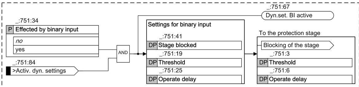
Figure 6-38 Influence of the Binary Input on the Overcurrent-Protection Stage
