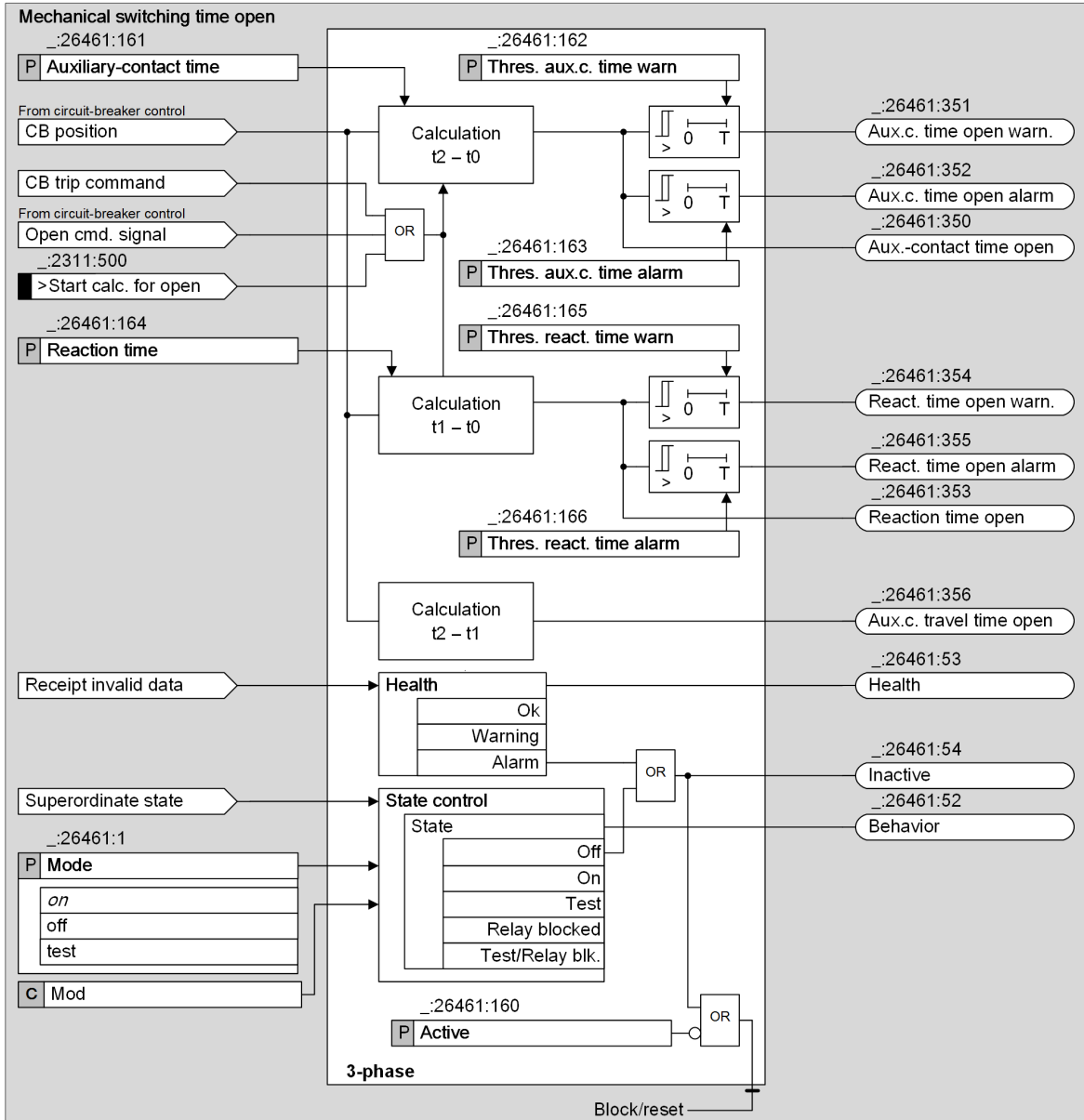
Figure 11-18 Logic of the Stage Mechanical Switching Time Open for Circuit Breakers 3-Pole
