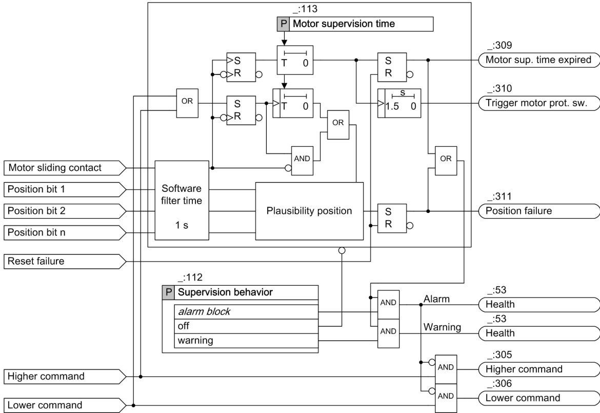
Figure 9-97 Position and Motor Supervision Logic
