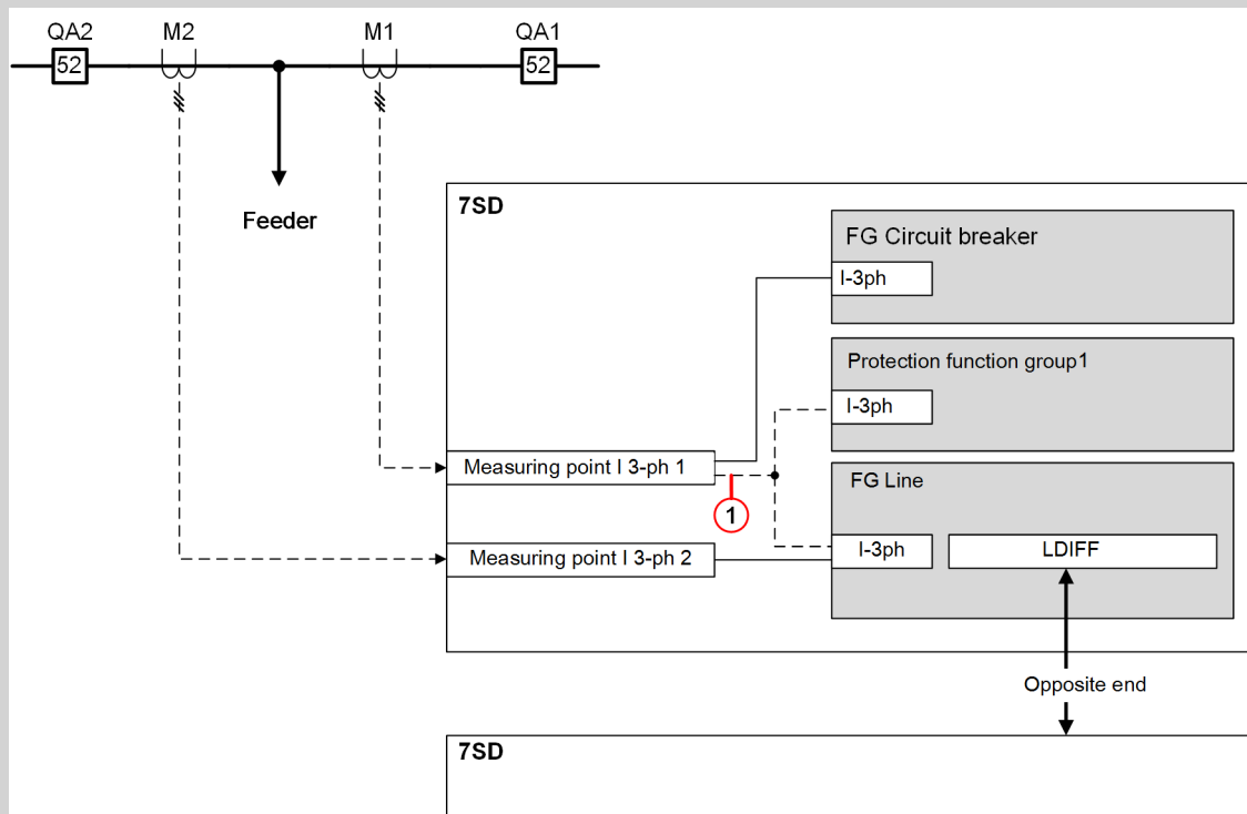
Figure 6-5 Possible Disconnection of Measuring Point for the Line Differential Protection
