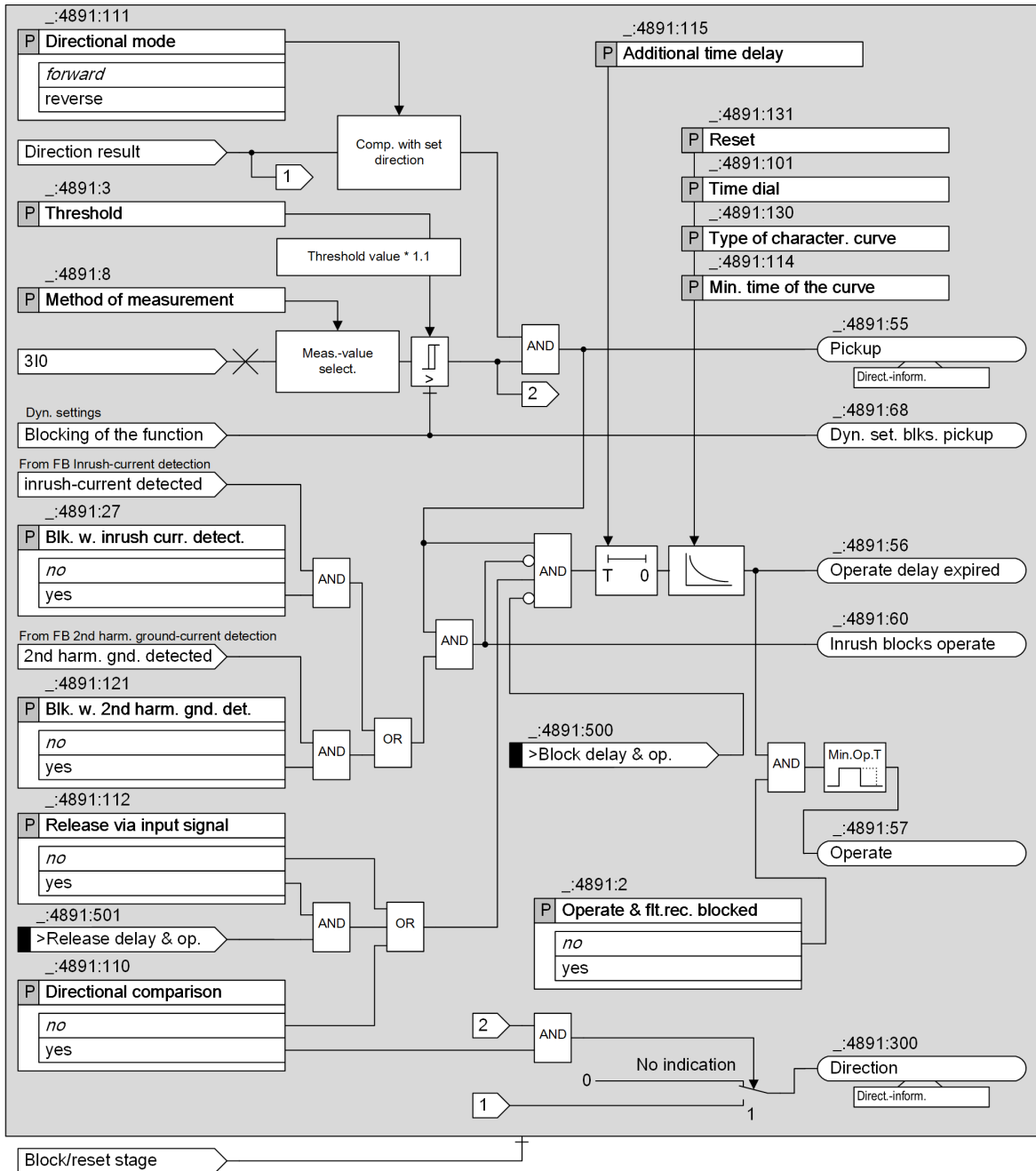
Figure 6-62 Logic Diagram of the Directional Inverse-Time Overcurrent Protection, Ground – Advanced
