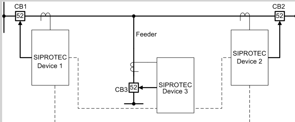
Figure 3-64 Differential Protection with 3 Devices for a Line with a Feeder
