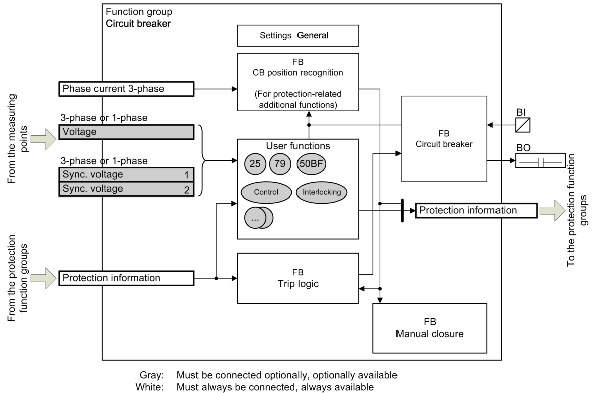
Figure 5-107 Structure of the Circuit-Breaker Function Group
