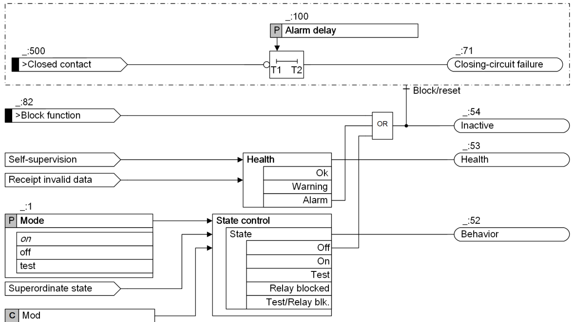
Figure 10-48 Logic Diagram of the Stage Closing-Circuit Supervision with 1 Binary Input
