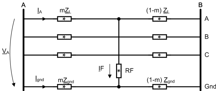
Figure 6-327 Short Circuit of a Phase-to-Ground Loop
