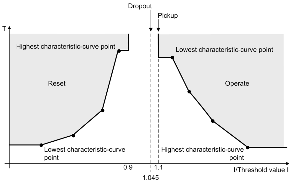
Figure 6-69 Pickup and Dropout Behaviors when Using a User-Defined Characteristic Curve
