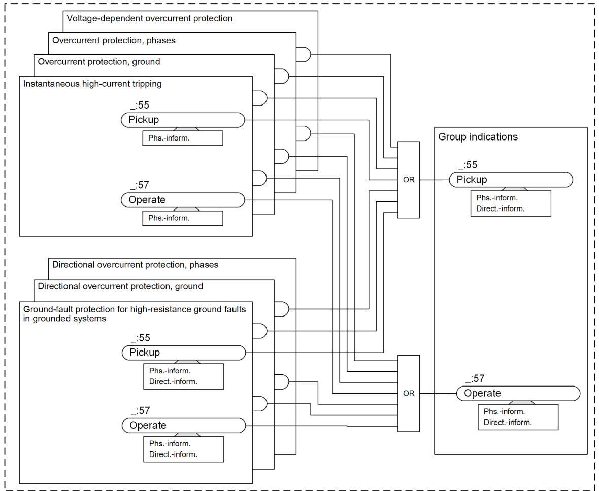
Figure 6-7 Logic Diagram of the Overcurrent Protection Group Indications
