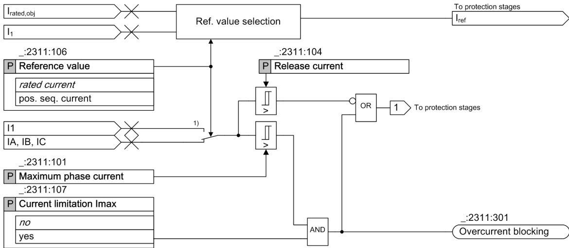
Figure 6-150 Logic Diagram of the General Functionality
