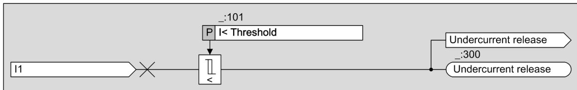
Figure 6-228 Logic Diagram of the I1 < Release Stage
