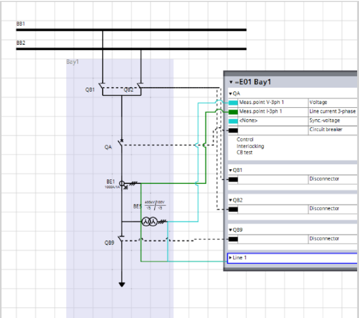
Figure 9-35 Feeder Bay for a Double Busbar System
