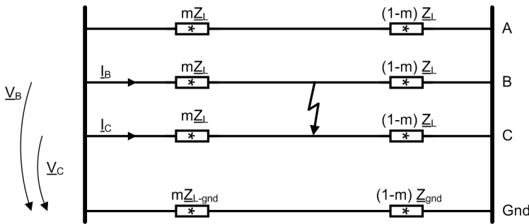
Figure 6-324 Short Circuit of a Phase-to-Phase Loop
