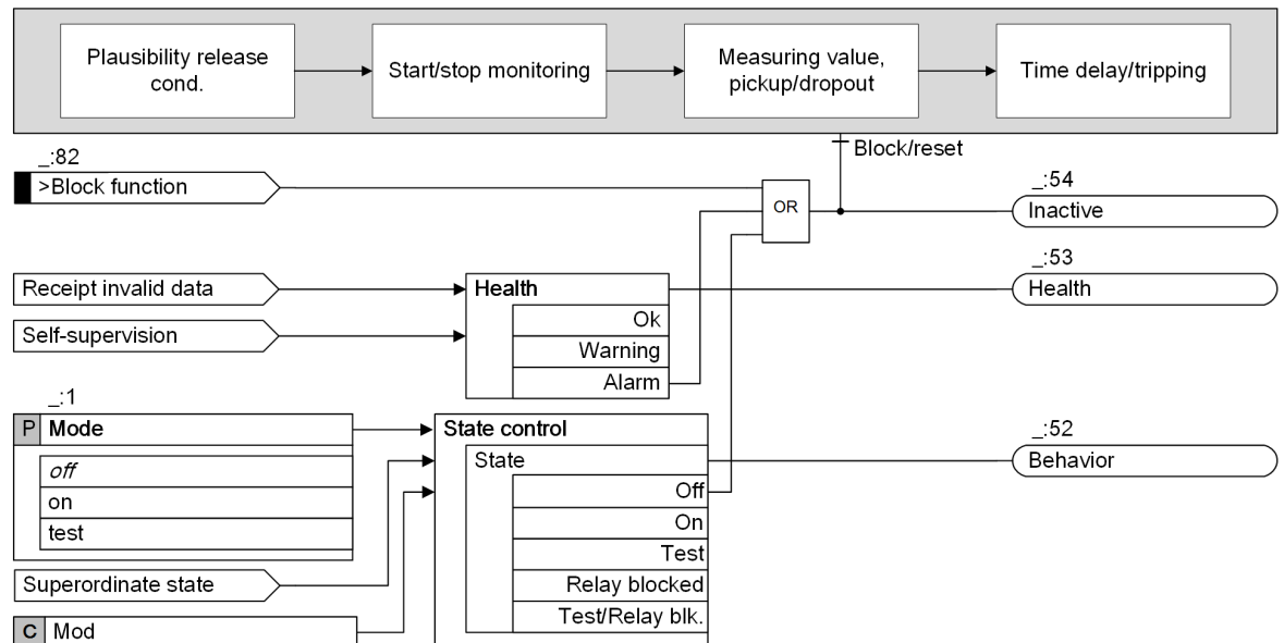
Figure 6-258 Logic Overview of the Function
