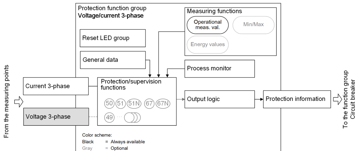
Figure 5-1 Structure of the Voltage-Current 3-Phase Function Group
