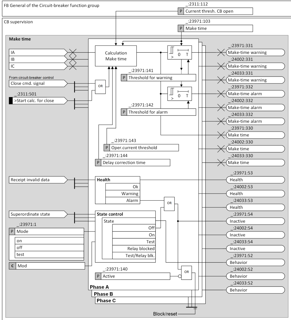
Figure 11-14 Logic of the Make Time
