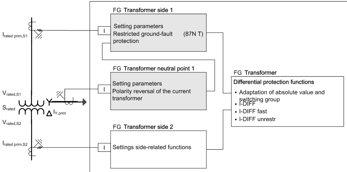
Figure 6-271 Function Group Structure of the Restricted Ground-Fault Protection
