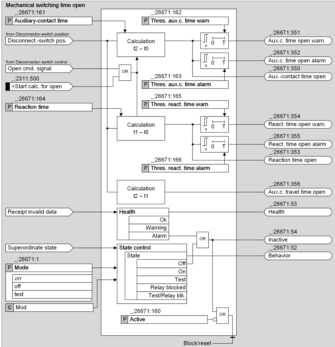
Figure 11-22 Logic of the Stage Mechanical Switching Time for Disconnecter
