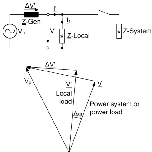
Figure 6-225 Vector Change after the Load Shedding
