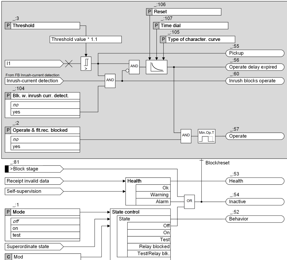
Figure 6-102 Logic Diagram of the Inverse-Time Positive-Sequence Overcurrent Protection
