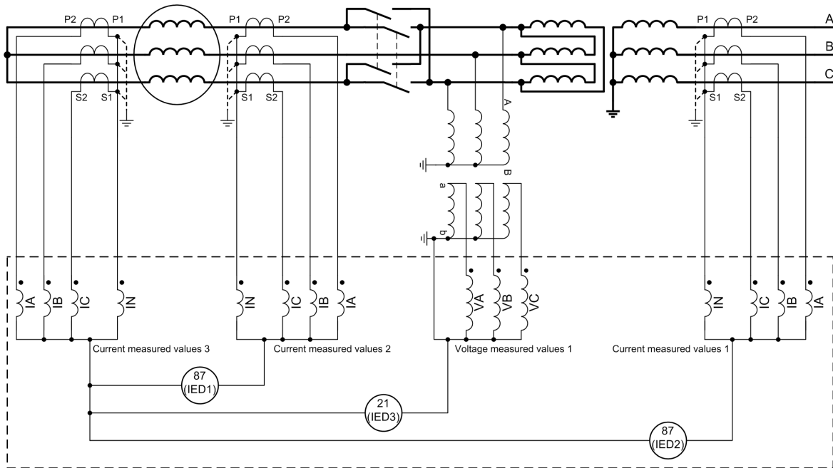
[ldw_phrrapp, 2, en_US] Figure 6-343 Application Example for Phase-Rotation Reversal in a Pump Station
