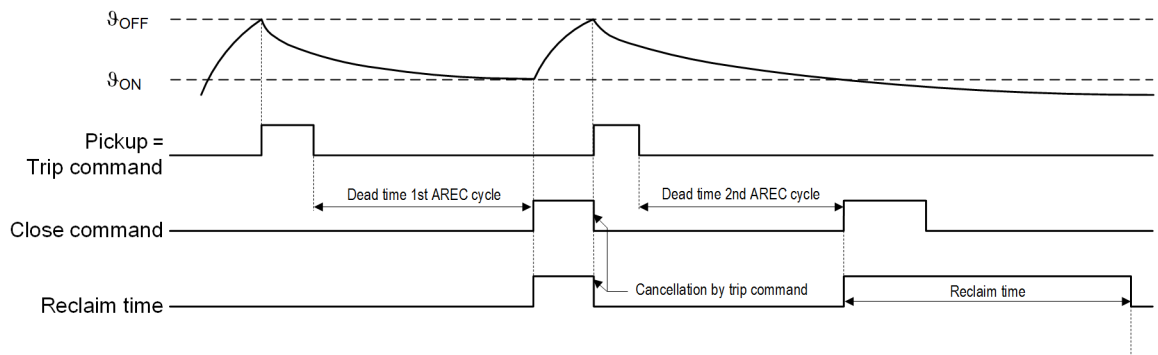
Figure 6-284 Process Diagram of a Two-Time Reclosing after Disconnection via Overload Protection
