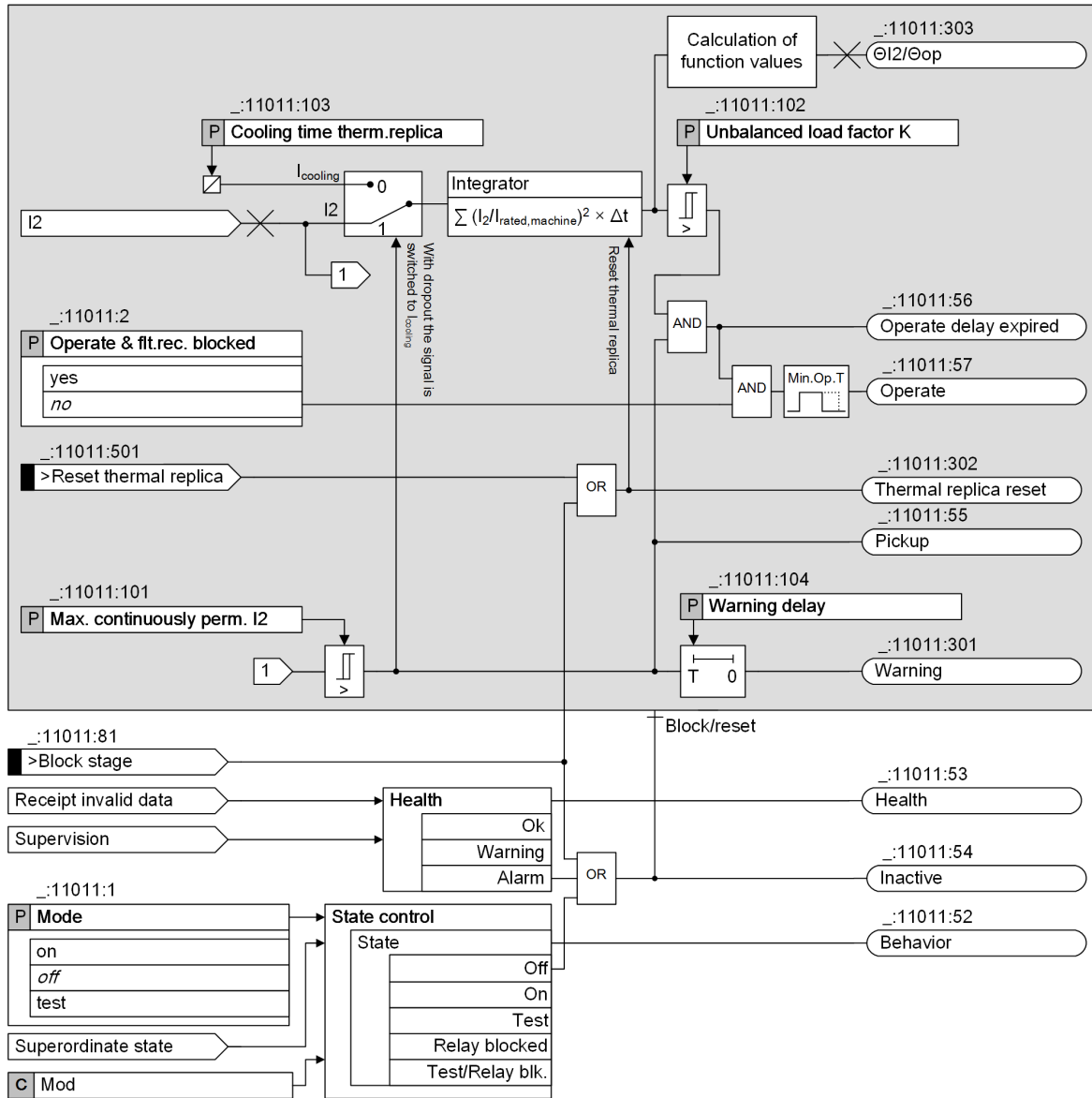
Figure 6-174 Logic Diagram of the Unbalanced-Load Protection Function
