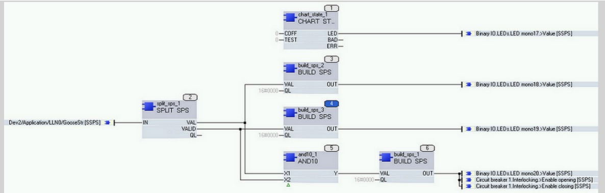
[sc_cfc_ran_1_en_US] Figure 3-41 CFC Chart with Building Blocks for Quality Processing (Switchgear Interlocking via GOOSE)
