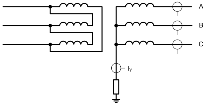
Figure 6-17 I0 Elimination Principle
