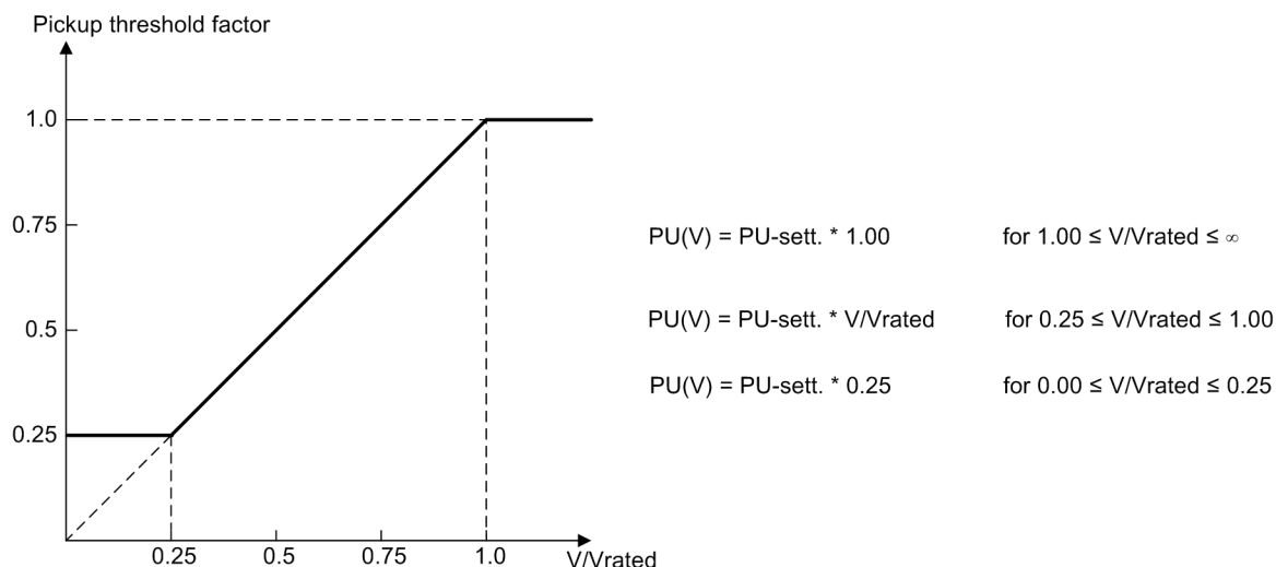
Figure 6-24 Voltage Influence of the Pickup Threshold
