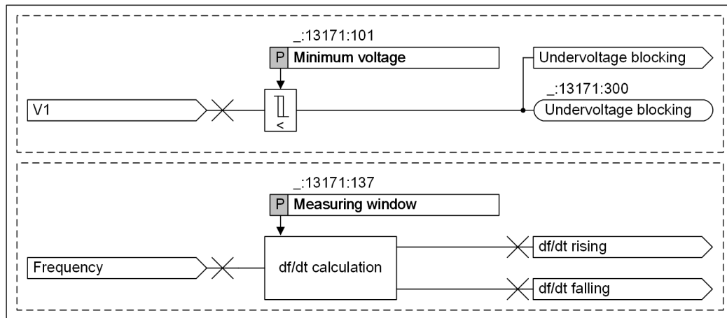
Figure 6-221 Logic Diagram of General Functionality
