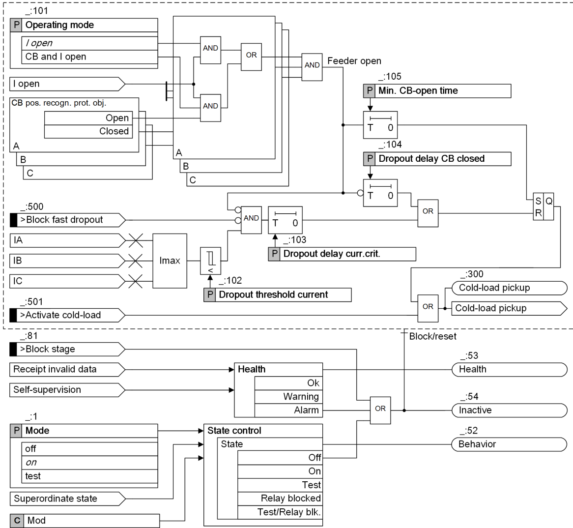
Figure 5-27 Logic Diagram of the Cold-Load Pickup Detection Function Block
