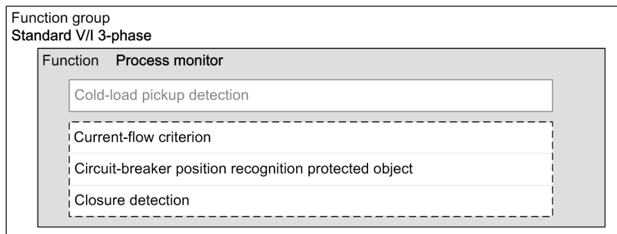
Figure 5-138 Structure/Embedding of the Function
