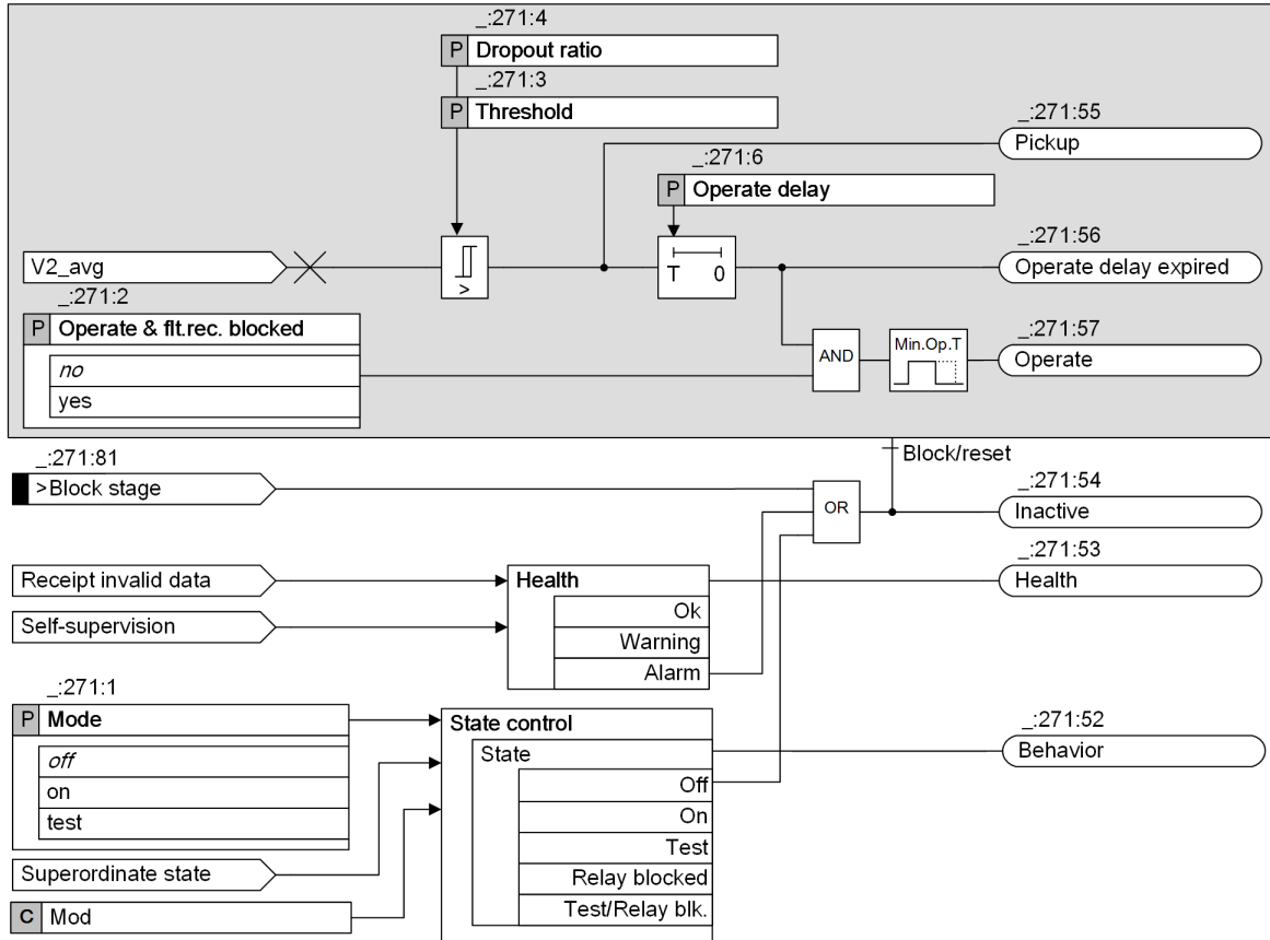
Figure 6-187 Logic Diagram of the Stage: Overvoltage Protection with Negative-Sequence Voltage
