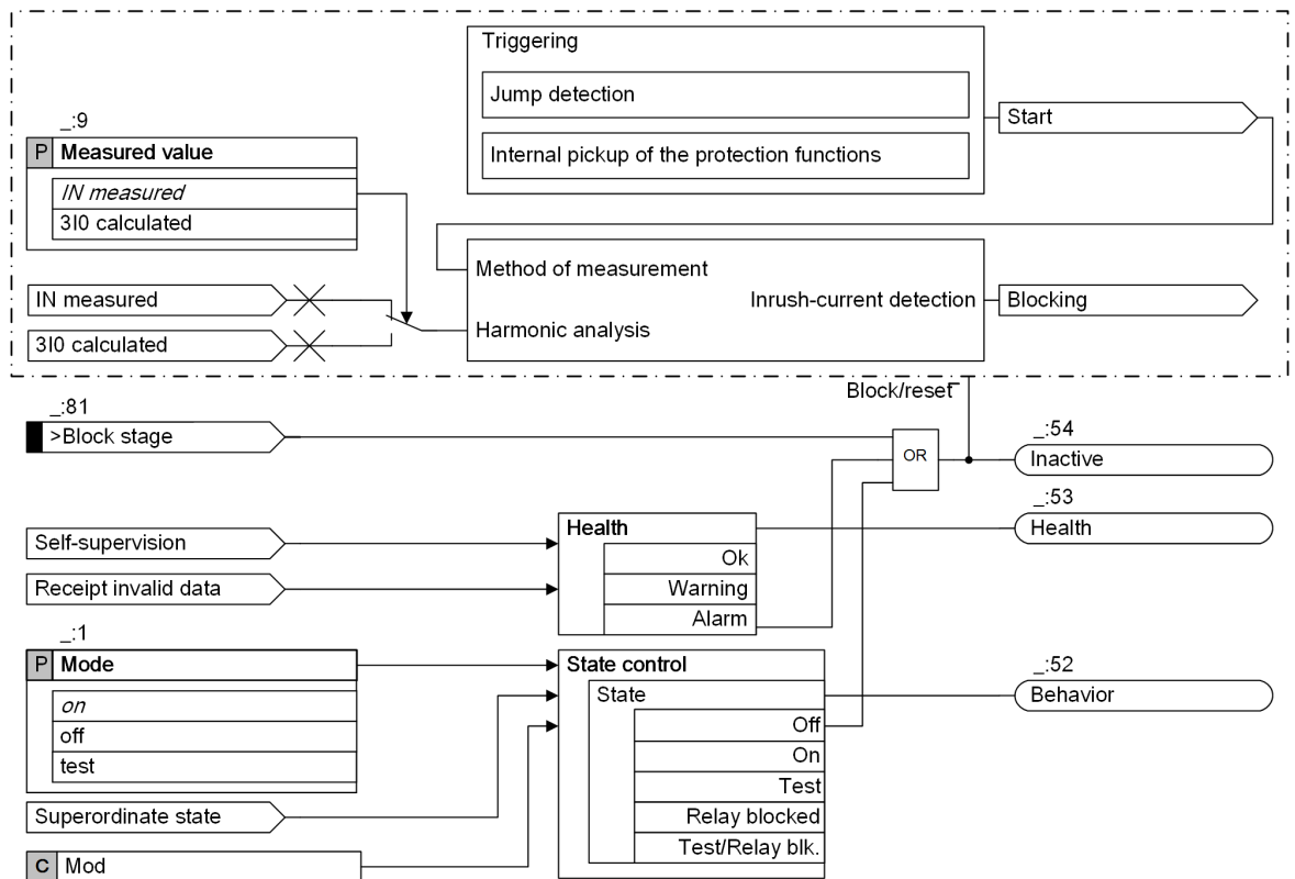
Figure 6-76 Logic of 2nd Harmonic Detection Ground
