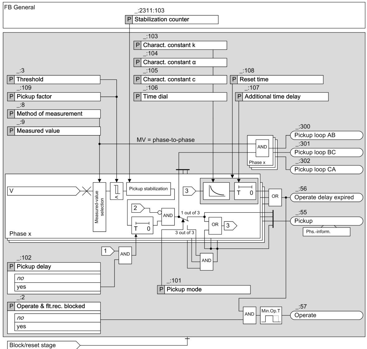
Figure 6-201 Logic Diagram of the Inverse-Time Undervoltage Protection with 3-Phase Voltage
