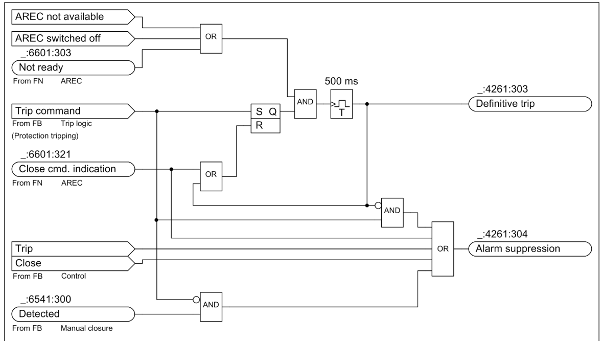
Figure 5-112 Definitive Tripping and Circuit-Breaker Tripping Alarm Suppression
