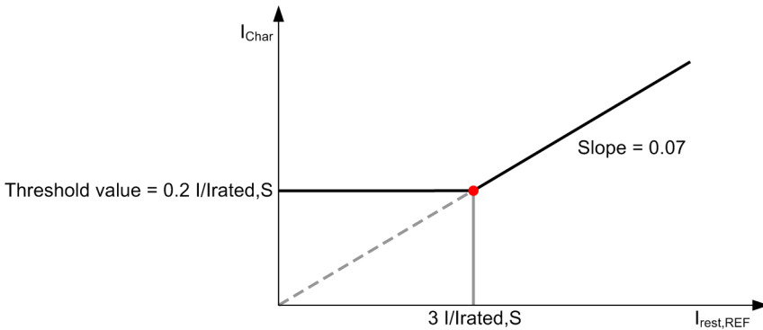
Figure 6-277 Derivation of the Setting Value for the Gradient
