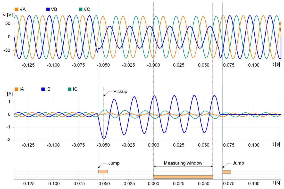
Figure 6-323 Determining the Measurement Window
