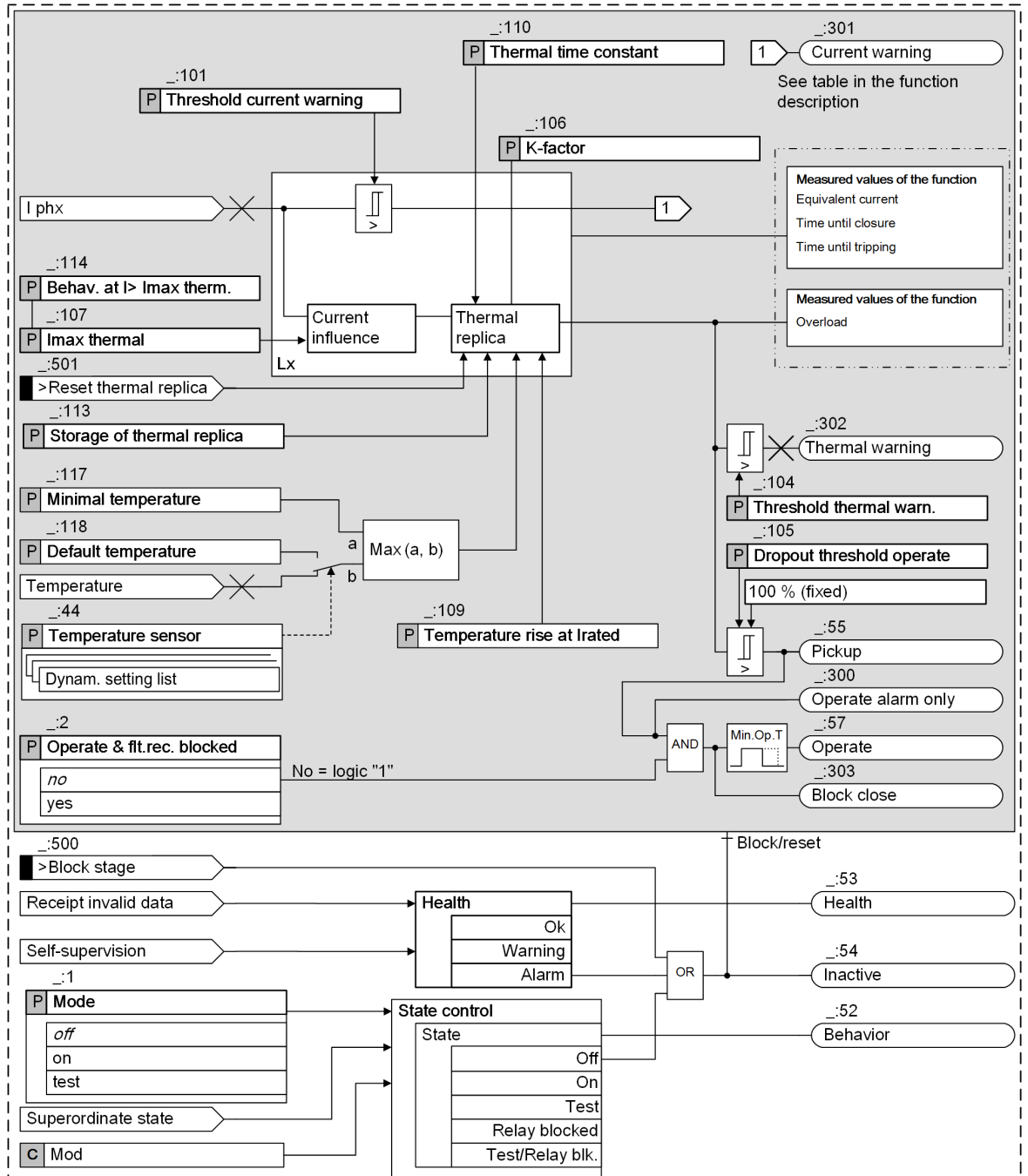
Figure 6-171 Logic Diagram of the Thermal Overload Protection Function
