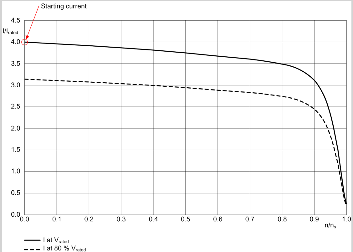
Figure 7-4 Starting-Data Diagram
