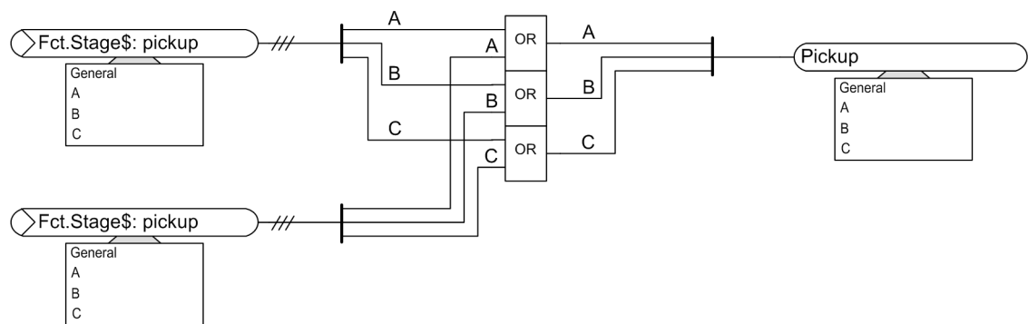
Figure 5-18 Generation of the Pickup Indication of the Motor Function Group
