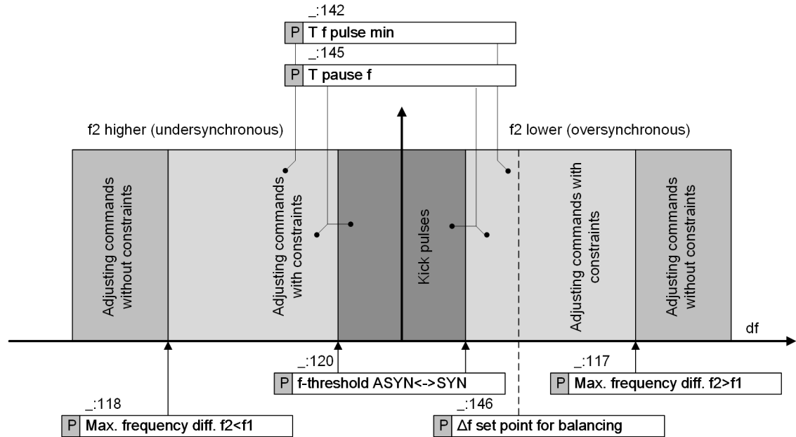
Figure 9-69 Kick Pulse and Frequency Adjustment Ranges
