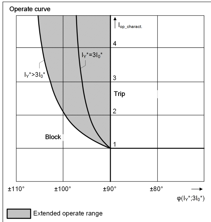
Figure 14-21 Restricted Ground-Fault Protection Operate Curve Depending on the Phase Angle between I_V^* and 3I_0^* with Extended Operate Range
