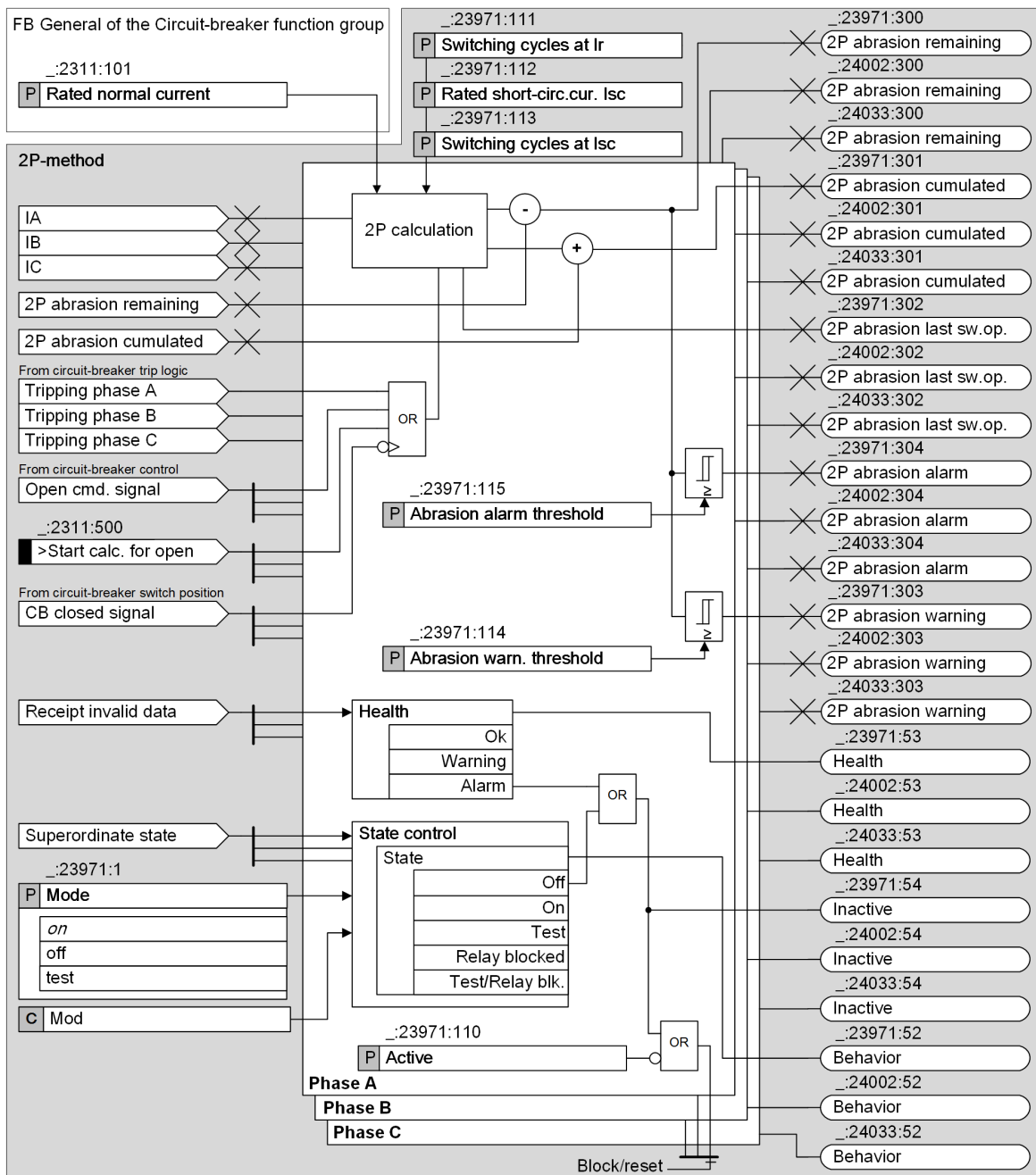
Figure 11-10 Logic 2P Method
