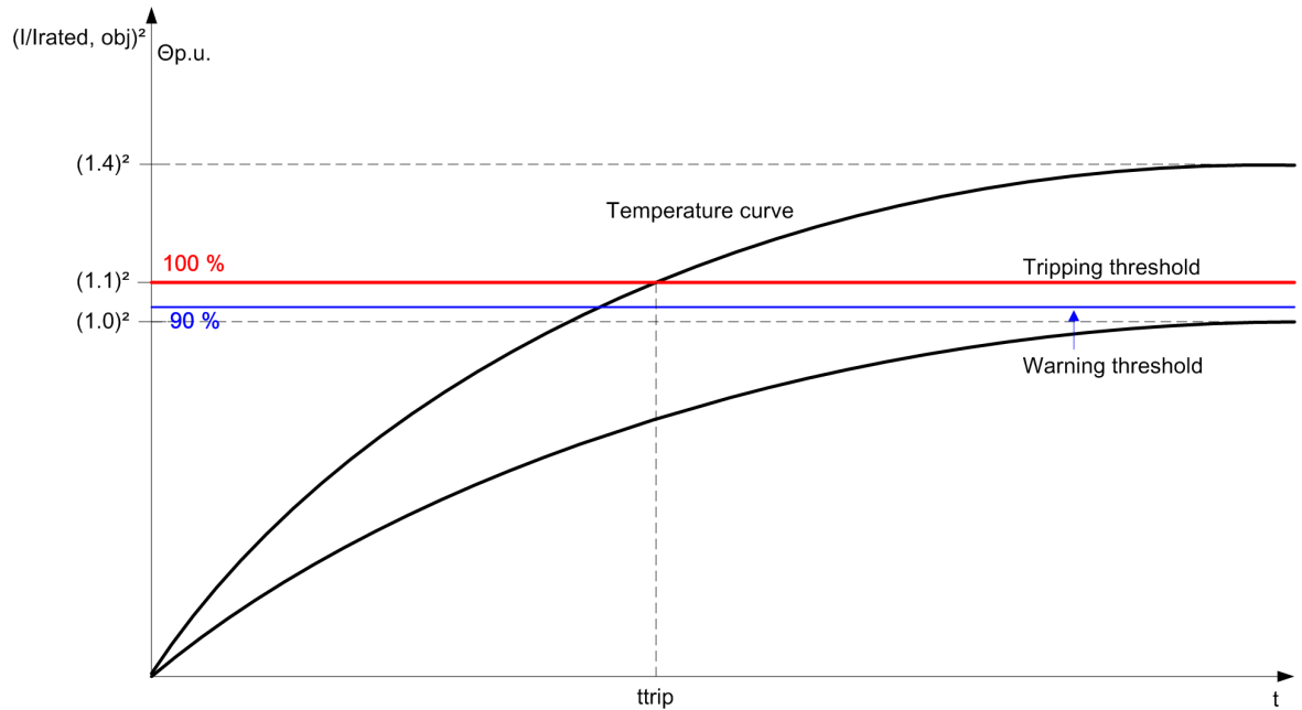
Figure 6-172 Temperature History for Different Overload Currents ( \kappa -factor = 1.1)
