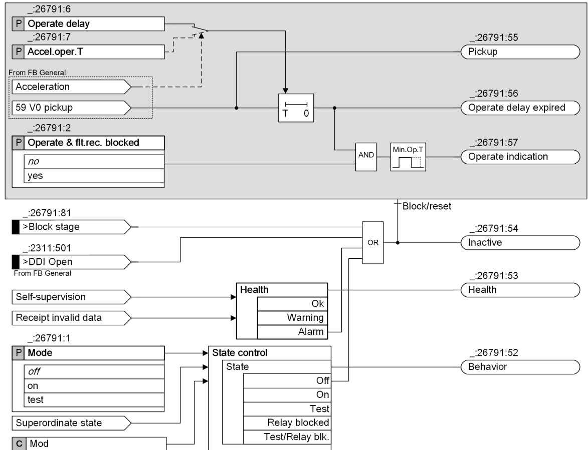
Figure 6-363 Logic Diagram of the Overvoltage-Protection Stage with Zero-Sequence Voltage/Residual Voltage
