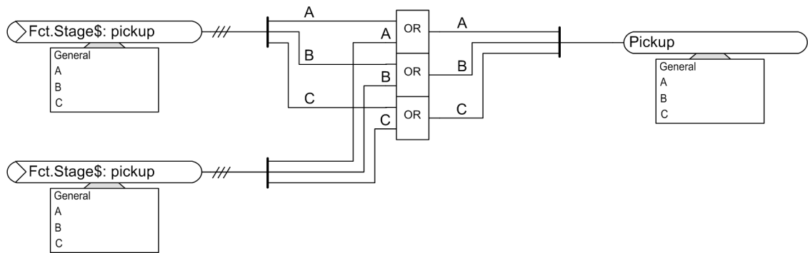
Figure 5-41 Generation of the Pickup Indication of the Capacitor Bank Function Group
