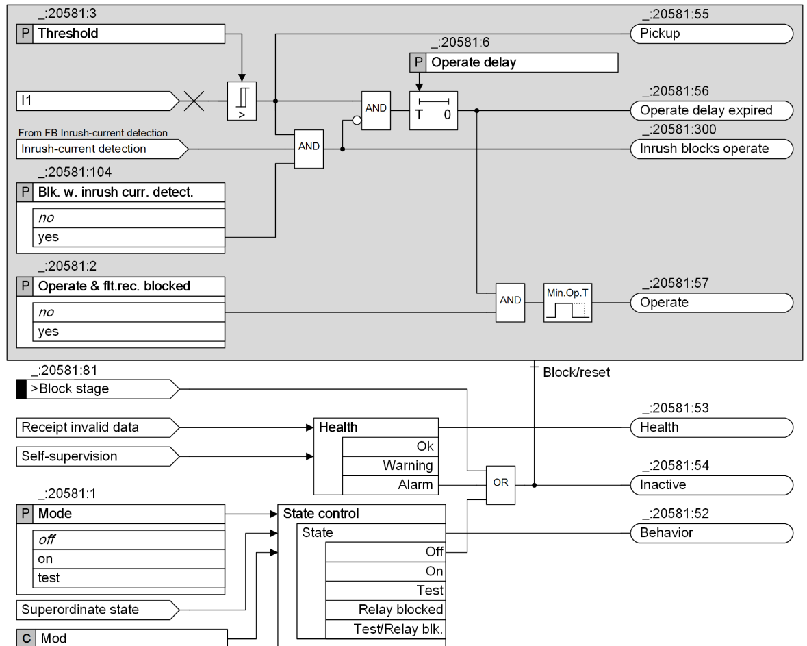
Figure 6-100 Logic Diagram of the Stage Definite-Time Positive-Sequence Overcurrent Protection
