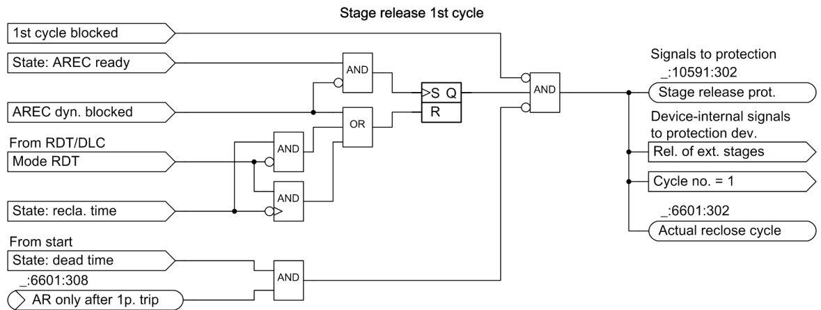
Figure 6-304 Stage Release for Protection Functions in the 1st Automatic Reclosing Cycle
