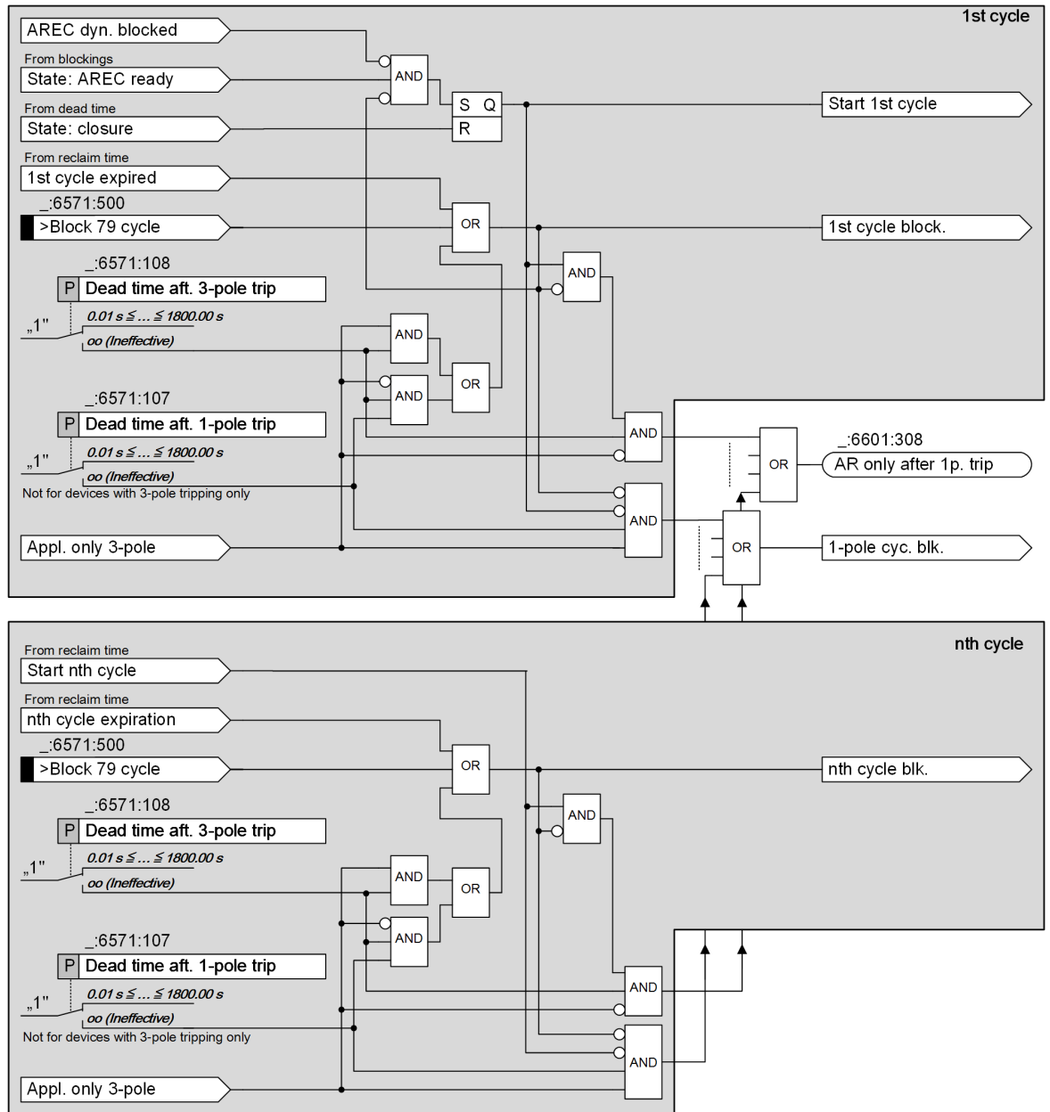
Figure 6-302 Cycle Control with Operating Mode: With Tripping/Without Action Time
