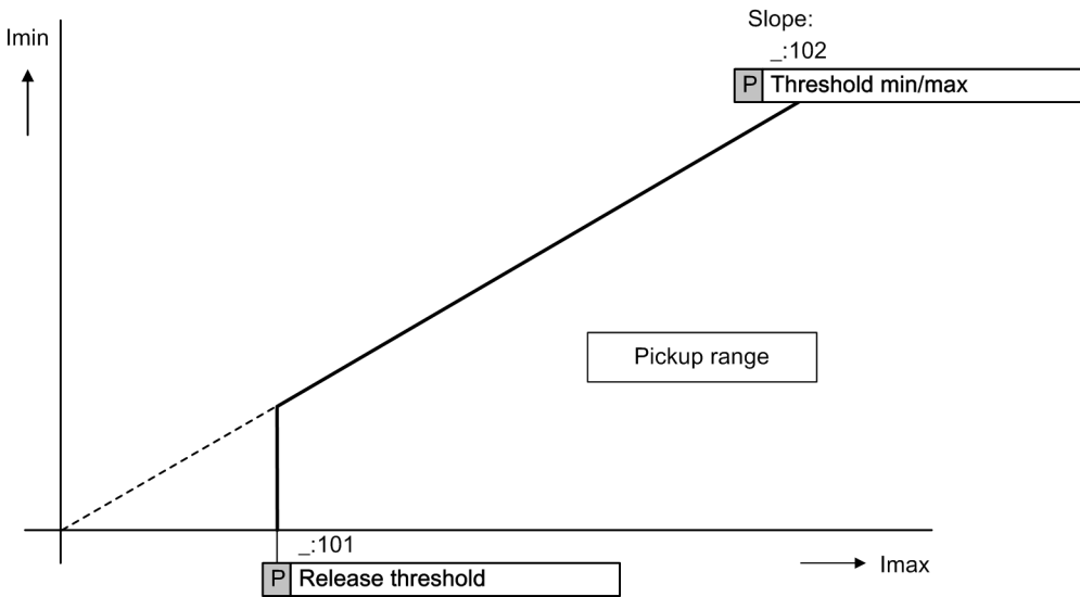
Figure 10-29 Characteristic of the Current-Balance Supervision
