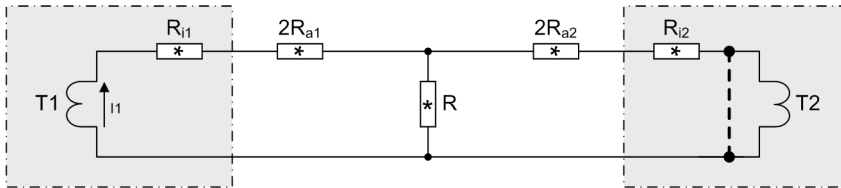
Figure 6-96 Simplified Connection Diagram of a Layout for High-Impedance Restricted Ground-Fault Protection
