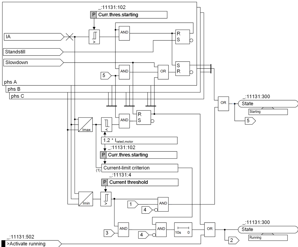
Figure 5-25 Logic Diagram of the Motor-State Detection, Part 2
