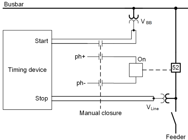
Figure 13-13 Measurement of the Circuit-Breaker Make Time
