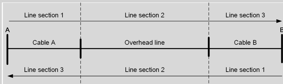
Figure 6-334 Line with 3 Line Sections
