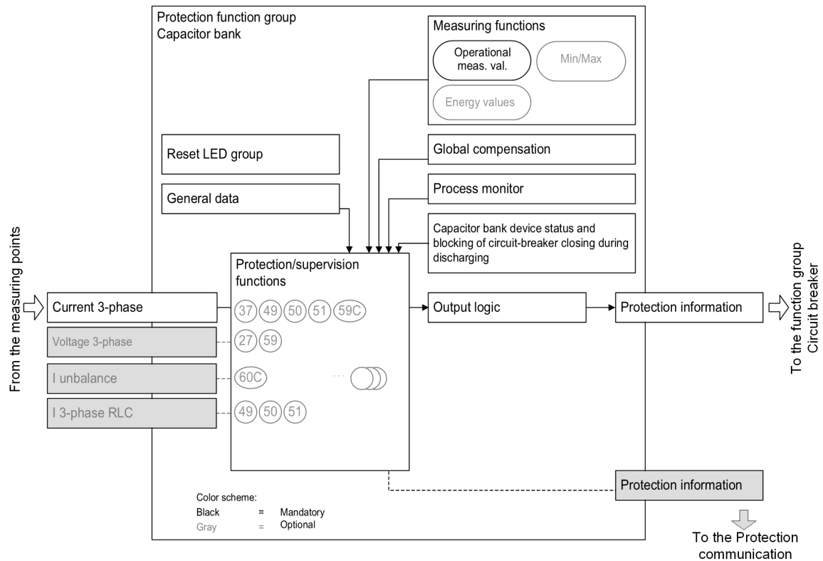
[dw_str_cap_comp, 1, en_US] Figure 5-35 Structure of the Capacitor Bank Function Group
