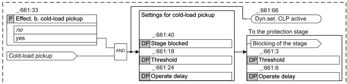
Figure 6-20 Influence of the Cold-Load Pickup Detection on the Overcurrent-Protection Stage
