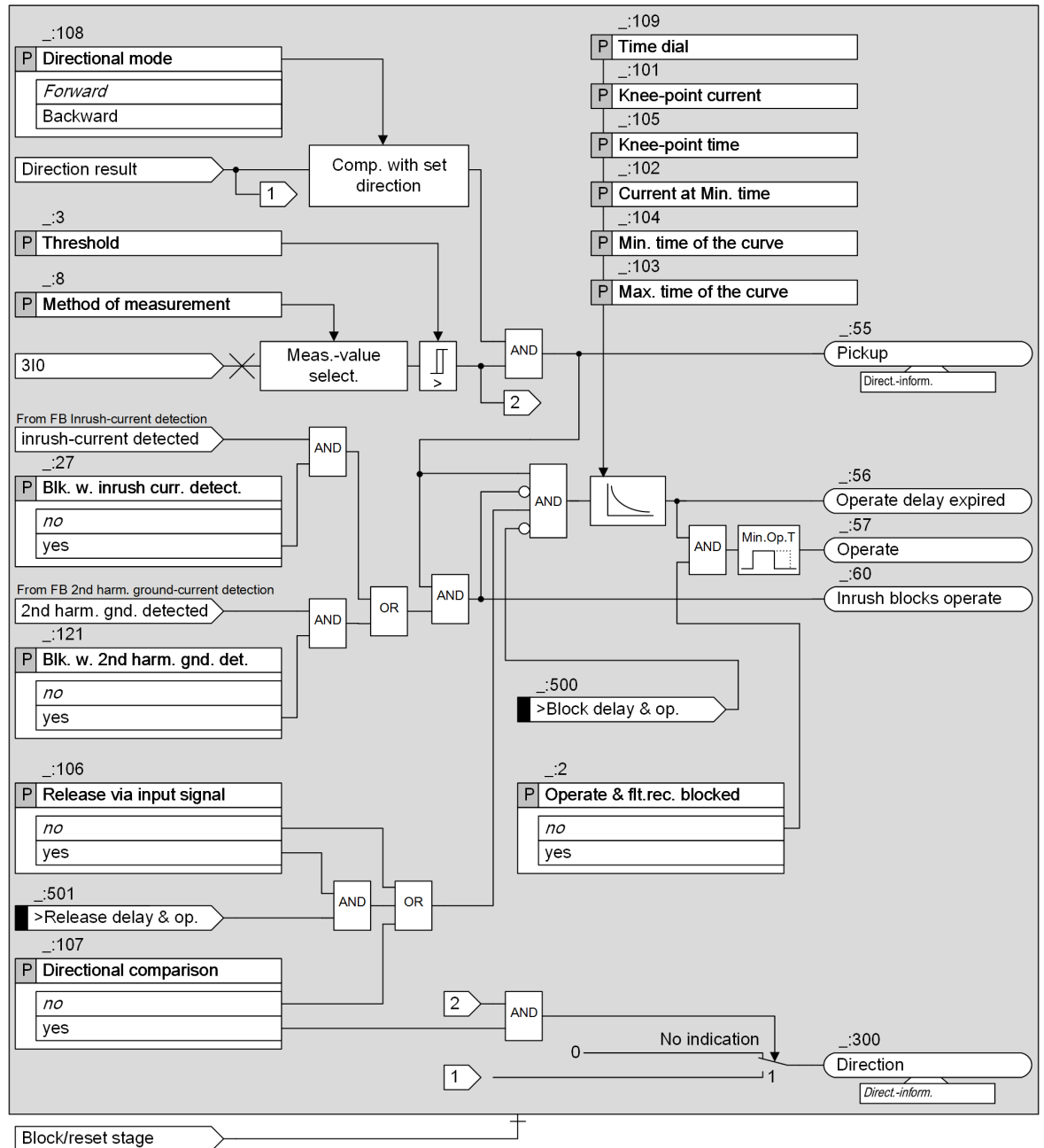
Figure 6-66 Logic Diagram of the Directional Logarithmic Inverse Time with Knee-Point Overcurrent Protection, Ground
