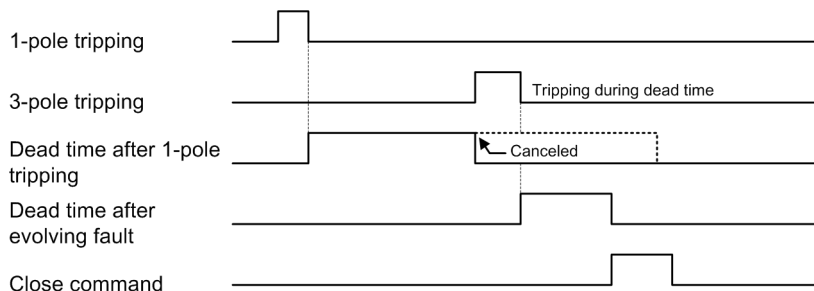
Figure 6-308 Cyclic Automatic Reclosing Function - Example for an Evolving Fault
