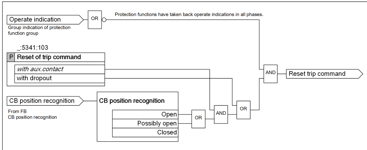
Figure 5-124 Trip-Command Reset
