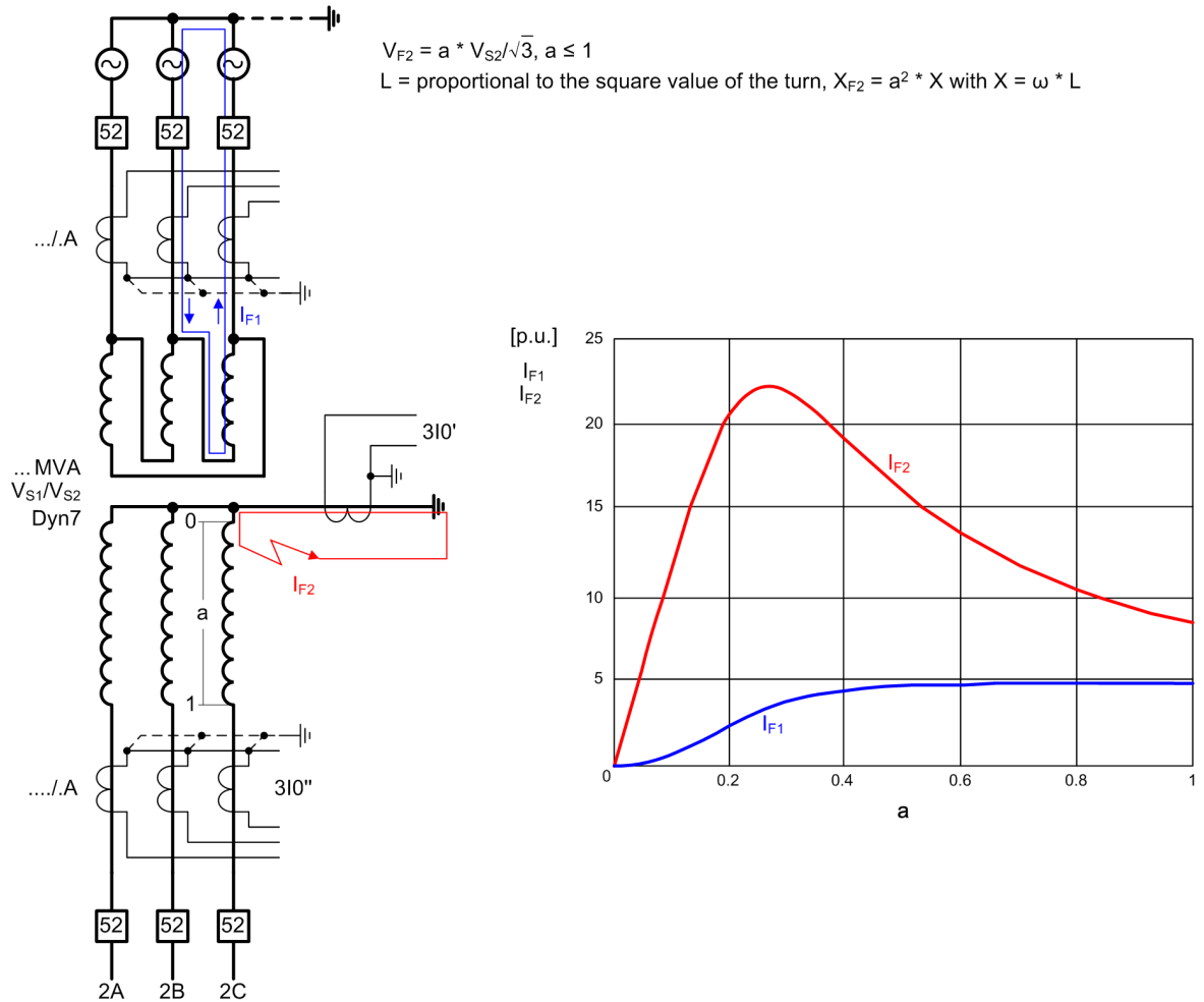
Figure 6-276 Principal Fault Current Curves with a 1-Pole Ground Fault
