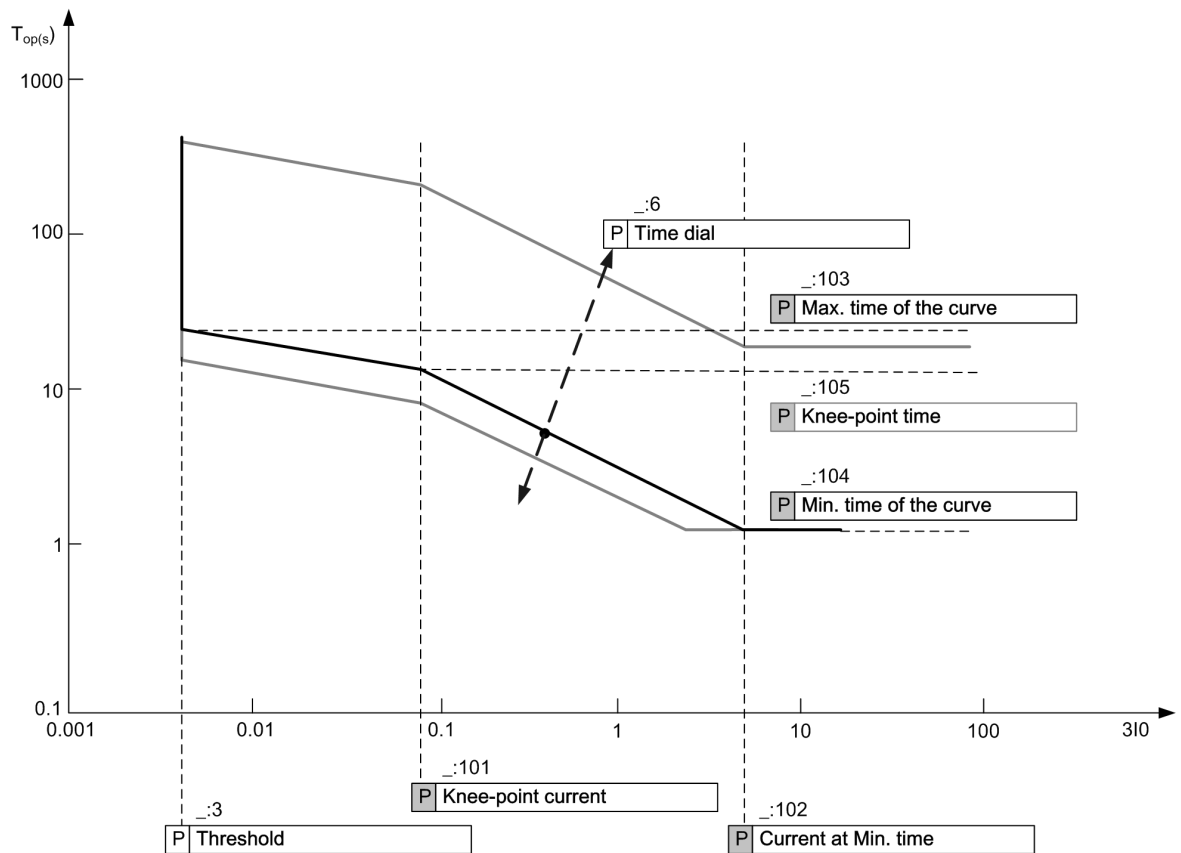
Figure 14-9 Operate Curve of the Logarithmic Inverse Time with Knee-Point Characteristic (In the Example of Threshold = 0.004 A )
