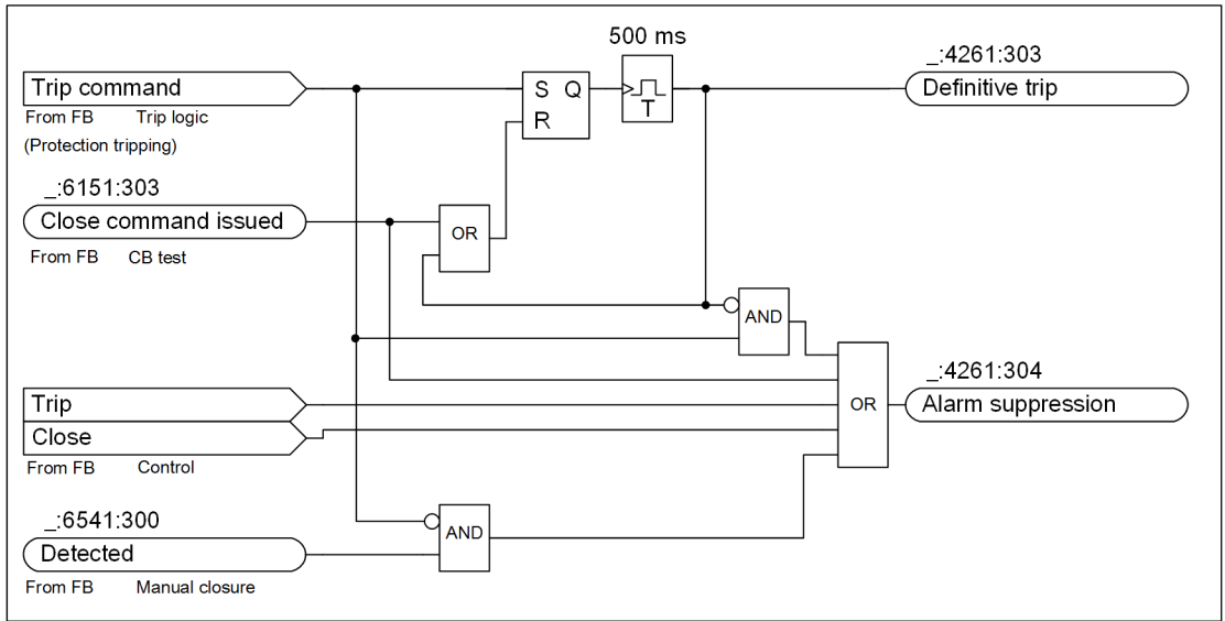
Figure 5-127 Definitive Tripping and Circuit-Breaker Tripping Alarm Suppression
