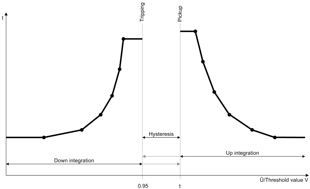
Figure 8-16 Pickup Behavior and Dropout Behavior when Using a User-Defined Characteristic Curve
