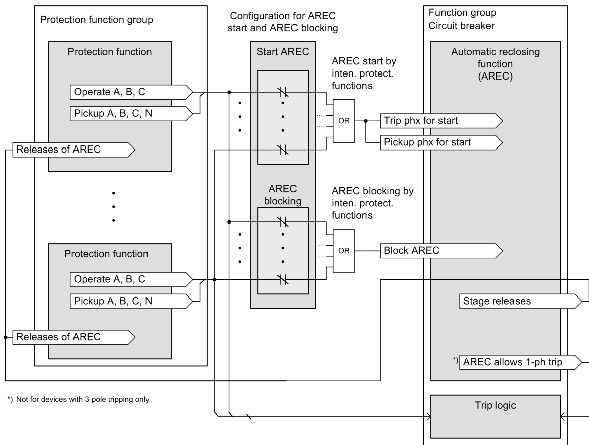
Figure 6-290 Signals between Protection Functions and Automatic Reclosing Functions
