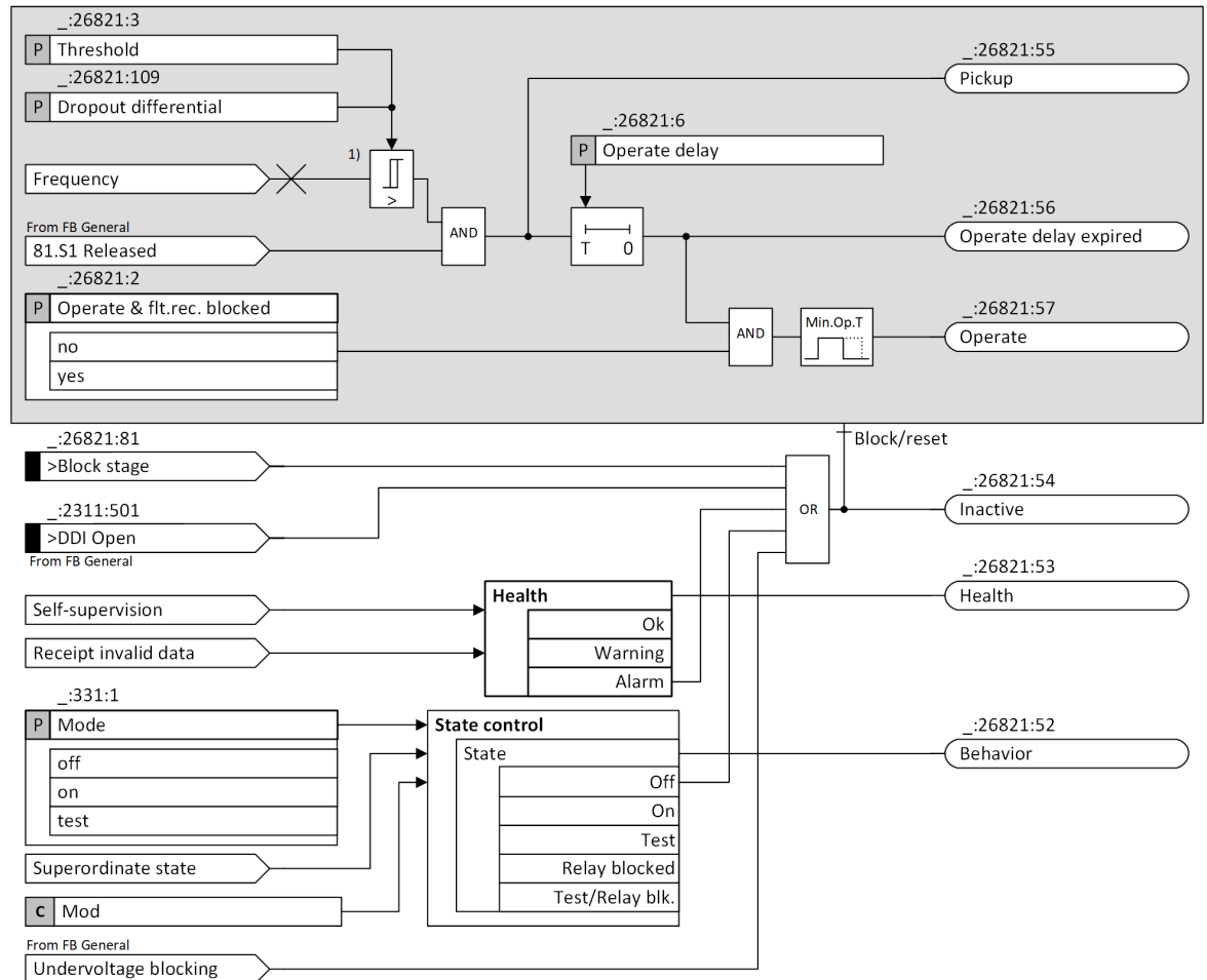
Figure 6-364 Logic Diagram of the Stage Overfrequency-Protection S1
