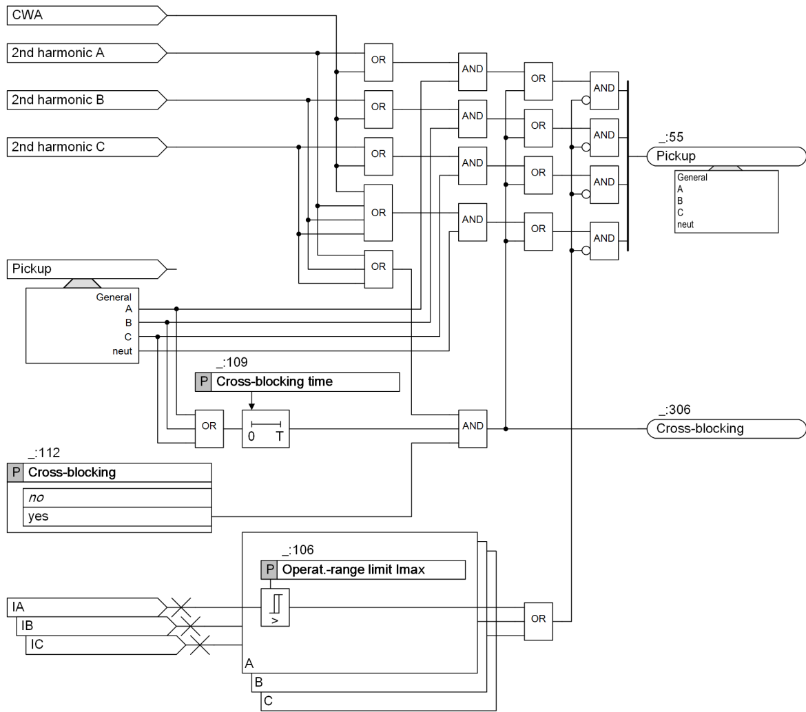
[lo_inrush_12_2_en_US] Figure 6-75 Logic Diagram of the Inrush-Current Detection
