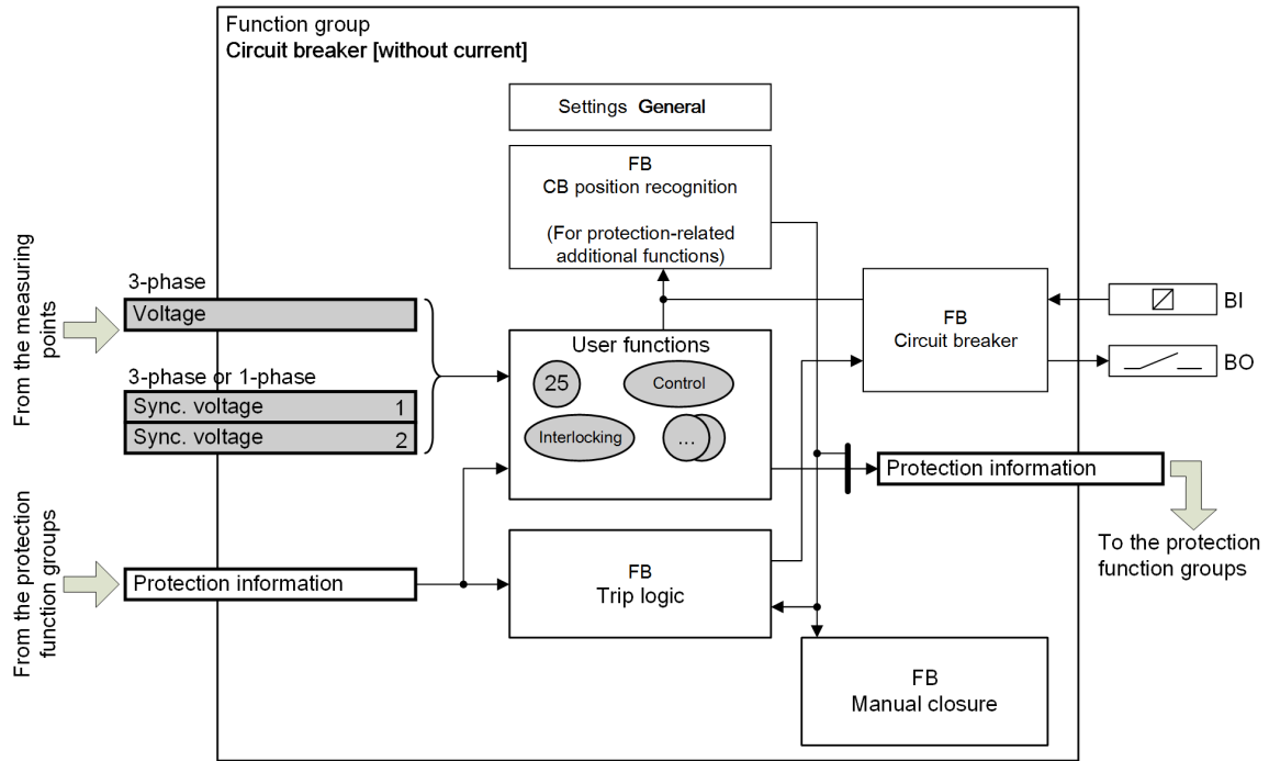
Figure 5-122 Structure of the Function-Group Type Circuit breaker [without current]
