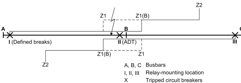
Figure 6-318 Example for Adaptive Dead Time (ADT)
