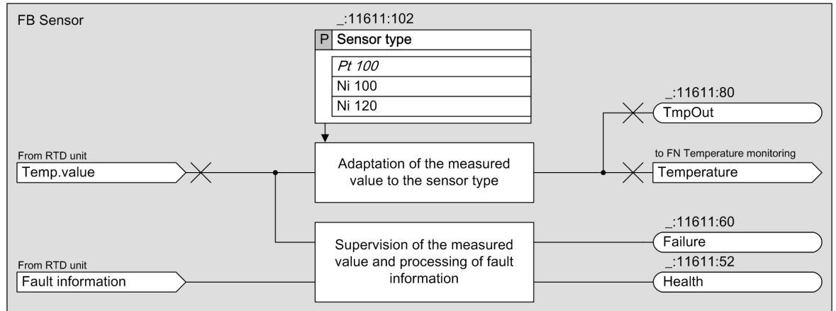
Figure 5-63 Logic Diagram of the Temperature Sensor Function Block
