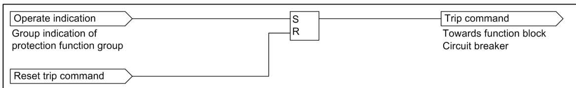
Figure 5-108 Trip Command
