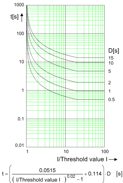
Figure 14-16 Operate Curves and Dropout-Time Characteristic Curves According to ANSI/IEEE
