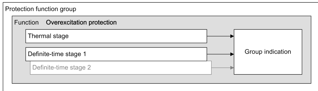
Figure 6-238 Structure/Embedding of the Function
