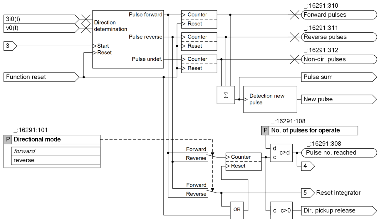
Figure 6-109 Logic Diagram of Direction Determination and Pulse Counting
