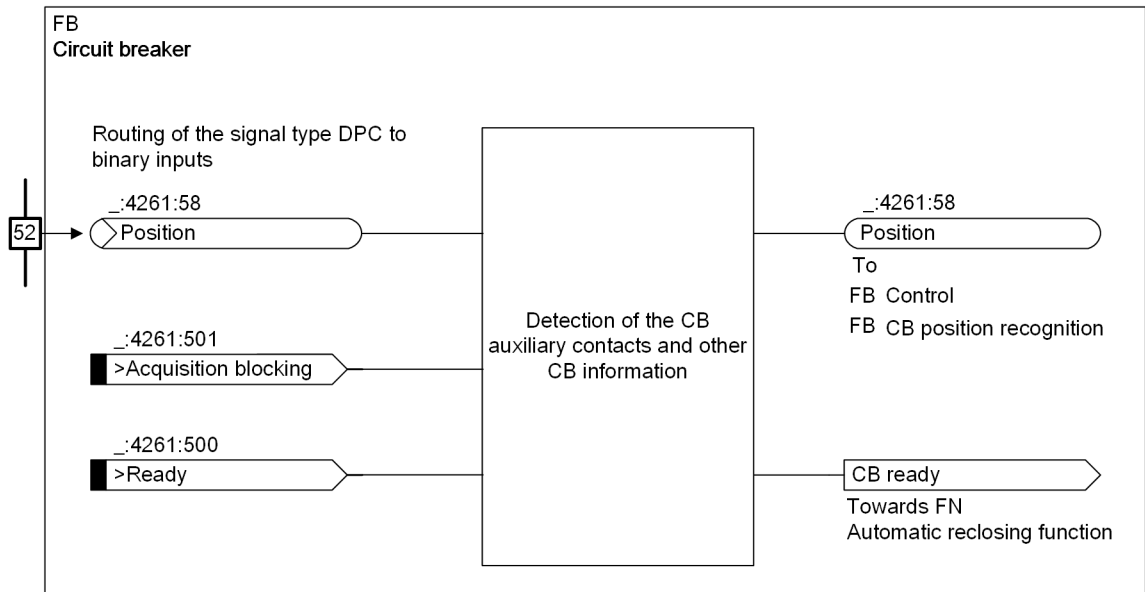
Figure 5-111 Acquisition of the Circuit-Breaker Information
