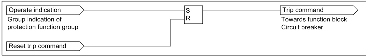
Figure 5-123 Trip Command
