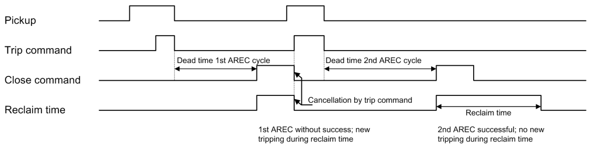
Figure 6-283 Process Diagram of a Two-Time Reclosing with Action Time (2nd AREC Successful)
