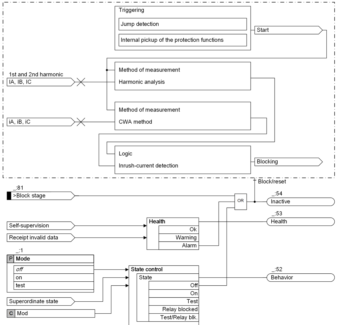
Figure 6-71 Basic Structure of the Inrush-Current Detection
