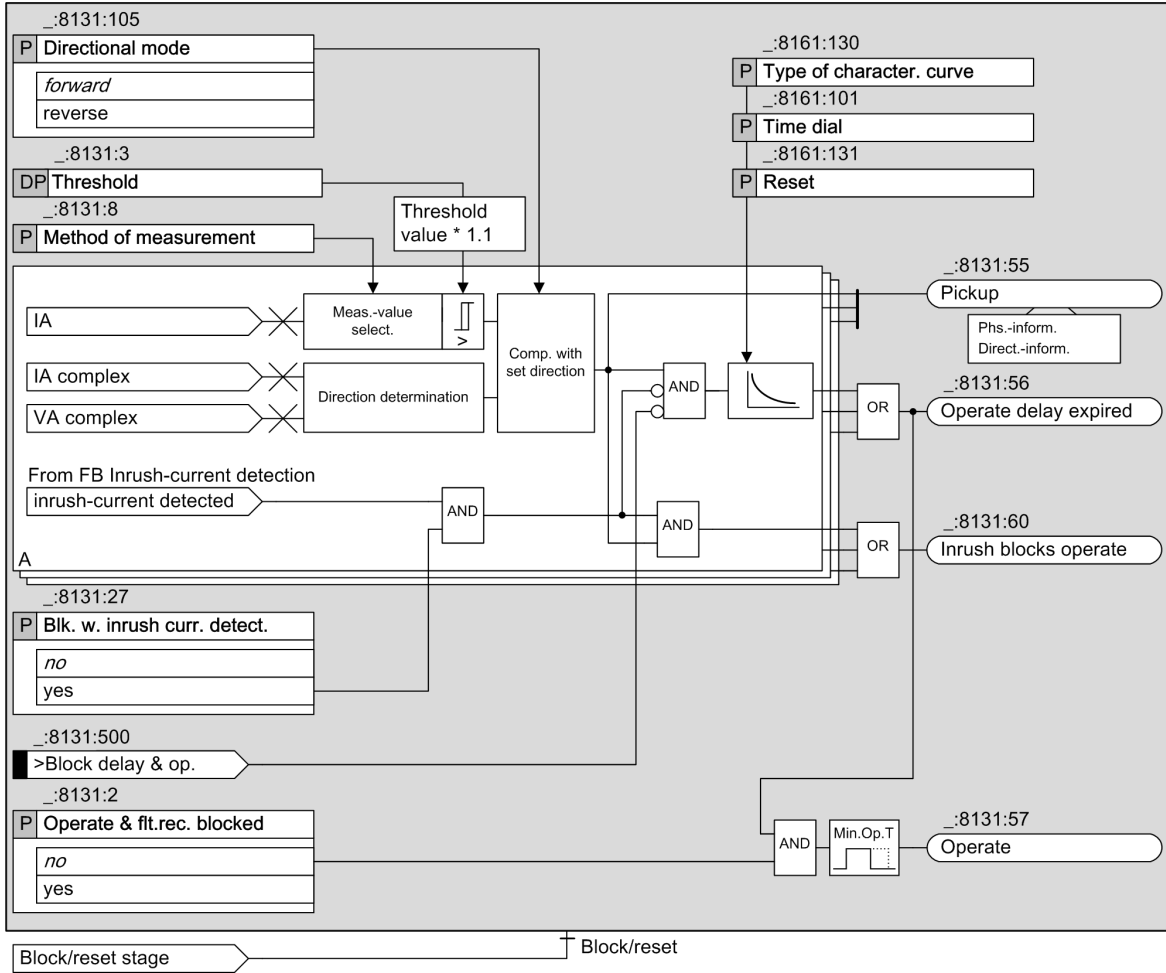
Figure 6-42 Logic Diagram of the Directional, Inverse-Time Overcurrent Protection, Phases - Basic
