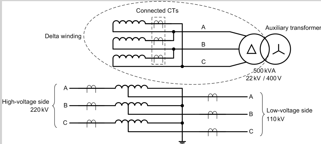
Figure 6-101 Auto Transformer with Tertiary Delta Winding
