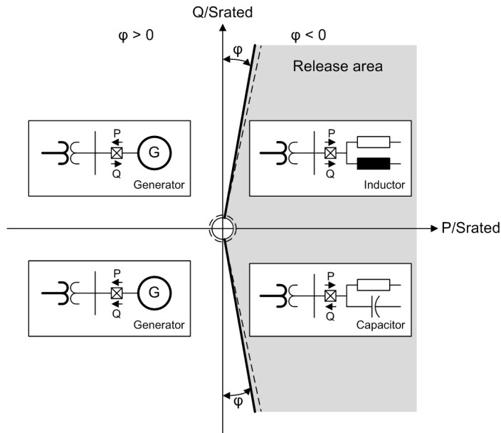
Figure 6-216 Power-Criterion Checking at \Phi (power criterion) \leq 0
