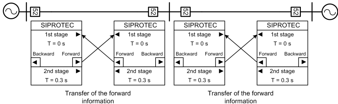
Figure 6-50 Selectivity through Directional Comparison Protection
