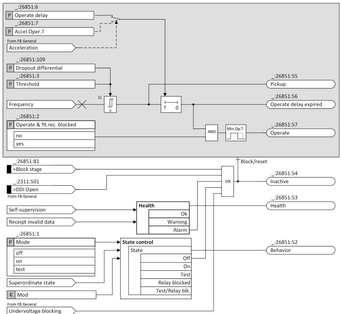
Figure 6-365 Logic Diagram of the Stage Overfrequency-Protection S2
