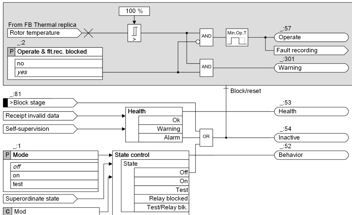
[lo_therm_tolp-rotor, 4, en_US] Figure 7-20 Logic Diagram of the Thermal Overload Protection Rotor (49R Overl.rot. Protection)
