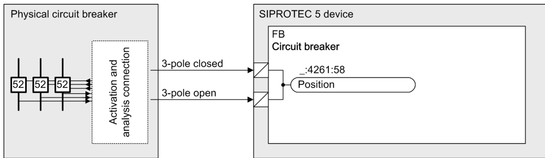
Figure 5-115 Recommended Evaluation of the Circuit-Breaker Switch Position
