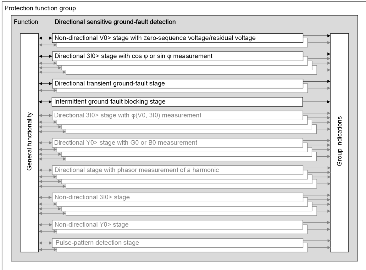
Figure 6-112 Structure/Embedding of the Directional Function in Protection Function Groups
