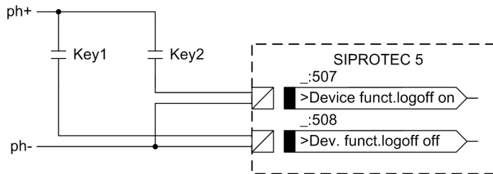
Figure 3-65 External Push-Button Wiring for Logging off the Device
