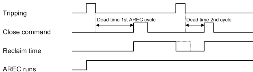
Figure 6-294 Operating-Mode Signal Examples: With Tripping/Without Action Time
