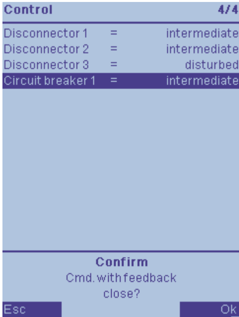
Figure 9-32 The Status of Interlocking Conditions is not Visible in the Control Menu
