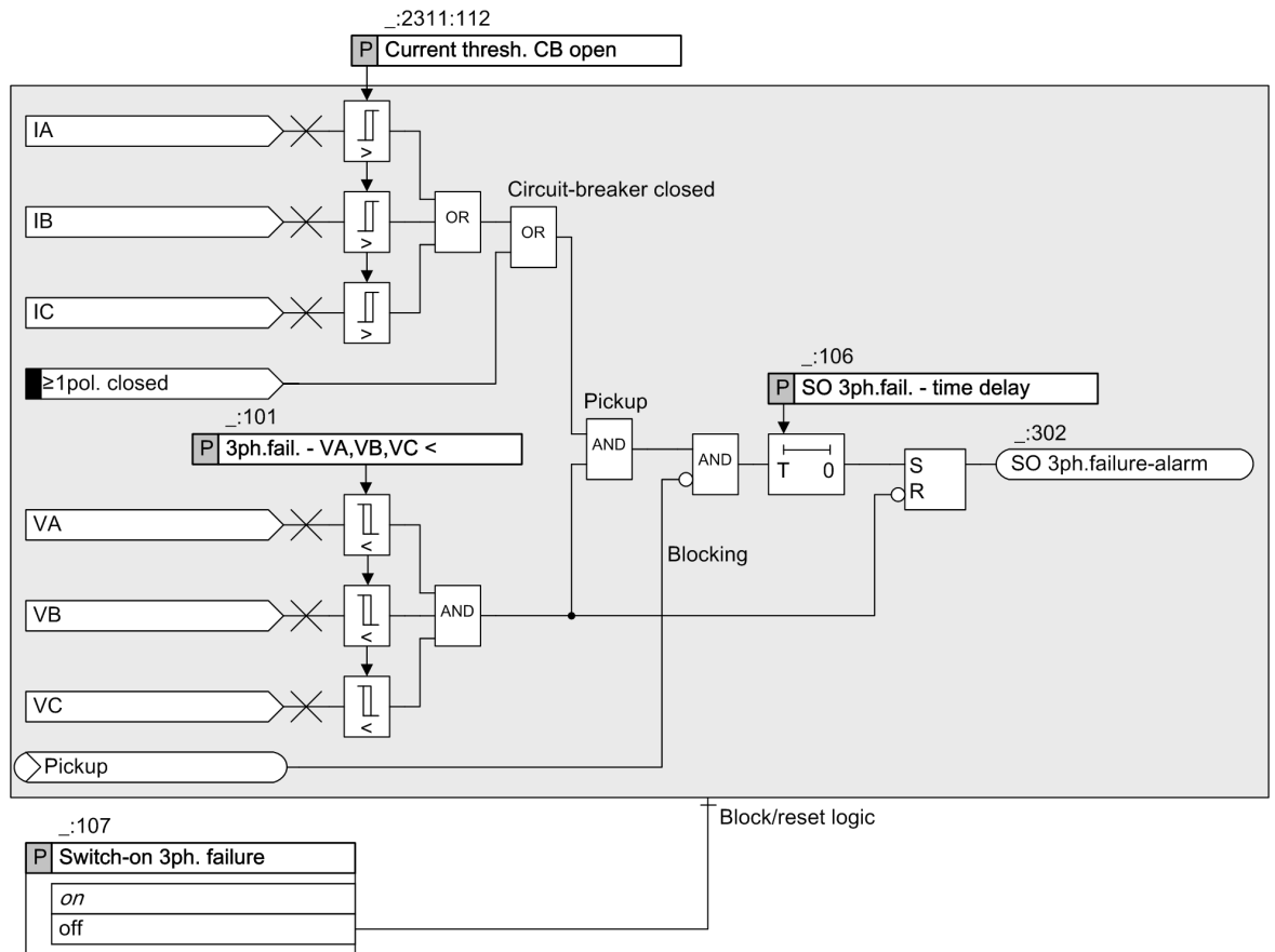
Figure 10-8 Logic Diagram Switching to 3-Phase Measuring-Voltage Failure
