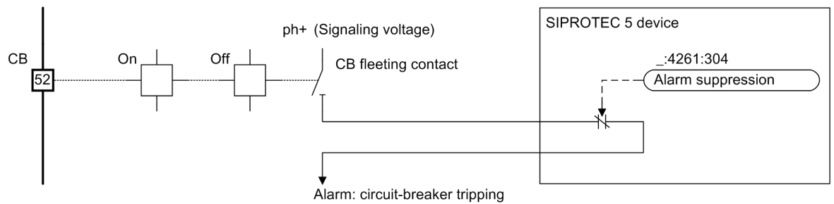
Figure 5-133 Circuit-Breaker Tripping Alarm Suppression
