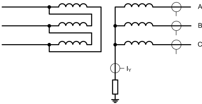
Figure 6-12 I0 Elimination Principle
