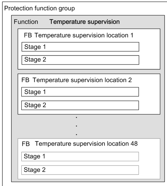
Figure 6-338 Structure/Embedding of the Function
