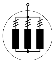
Fully parallel-connected internal winding systems
