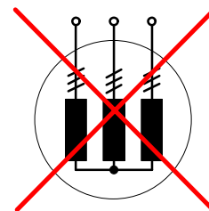
Winding systems separated at input side with common internal neutral
