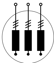
Fully isolated, separate winding systems without phase displacement
