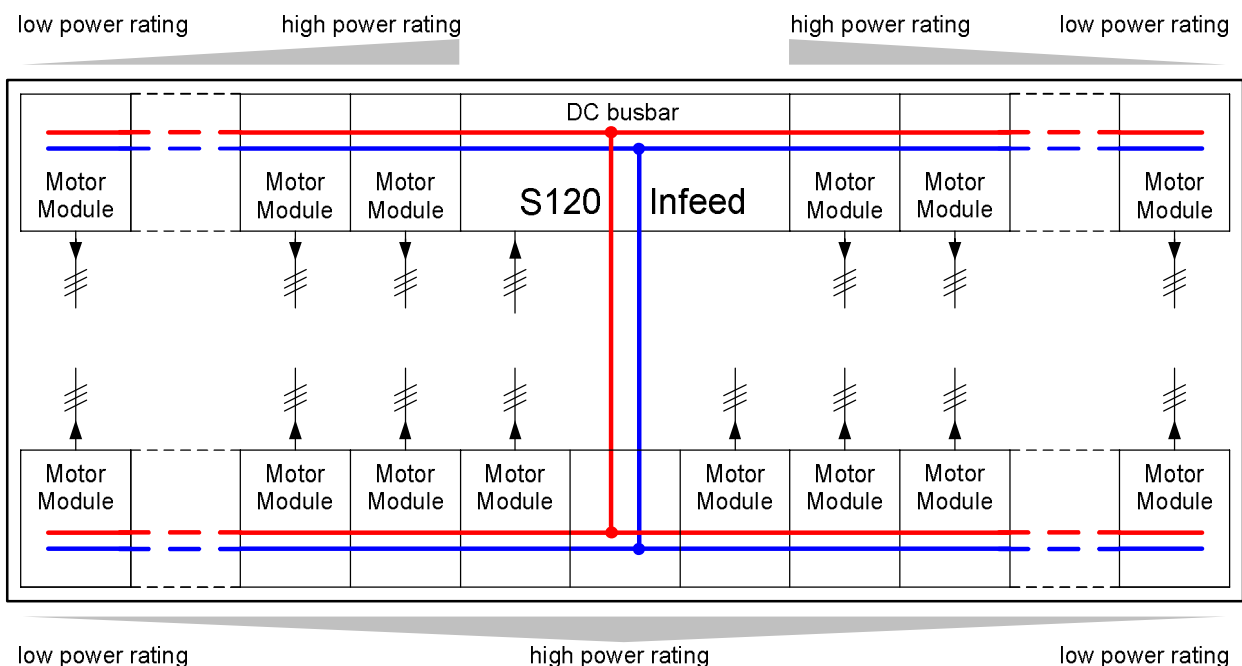
Example 4: Linear arrangement of the DC busbar in two sub-configurations / opposite arrangement
