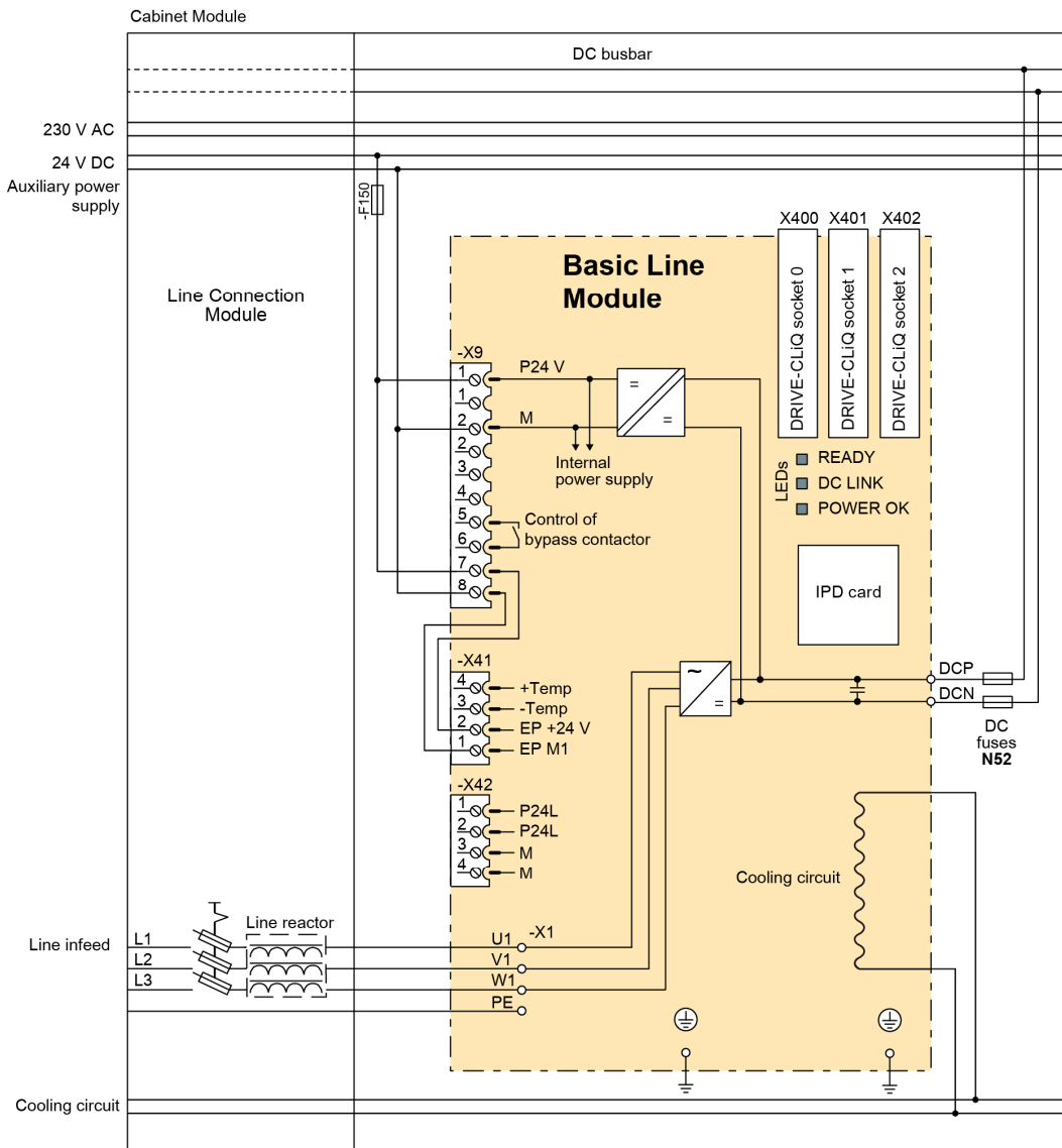
Example of a liquid-cooled Basic Line Connection Module ( \leq 800 A) with fuse switch disconnector and line reactor in the Line Connection Module and DC fuses (option N52) in the Basic Line Module
