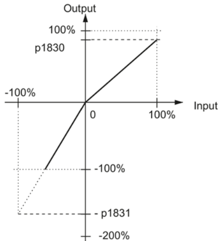
Figure 5-15 Example of piston plane adaptation characteristic
