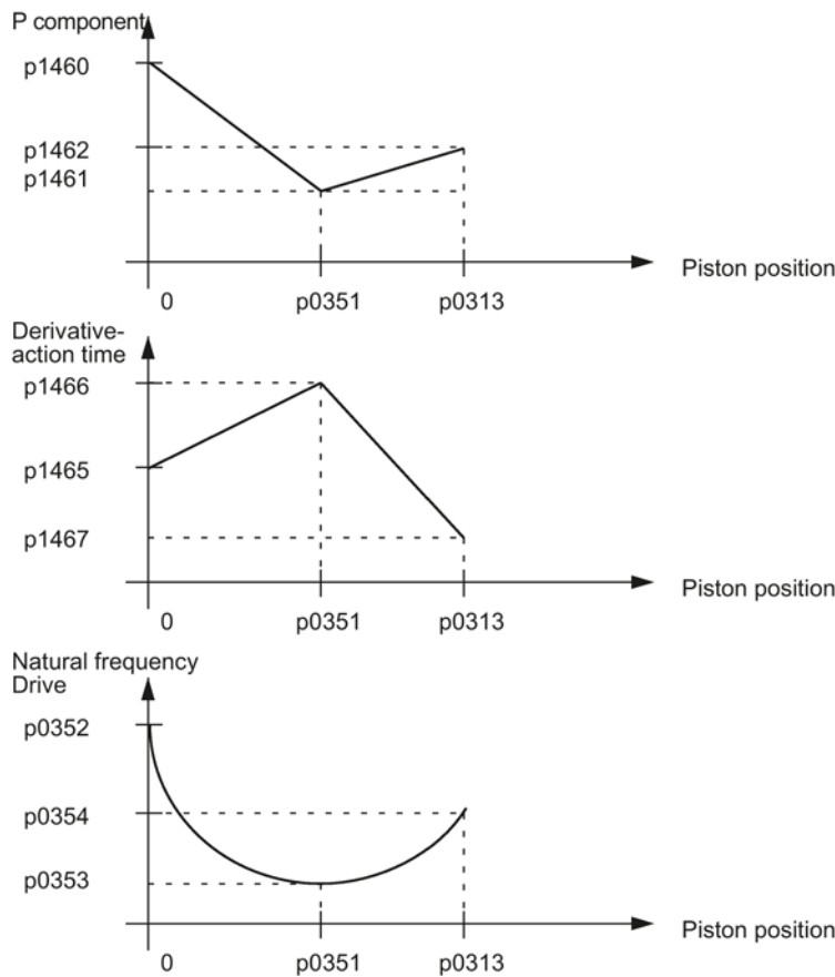
Figure 5-7 Adaptation
