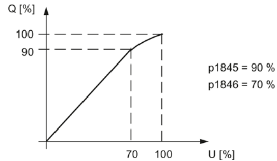
Figure 5-17 Example of transition point compensation
