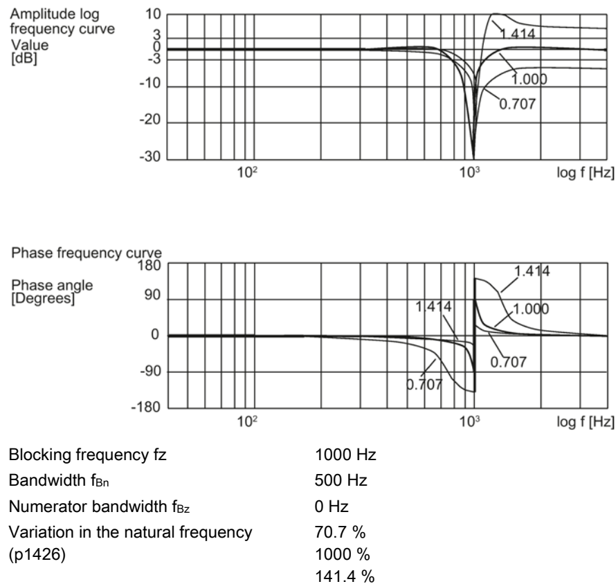
Figure 5-6 Frequency response of the general bandstop filter
