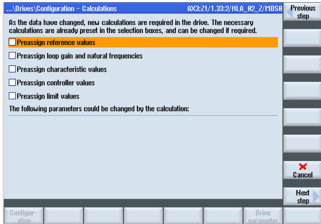
Figure 4-8 Configuration - calculations
