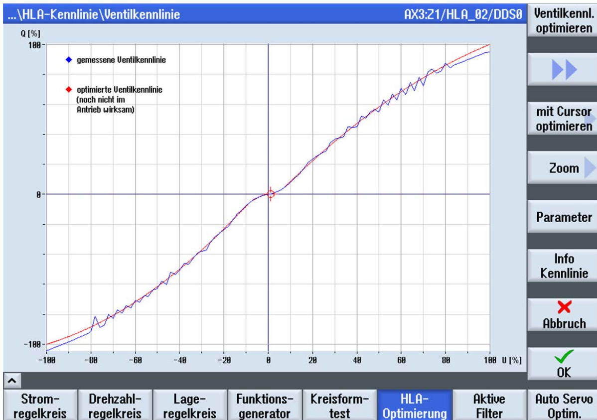
Figure 4-32 Graphically tuning the valve characteristic
