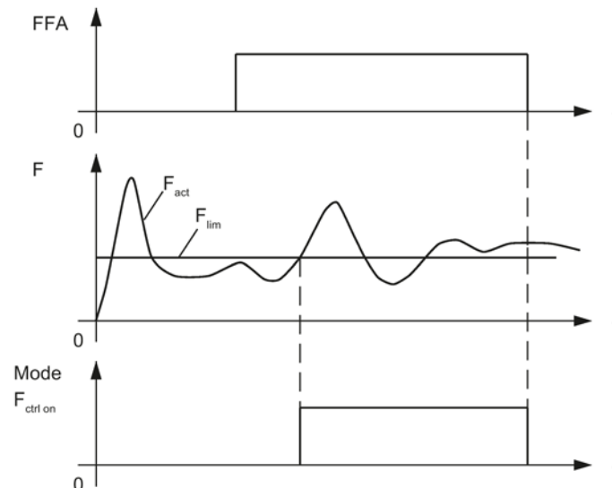
Figure 5-11 Deselecting force control by deactivating the "Travel to fixed stop" function.
