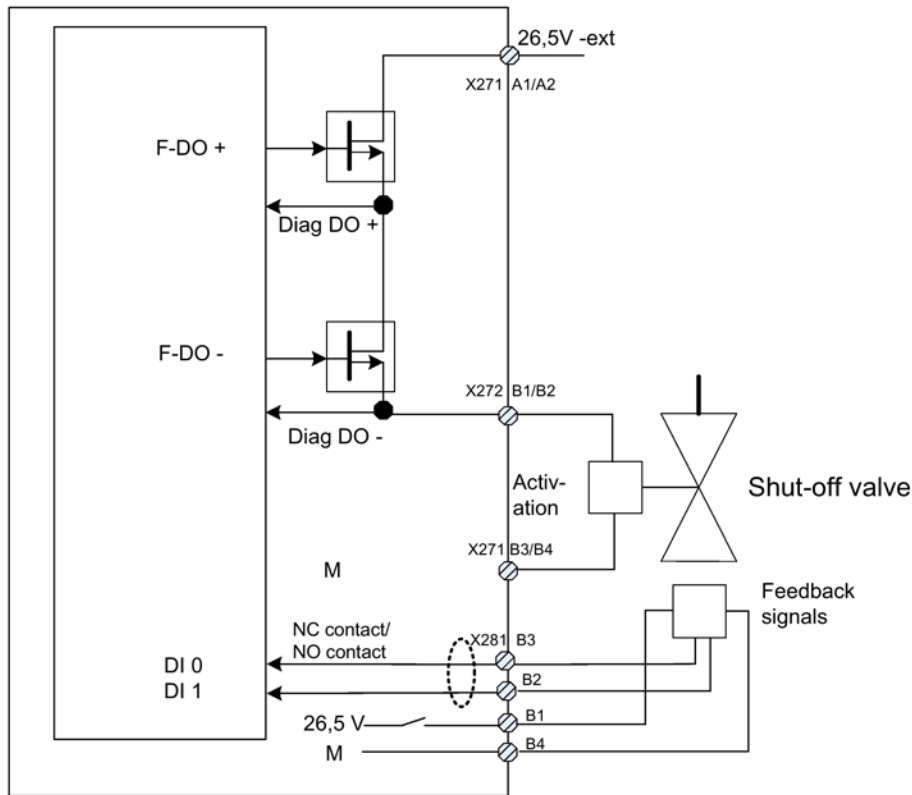
Figure 3-5 Interconnection of the shutoff valve
