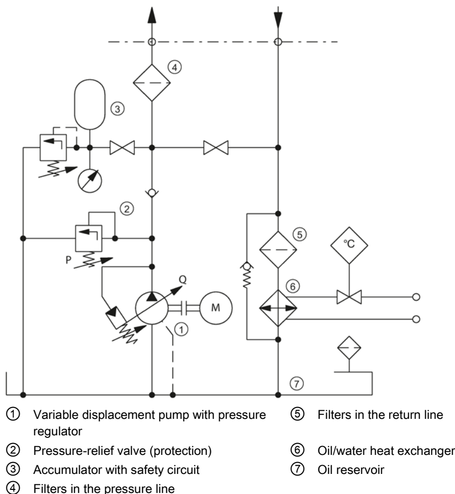
Figure 3-6 Overview of a typical hydraulic power unit
