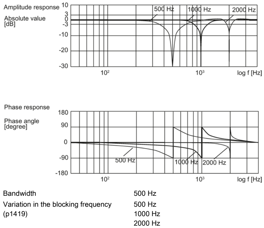
Figure 5-4 Frequency response of the non-damped bandstop filter
