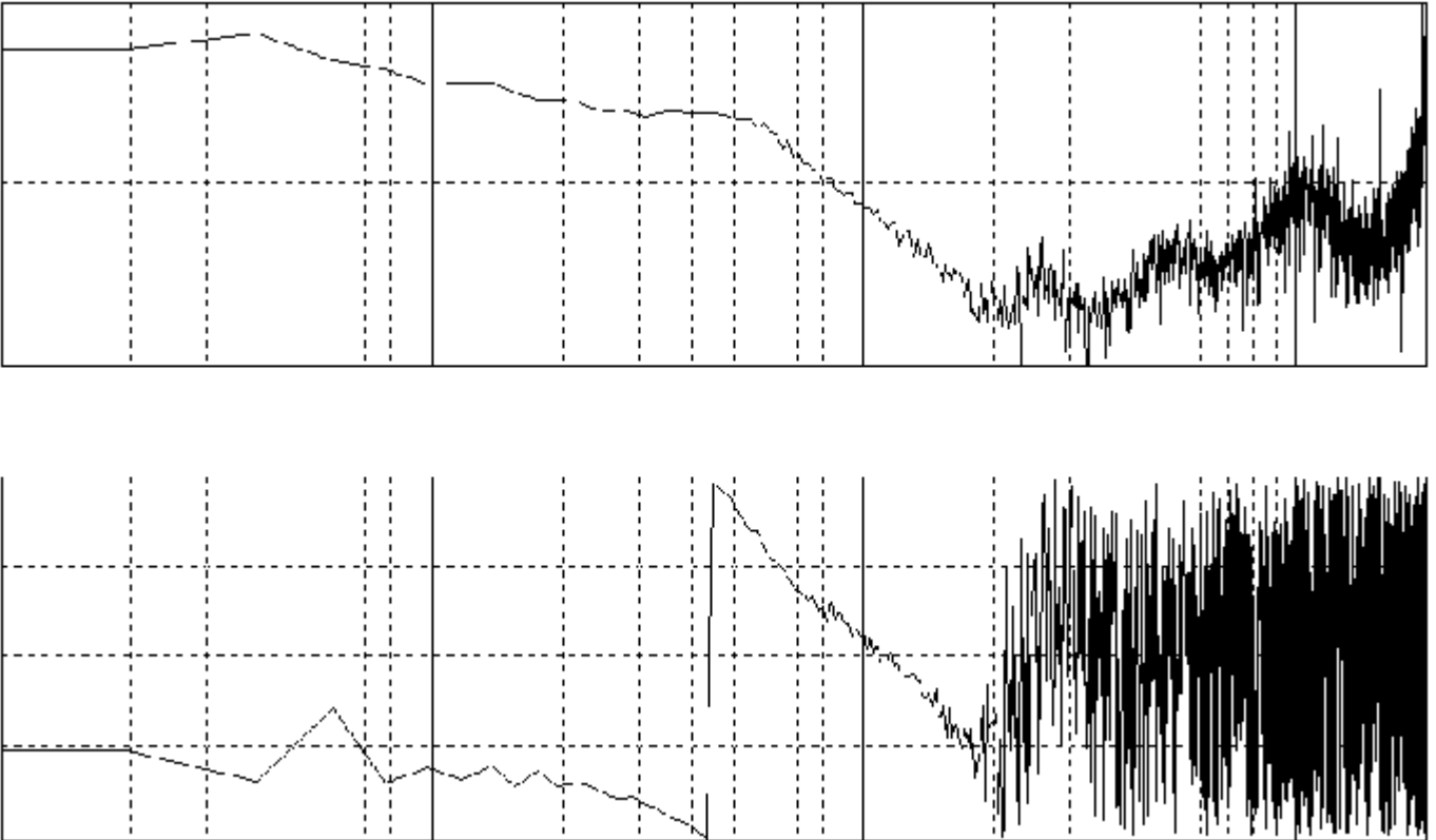
Figure 4-52 Bode diagram for velocity controlled system + controller (example)
