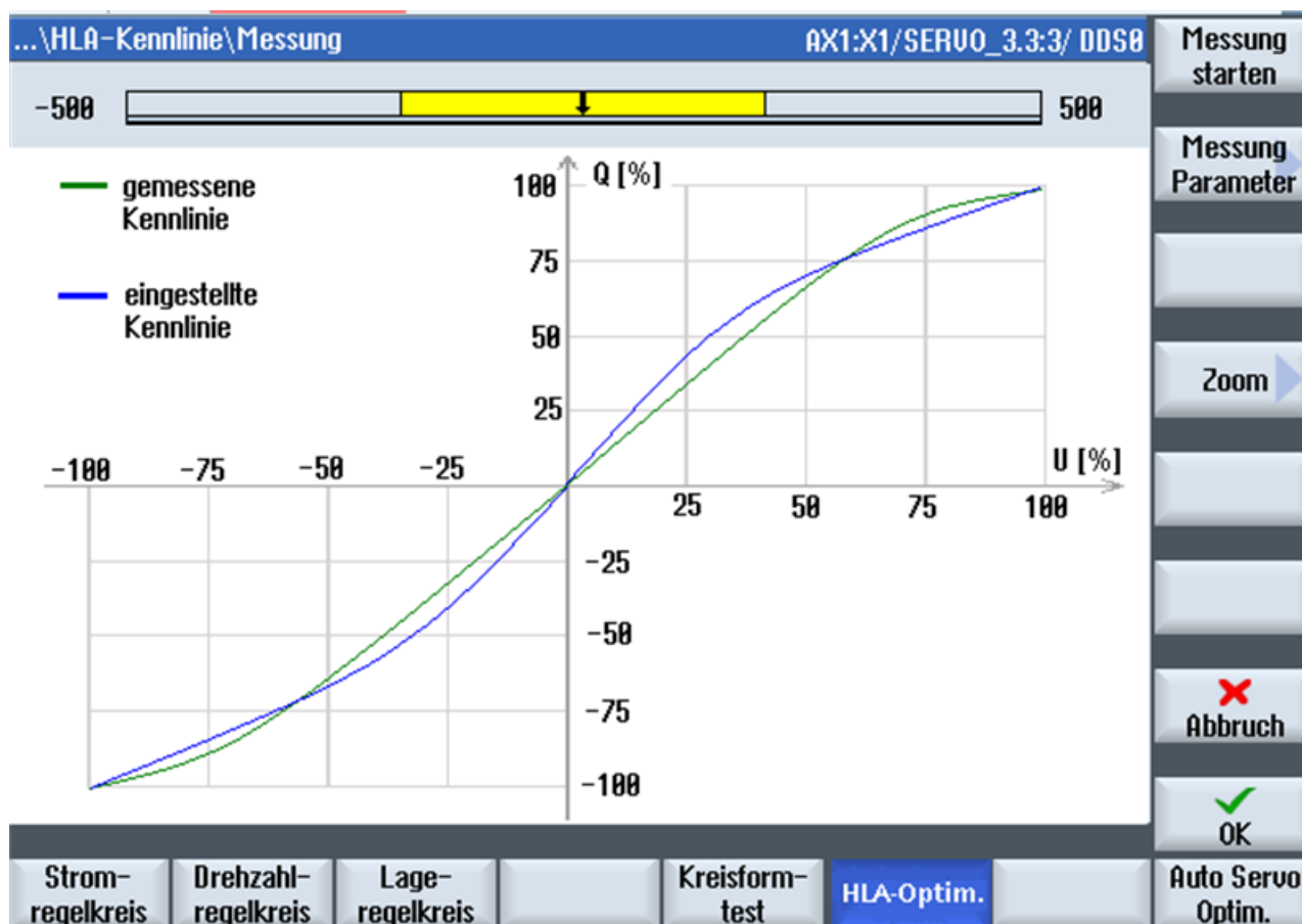
Figure 4-28 Characteristic: Measurement
