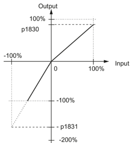
Figure 4-34 Characteristic plane adaptation
