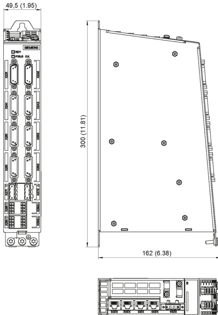
Figure 6-3 Dimension drawing of the HLA module, all dimensions in mm and (inches)
