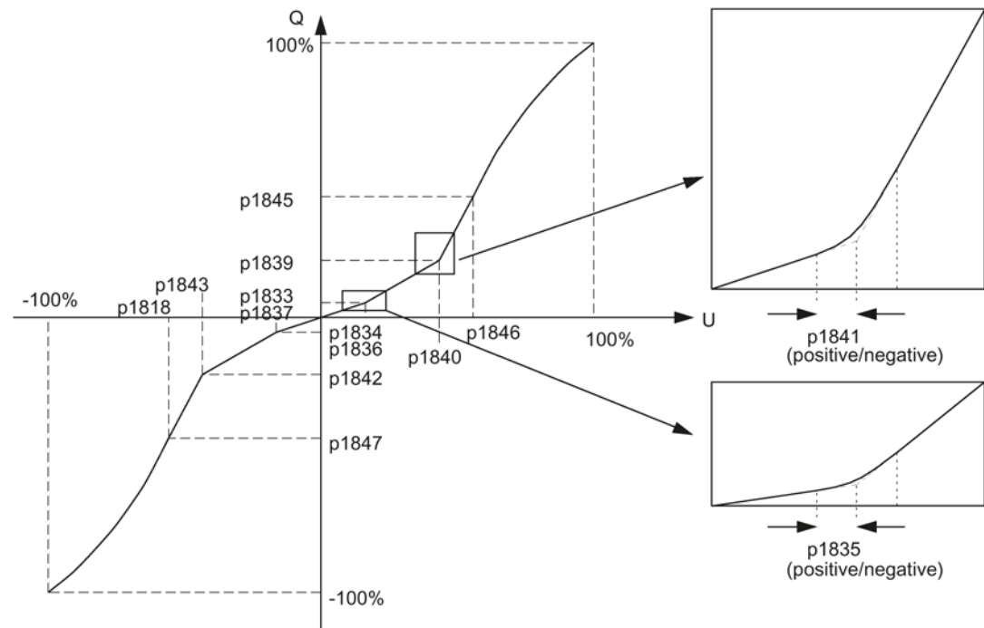
Figure 5-16 Valve characteristic with transition point in zero, fine control and saturation ranges
