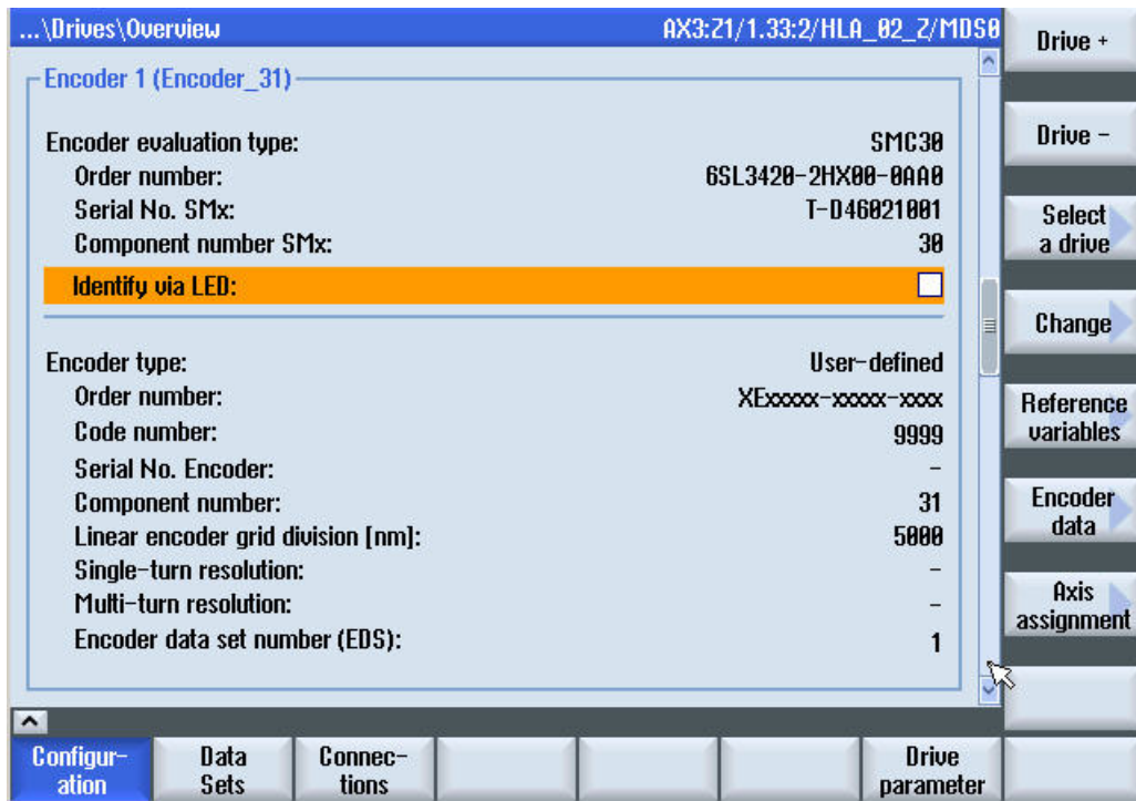
Figure 4-17 Encoder overview
