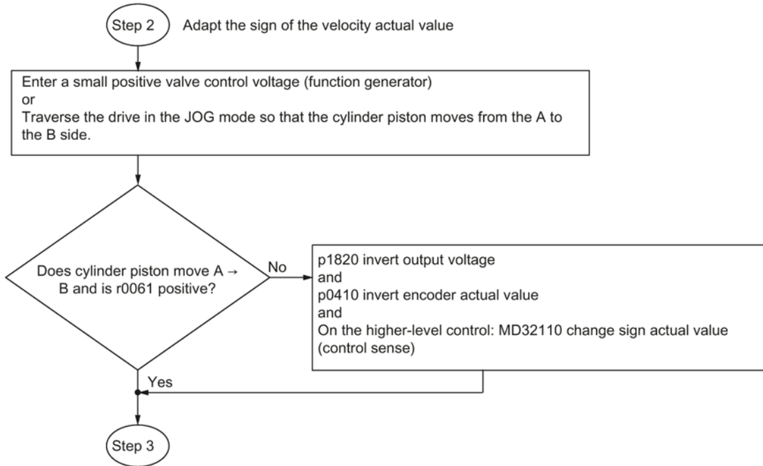
Figure 4-40 Commissioning flowchart, definition of the drive traversing direction
