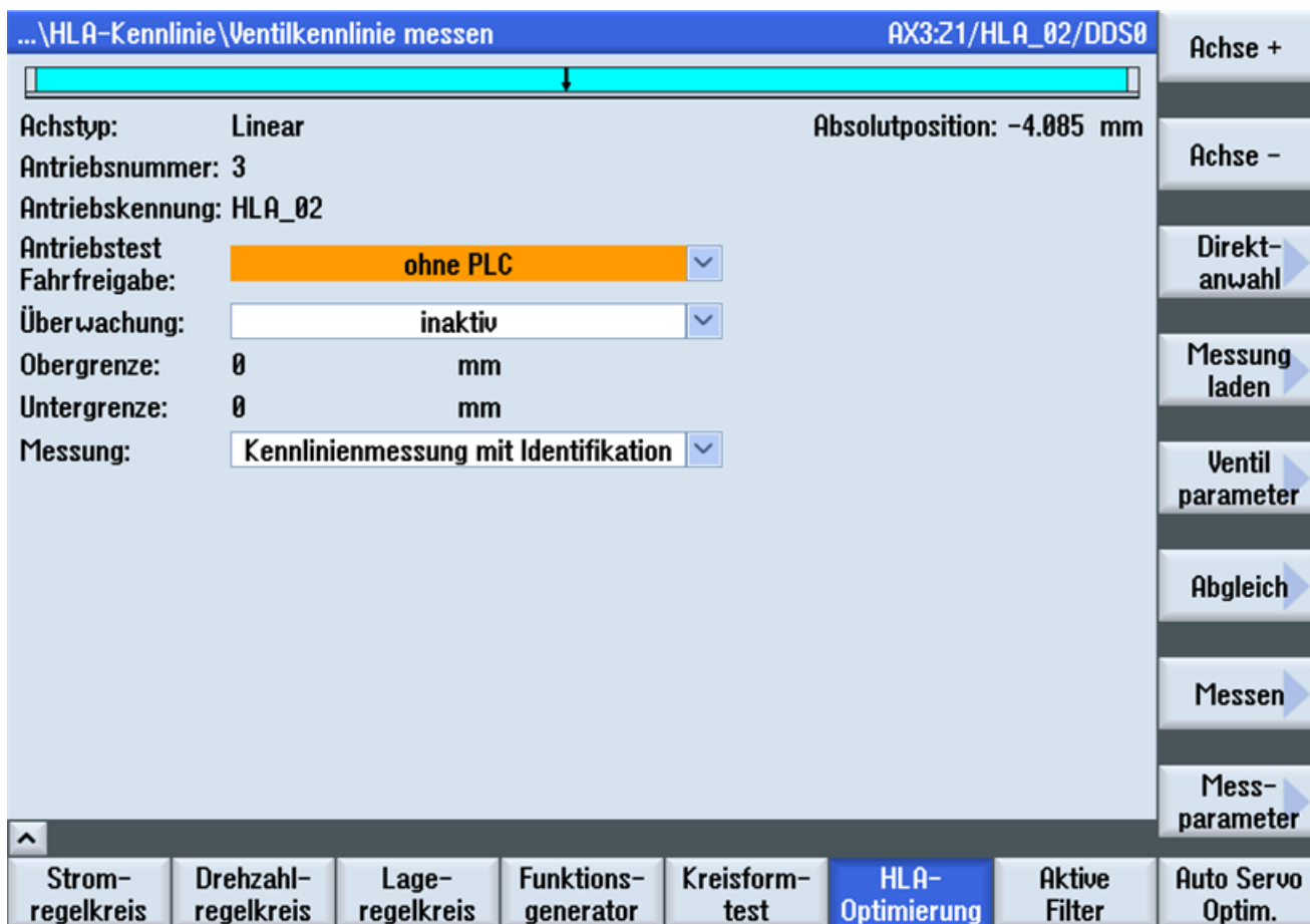
Figure 4-27 Measure valve characteristic
