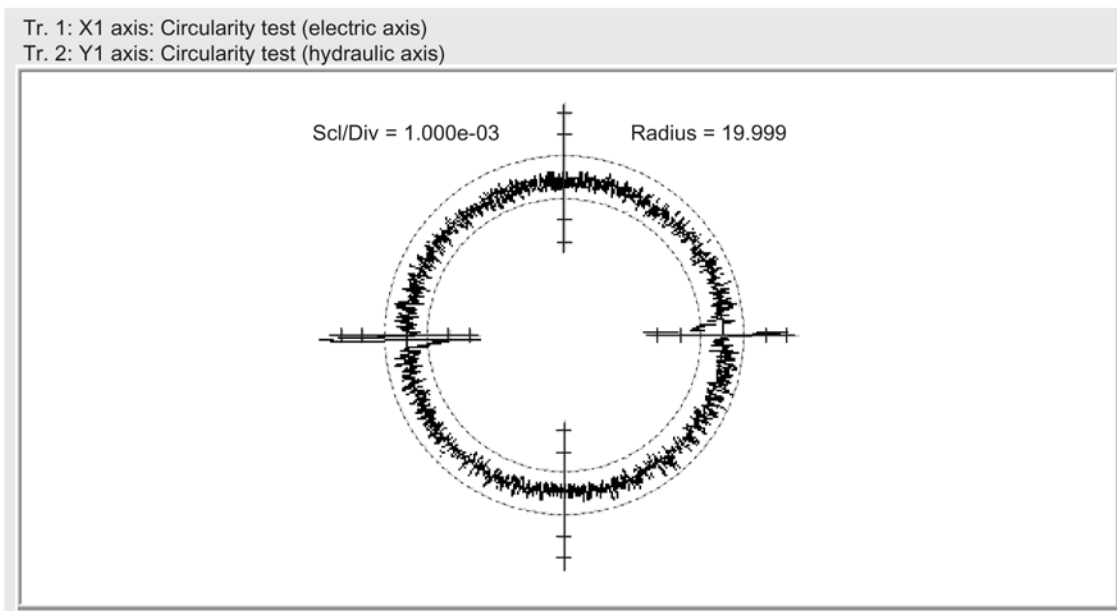
Figure 4-57 Example of circularity test on an HR valve size 06, 15 l/min, transition point 60 %; V=400 mm/min (traversing velocity)
