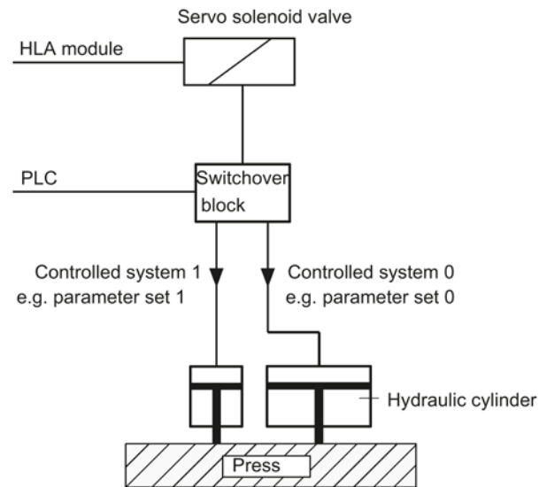
Figure 5-1 Example of a parameter set switchover
