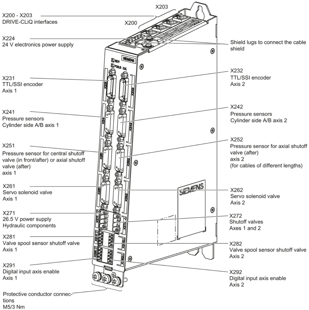
Figure 6-1 Overview of the HLA module interfaces
