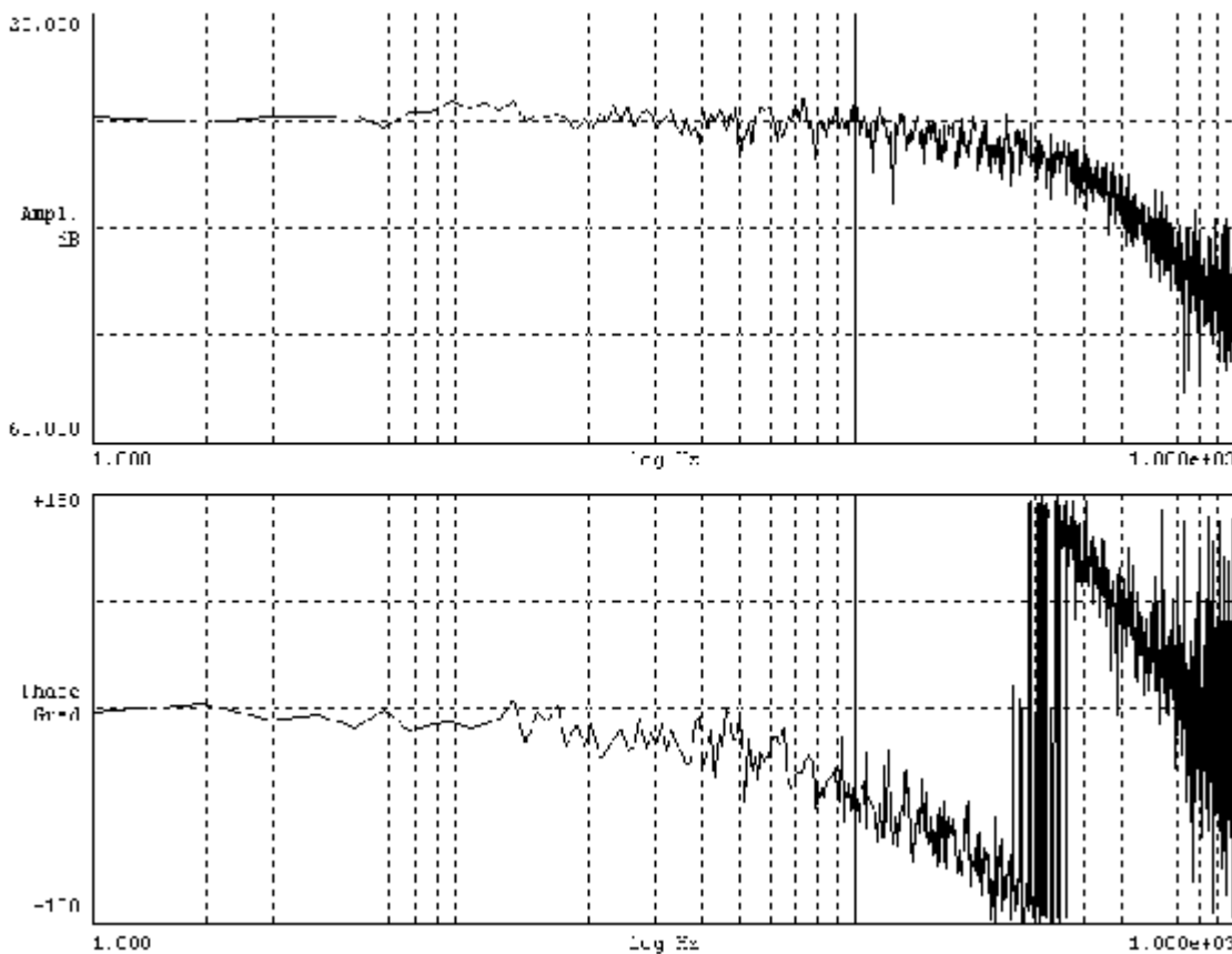
Figure 4-47 Valve frequency response for an HR servo solenoid valve (example)
