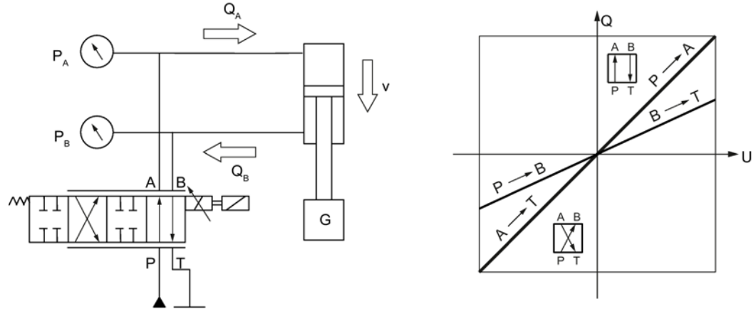
Figure 3-3 Asymmetrical characteristics
