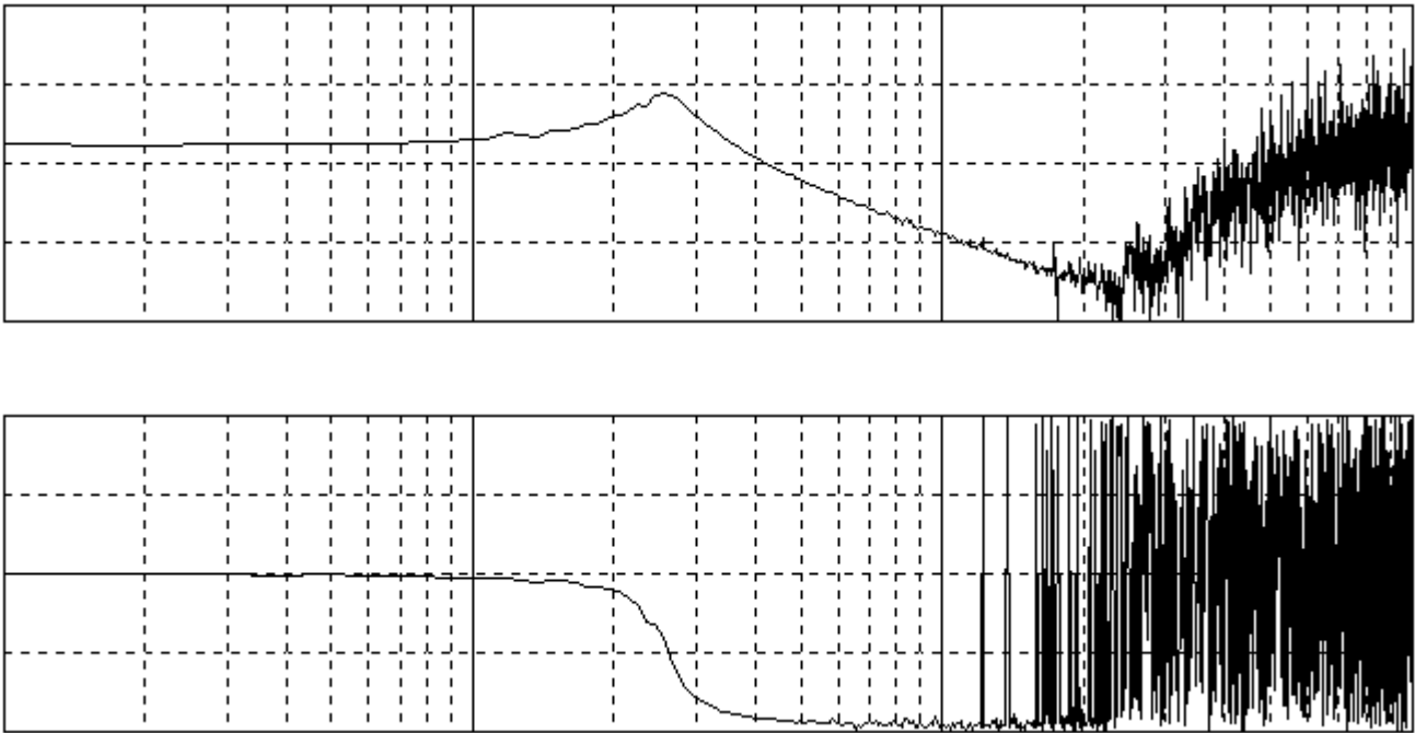
Figure 4-51 Bode diagram showing velocity controlled system v_{act}/Q_{act} (example)
