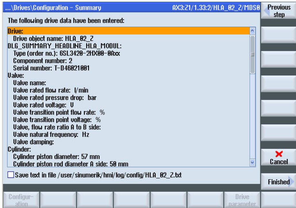
Figure 4-14 Configuration - summary
