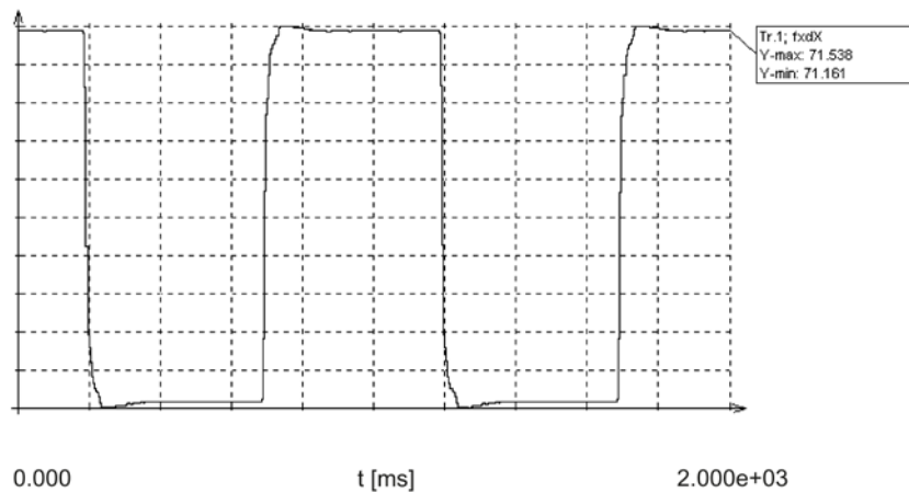
Figure 4-56 Trace "position actual value" for "square-wave" signal at the position setpoint
