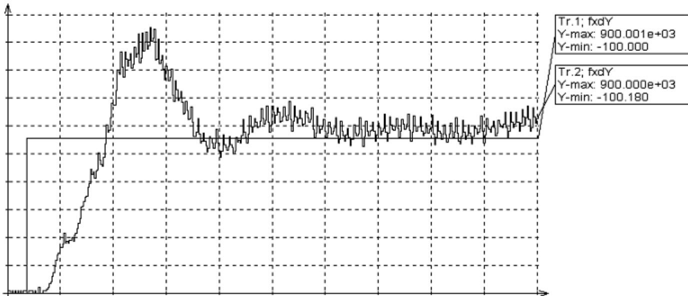
Figure 4-49 Time response of setpoint step change in the velocity control loop (example)
