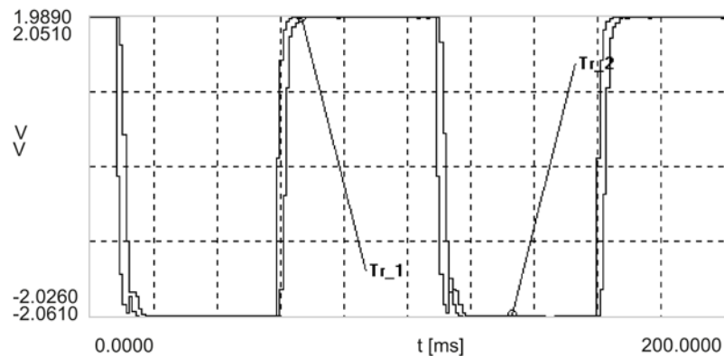
Figure 4-54 Trace "valve actual value" for "square-wave" signal at the valve setpoint
