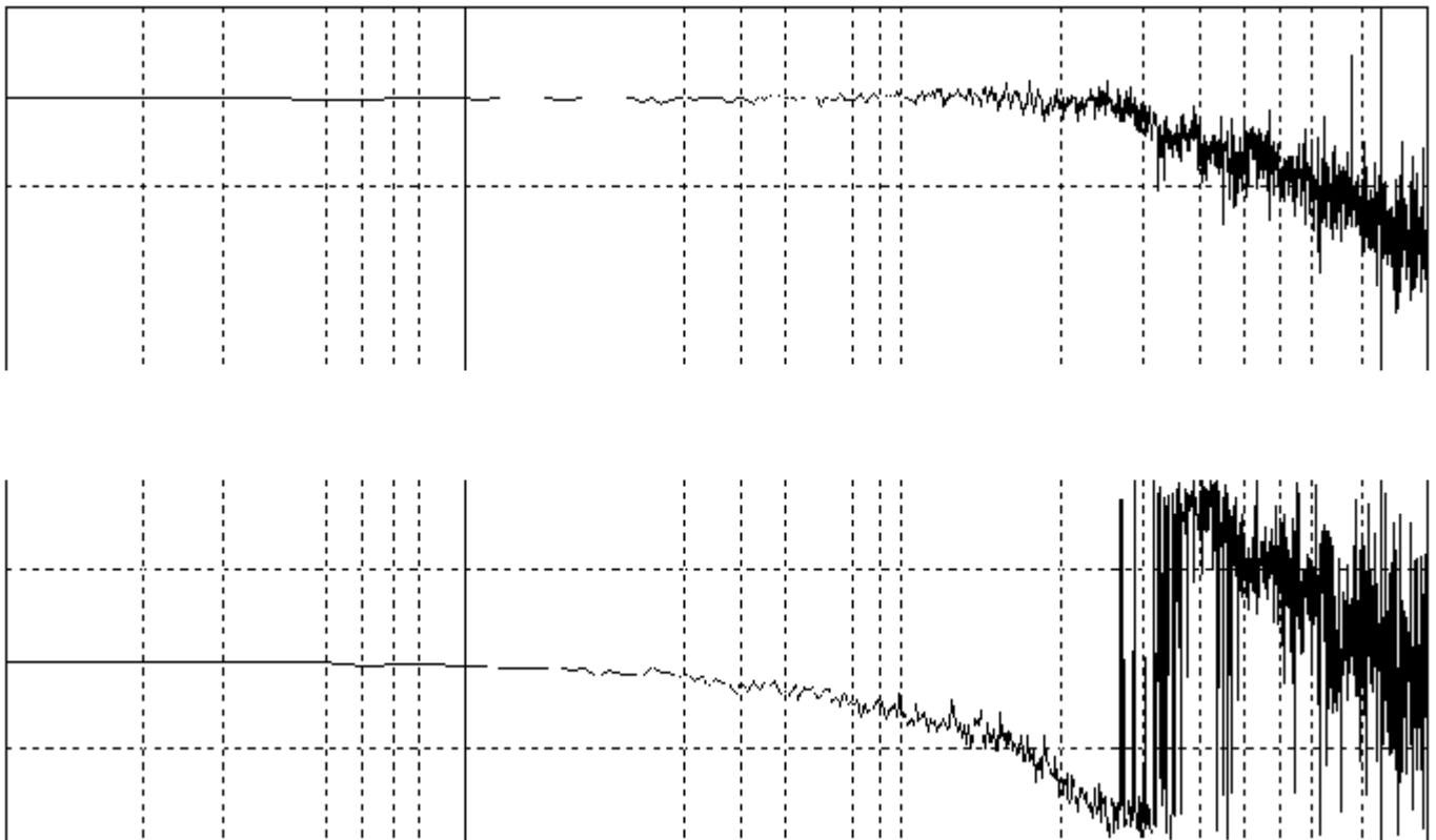
Figure 4-53 Measuring the position control loop (example)
