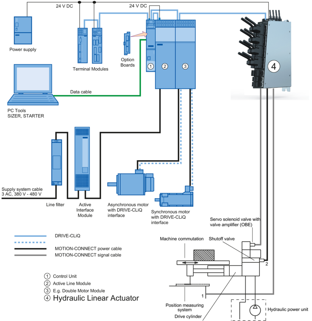
Figure 2-1 Example of a SINAMICS drive system with electrical and hydraulic components
