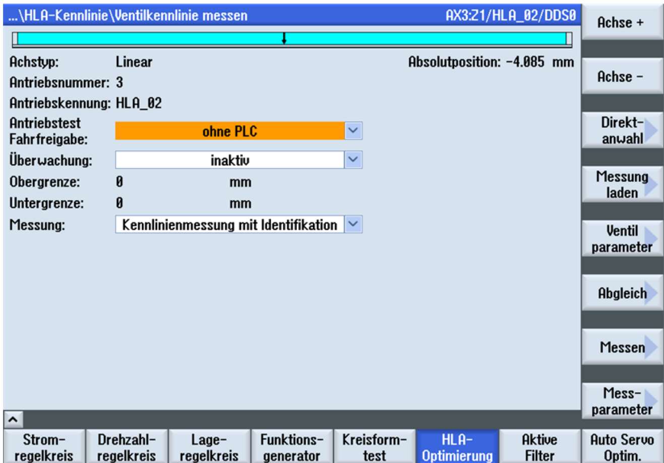
Figure 4-25 Measure valve characteristic
