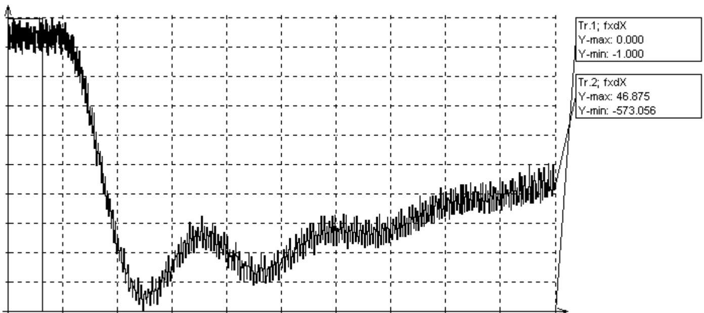
Figure 4-50 Time response of disturbance step change, integral branch of velocity controller deactivated (example)
