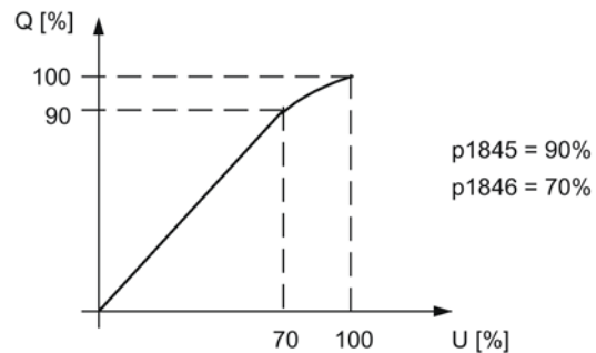
Figure 4-35 Characteristic to linearize the valve
