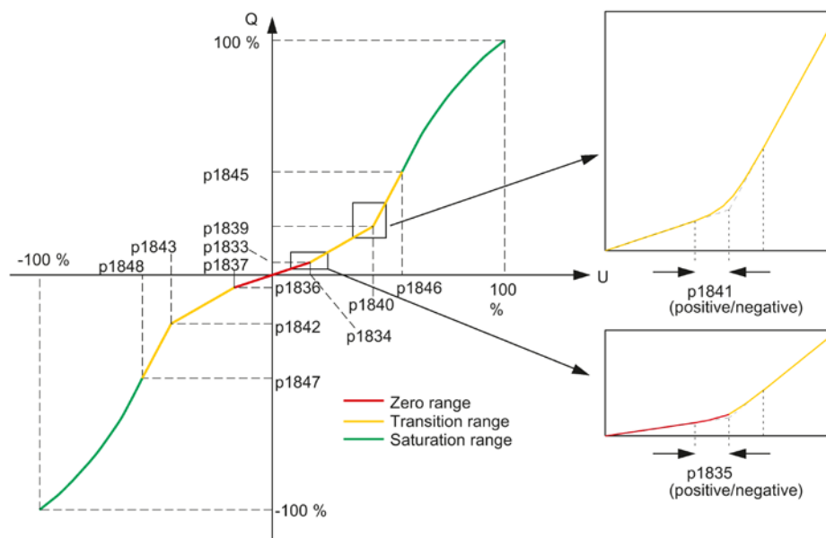
Figure 4-23 Measured characteristic → SINAMICS parameters
