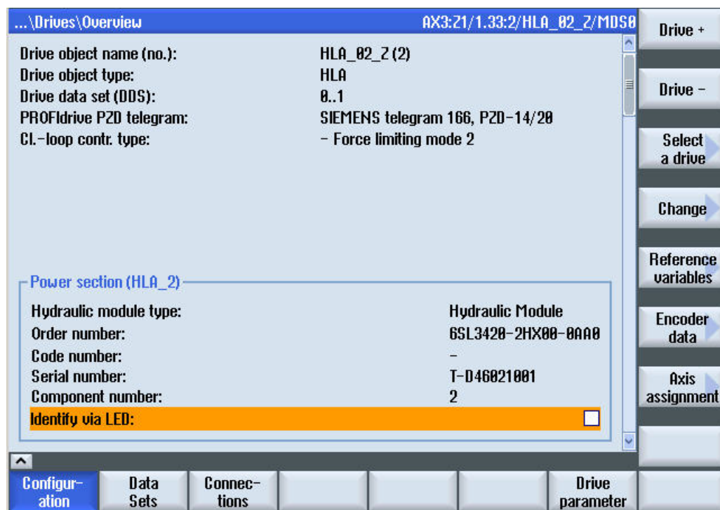
Figure 4-15 Overview of the hydraulic module
