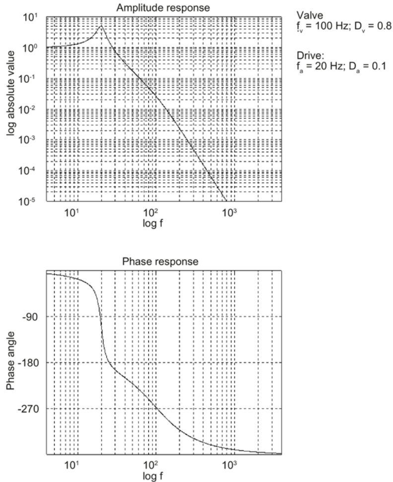
Figure 4-45 Frequency response of controlled system ( f_{\text{valve}} \gg f_{\text{cylinder}} )
