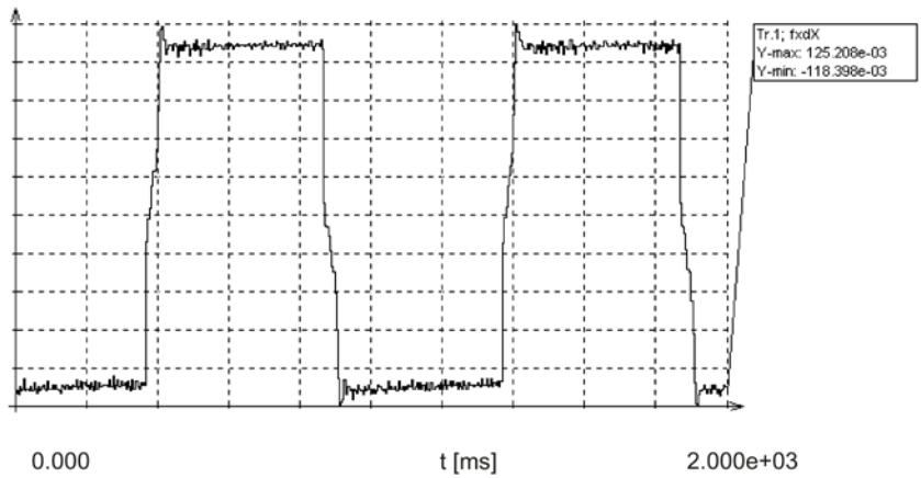
Figure 4-55 Trace "velocity actual value" for "square-wave" signal at the velocity setpoint
