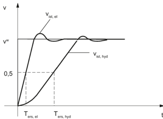
Figure 4-46 Hydraulic/electrical interpolation
