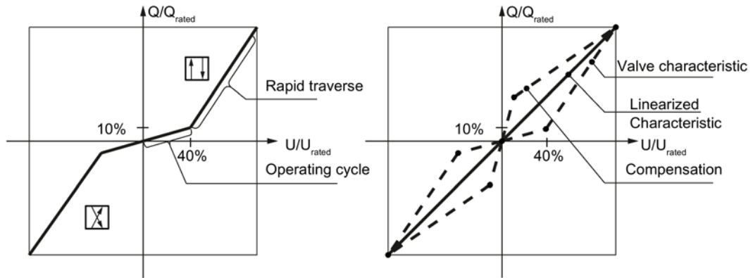
Figure 3-2 Diagram of a servo solenoid valve characteristic with transition point and its compensation in the HLA module
