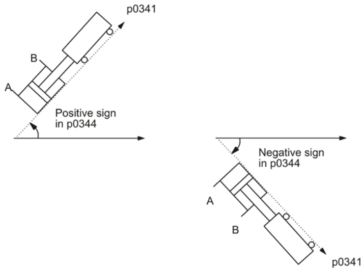
Figure 5-19 Mounting position of the drive referred to the A side
