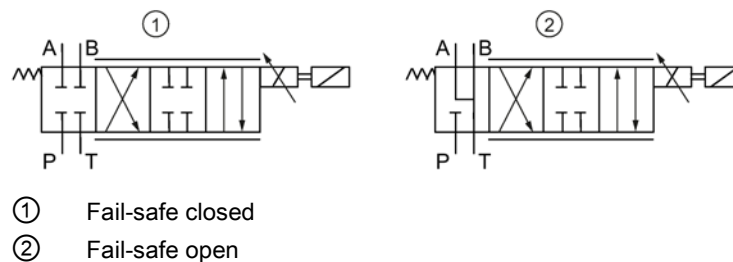
Figure 3-4 Fail-safe position in the valve symbol
