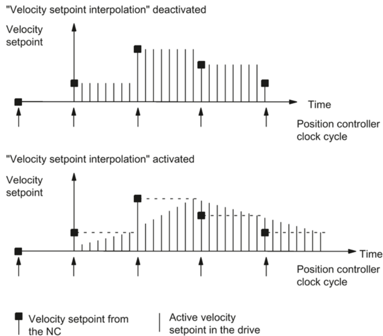
Figure 5-2 Velocity setpoint interpolation
