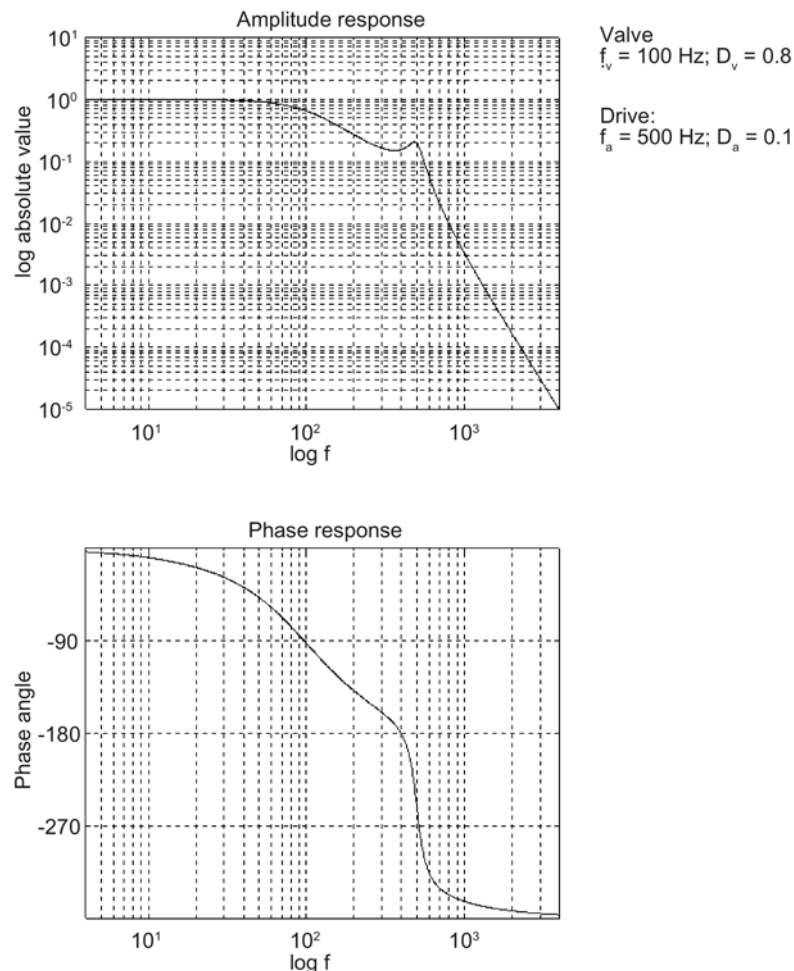
Figure 4-43 Frequency response of controlled system ( f_{\text{valve}} \ll f_{\text{cylinder}} )
