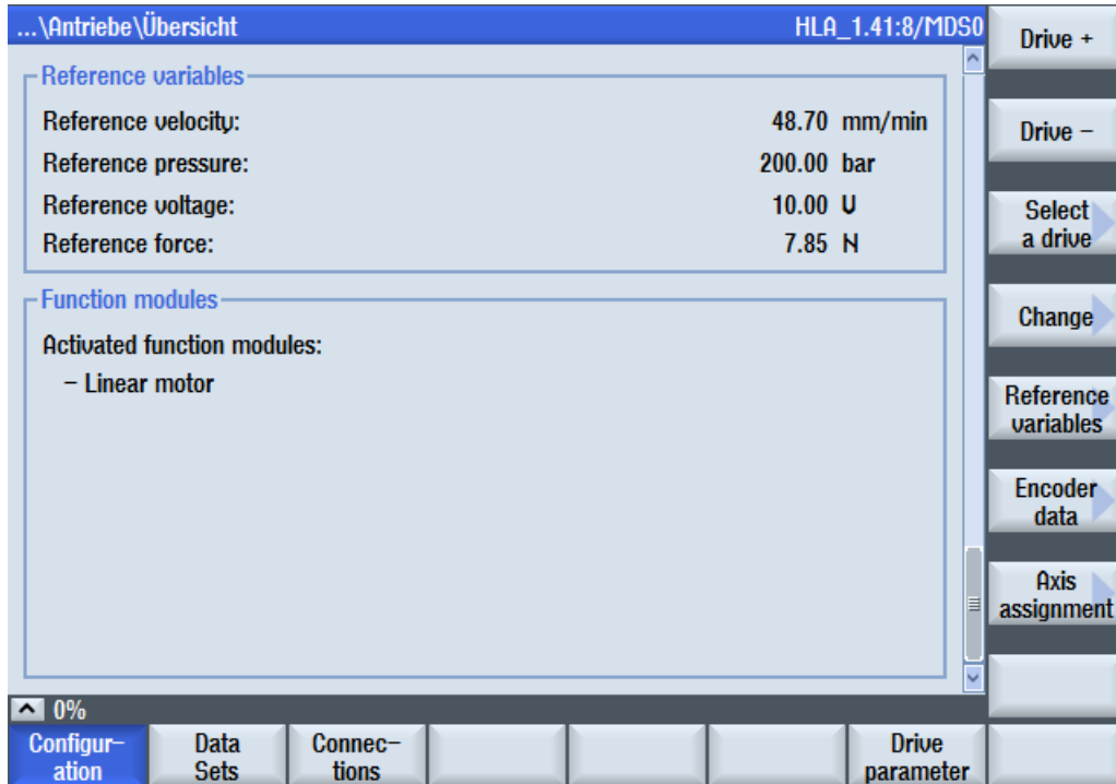
Figure 4-19 Overview of the reference variables/function modules
