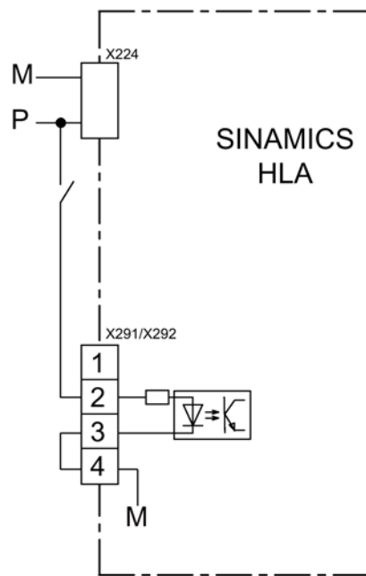
Figure 6-2 Wiring the enabling terminals incl. the internal optocoupler
