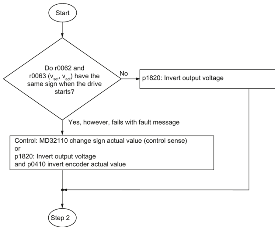
Figure 4-39 Commissioning flowchart, determining the control sense
