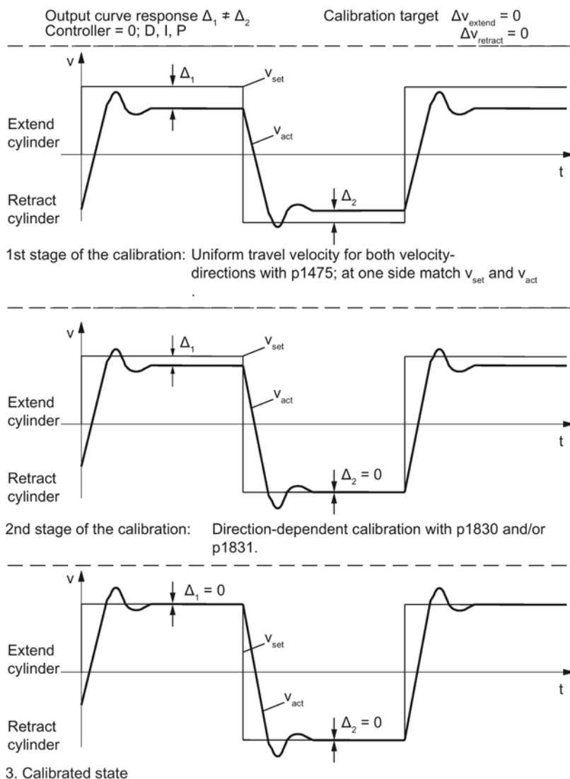
Figure 4-42 Calibrating the controlled system gain
