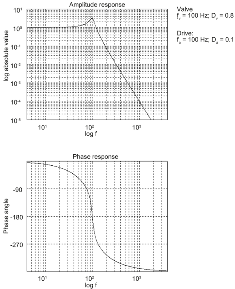
Figure 4-44 Frequency response of controlled system ( f_{\text{valve}} \approx f_{\text{cylinder}} )
