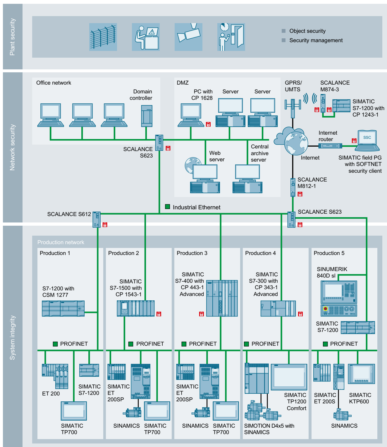
Figure 6-2 SCALANCE S application example
