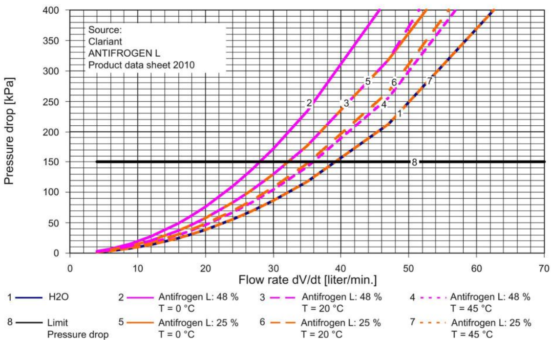
Pressure drop as a function of volumetric flow rate for Active Line Modules in frame size JXL and Motor Modules in frame size JXL
