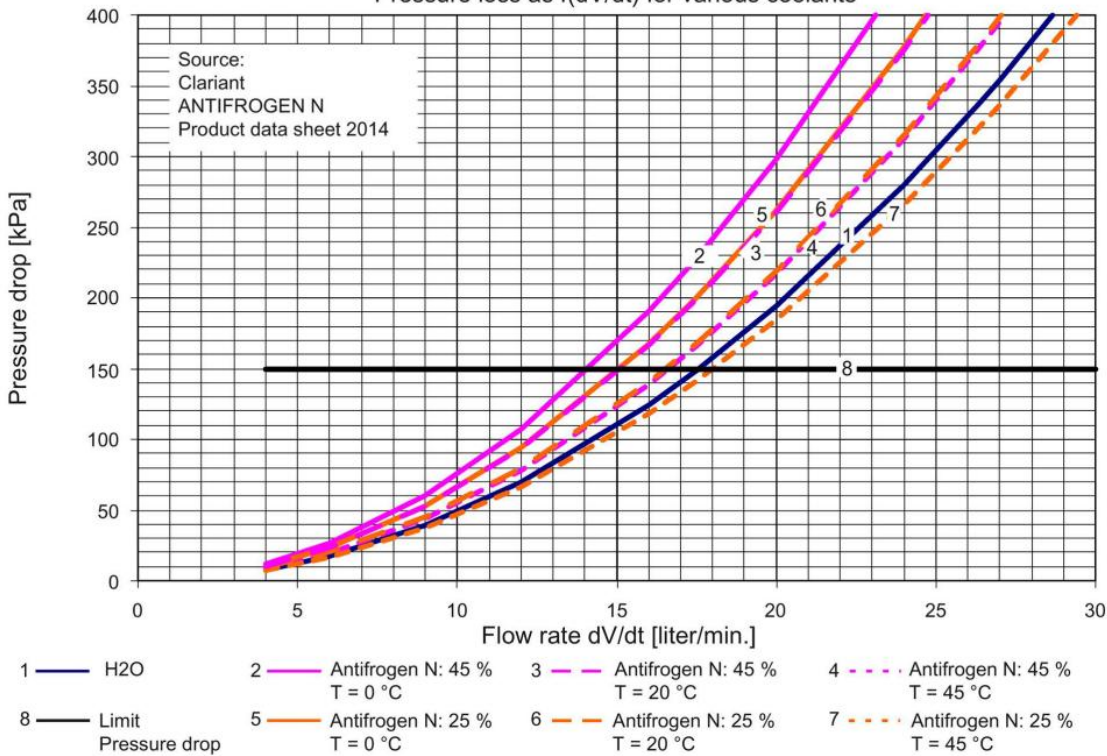
Pressure drop as a function of volumetric flow rate for Power Modules in frame size GL and Motor Modules in frame size GXL
