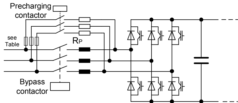
SINAMICS S120 Smart Line Modules: Precharging by means of precharging contactor and precharging resistors
