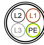
asymmetrical 4-wire cable including the PE conductor
