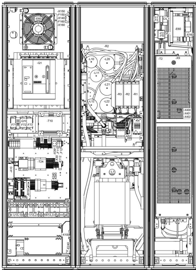
Example of an Active Line Connection Module with degree of protection IP55 (Line Connection Module (on the left) + Active Line Module (on the right) incl. Active Interface Module (in the center))
