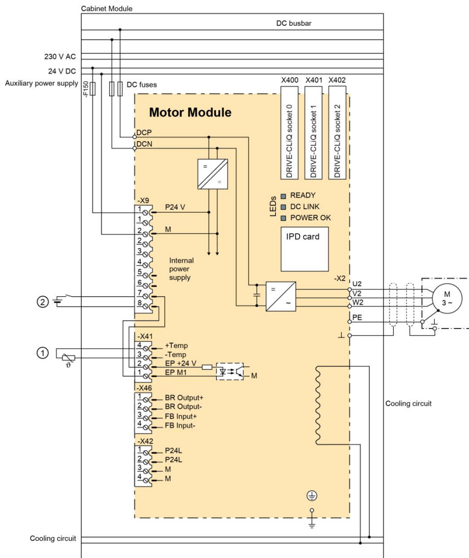
Example of a liquid-cooled Motor Module with DC fuses between the Motor Module and the DC busbar
