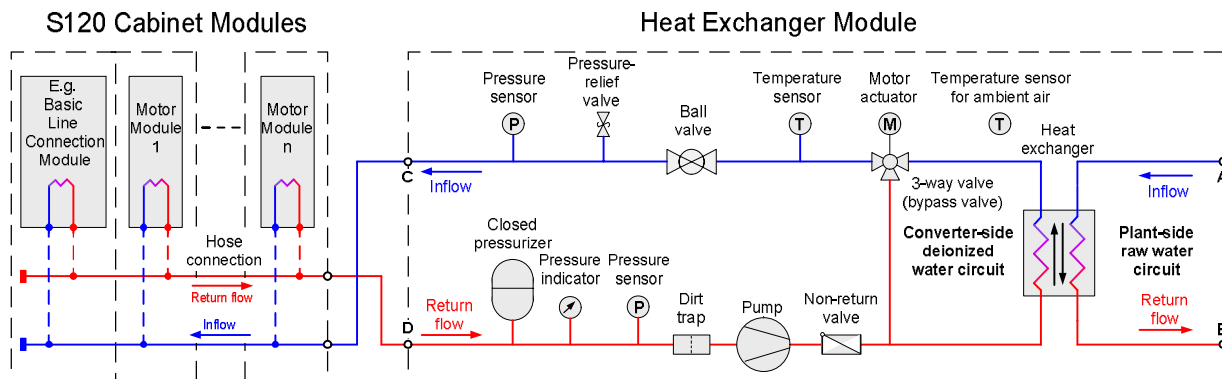
S120 Cabinet Modules: Schematic diagram of the converter-side deionized water circuit and the Heat Exchanger Module
