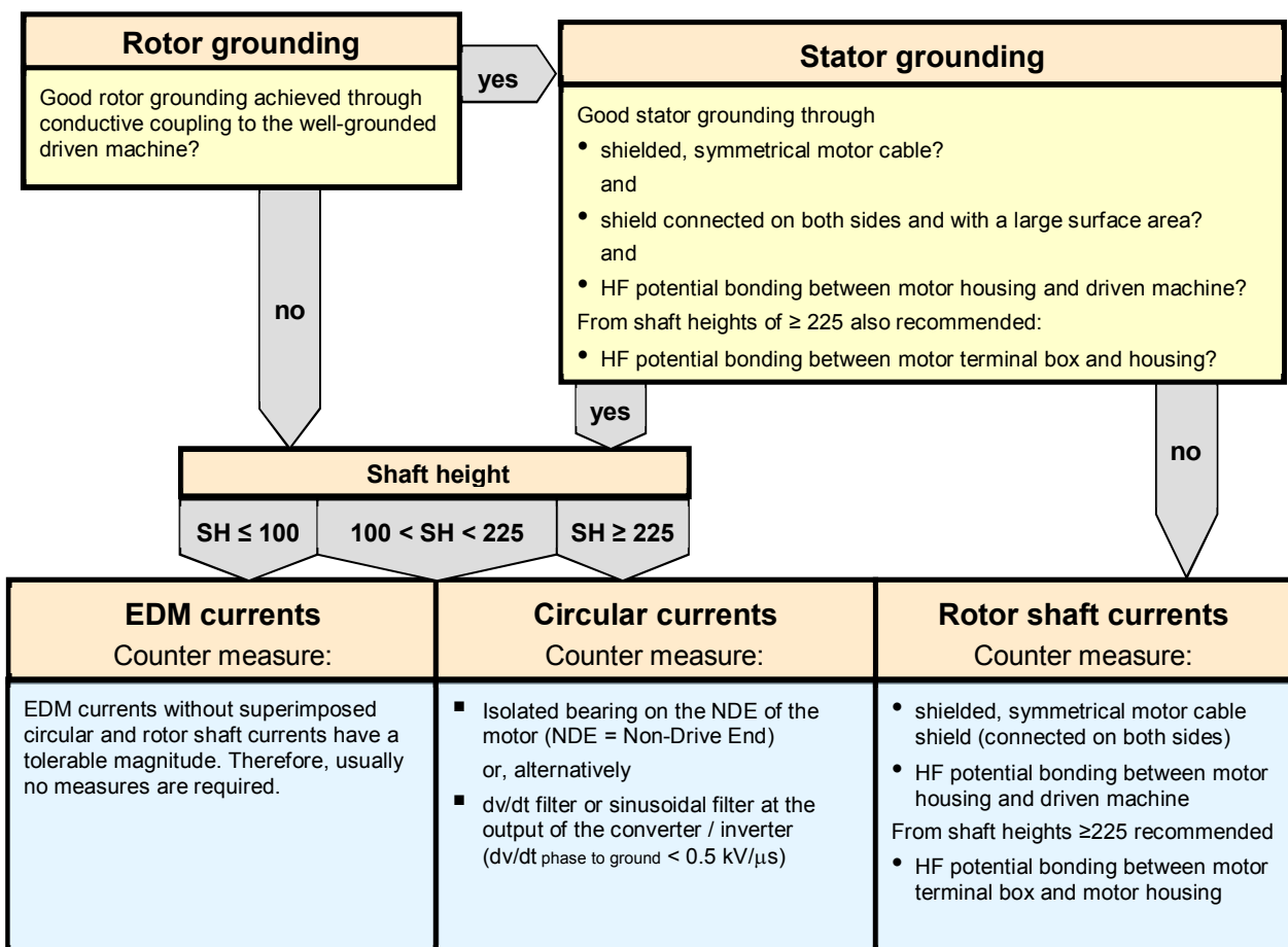
Dominant bearing current types dependent on the shaft height and the grounding conditions of stator and rotor
