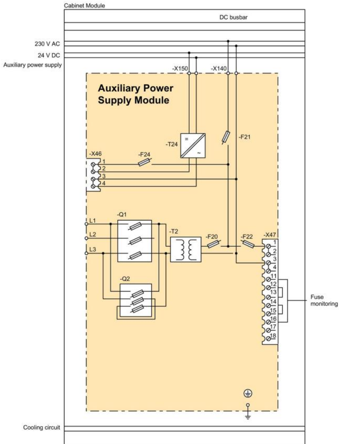
Design of the Auxiliary Power Supply Module for liquid-cooled SINAMICS S120 Cabinet Modules
