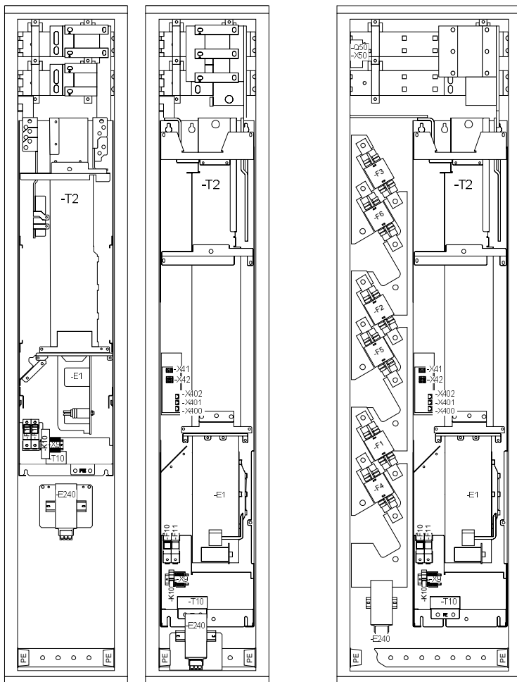
Air-cooled Basic Line Modules in frame sizes FB and GB / GD, and Basic Line Module for parallel connections
