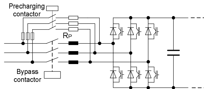
Precharging with S120 Smart Line Modules via precharging contactor and precharging resistors
