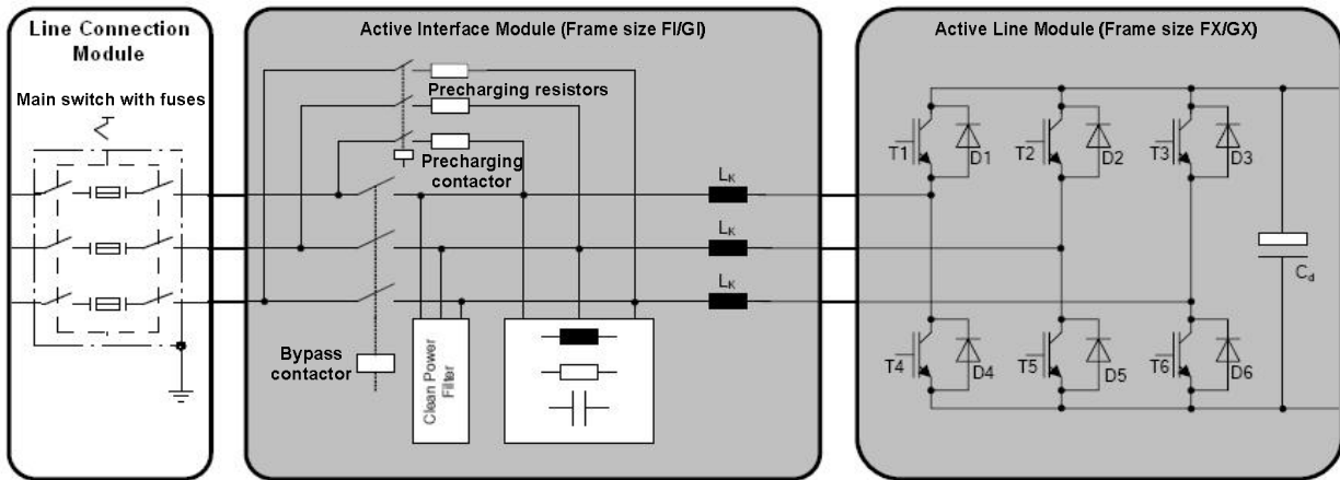
Precharging with air-cooled Active Line Modules + Active Interface Modules in frame sizes FX+FI and GX+GI
