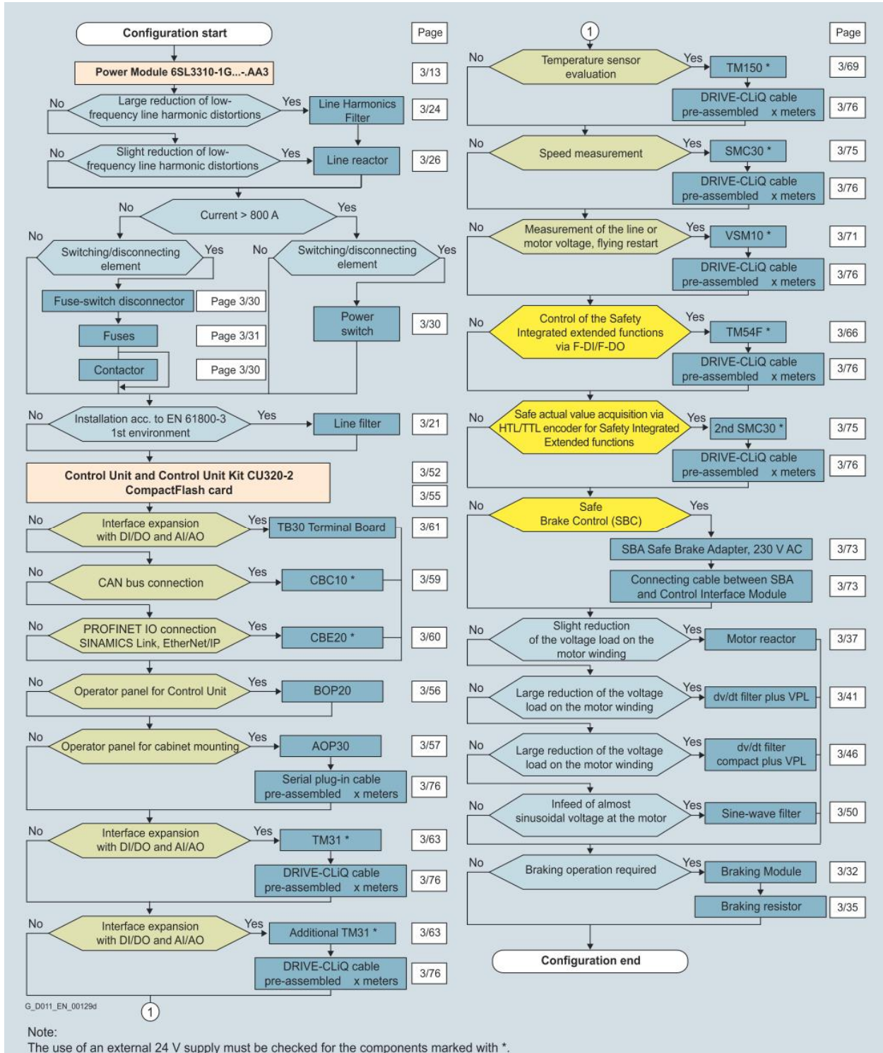
Flowchart for selecting the components of a drive system with SINAMICS G130 converter Chassis units
