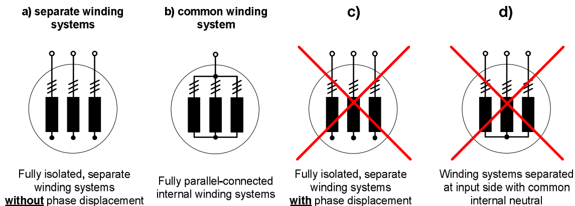
Admissible and inadmissible winding systems for parallel connections of converters illustrated by the example of motors with three parallel windings
