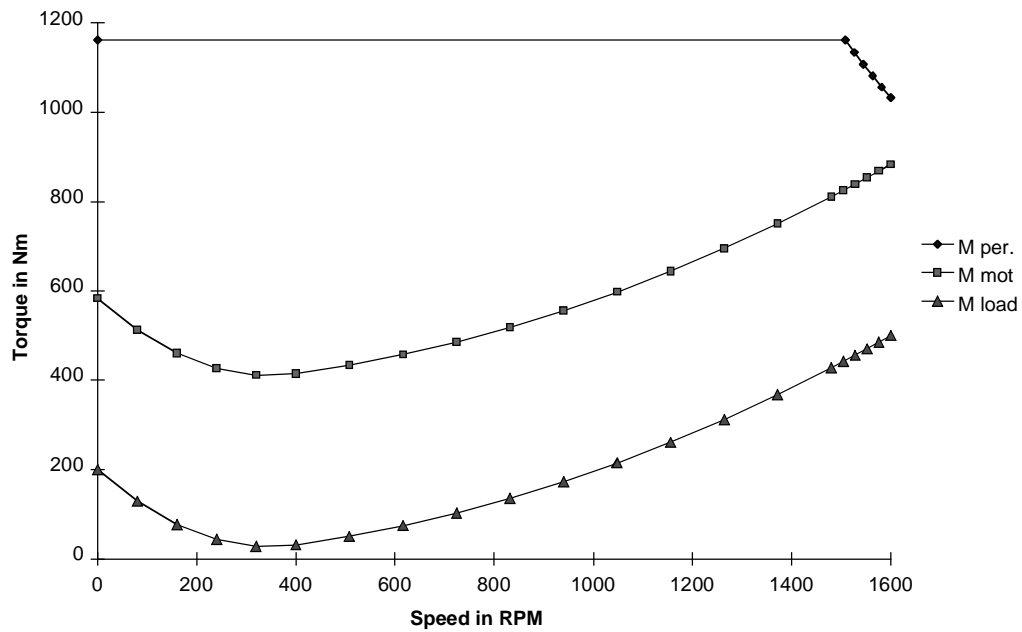
Load torque, motor torque and permissible torque as a function of the speed
