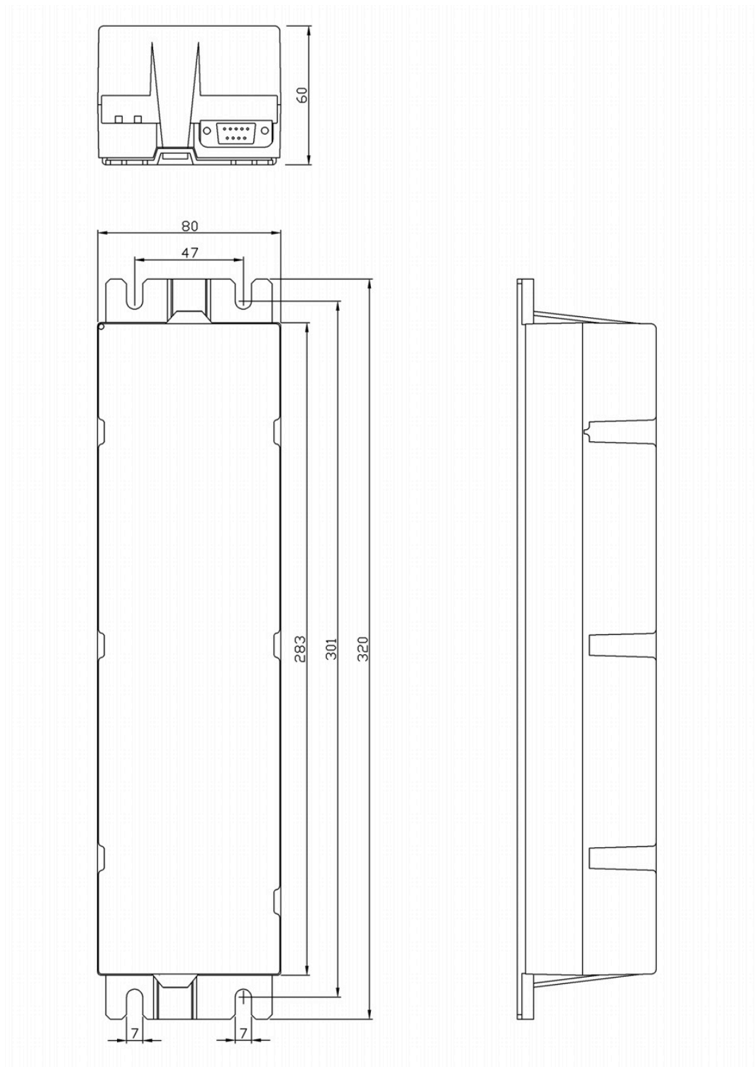
Figure 5-3 Controller
