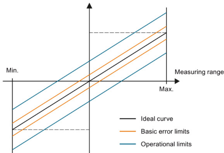
Figure 2-13 Operational and basic error limits
