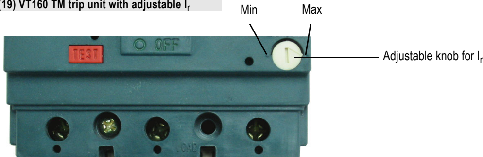
(19) VT160 TM trip unit with adjustable I_r
