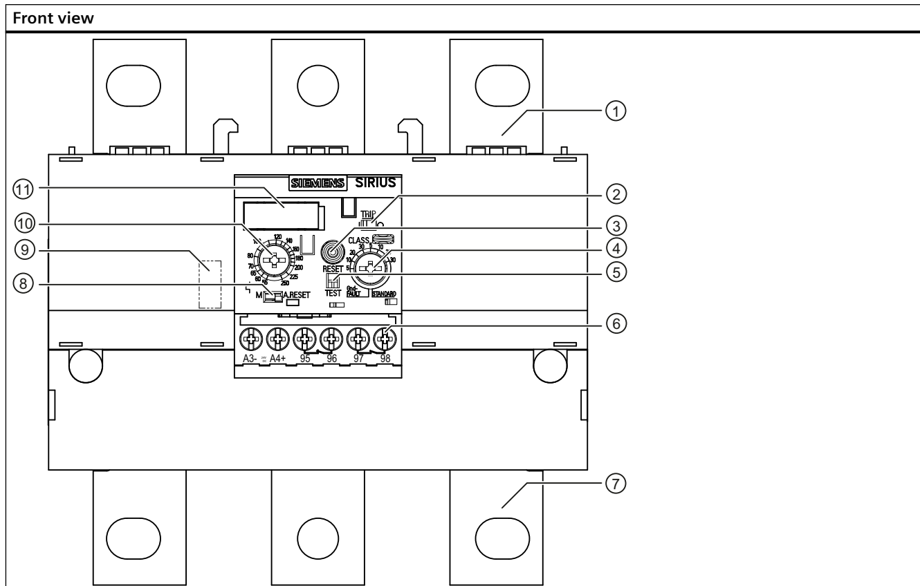
3RB2163 overload relay equipment
