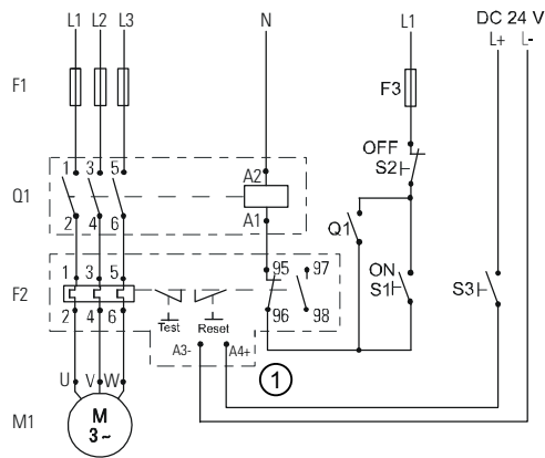
① Electrical remote RESET (3RB21 / 3RB31 only)
