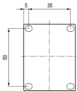
Figure C-45 Drilling plan for contactors with screw-type connections and ring cable lug connections (size S00)
