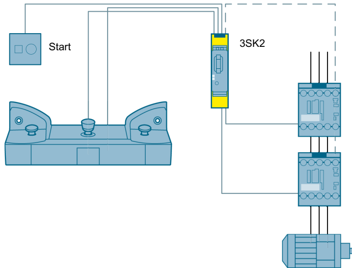
Figure 3-45 Two-hand operation to SIL 3 or PL e with a 3SK2 safety relay
