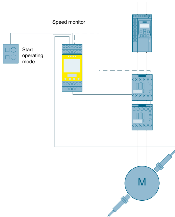
Figure 3-41 Safe speed monitoring to SIL 3 or PL e with a speed monitor
