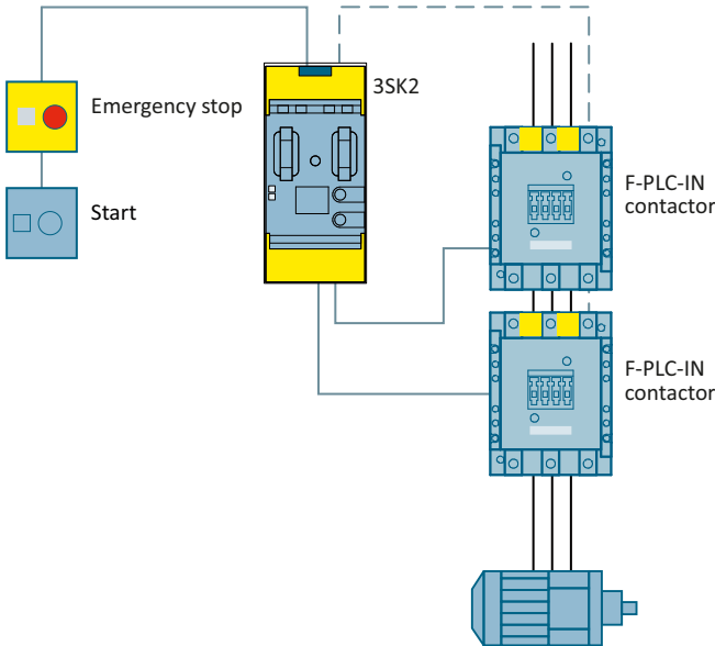
Figure 3-12 Emergency stop shutdown to SIL 3 or PL e with contactors with F-PLC-IN and 3SK2 safety relay
