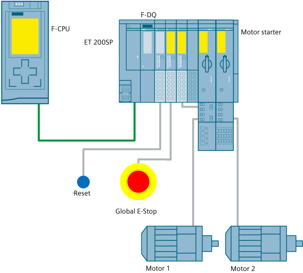
Figure 3-16 Emergency stop shutdown to SIL 3 or PL e with fail-safe digital output module and fail-safe motor starters in the ET 200SP system
