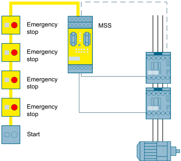
Figure 3-11 Emergency stop shutdown via AS-i to SIL 3 or PL e with a Modular Safety System
