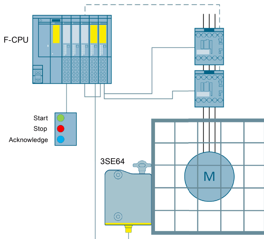
Figure 3-34 Protective door monitoring with tumbler by means of a 3SE64 RFID safety switch up to SIL 3 or PL e and a fail-safe controller
