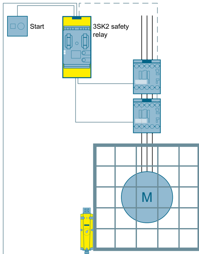
Figure 3-31 Protective door monitoring with tumbler to SIL 2 or PL d with a 3SK2 safety relay
