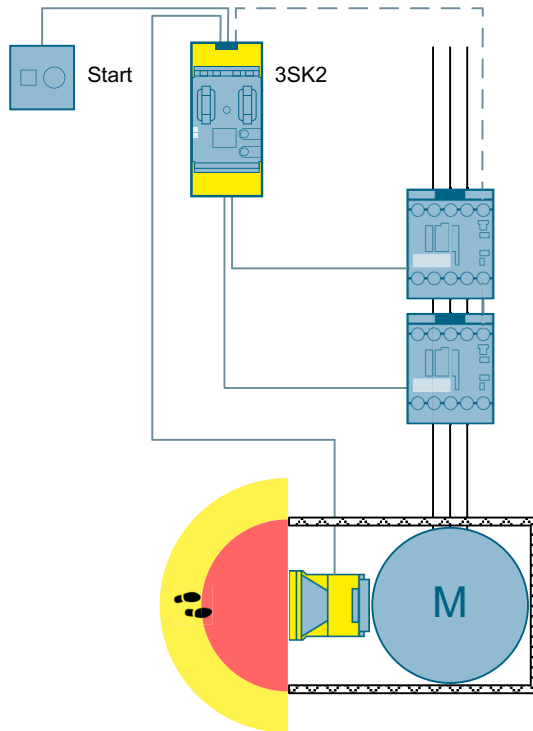
Figure 3-40 Area monitoring using a laser scanner to SIL 2 or PL d with a 3SK2 safety relay
