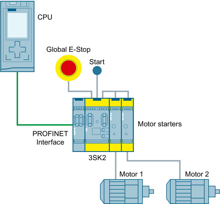
Figure 3-18 Emergency stop shutdown up to SIL 3 or PL e via 3SK2 safety relay with PROFINET connection and fail-safe motor starters
