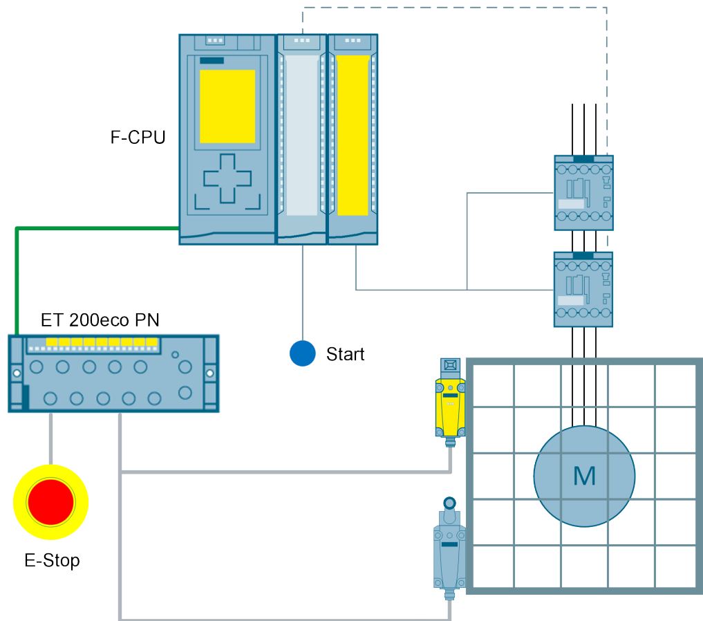
Figure 3-56 Emergency stop shutdown and protective door monitoring up to SIL 3 or PL e via ET 200ecoPN and F-CPU
