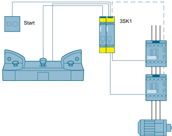
Figure 3-44 Two-hand operation to SIL 3 or PL e with a 3SK1 safety relay
