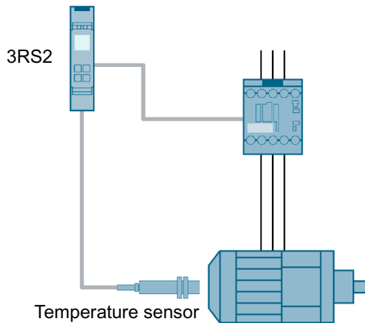
Figure 3-46 Safe temperature monitoring up to SIL 1 or PL c with a 3RS2 temperature monitoring relay
