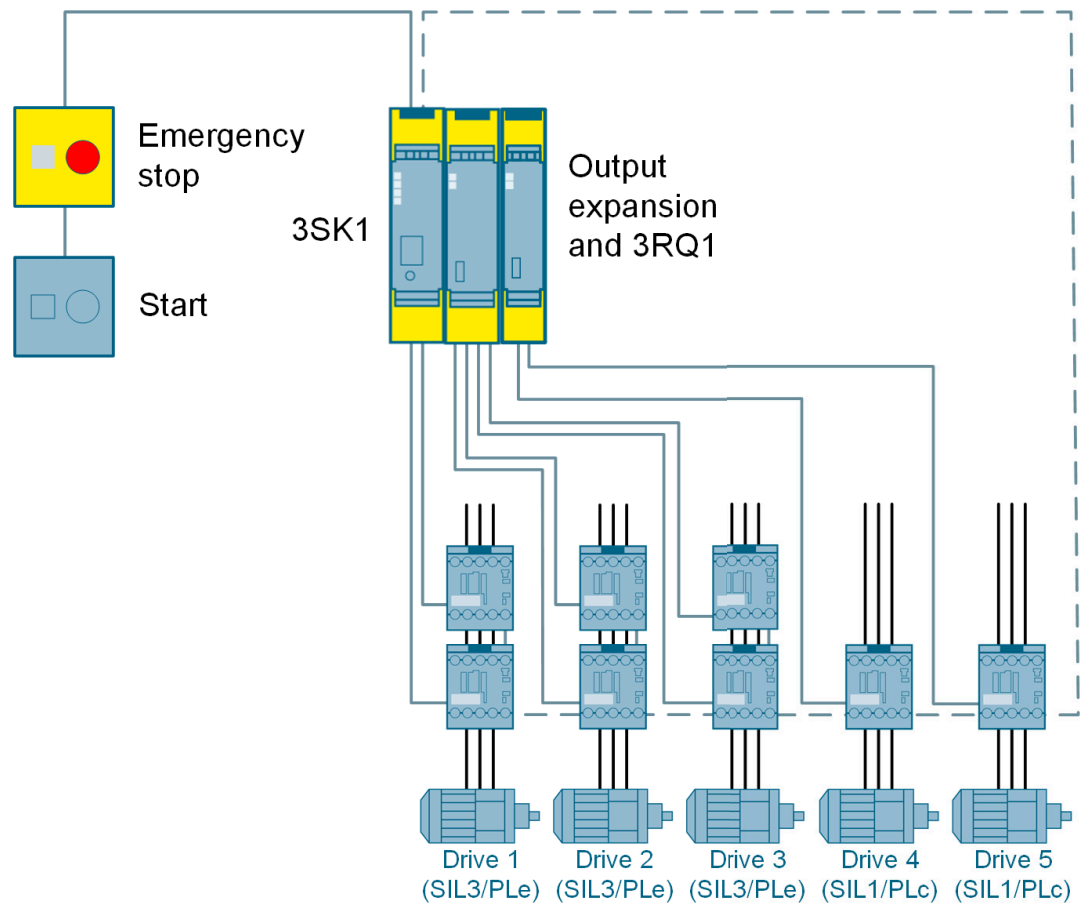
Figure 3-57 Emergency stop shutdown of multiple motors to SIL 3 or PL e with a 3SK1 safety relay
