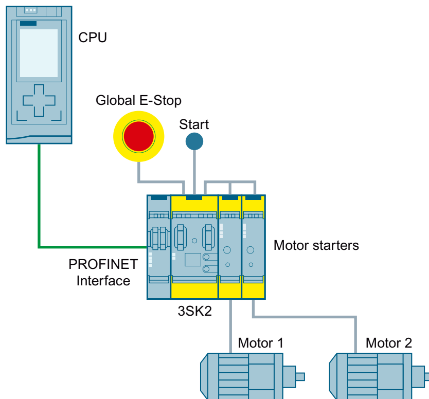
Figure 3-19 Emergency stop group shutdown up to SIL 3 or PL e via 3SK2 safety relay with PROFINET connection and fail-safe motor starters
