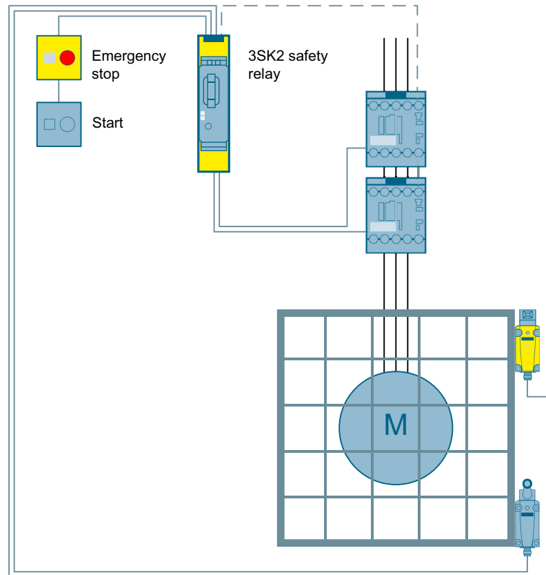
Figure 3-50 Emergency stop monitoring and protective door monitoring to SIL 3 or PL e with a 3SK2 safety relay
