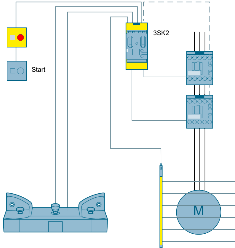
Figure 3-51 Access monitoring using a light curtain with two-hand operation and emergency stop to SIL 3 or PL e with a 3SK2 safety relay
