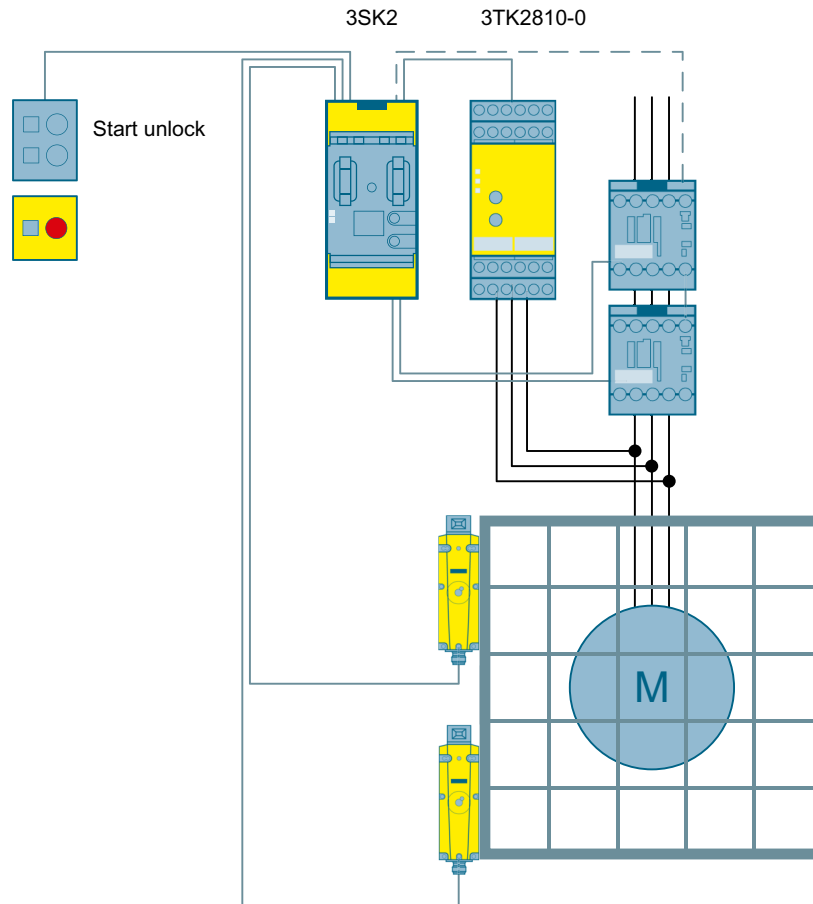
Figure 3-42 Safe standstill monitoring including protective door tumbler to SIL 3 or PL e with a 3SK2 safety relay
