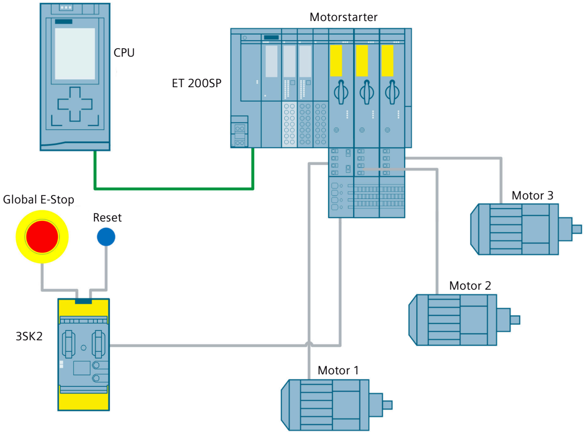
Figure 3-15 Emergency stop shutdown to SIL 3 or PL e with fail-safe motor starters in the ET 200SP system and a 3SK2 safety relay
