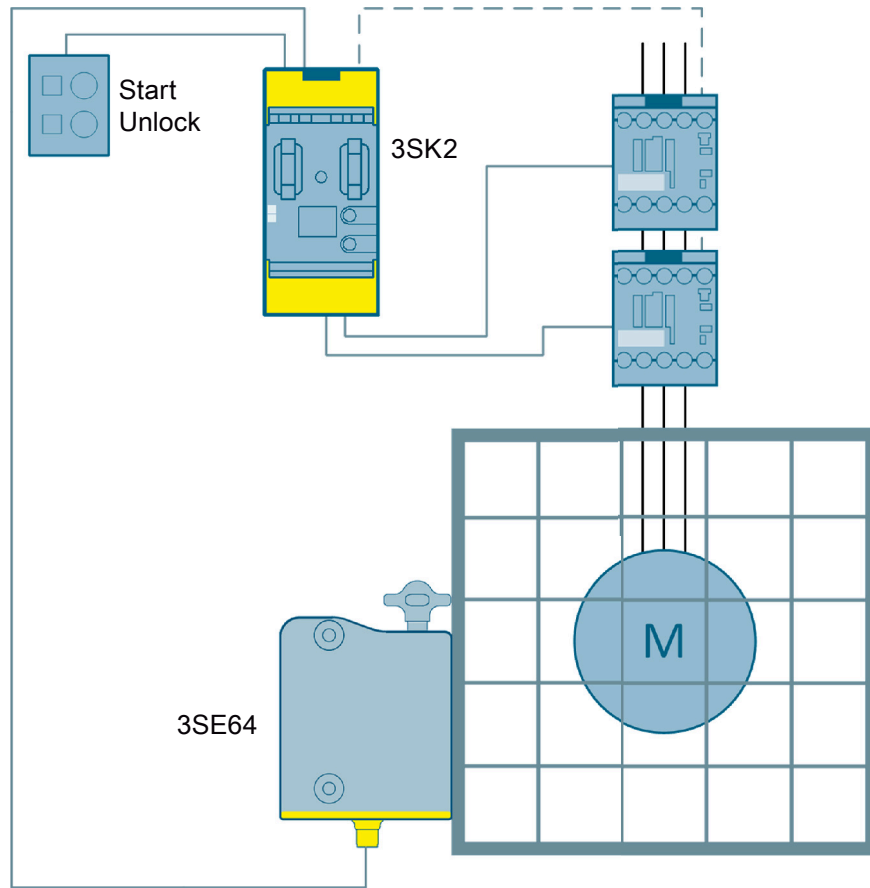
Figure 3-33 Protective door monitoring with tumbler by means of a 3SE64 RFID safety switch up to SIL 3 or PL e and a 3SK2 safety relay
