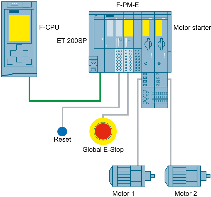
Figure 3-17 Emergency stop shutdown to SIL 3 or PL e with fail-safe power module and fail-safe motor starters in the ET 200SP system
