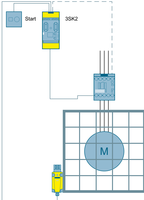
Figure 3-23 Protective door monitoring to SIL 1 or PL c with a 3SK2 safety relay
