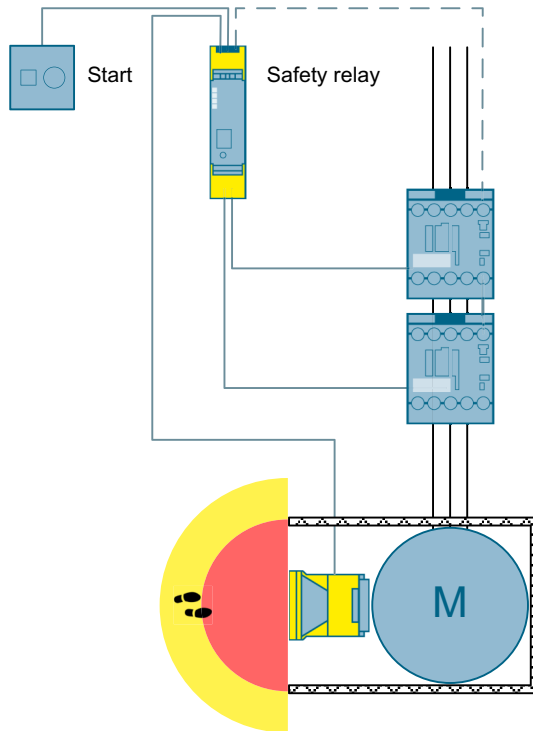
Figure 3-39 Area monitoring using a laser scanner to SIL 2 or PL d with a 3SK1 safety relay
