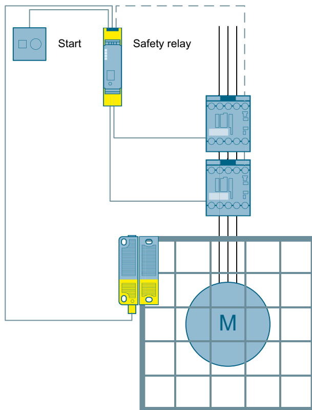
Figure 3-29 Protective door monitoring by means of RFID switch to SIL 3 or PL e with a 3SK1 safety relay
