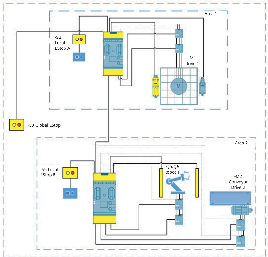
Figure 3-59 Cascading of 3SK2 safety relays up to SIL 3 or PL e
