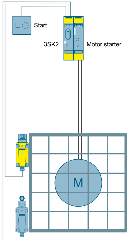
Figure 3-27 Protective door monitoring to SIL 3 or PL e with fail-safe motor starters and a 3SK2 safety relay
