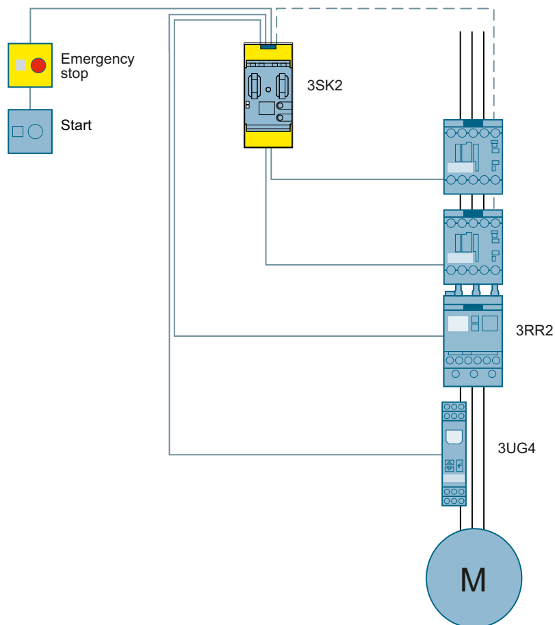
Figure 3-48 Safe current monitoring including emergency stop shutdown up to PL d with a 3SK2 safety relay and two current monitoring relays
