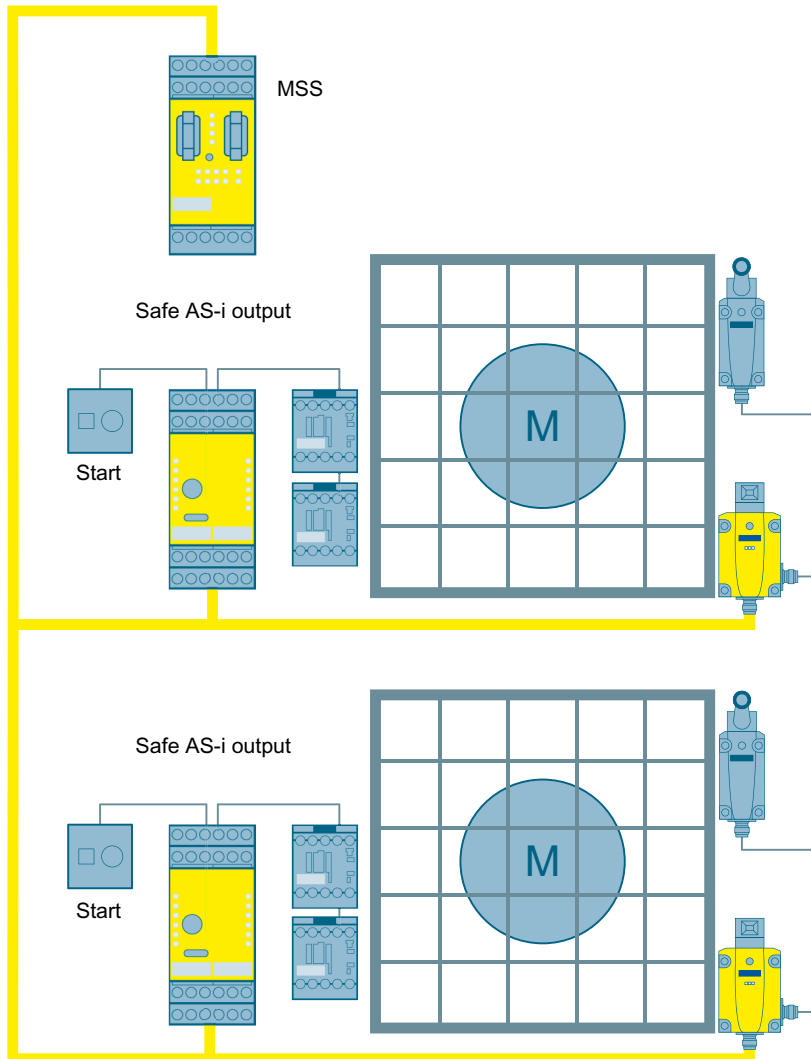
Figure 3-28 Protective door monitoring via AS-i to SIL 3 or PL e with a Modular Safety System
