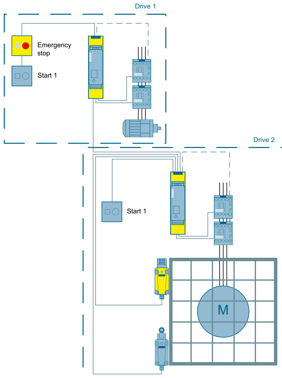
Figure 3-52 Cascading of 3SK1 safety relays to SIL 3 or PL e
