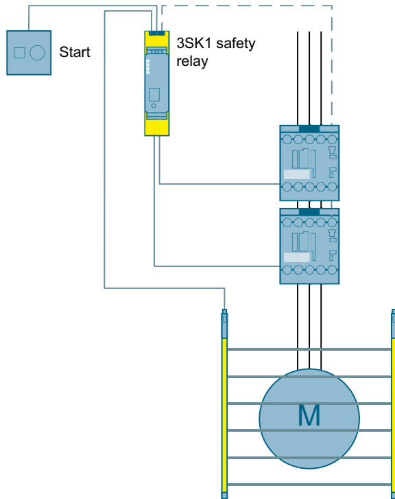
Figure 3-35 Access monitoring using a light curtain to SIL 3 or PL e with a 3SK1 safety relay
