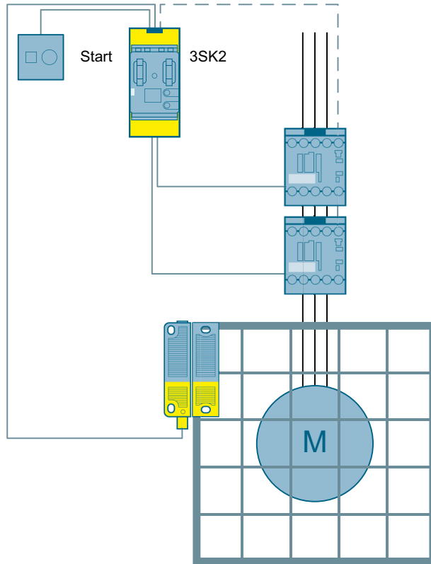
Figure 3-30 Protective door monitoring by means of RFID switch to SIL 3 or PL e with a 3SK2 safety relay
