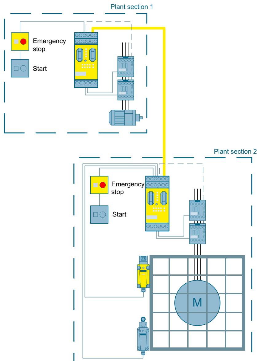
Figure 3-53 Safe slave-to-slave communication between several plant sections to SIL 3 or PL e via AS-i
