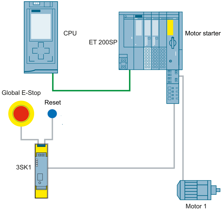
Figure 3-14 Emergency stop shutdown to SIL 3 or PL e with a fail-safe motor starter in the ET 200SP system and a 3SK1 safety relay
