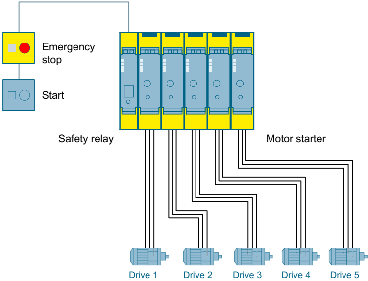
Figure 3-9 Emergency stop shutdown to SIL 3 or PL e with fail-safe motor starters and a 3SK1 safety relay
