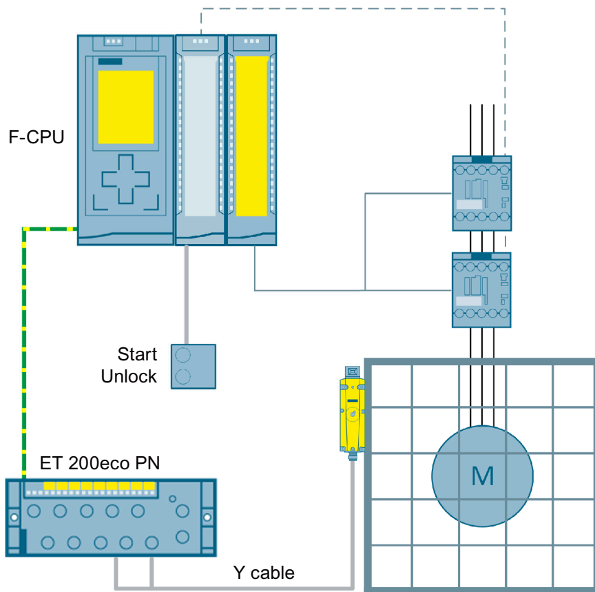
Figure 3-32 Protective door monitoring with tumbler up to SIL 2 or PL d e via ET 200eco PN and F-CPU
