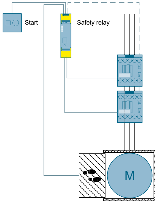
Figure 3-37 Access monitoring using a safety mat to SIL 3 or PL e with a 3SK1 safety relay
