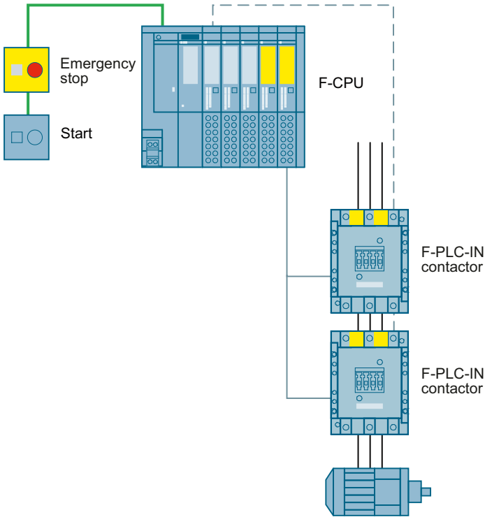
Figure 3-13 Emergency stop shutdown to SIL 3 or PL e with contactors with F-PLC-IN and fail-safe controller
