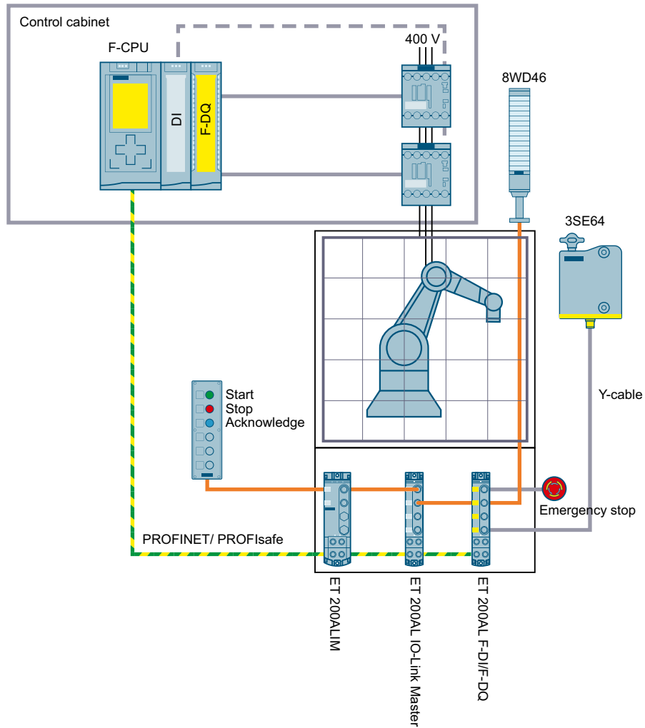
Figure 3-58 Protective door monitoring with tumbler by means of a 3SE64 RFID safety switch including emergency stop shutdown up to SIL 3 or PL e and via ET 200AL and F-CPU
