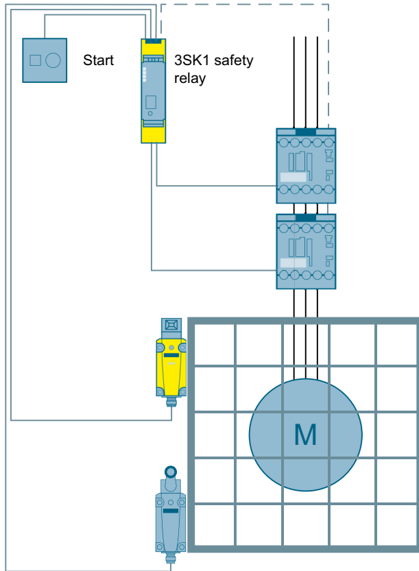
Figure 3-24 Protective door monitoring to SIL 3 or PL e with a 3SK1 safety relay
