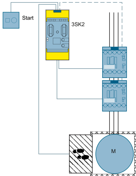
Figure 3-38 Access monitoring using a safety mat to SIL 3 or PL e with a 3SK2 safety relay
