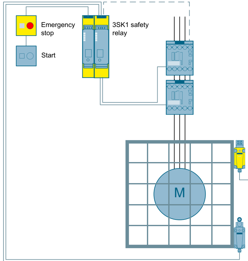
Figure 3-49 Emergency stop monitoring and protective door monitoring to SIL 3 or PL e with a 3SK1 safety relay
