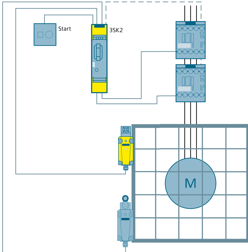
Figure 3-25 Protective door monitoring to SIL 3 or PL e with fail-safe motor starters and a 3SK2 safety relay
