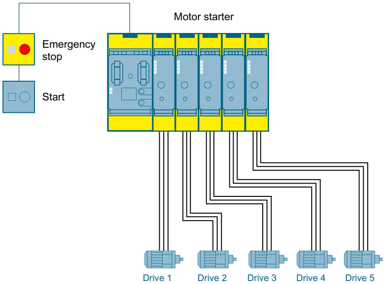
Figure 3-10 Emergency stop shutdown to SIL 3 or PL e with fail-safe motor starters and a 3SK2 safety relay
