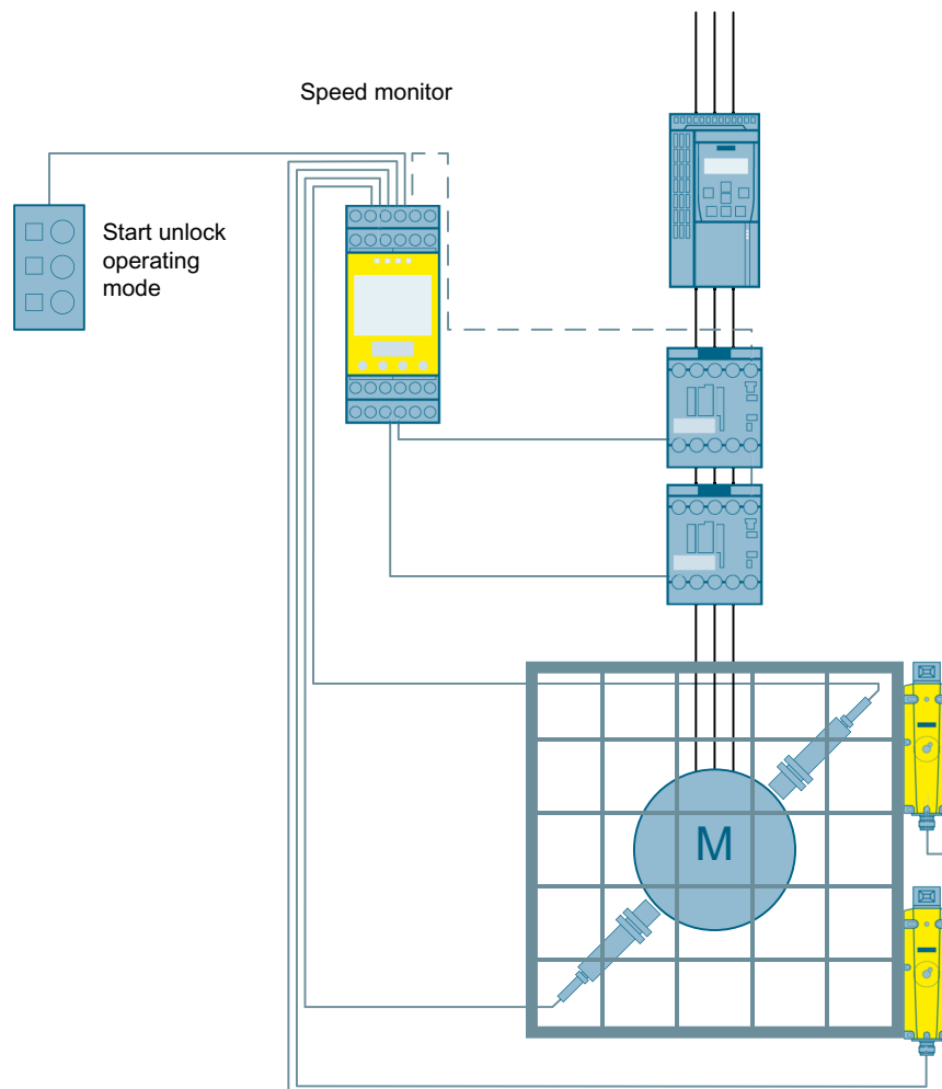
Figure 3-43 Safe speed monitoring, protective door monitoring and tumbler monitoring to SIL 3 or PL e with a speed monitor
