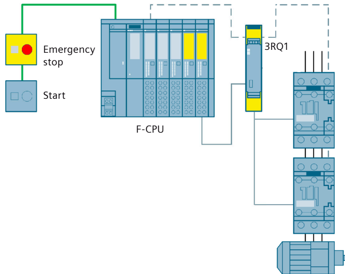
Figure 3-21 Emergency stop shutdown to SIL 3 or PL e with a 3RQ1 coupling relay and fail-safe controller
