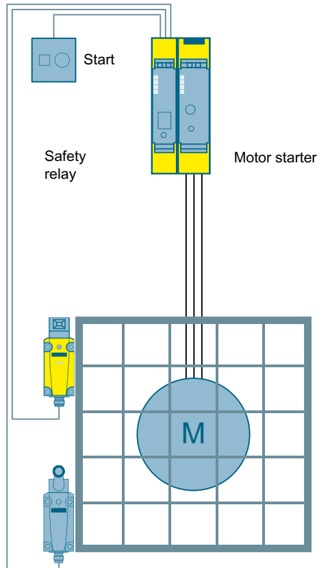
Figure 3-26 Protective door monitoring to SIL 3 or PL e with a fail-safe motor starter and a 3SK1 safety relay
