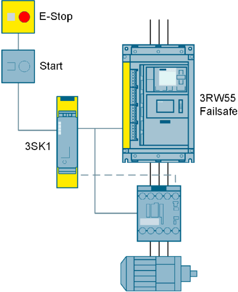
Figure 3-20 Emergency stop shutdown up to SIL 3 or PL e with a 3RW55 Failsafe soft starter and 3SK1 safety relay
