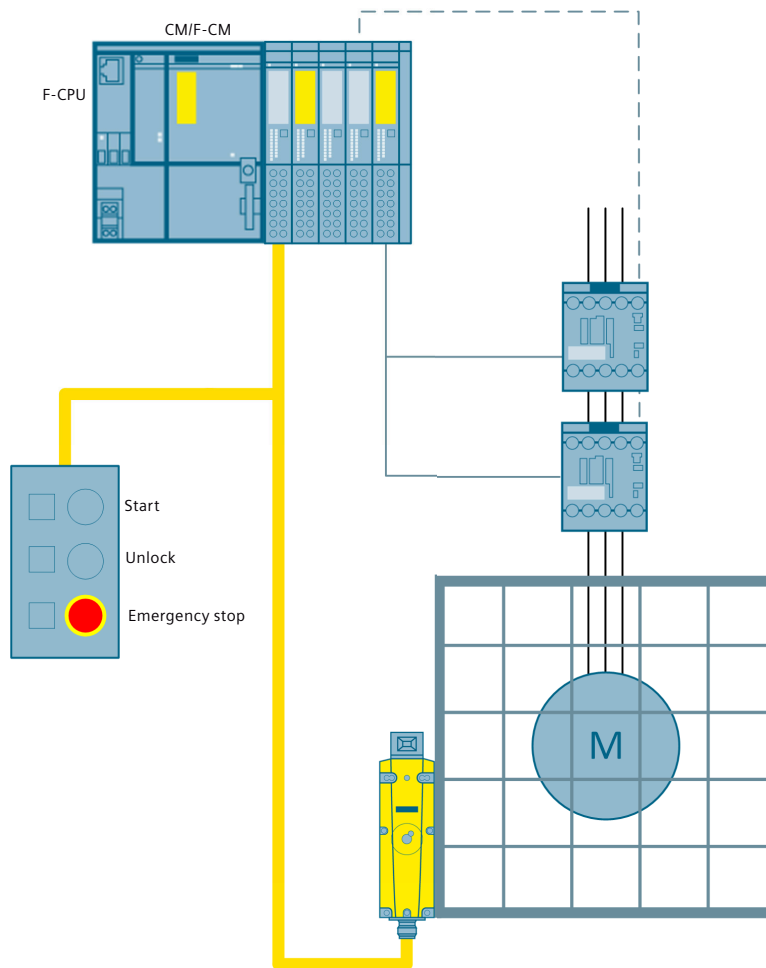
Figure 3-55 Emergency stop shutdown up to SIL 3 or PL e and protective door monitoring up to SIL 2 or PL d with tumbler via AS-i ET 200SP Master
