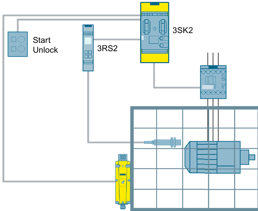
Figure 3-47 Safe temperature monitoring and protective door monitoring with tumbler up to SIL 1 or PL c with a 3RS2 temperature monitoring relay and 3SK2 safety relay
