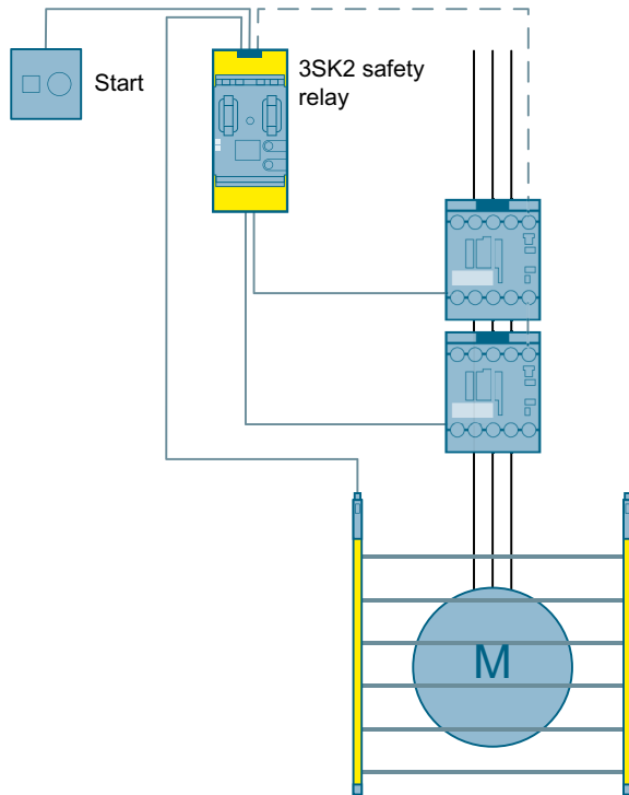
Figure 3-36 Access monitoring using a light curtain to SIL 3 or PL e with a 3SK2 safety relay
