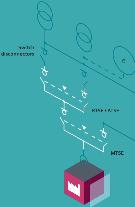
Figure 12: Transfer switches for switching over between networks or loads
