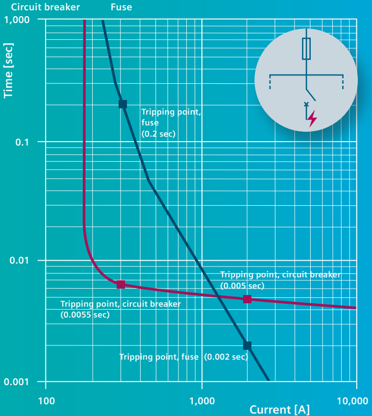
Figure 4: Combination of characteristic curves for partial selectivity
