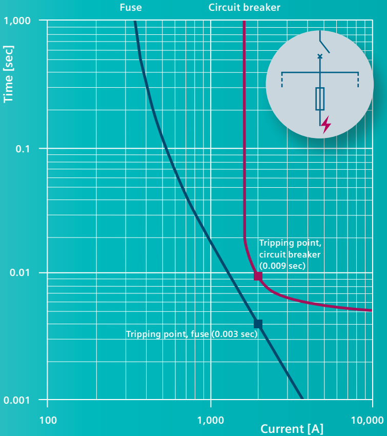
Figure 3: Combination of characteristic curves for full selectivity
