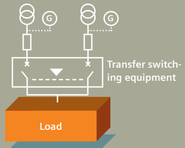
Figure 14: Transfer switching with switch disconnectors and circuit breakers
