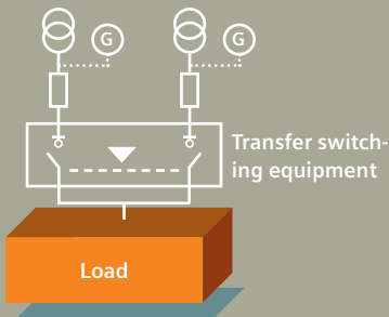
Figure 14: Transfer switching with switch disconnectors and circuit breakers
