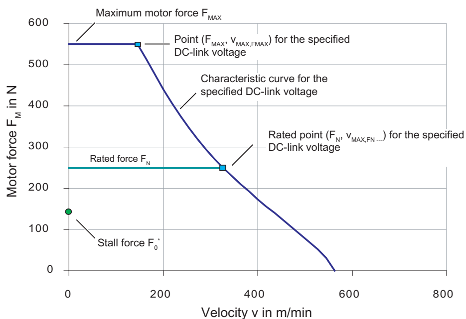
Figure 15-1 Characteristic curve_motor thrust over velocity, schematic
