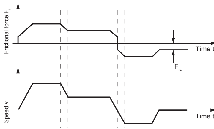
Figure 7-4 Example of frictional forces
