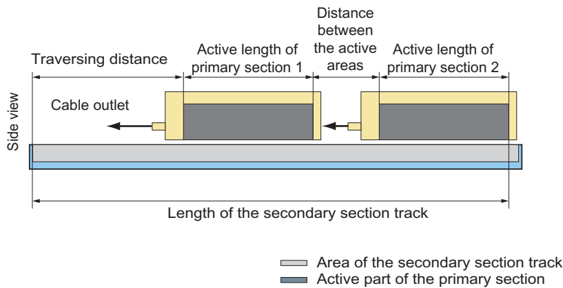
Figure 7-11 Determination of the length of the secondary section with several primary sections
