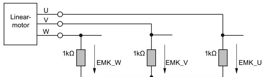
Figure 10-6 Configuration for taking the measurements
