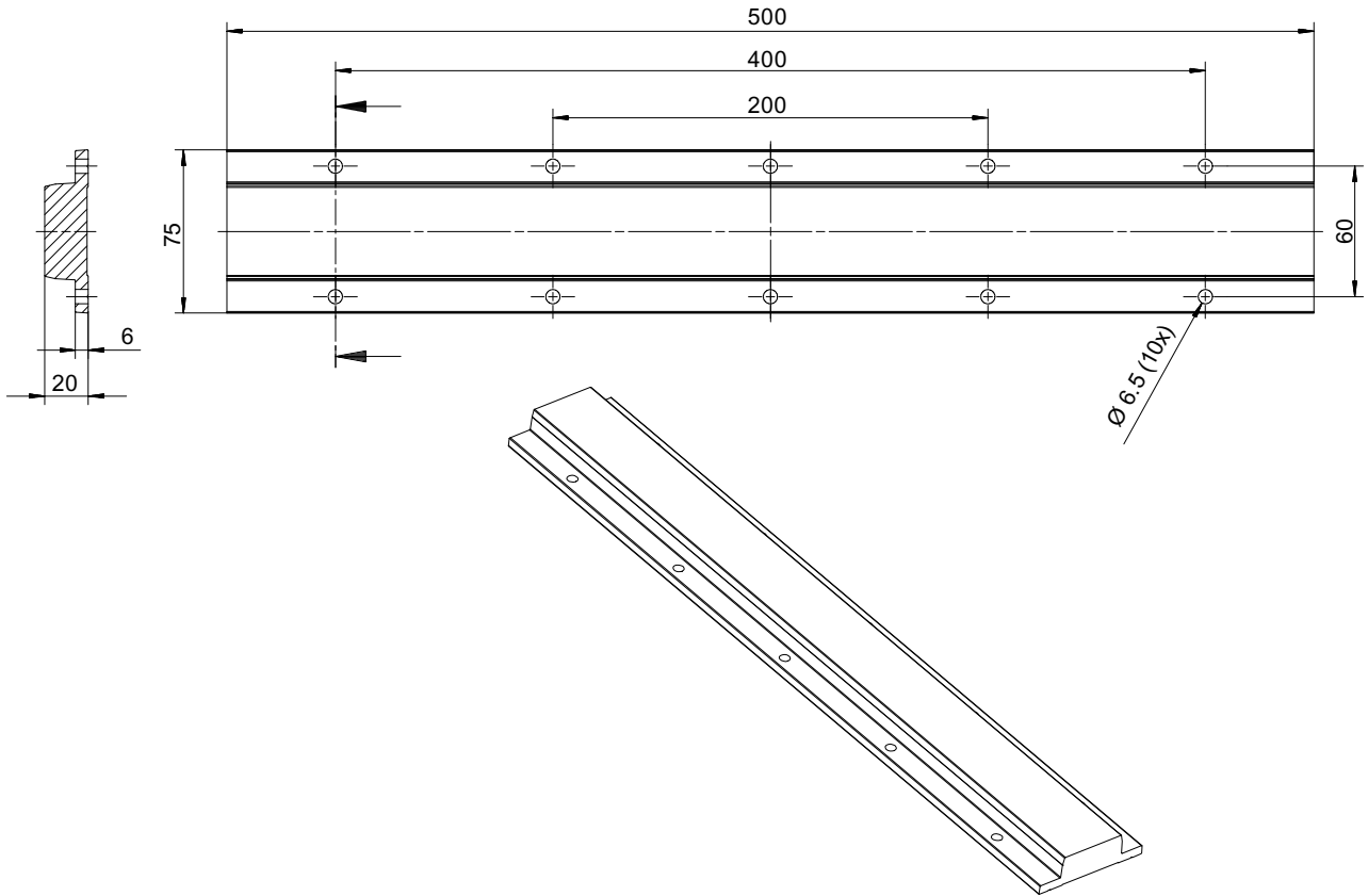
Figure 16-12 Installation dimensions of the secondary section in the case of the 1FN6003-1SF00-0AA0
