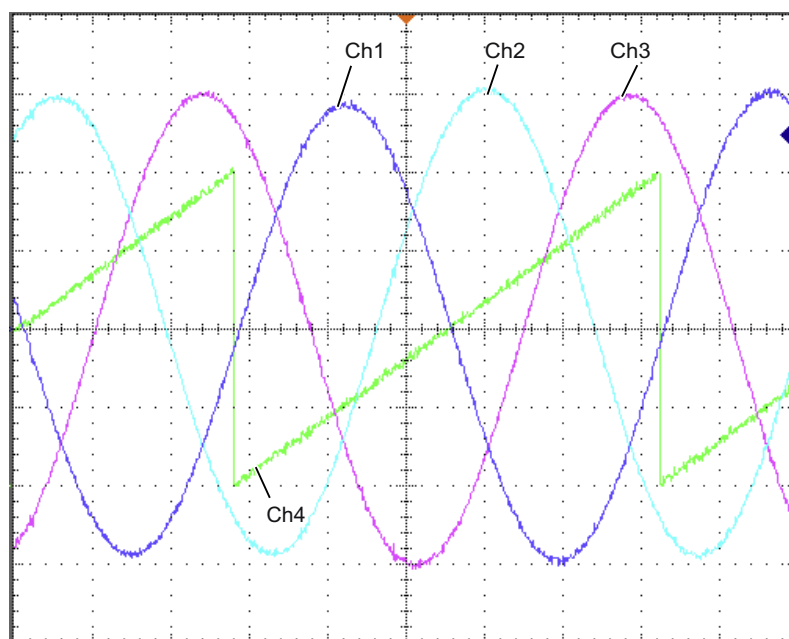
Figure 10-8 Oscillogram
